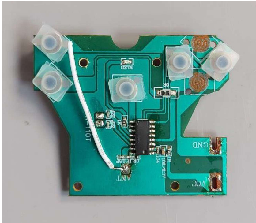
Internal View
