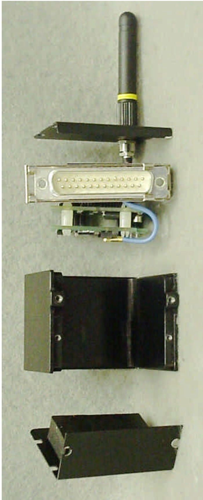
Photo 4. EUT, Exploded View, Front View
