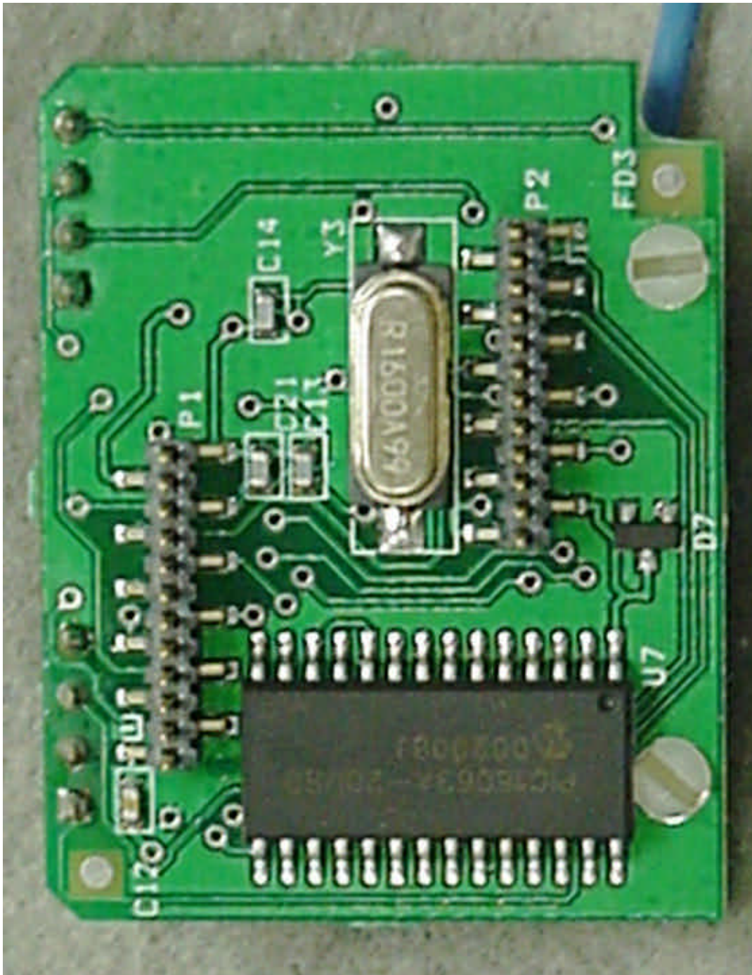
Photo 8. EUT, Top View of Transceiver Board
