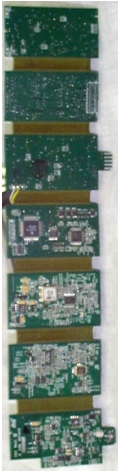
Photo 10. Complete Circuit Board – Side 1
