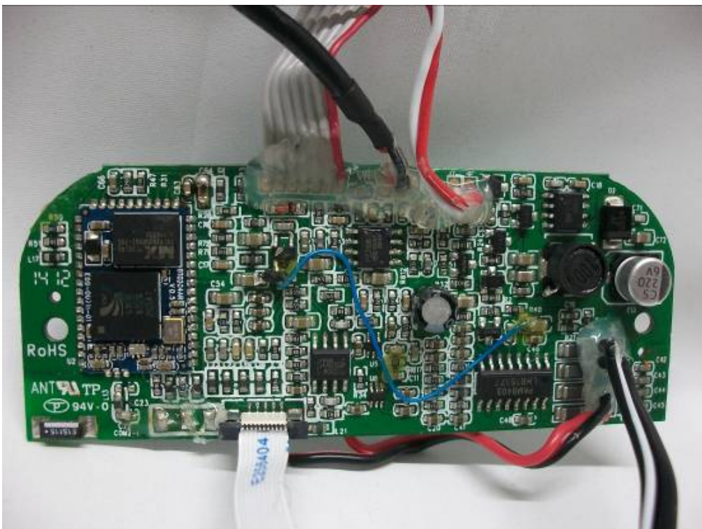
INTERNAL PHOTO OF TX – 4
