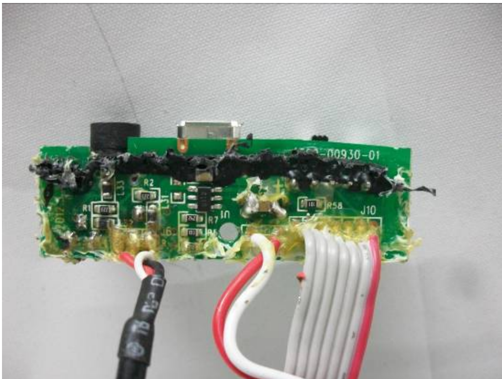
INTERNAL PHOTO OF TX – 8
