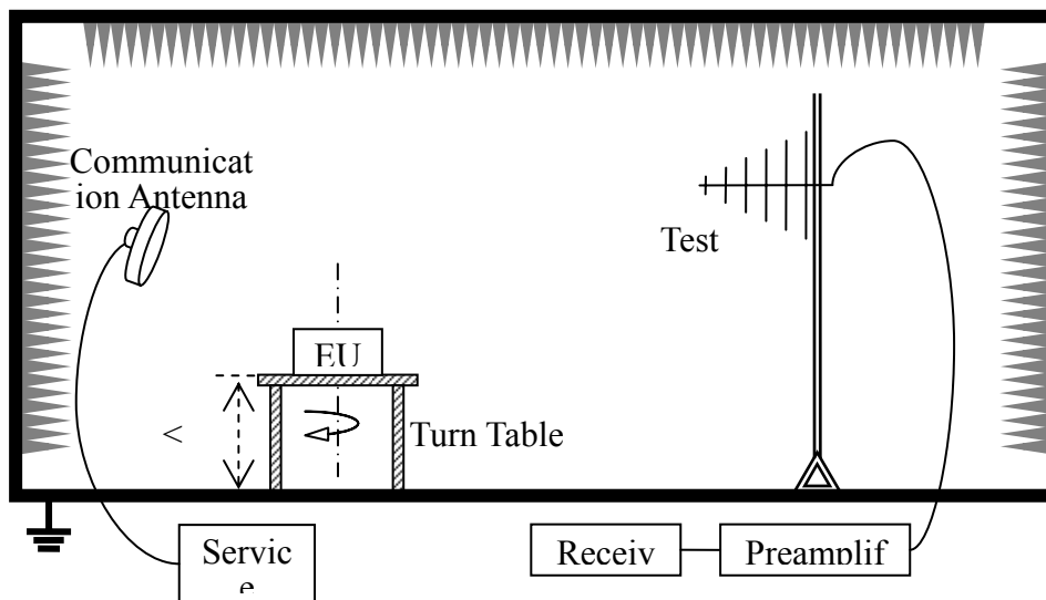
Radiated emissions below 30MHz
