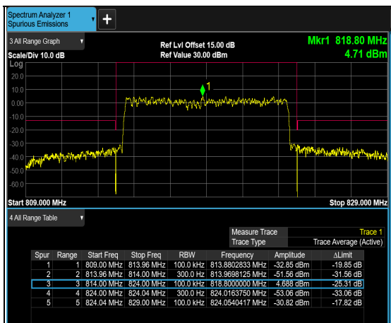
FULL (819MHz)
