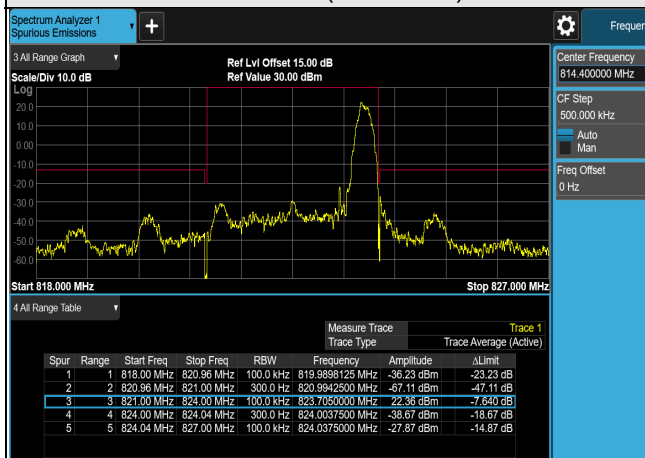
1RB#MAX (822.5MHz)
