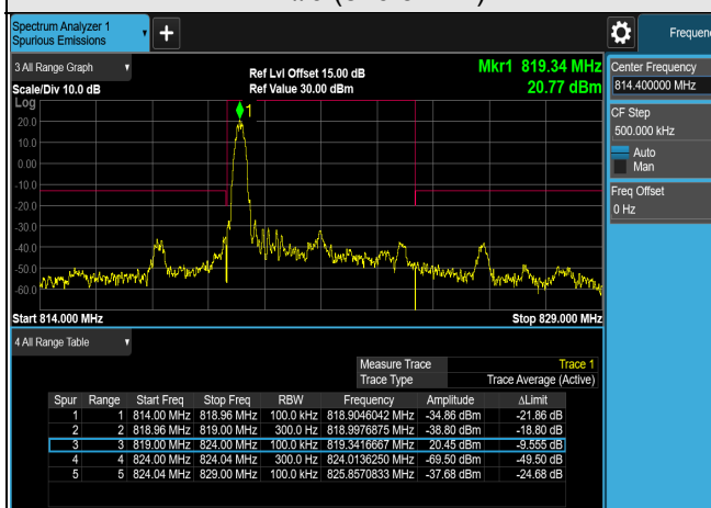
1RB#0 (821.5MHz)
