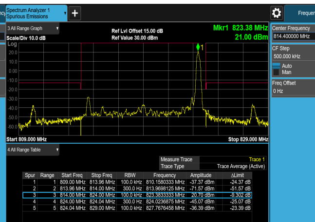
1RB#MAX (819MHz)
