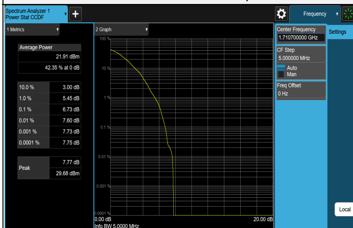
64QAM CH 19957 (1710.7MHz)
