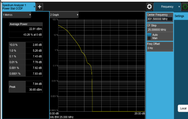
16QAM CH 26865 (831.5MHz)
