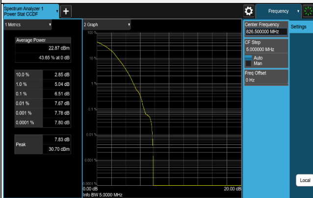
16QAM CH 26815 (826.5MHz)
