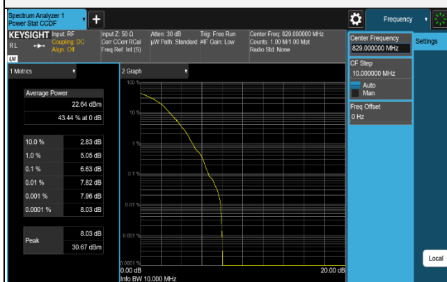
16QAM CH 20450 (829MHz)
