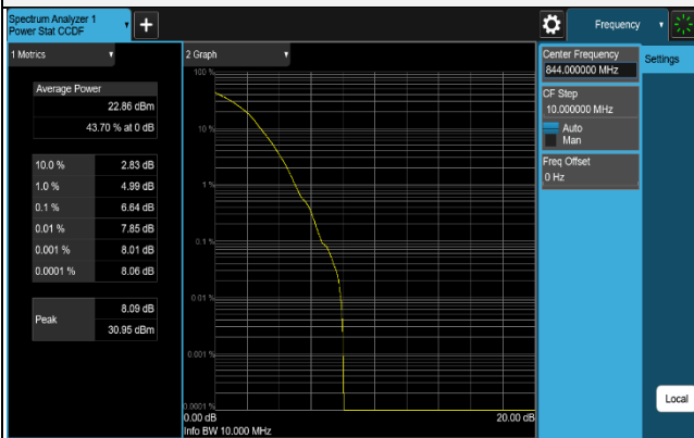
16QAM CH 26990 (844MHz)
