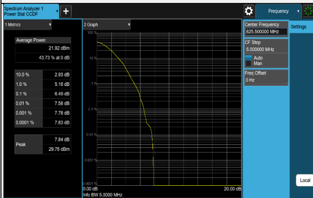
64QAM CH 26805 (825.5MHz)
