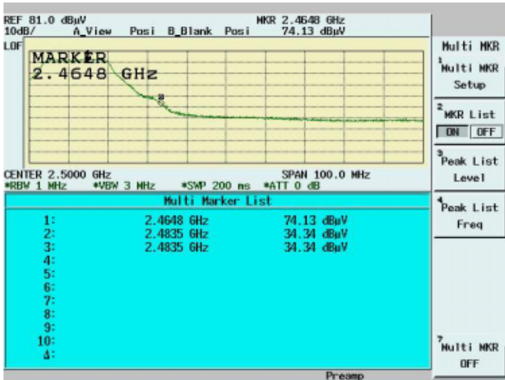
Band Edge measurement for radiated emission in Restricted Band(Radiated) Average Mode (Channel 11)
