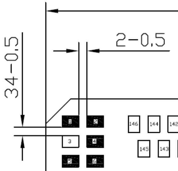
Pin1 location
