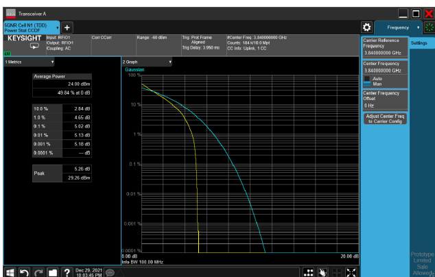
5G NR n77_CH656000_80M_1RB_QPSK_Ratio
