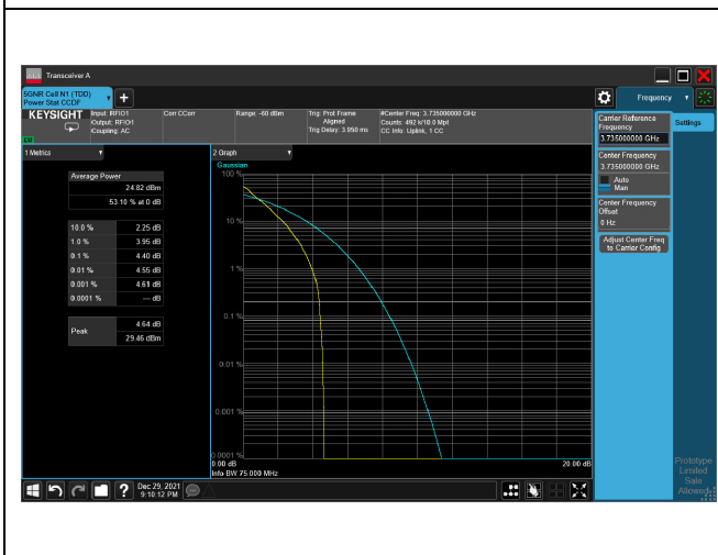
5G NR n77_CH649000_70M_1RB_16-QAM_Ratio
