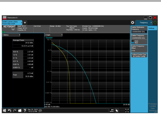
5G NR n77_CH656000_70M_1RB_16-QAM_Ratio
