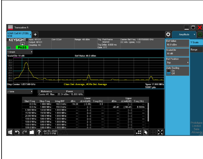
5G NR n2_CH3805000_15M_pi/2 BPSK_1RB78
