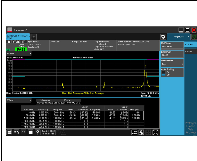
5G NR n77_CH 632668_80M_QPSK_1RB0
