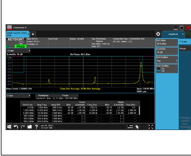
5G NR n77_CH 634000_80M_QPSK_1RB216
