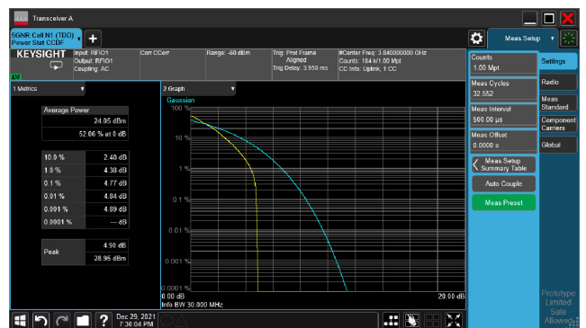
5G NR n77_CH656000_30M_1RB_16-QAM_Ratio
