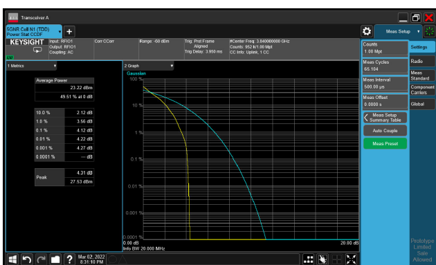
5G NR n77_CH656000_15M_1RB_QPSK_Ratio
