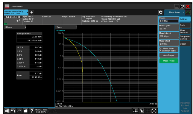
5G NR n77_CH656000_15M_1RB_16-QAM_Ratio
