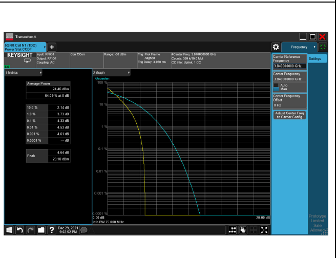
5G NR n77_CH656000_60M_1RB_16-QAM_Ratio
