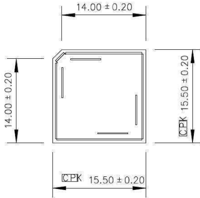
Figure 4-1. Top view
