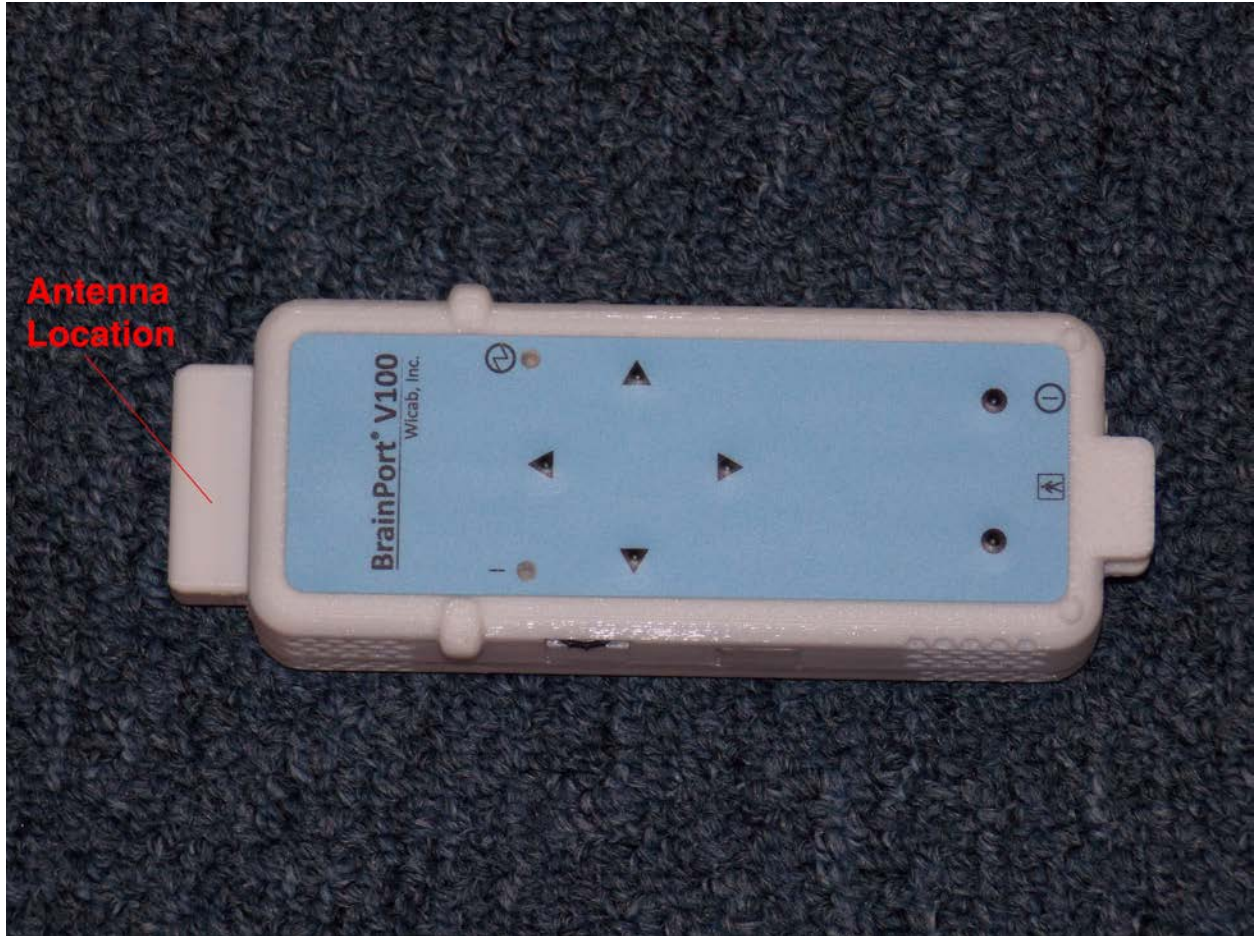
Antenna Location
