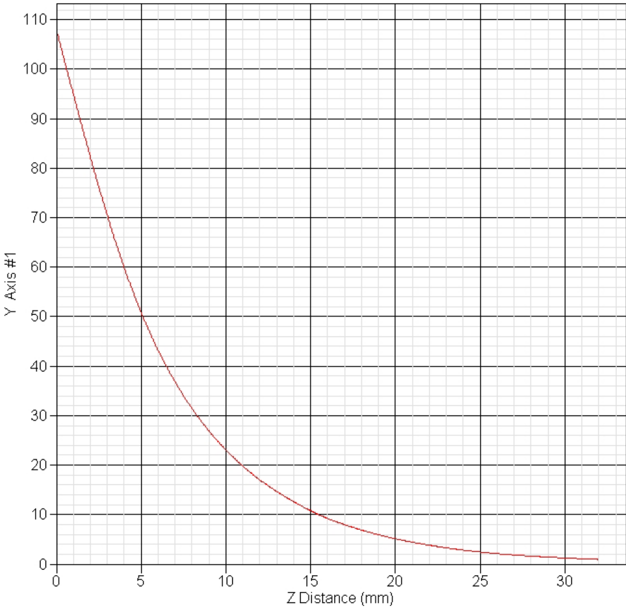
SAR-Z Axis at Hotspot x:9.00 y:-2.00
