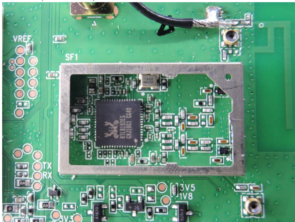
(16) EUT Photo (WIFI module)
