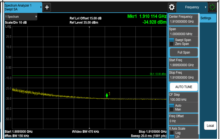
FULL (1902.5 MHz)
