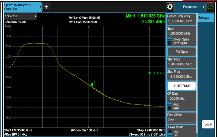
1RB (1907.5 MHz)
