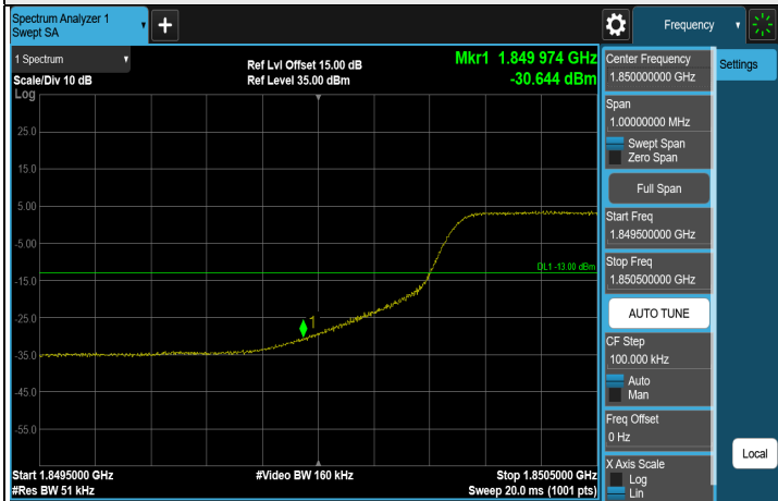
FULL (1852.5 MHz)
