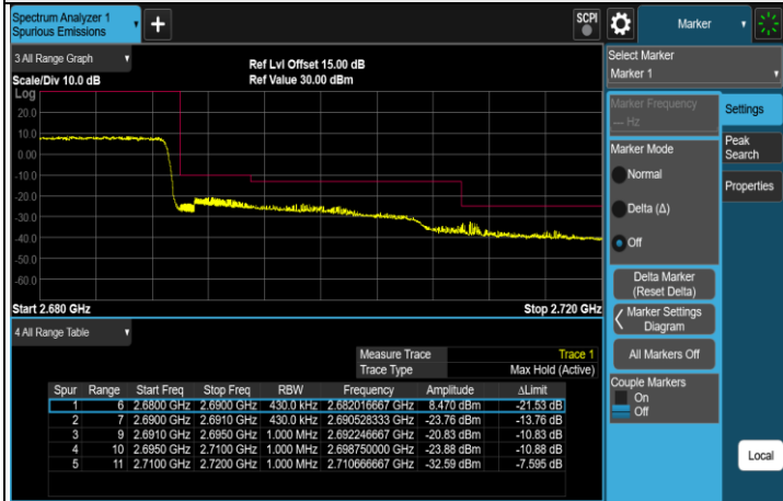
FULL CH 41490 (2680 MHz)
