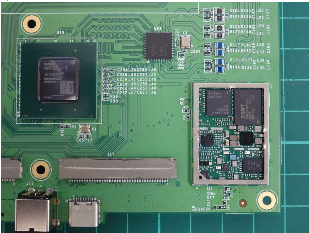
(73) EUT Photo
