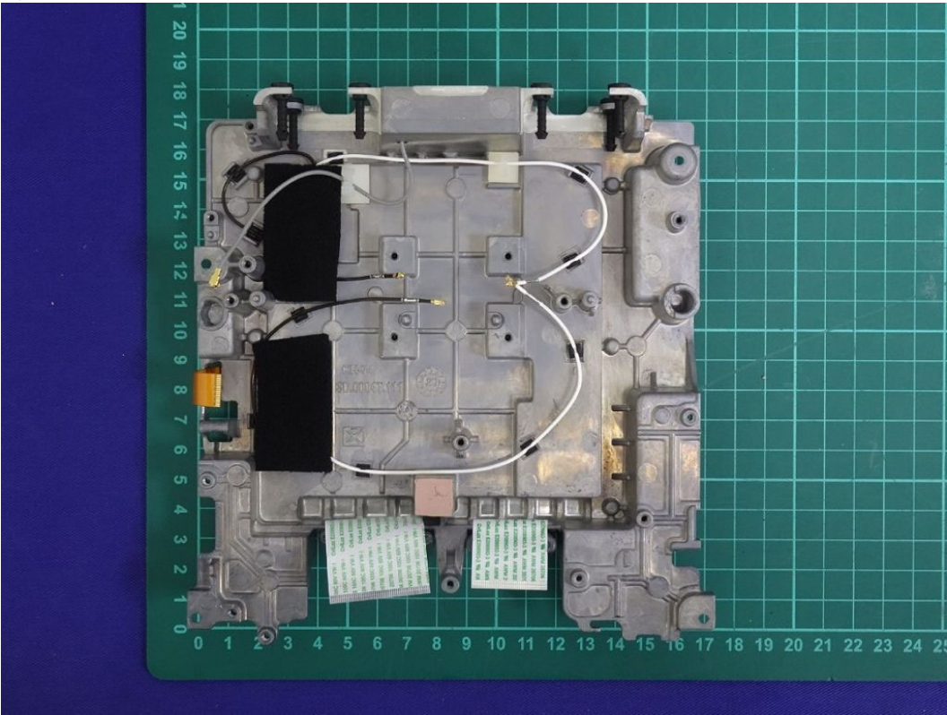
(76) EUT Photo
