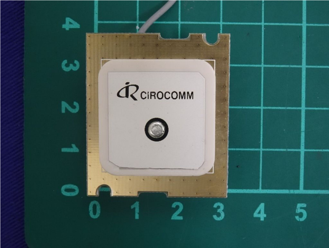
(80) EUT Photo
