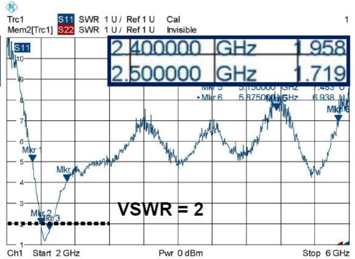
Antenna 2
