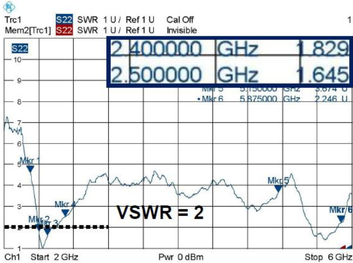
Antenna 1
