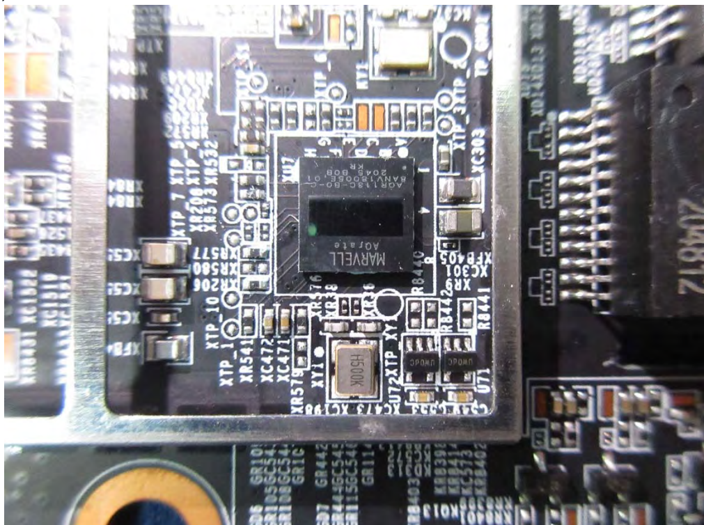
(68) EUT Photo
