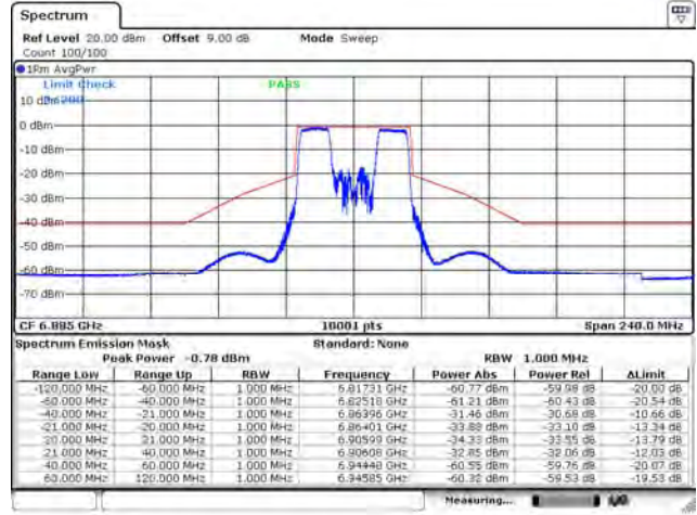
802.11ax (40 MHz) / Ant. 1 / 6885 MHz
