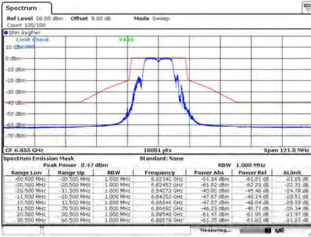
802.11ax (20 MHz) / Ant. 3 / 6855 MHz
