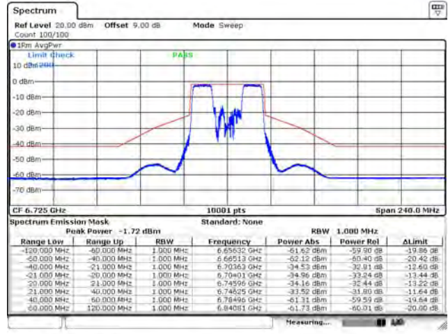
802.11ax (40 MHz) / Ant. 2 / 6725 MHz
