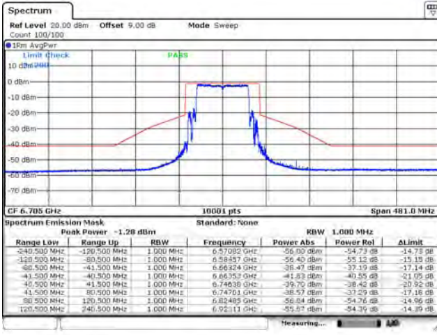
802.11ax (80 MHz) / Ant. 2 / 6705 MHz
