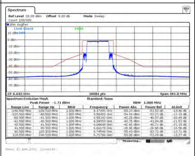
802.11ax (80 MHz) / Ant. 0 / 6625 MHz
