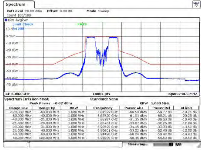
802.11ax (40 MHz) / Ant. 2 / 6885 MHz
