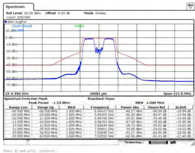
802.11ax (20 MHz) / Ant. 0 / 6995 MHz
