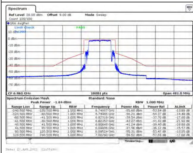
802.11ax (80 MHz) / Ant. 3 / 6865 MHz
