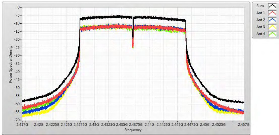
Channel 6 (2437MHz)
