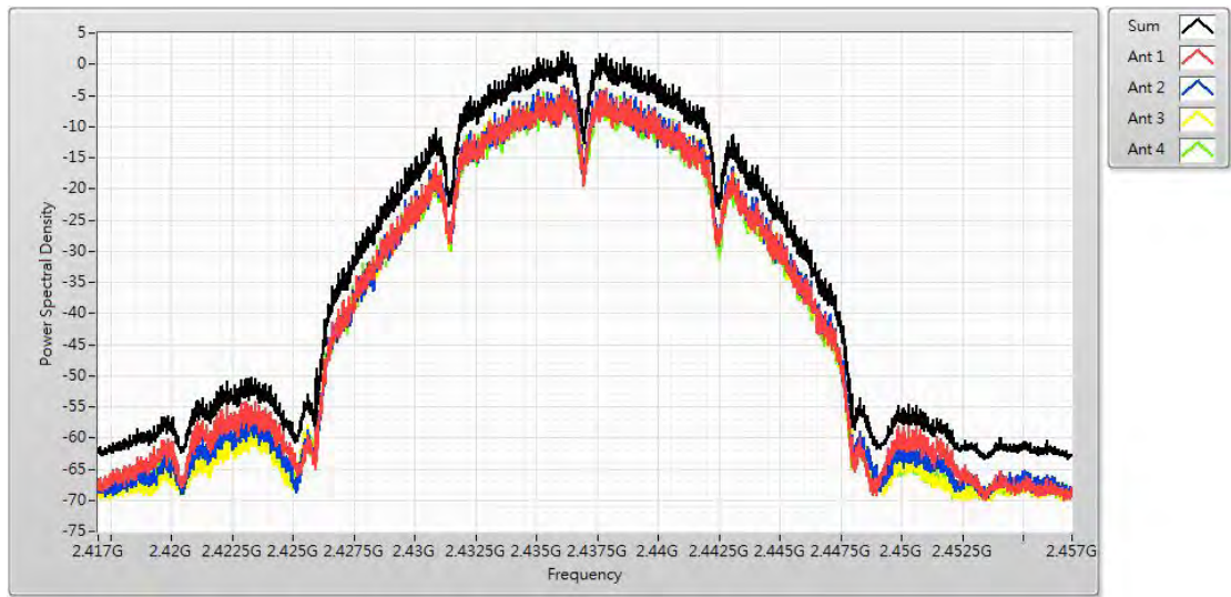
Channel 6 (2437MHz)
