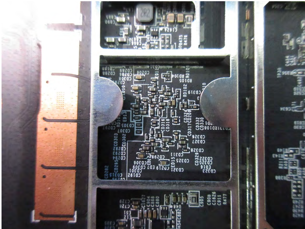
(73) EUT Photo
