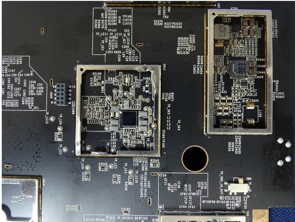
(79) EUT Photo
