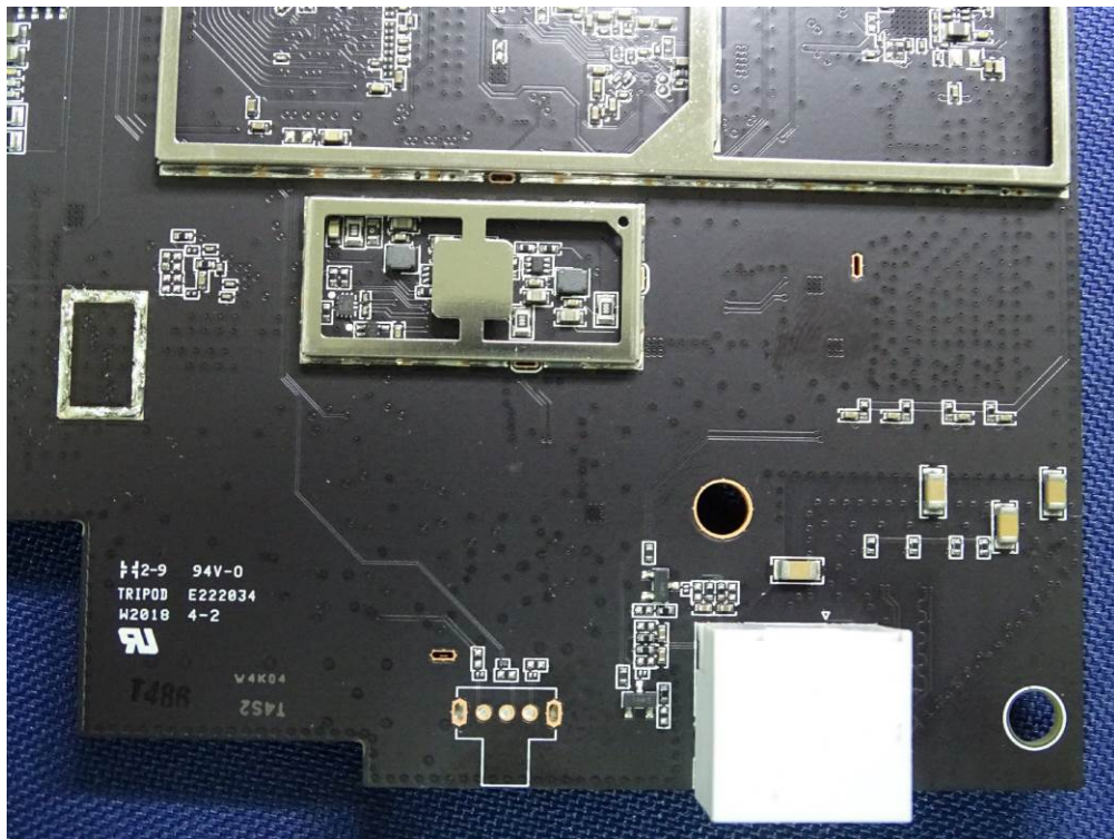
(55) EUT Photo
