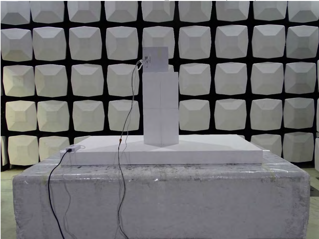
Back View of Radiated Test _ 30MHz-1GHz (Mode 1)
