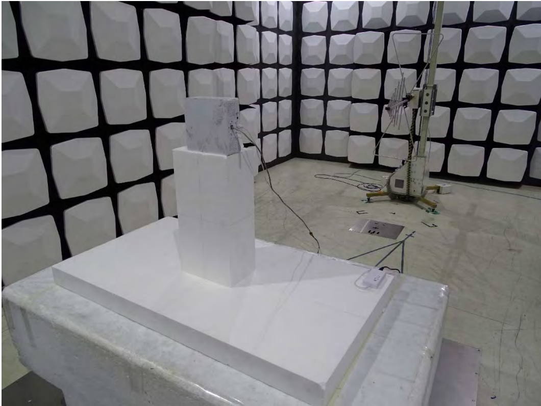
Front View of Radiated Test _ 30MHz-1GHz (Mode 1)
