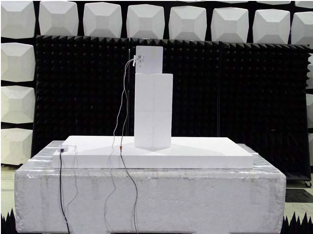
Back View of Radiated Test (Horn) _ 1-18GHz
