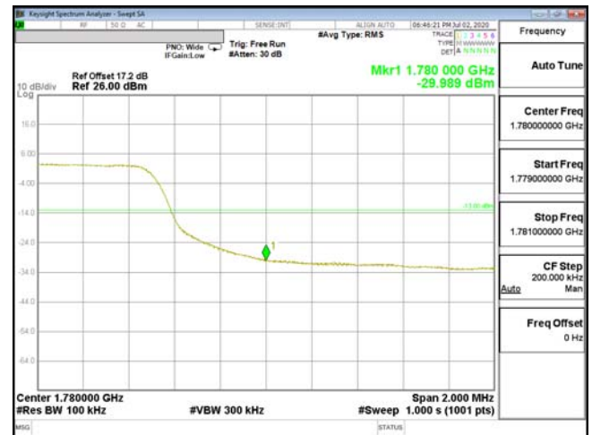
EDGE-ENDC_66A_n5-QPSK_10M(50,0)_CH132622_1775
