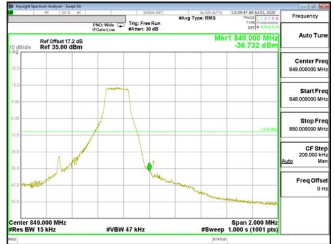
EDGE-ENDC_5A_n2-16QAM_1.4M(1,5)_CH20643_848.3
