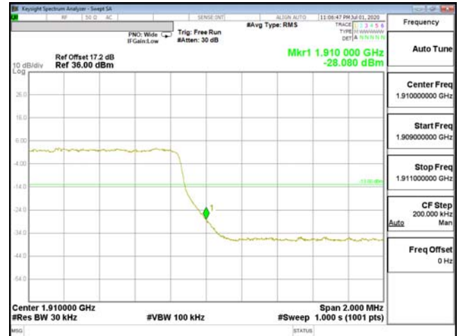
EDGE-ENDC_2A_n5-16QAM_3M(15,0)_CH19185_1908.5
