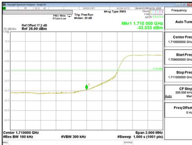
EDGE-ENDC_66A_n5-QPSK_10M(50,0)_CH132022_1715
