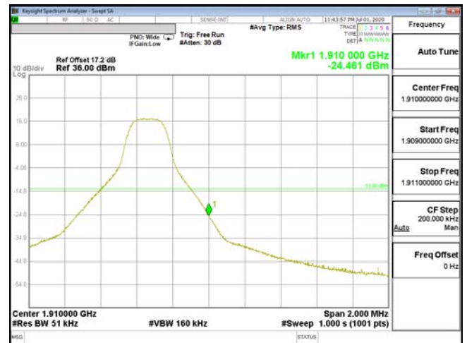
EDGE-ENDC_2A_n5-16QAM_5M(1,24)_CH19175_1907.5
