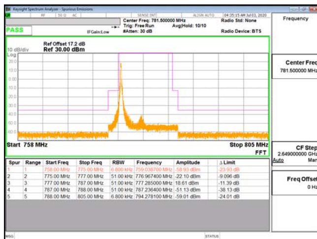
EDGE-ENDC_13A_n66-16QAM_5M(1,0)_CH23205_779.5
