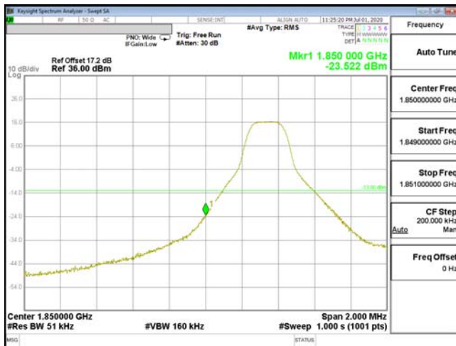
EDGE-ENDC_2A_n5-64QAM_5M(1,0)_CH18625_1852.5
