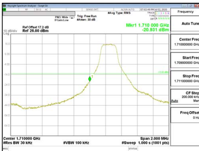
EDGE-ENDC_66A_n5-16QAM_3M(1,0)_CH131987_1711.5
