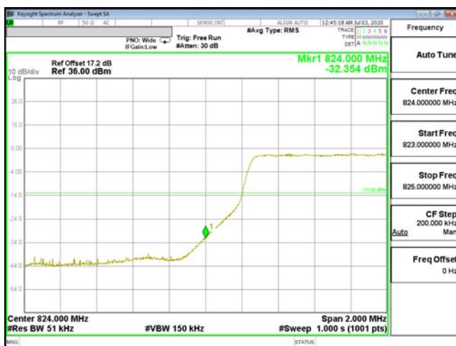
EDGE-ENDC_5A_n2-QPSK_5M(25,0)_CH20425_826.5
