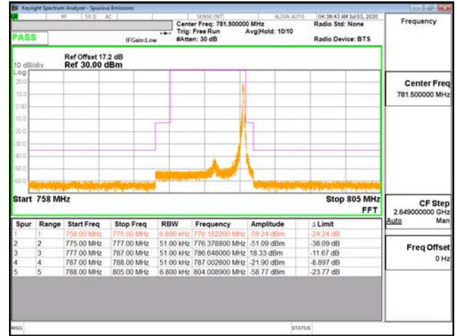
EDGE-ENDC_13A_n66-QPSK_5M(1,24)_CH23255_784.5
