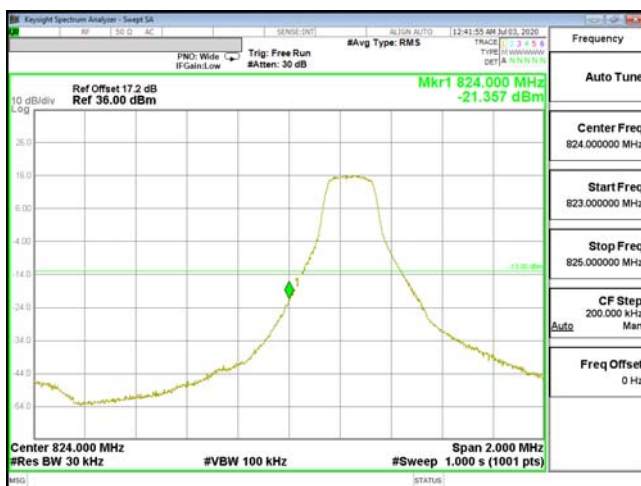
EDGE-ENDC_5A_n2-16QAM_3M(1,0)_CH20415_825.5
