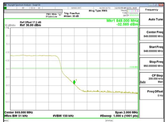
EDGE-ENDC_5A_n2-16QAM_5M(25,0)_CH20625_846.5
