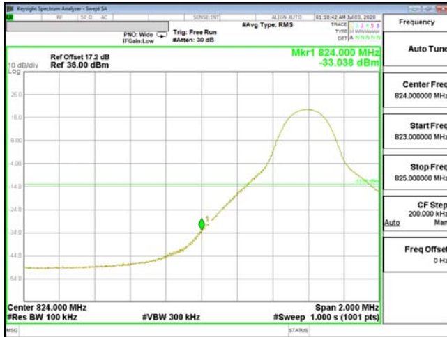
EDGE-ENDC_5A_n2-QPSK_10M(1,0)_CH20450_829
