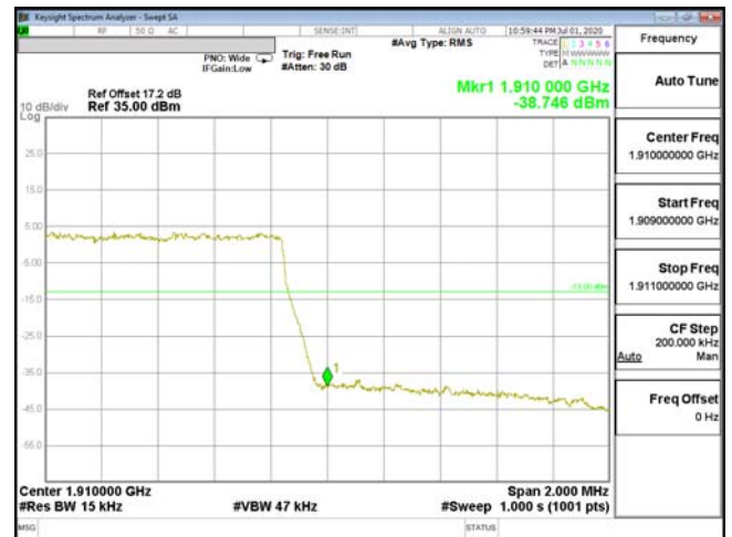
EDGE-ENDC_2A_n5-64QAM_1.4M(6,0)_CH19193_1909.3
