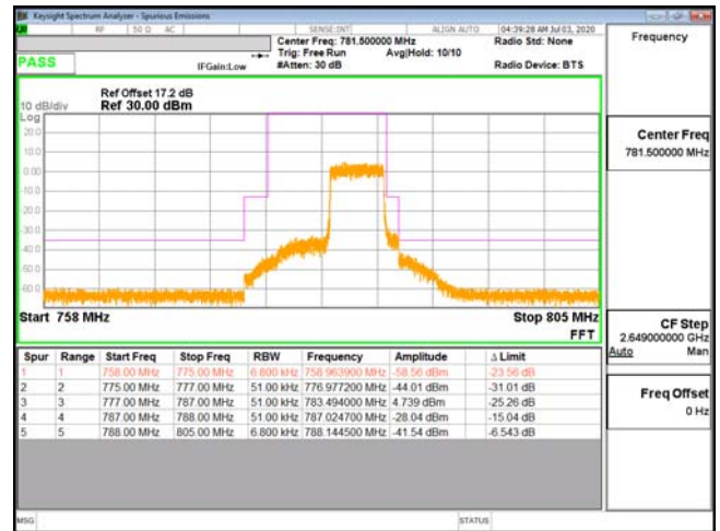
EDGE-ENDC_13A_n66-16QAM_5M(25,0)_CH23255_784.5
