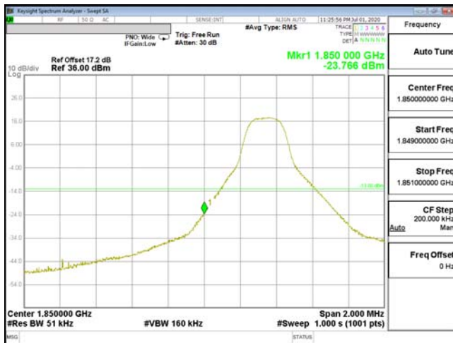
EDGE-ENDC_2A_n5-16QAM_5M(1,0)_CH18625_1852.5
