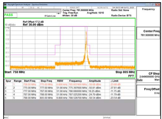
EDGE-ENDC_13A_n66-16QAM_5M(1,24)_CH23255_784.5
