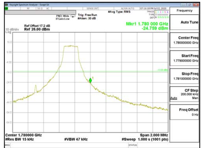
EDGE-ENDC_66A_n5-16QAM_1.4M(1,5)_CH132665_1779.3
