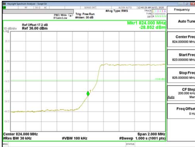
EDGE-ENDC_5A_n2-16QAM_3M(15,0)_CH20415_825.5
