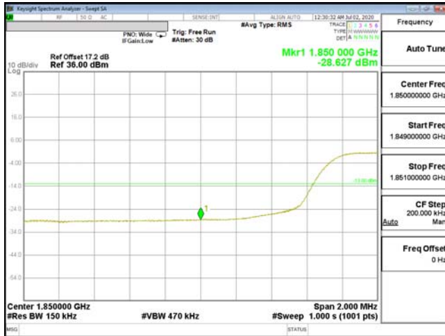
EDGE-ENDC_2A_n5-64QAM_15M(75,0)_CH18675_1857.5
