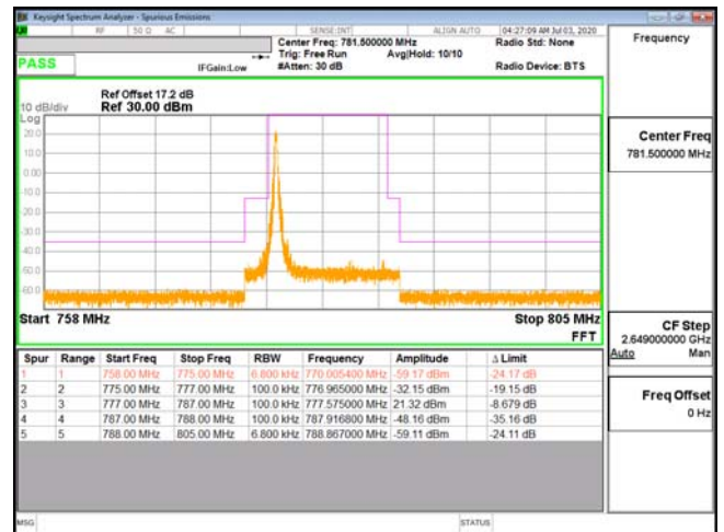
EDGE-ENDC_13A_n66-16QAM_10M(1,0)_CH23230_782
