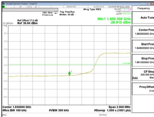
EDGE-ENDC_2A_n5-16QAM_10M(50,0)_CH18650_1855
