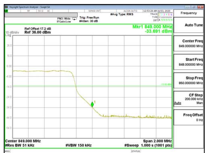
EDGE-ENDC_5A_n2-64QAM_5M(25,0)_CH20625_846.5
