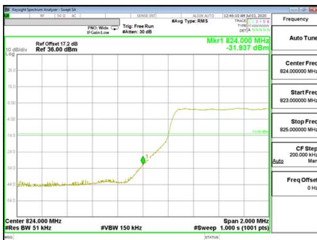
EDGE-ENDC_5A_n2-16QAM_5M(25,0)_CH20425_826.5
