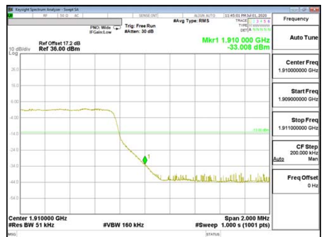
EDGE-ENDC_2A_n5-64QAM_5M(25,0)_CH19175_1907.5
