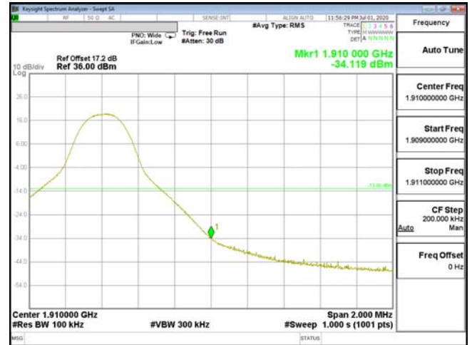
EDGE-ENDC_2A_n5-64QAM_10M(1,49)_CH19150_1905
