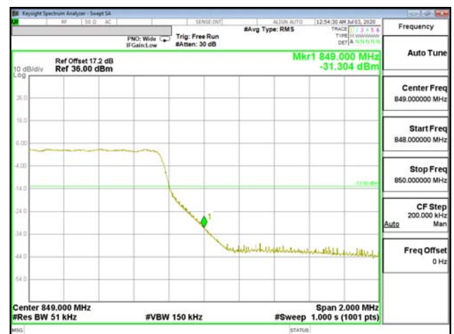
EDGE-ENDC_5A_n2-QPSK_5M(25,0)_CH20625_846.5
