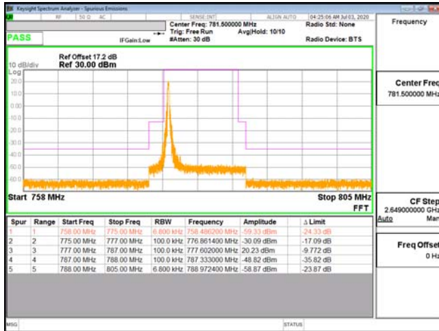
EDGE-ENDC_13A_n66-64QAM_10M(1,0)_CH23230_782
