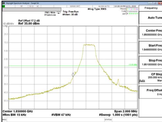
EDGE-ENDC_2A_n5-16QAM_1.4M(1,0)_CH18607_1850.7
