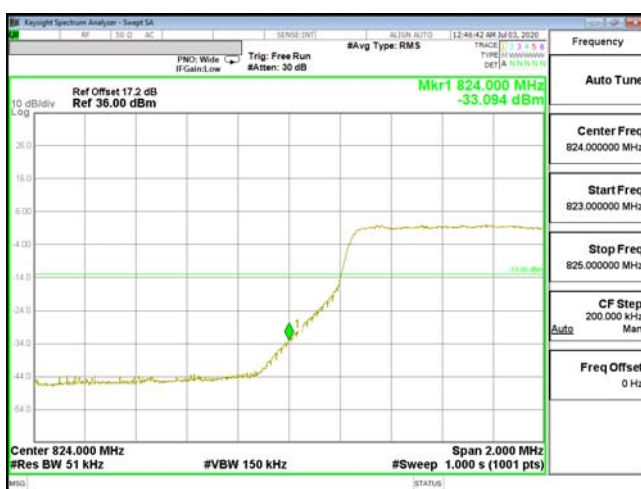
EDGE-ENDC_5A_n2-64QAM_5M(25,0)_CH20425_826.5
