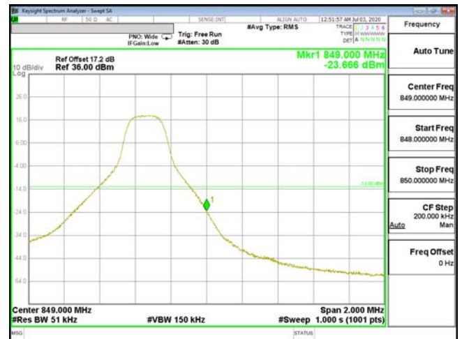
EDGE-ENDC_5A_n2-16QAM_5M(1,0)_CH20625_846.5
