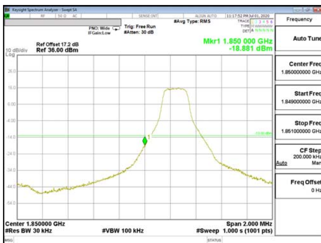
EDGE-ENDC_2A_n5-16QAM_3M(1,0)_CH18615_1851.5
