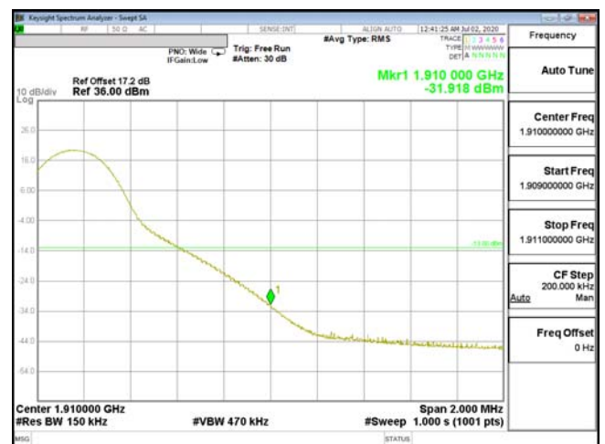
EDGE-ENDC_2A_n5-64QAM_15M(1,74)_CH19125_1902.5
