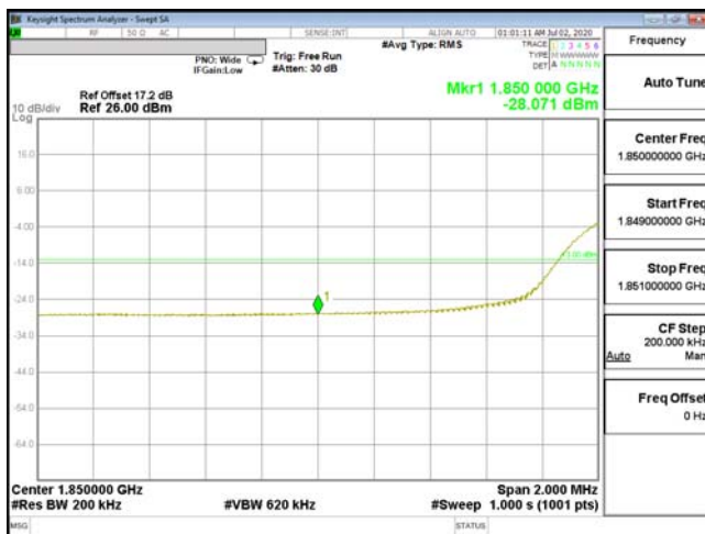
EDGE-ENDC_2A_n5-64QAM_20M(100,0)_CH18700_1860
