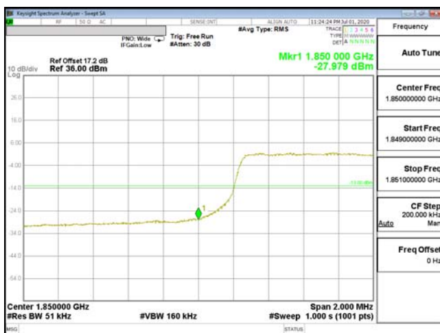
EDGE-ENDC_2A_n5-64QAM_5M(25,0)_CH18625_1852.5
