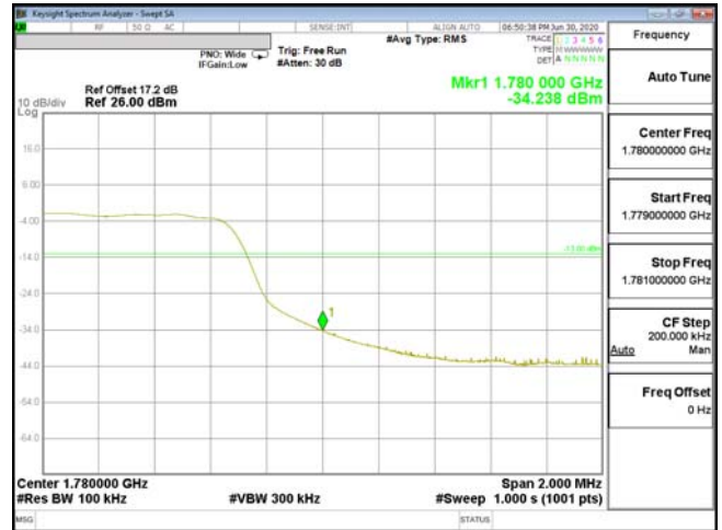
EDGE-ENDC_13A_n66-256QAM_10M(50,2)_CH355000_1775
