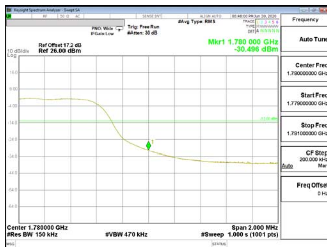
EDGE-ENDC_13A_n66-16QAM_15M(75,4)_CH354500_1772.5
