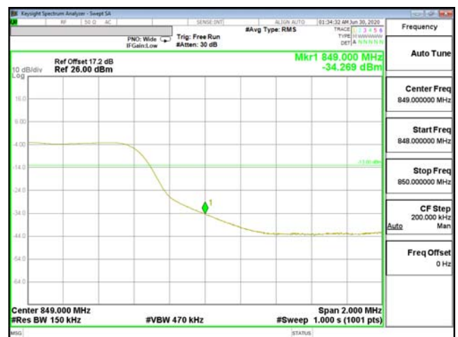
EDGE-ENDC_2A_n5-256QAM_15M(75,4)_CH168300_841.5
