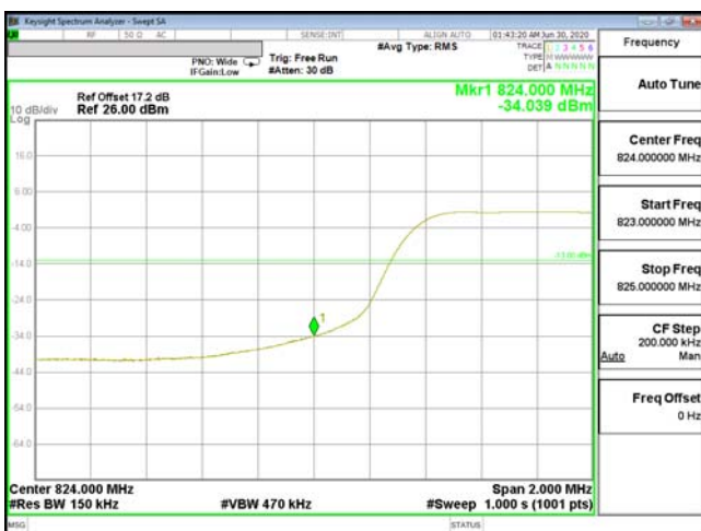
EDGE-ENDC_2A_n5-64QAM_15M(75,0)_CH166300_831.5
