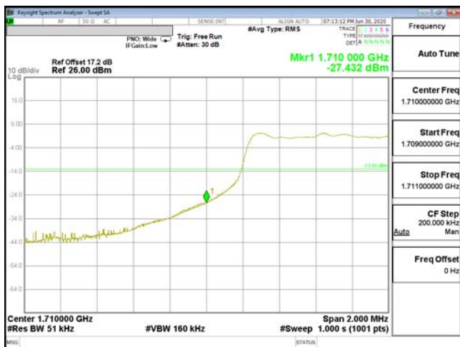
EDGE-ENDC_13A_n66-16QAM_5M(25,0)_CH342500_1712.5
