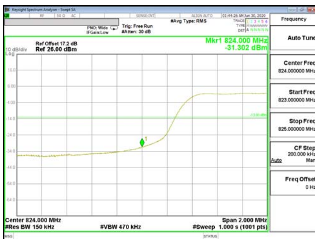
EDGE-ENDC_2A_n5-QPSK_15M(75,0)_CH166300_831.5
