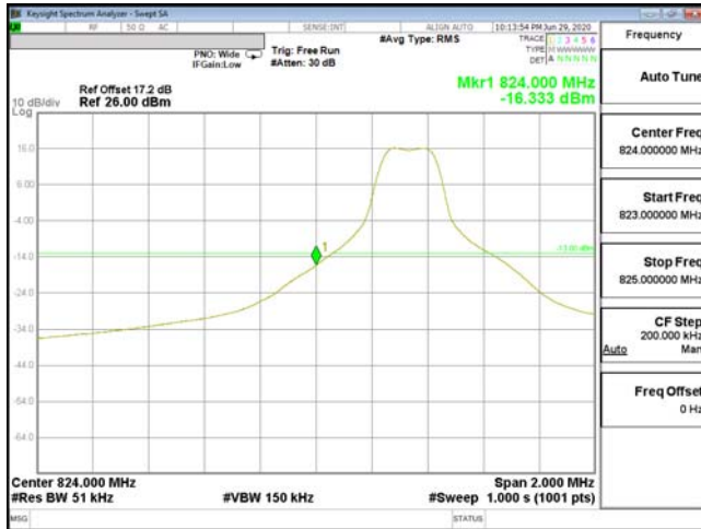
EDGE-ENDC_2A_n5-QPSK_5M(1,0)_CH165300_826.5
