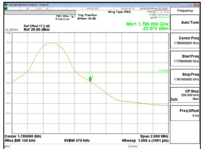
EDGE-ENDC_13A_n66-256QAM_15M(1,78)_CH354500_1772.5
