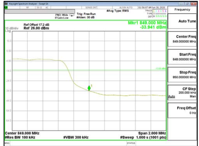
EDGE-ENDC_2A_n5-256QAM_10M(50,2)_CH168800_844
