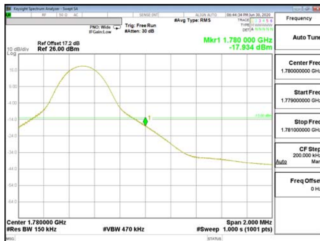
EDGE-ENDC_13A_n66-16QAM_15M(1,78)_CH354500_1772.5
