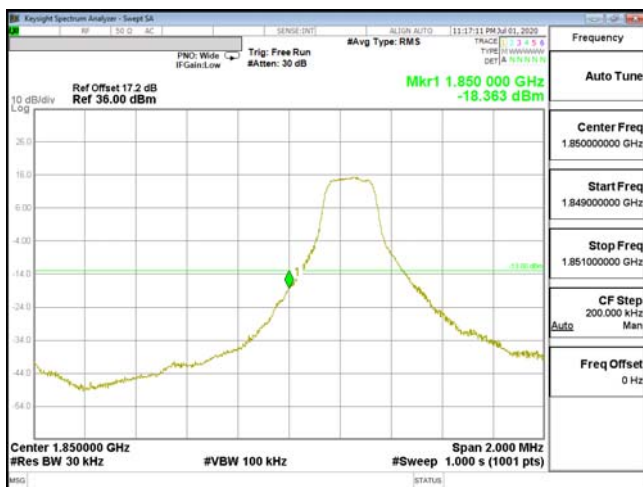
EDGE-ENDC_2A_n5-QPSK_3M(1,0)_CH18615_1851.5
