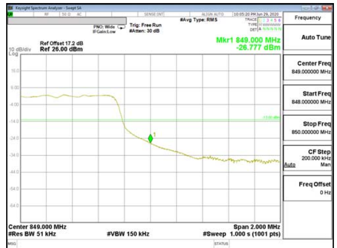
EDGE-ENDC_2A_n5-16QAM_5M(25,0)_CH169300_846.5
