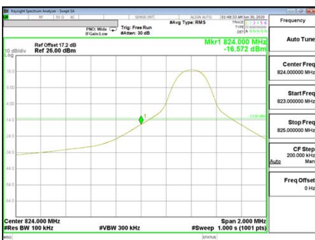
EDGE-ENDC_2A_n5-64QAM_10M(1,0)_CH165800_829
