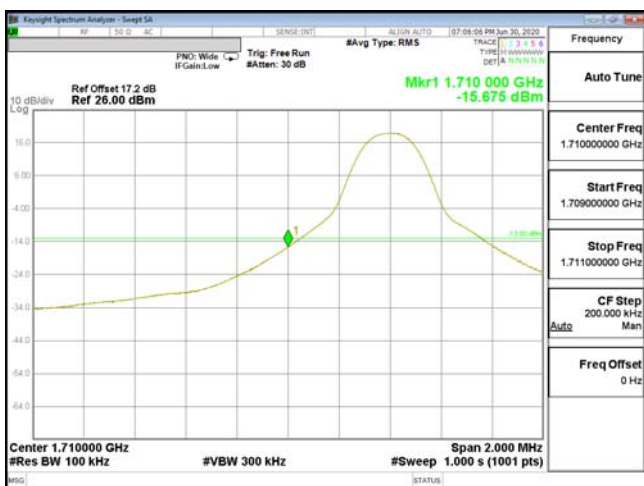
EDGE-ENDC_13A_n66-QPSK_10M(1,0)_CH343000_1715
