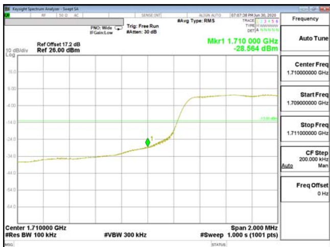
EDGE-ENDC_13A_n66-PI2-BPSK_10M(50,0)_CH343000_1715
