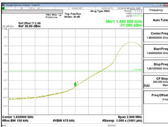
EDGE-ENDC_2A_n5-QPSK_15M(1,0)_CH18675_1857.5
