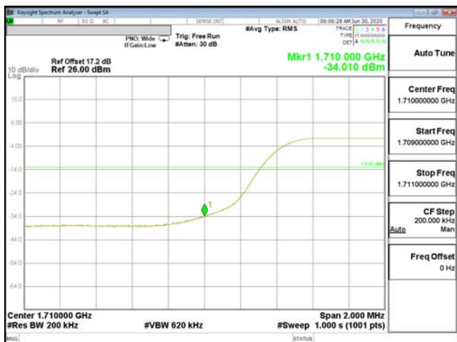
EDGE-ENDC_13A_n66-64QAM_20M(100,0)_CH344000_1720
