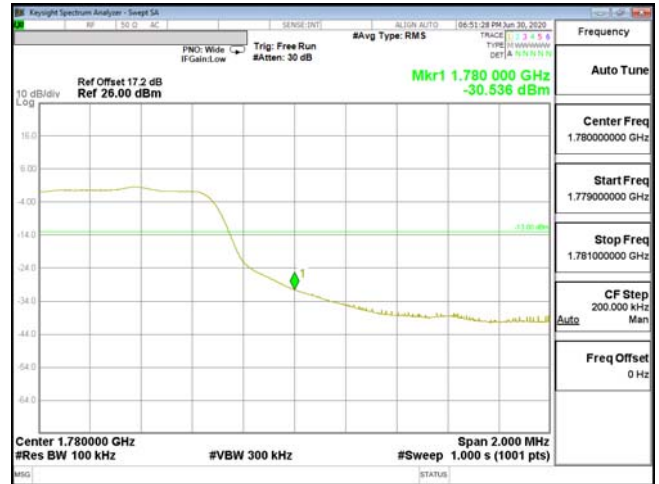
EDGE-ENDC_13A_n66-64QAM_10M(50,2)_CH355000_1775
