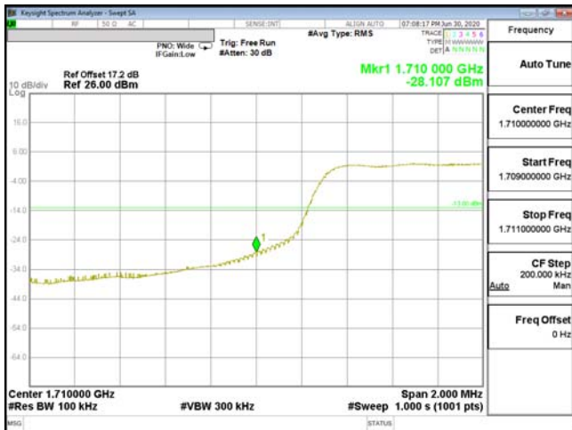
EDGE-ENDC_13A_n66-QPSK_10M(50,0)_CH343000_1715
