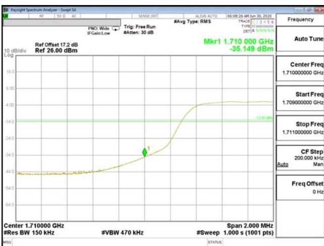
EDGE-ENDC_13A_n66-256QAM_15M(75,0)_CH343500_1717.5
