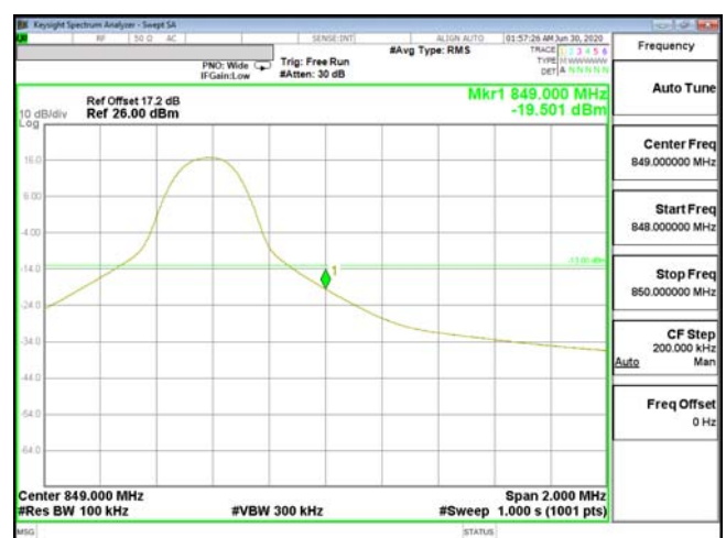
EDGE-ENDC_2A_n5-64QAM_10M(1,51)_CH168800_844
