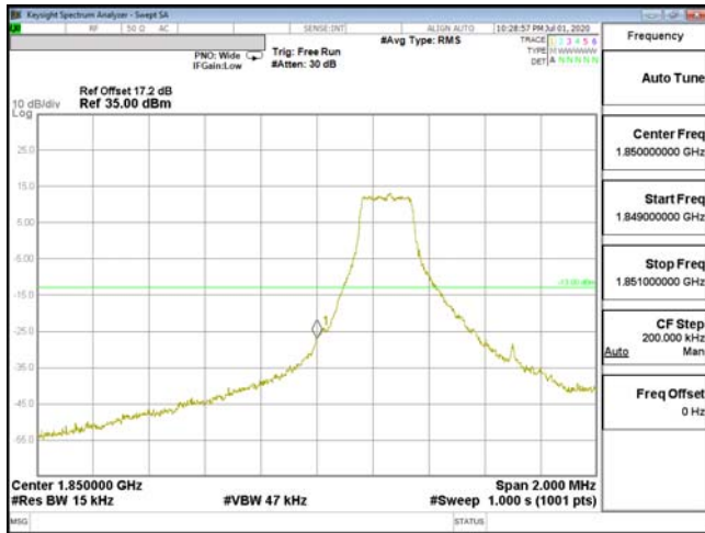
EDGE-ENDC_2A_n5-QPSK_1.4M(1,0)_CH18607_1850.7
