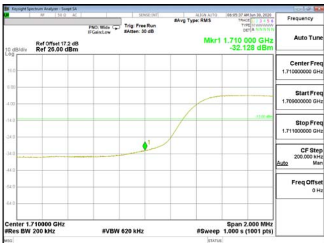
EDGE-ENDC_13A_n66-QPSK_20M(100,0)_CH344000_1720
