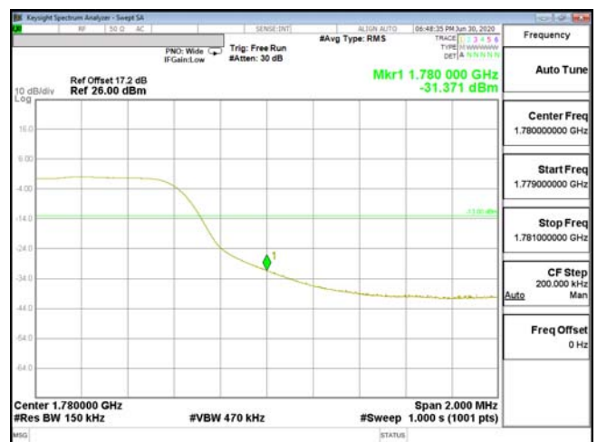
EDGE-ENDC_13A_n66-64QAM_15M(75,4)_CH354500_1772.5
