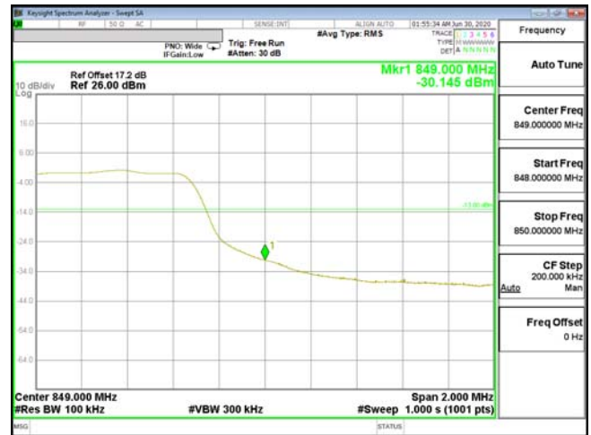
EDGE-ENDC_2A_n5-64QAM_10M(50,2)_CH168800_844
