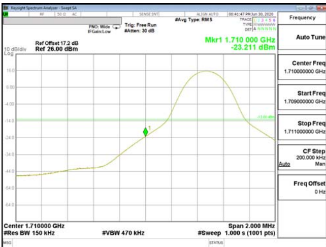
EDGE-ENDC_13A_n66-256QAM_15M(1,0)_CH343500_1717.5
