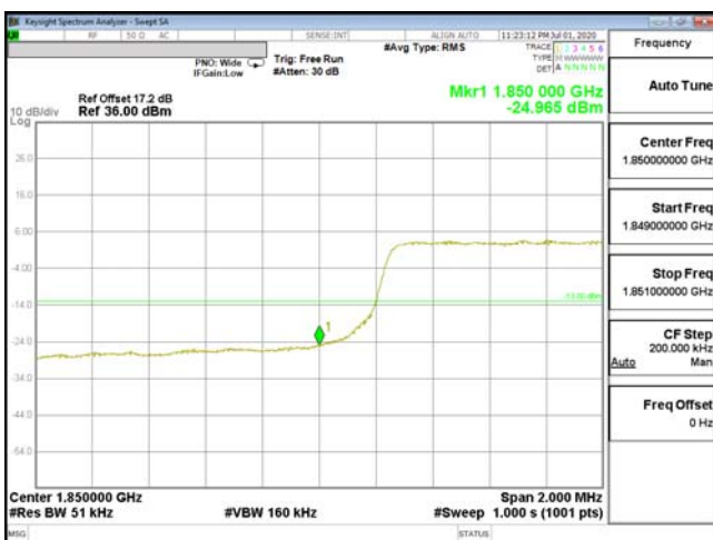
EDGE-ENDC_2A_n5-QPSK_5M(25,0)_CH18625_1852.5
