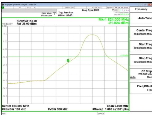
EDGE-ENDC_2A_n5-256QAM_10M(1,0)_CH165800_829
