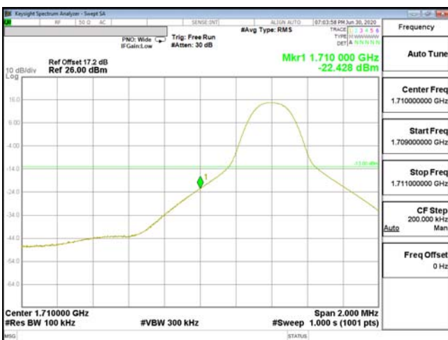
EDGE-ENDC_13A_n66-256QAM_10M(1,0)_CH343000_1715
