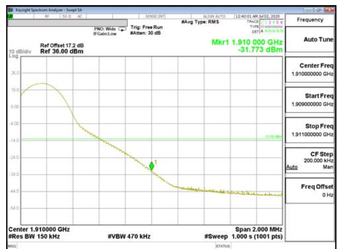
EDGE-ENDC_2A_n5-QPSK_15M(1,74)_CH19125_1902.5
