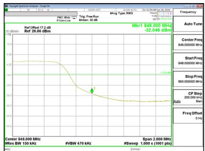
EDGE-ENDC_2A_n5-64QAM_15M(75,4)_CH168300_841.5
