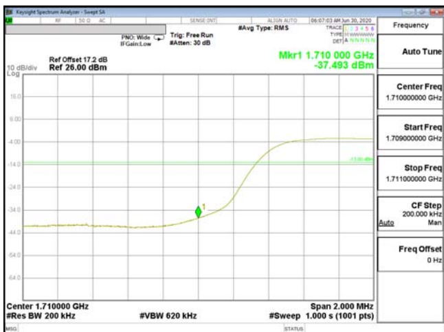
EDGE-ENDC_13A_n66-256QAM_20M(100,0)_CH344000_1720
