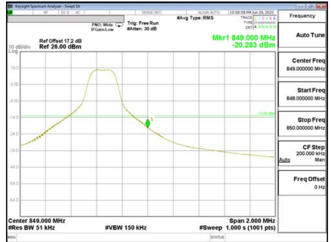
EDGE-ENDC_2A_n5-16QAM_5M(1,24)_CH169300_846.5
