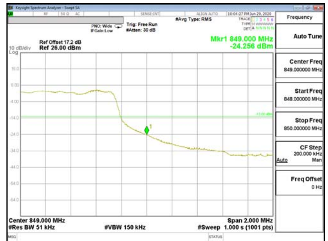
EDGE-ENDC_2A_n5-QPSK_5M(25,0)_CH169300_846.5
