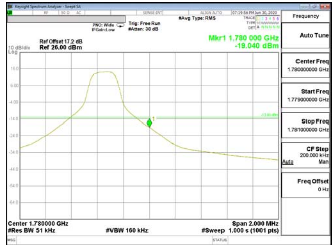
EDGE-ENDC_13A_n66-64QAM_5M(1,24)_CH355500_1777.5
