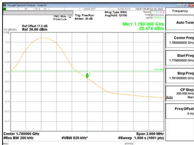
EDGE-ENDC_13A_n66-PI2-BPSK_20M(1,105)_CH354000_1770
