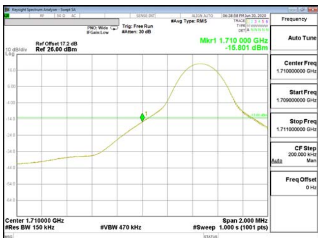
EDGE-ENDC_13A_n66-PI2-BPSK_15M(1,0)_CH343500_1717.5
