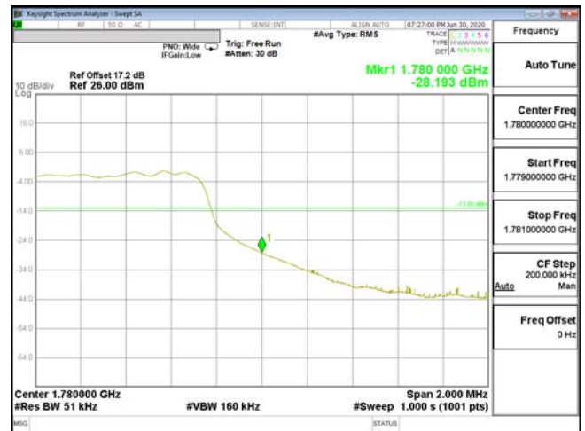
EDGE-ENDC_13A_n66-256QAM_5M(25,0)_CH355500_1777.5
