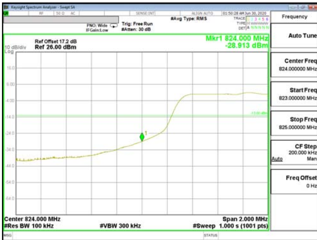
EDGE-ENDC_2A_n5-64QAM_10M(50,0)_CH165800_829
