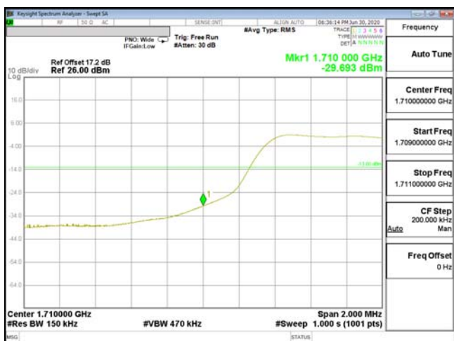
EDGE-ENDC_13A_n66-16QAM_15M(75,0)_CH343500_1717.5
