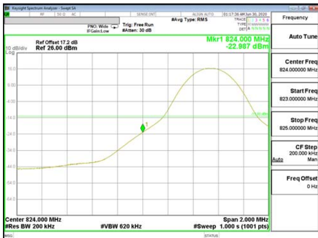
EDGE-ENDC_2A_n5-256QAM_20M(1,0)_CH166800_834
