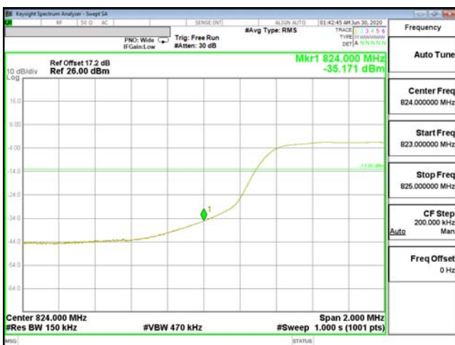
EDGE-ENDC_2A_n5-256QAM_15M(75,0)_CH166300_831.5
