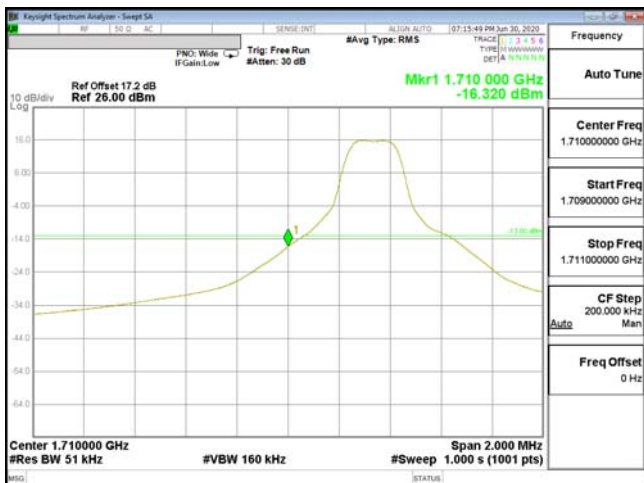
EDGE-ENDC_13A_n66-QPSK_5M(1,0)_CH342500_1712.5
