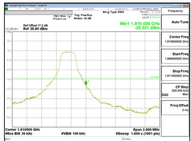
EDGE-ENDC_2A_n5-QPSK_3M(1,14)_CH19185_1908.5
