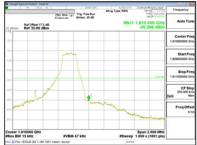
EDGE-ENDC_2A_n5-QPSK_1.4M(1,5)_CH19193_1909.3
