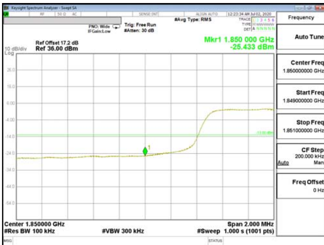
EDGE-ENDC_2A_n5-QPSK_10M(50,0)_CH18650_1855
