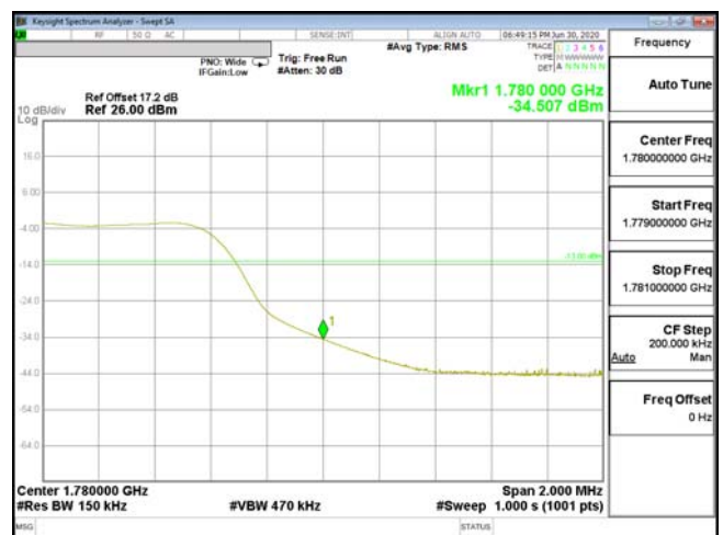
EDGE-ENDC_13A_n66-256QAM_15M(75,4)_CH354500_1772.5
