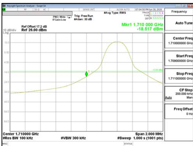
EDGE-ENDC_13A_n66-64QAM_10M(1,0)_CH343000_1715
