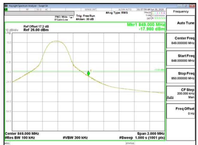
EDGE-ENDC_2A_n5-16QAM_10M(1,51)_CH168800_844
