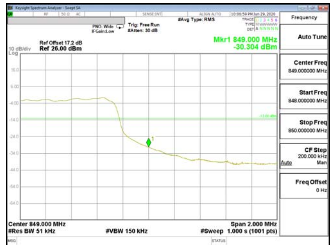
EDGE-ENDC_2A_n5-256QAM_5M(25,0)_CH169300_846.5
