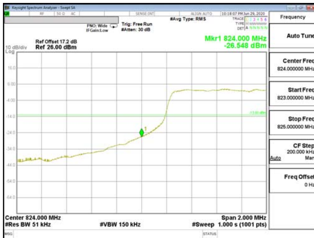
EDGE-ENDC_2A_n5-QPSK_5M(25,0)_CH165300_826.5
