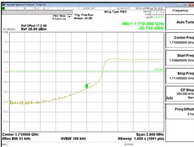
EDGE-ENDC_13A_n66-256QAM_5M(25,0)_CH342500_1712.5
