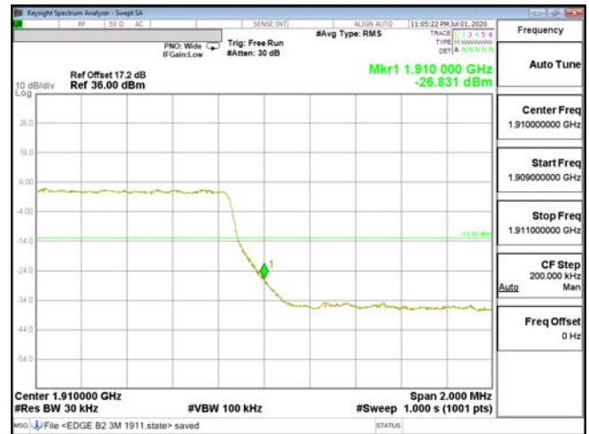
EDGE-ENDC_2A_n5-QPSK_3M(15,0)_CH19185_1908.5
