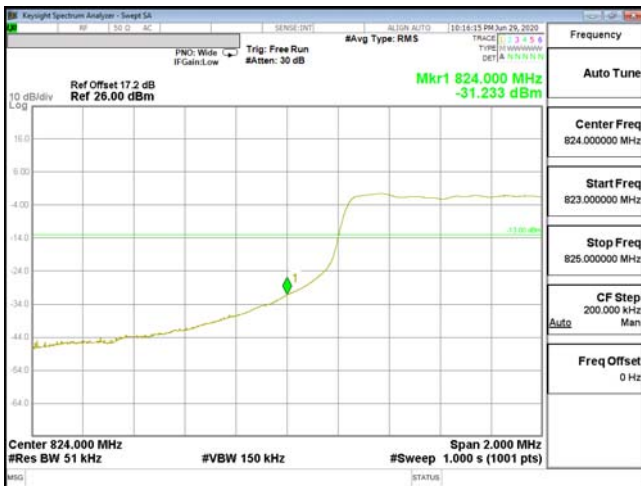
EDGE-ENDC_2A_n5-256QAM_5M(25,0)_CH165300_826.5
