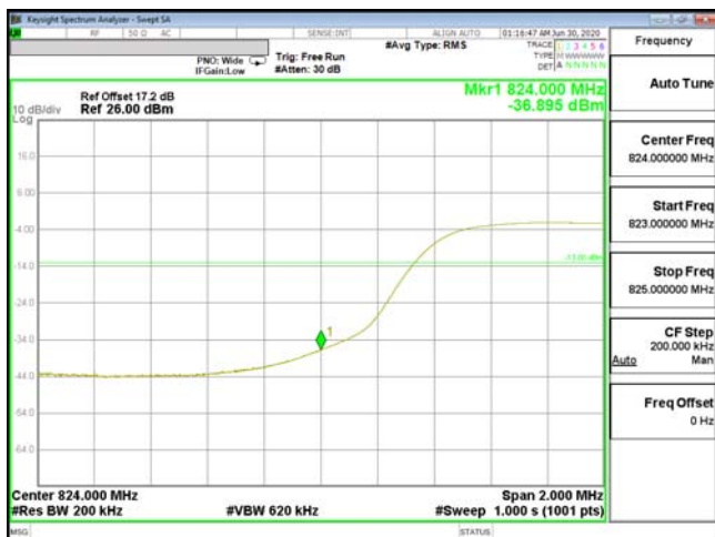
EDGE-ENDC_2A_n5-256QAM_20M(100,0)_CH166800_834
