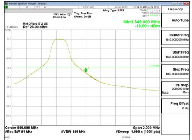
EDGE-ENDC_2A_n5-QPSK_5M(1,24)_CH169300_846.5
