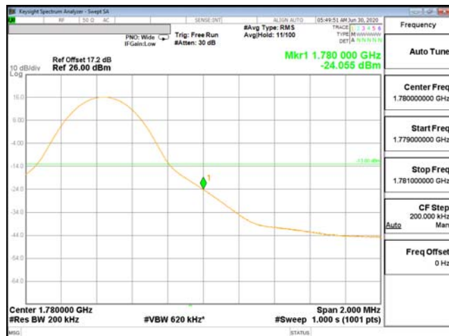
EDGE-ENDC_13A_n66-256QAM_20M(1,105)_CH354000_1770
