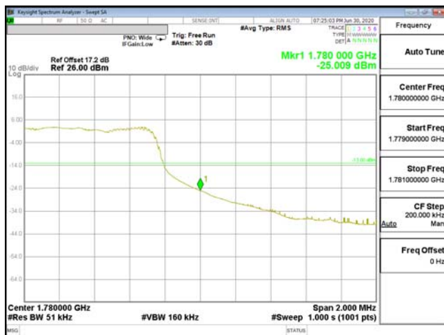
EDGE-ENDC_13A_n66-QPSK_5M(25,0)_CH355500_1777.5
