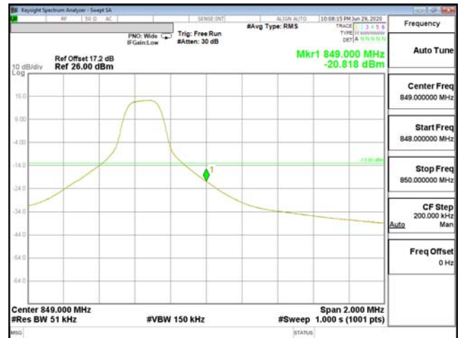
EDGE-ENDC_2A_n5-64QAM_5M(1,24)_CH169300_846.5
