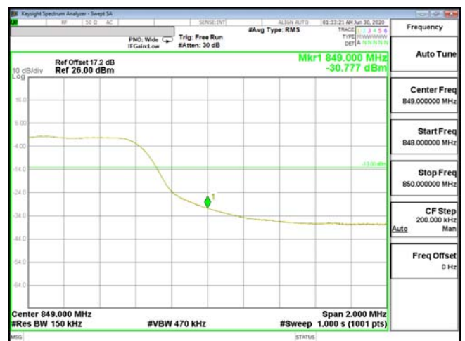
EDGE-ENDC_2A_n5-16QAM_15M(75,4)_CH168300_841.5
