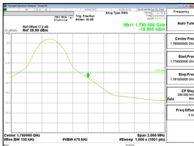
EDGE-ENDC_13A_n66-PI2-BPSK_15M(1,78)_CH354500_1772.5
