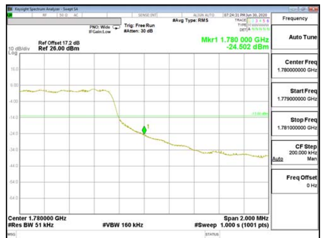
EDGE-ENDC_13A_n66-PI2-BPSK_5M(25,0)_CH355500_1777.5
