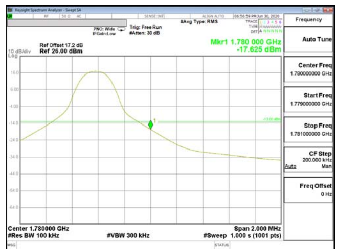
EDGE-ENDC_13A_n66-64QAM_10M(1,51)_CH355000_1775
