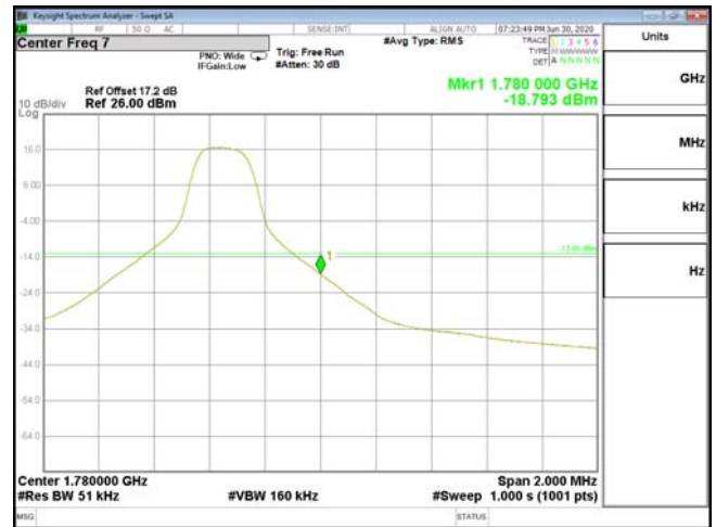
EDGE-ENDC_13A_n66-PI2-BPSK_5M(1,24)_CH355500_1777.5
