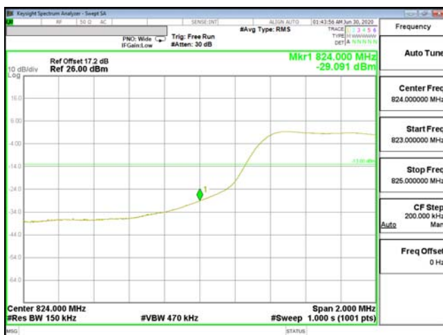
EDGE-ENDC_2A_n5-16QAM_15M(75,0)_CH166300_831.5
