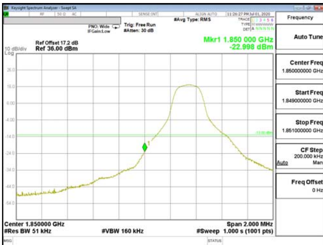
EDGE-ENDC_2A_n5-QPSK_5M(1,0)_CH18625_1852.5
