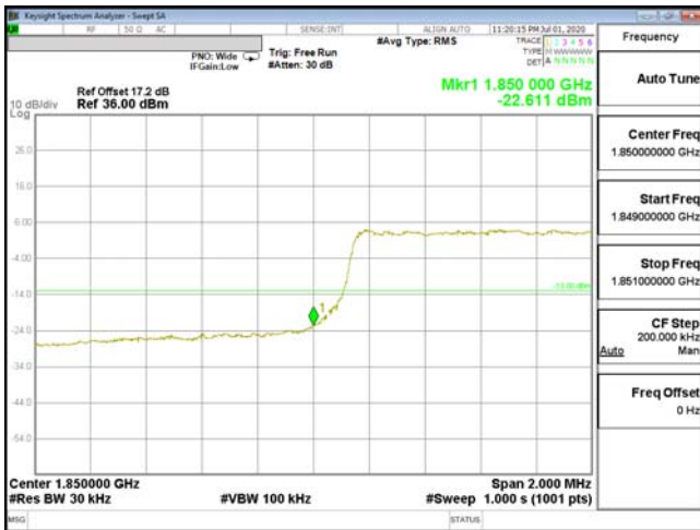
EDGE-ENDC_2A_n5-QPSK_3M(15,0)_CH18615_1851.5
