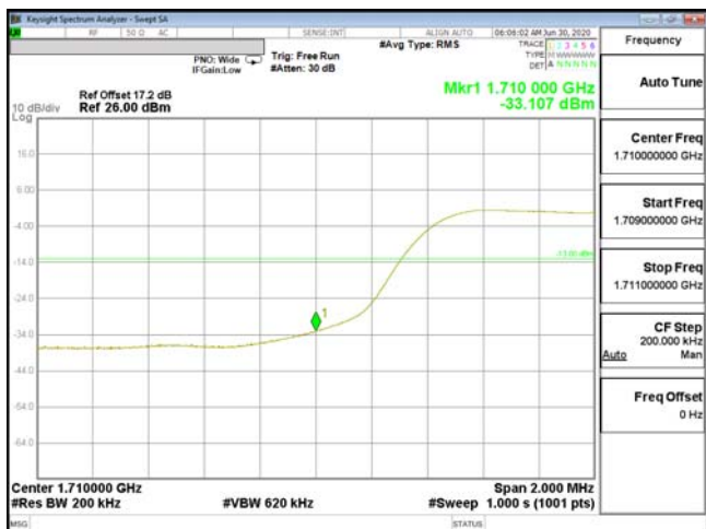
EDGE-ENDC_13A_n66-16QAM_20M(100,0)_CH344000_1720
