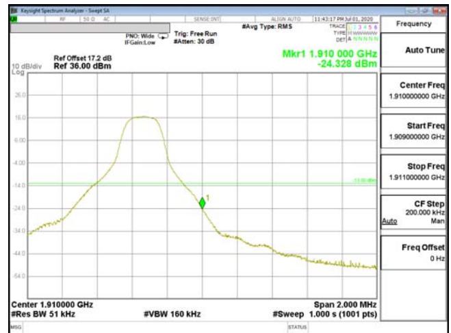
EDGE-ENDC_2A_n5-QPSK_5M(1,24)_CH19175_1907.5
