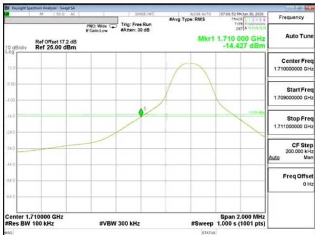
EDGE-ENDC_13A_n66-PI2-BPSK_10M(1,0)_CH343000_1715
