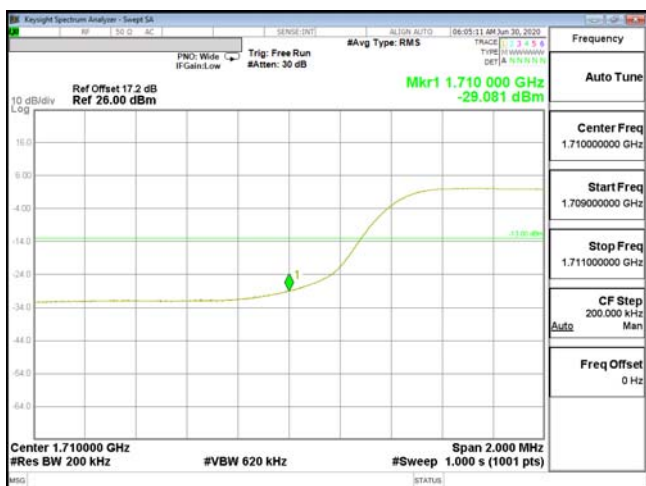
EDGE-ENDC_13A_n66-PI2-BPSK_20M(100,0)_CH344000_1720
