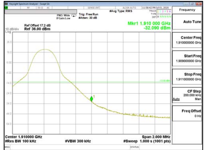
EDGE-ENDC_2A_n5-QPSK_10M(1,49)_CH19150_1905
