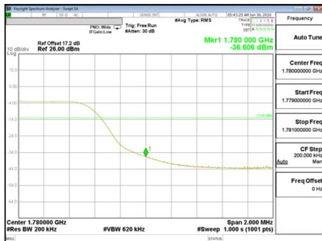
EDGE-ENDC_13A_n66-256QAM_20M(100,6)_CH354000_1770
