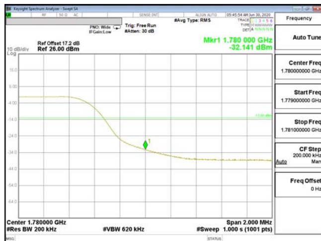
EDGE-ENDC_13A_n66-16QAM_20M(100,6)_CH354000_1770
