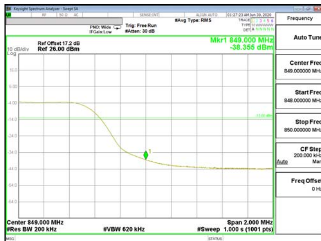
EDGE-ENDC_2A_n5-256QAM_20M(100,6)_CH167800_839
