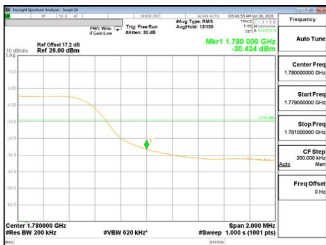
EDGE-ENDC_13A_n66-PI2-BPSK_20M(100,6)_CH354000_1770
