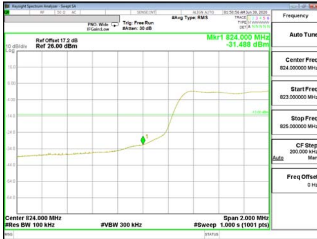
EDGE-ENDC_2A_n5-16QAM_10M(50,0)_CH165800_829
