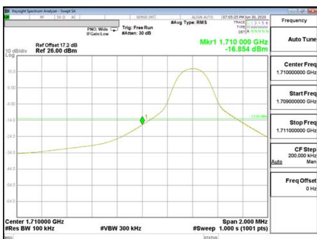
EDGE-ENDC_13A_n66-16QAM_10M(1,0)_CH343000_1715
