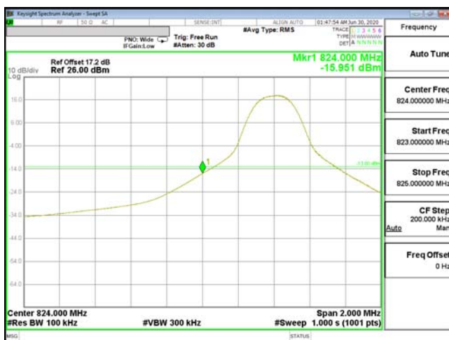
EDGE-ENDC_2A_n5-16QAM_10M(1,0)_CH165800_829
