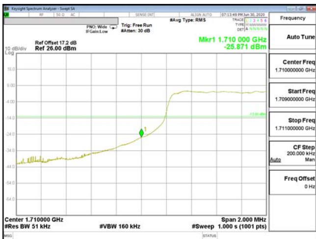
EDGE-ENDC_13A_n66-QPSK_5M(25,0)_CH342500_1712.5
