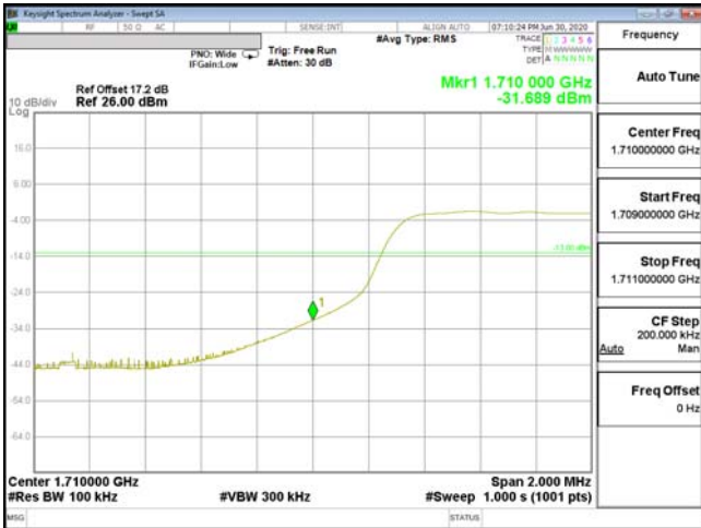
EDGE-ENDC_13A_n66-256QAM_10M(50,0)_CH343000_1715
