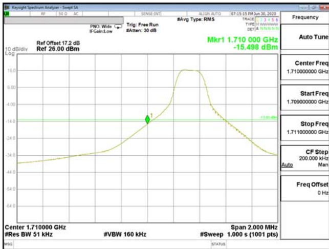
EDGE-ENDC_13A_n66-PI2-BPSK_5M(1,0)_CH342500_1712.5
