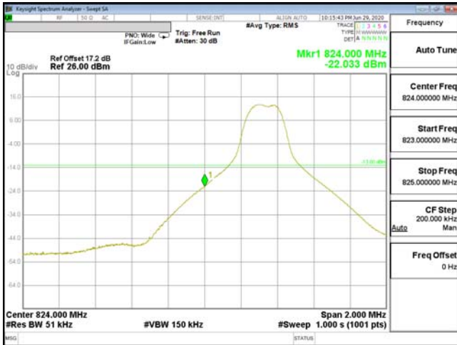
EDGE-ENDC_2A_n5-256QAM_5M(1,0)_CH165300_826.5
