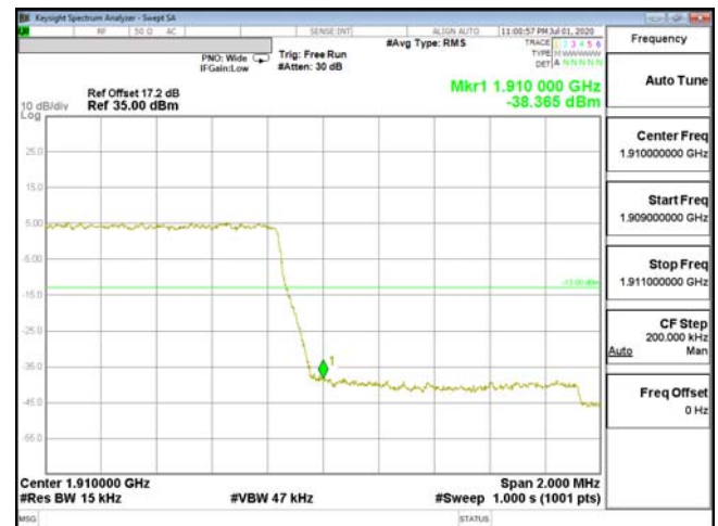
EDGE-ENDC_2A_n5-QPSK_1.4M(6,0)_CH19193_1909.3
