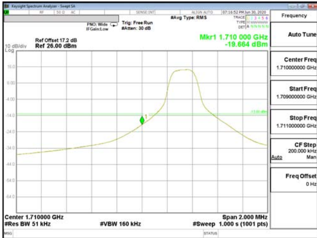
EDGE-ENDC_13A_n66-64QAM_5M(1,0)_CH342500_1712.5
