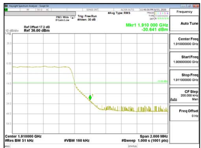
EDGE-ENDC_2A_n5-QPSK_5M(25,0)_CH19175_1907.5
