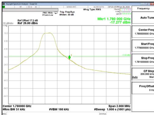
EDGE-ENDC_13A_n66-QPSK_5M(1,24)_CH355500_1777.5
