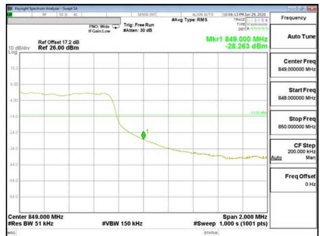
EDGE-ENDC_2A_n5-64QAM_5M(25,0)_CH169300_846.5
