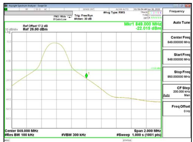
EDGE-ENDC_2A_n5-256QAM_10M(1,51)_CH168800_844
