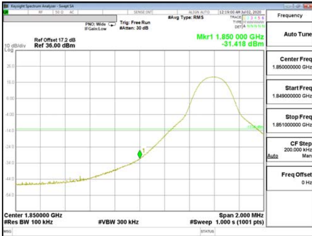
EDGE-ENDC_2A_n5-QPSK_10M(1,0)_CH18650_1855
