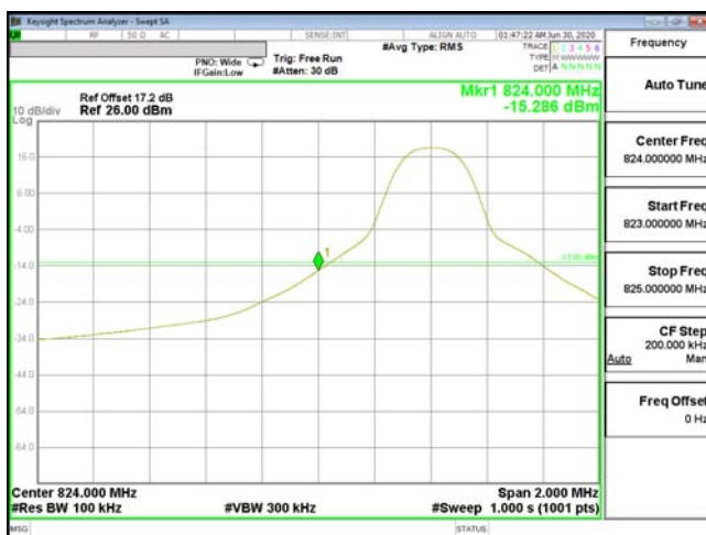
EDGE-ENDC_2A_n5-QPSK_10M(1,0)_CH165800_829
