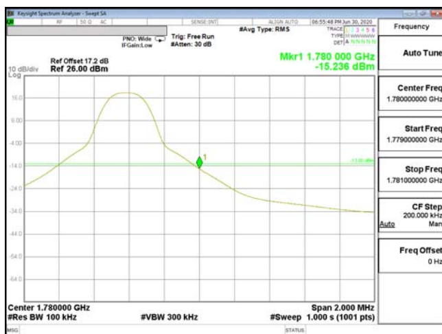
EDGE-ENDC_13A_n66-QPSK_10M(1,51)_CH355000_1775
