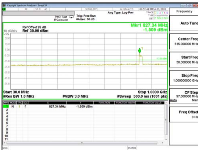
CSE-ENDC_66A_n5-QPSK_15M_CH132322_1745(1,74)
