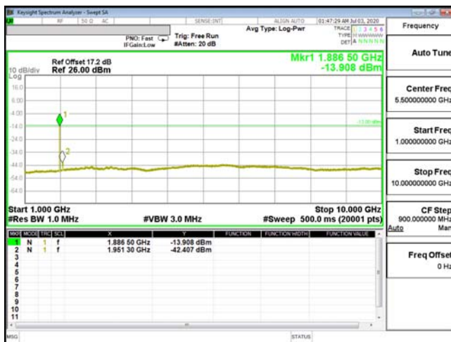
CSE-ENDC_5A_n2-64QAM_10M_CH20600_844(1,0)
