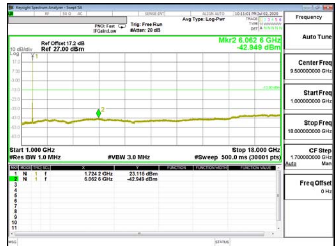
CSE-ENDC_66A_n5-QPSK_15M_CH132047_1717.5(1,74)
