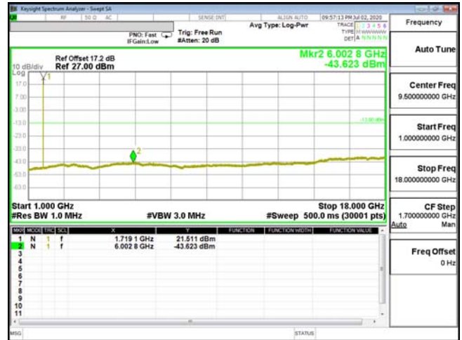
CSE-ENDC_66A_n5-QPSK_10M_CH132022_1715(1,49)
