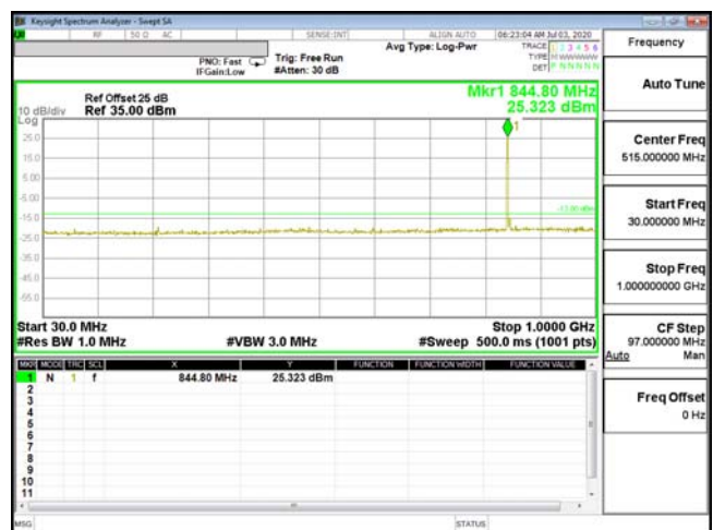
CSE-ENDC_5A_n2-16QAM_5M_CH20625_846.5(1,0)30M-1G
