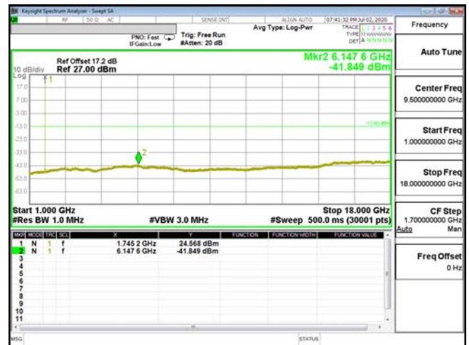
CSE-ENDC_66A_n5-16QAM_1.4M_CH132322_1745(1,3)
