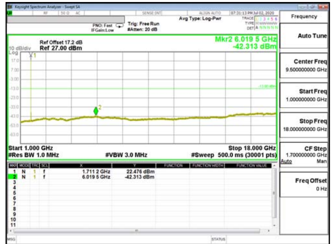
CSE-ENDC_66A_n5-QPSK_1.4M_CH131979_1710.7(1,5)-
