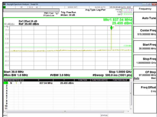
CSE-ENDC_5A_n2-16QAM_1.4M_CH20525_836.5(1,3)-30M-1G
