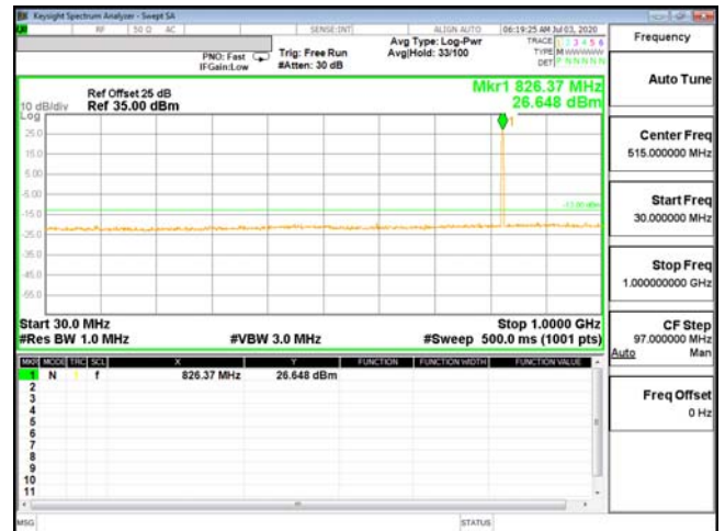
CSE-ENDC_5A_n2-64QAM_5M_CH20425_826.5(1,12)30M-1G
