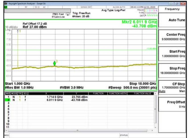
CSE-ENDC_66A_n5-16QAM_5M_CH131997_1712.5(1,24)
