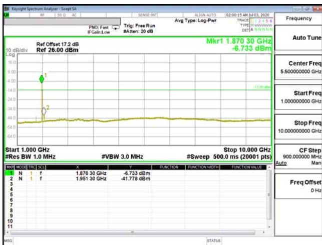
CSE-ENDC_5A_n2-16QAM_5M_CH20525_836.5(1,24)
