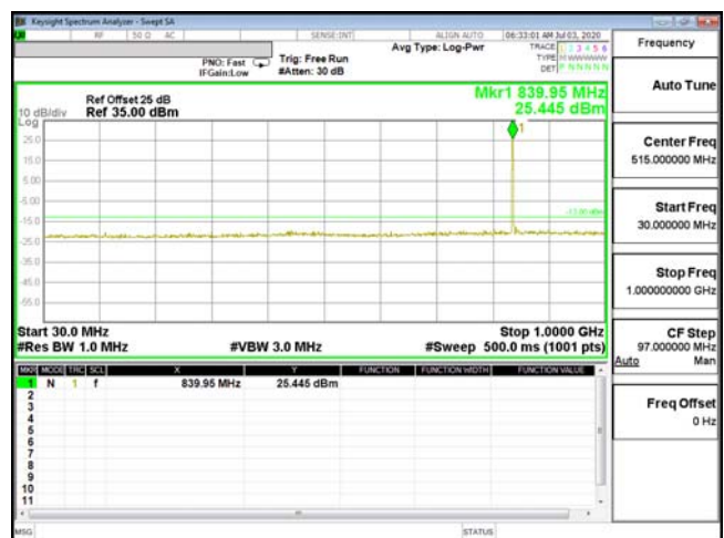
CSE-ENDC_5A_n2-16QAM_10M_CH20600_844(1,0)-30M-1G
