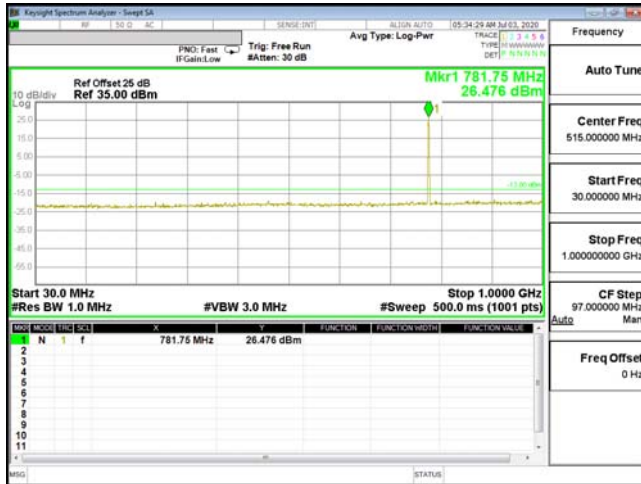
CSE-ENDC_13A_n66-64QAM_5M_CH23205_779.5(1,24)
