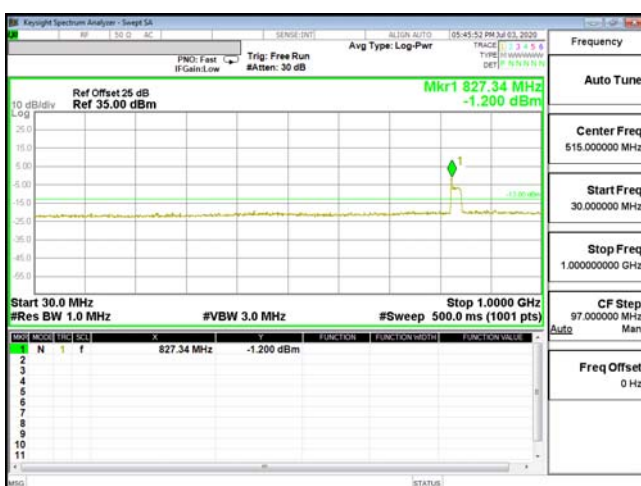
CSE-ENDC_66A_n5-QPSK_3M_CH132657_1778.5(1,7)
