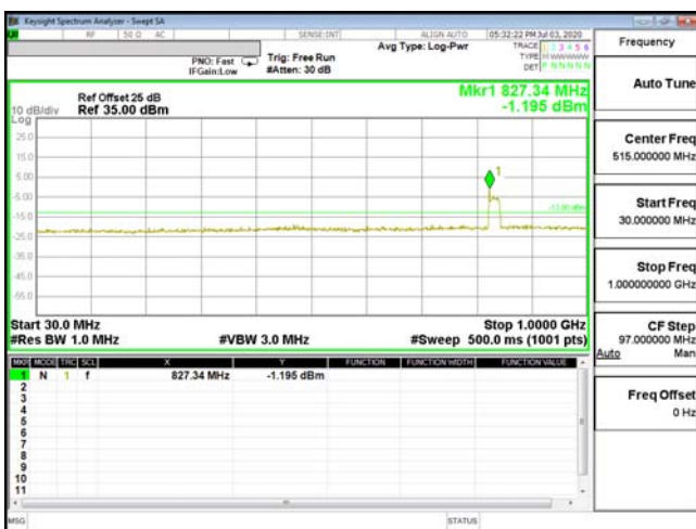
CSE-ENDC_66A_n5-16QAM_1.4M_CH132665_1779.3.7(1,3)
