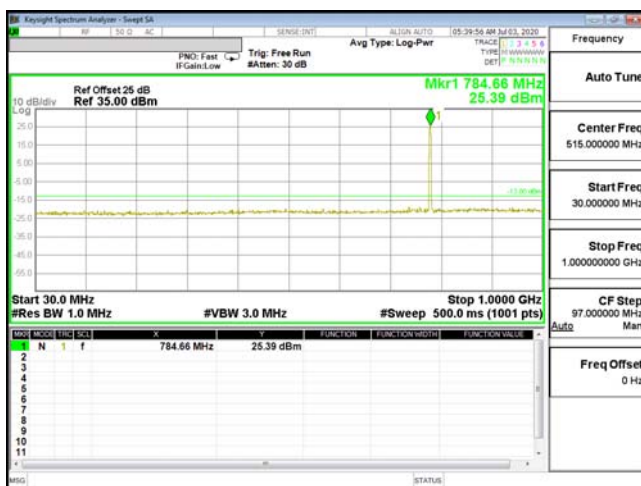
CSE-ENDC_13A_n66-64QAM_5M_CH23255_784.5(1,12)
