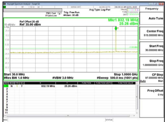
CSE-ENDC_5A_n2-16QAM_10M_CH20525_836.5(1,0)30M-1G
