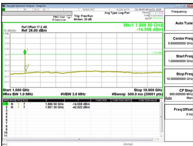
CSE-ENDC_5A_n2-16QAM_10M_CH20600_844(1,0)
