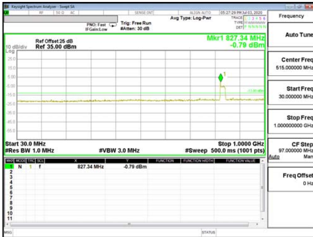
CSE-ENDC_66A_n5-QPSK_1.4M_CH131979_1710.7(1,5)
