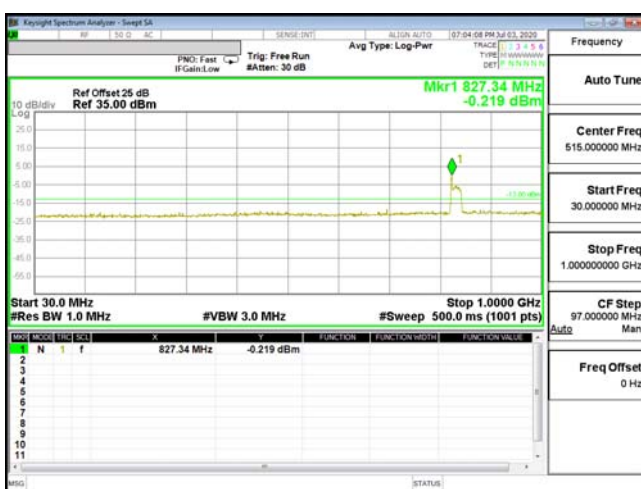
CSE-ENDC_66A_n5-QPSK_20M_CH132572_1770(1,0)
