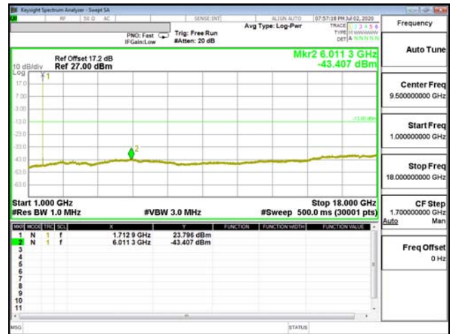
CSE-ENDC_66A_n5-16QAM_3M_CH131987_1711.5(1,14)
