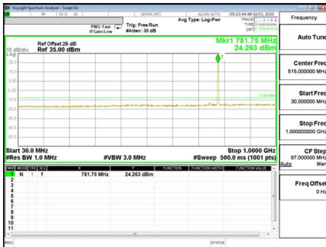
CSE-ENDC_13A_n66-16QAM_10M_CH23230_782(1,25)
