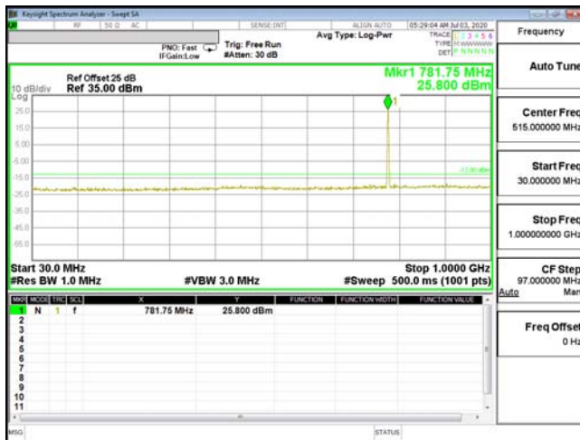
CSE-ENDC_13A_n66-16QAM_5M_CH23230_782(1,12)
