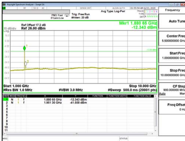
CSE-ENDC_5A_n2-64QAM_10M_CH20525_836.5(1,49)
