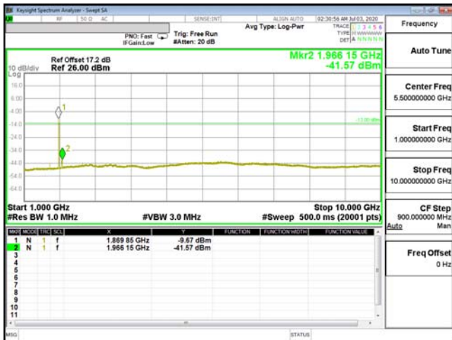
CSE-ENDC_5A_n2-16QAM_3M_CH20415_825.5(1,7)
