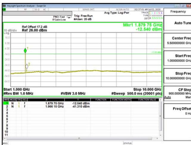
CSE-ENDC_5A_n2-64QAM_3M_CH20625_846.5(1,0)
