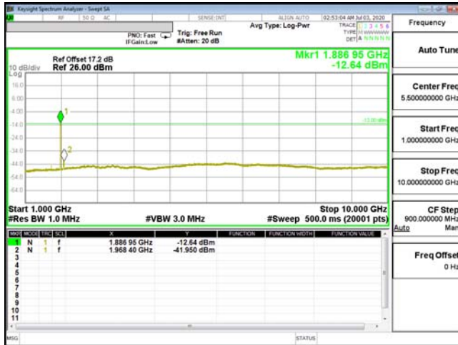
CSE-ENDC_5A_n2-64QAM_1.4M_CH20407_824.7(1,0)
