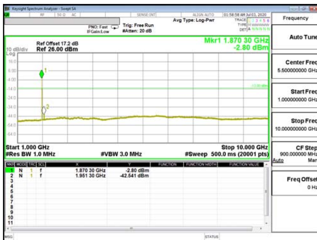
CSE-ENDC_5A_n2-64QAM_5M_CH20525_836.5(1,24)
