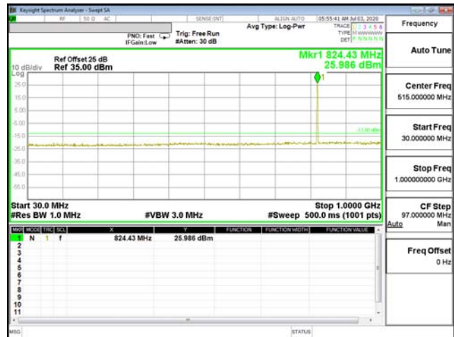
CSE-ENDC_5A_n2-16QAM_1.4M_CH20407_824.7(1,0)-30M-1G
