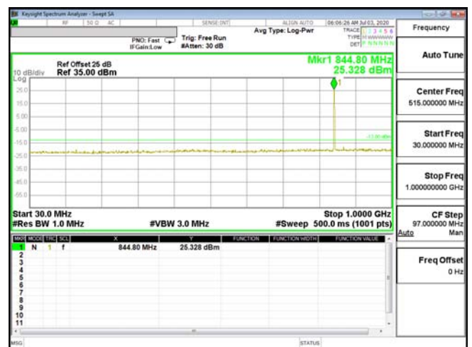
CSE-ENDC_5A_n2-64QAM_3M_CH20625_846.5(1,0)30M-1G
