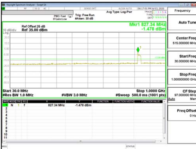
CSE-ENDC_66A_n5-QPSK_10M_CH132322_1745(1,49)
