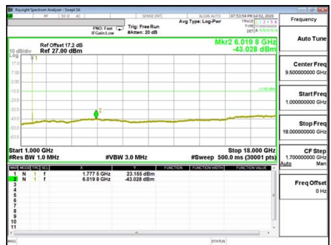
CSE-ENDC_66A_n5-16QAM_3M_CH132657_1778.5(1,0)
