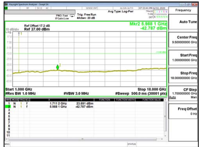
CSE-ENDC_66A_n5-16QAM_1.4M_CH131979_1710.7(1,5)
