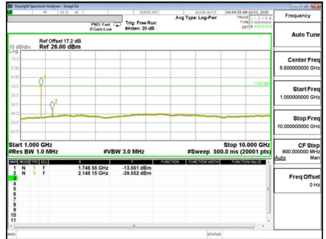
CSE-ENDC_13A_n66-64QAM_5M_CH23205_779.5(1,24)
