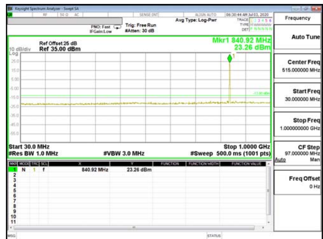
CSE-ENDC_5A_n2-QPSK_10M_CH20525_836.5(1,49)30M-1G
