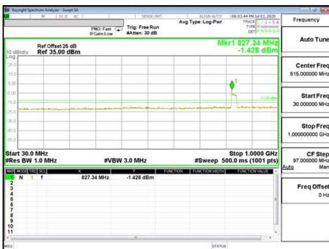
CSE-ENDC_66A_n5-QPSK_5M_CH132647_1777.5(1,0)
