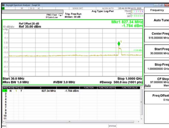
CSE-ENDC_66A_n5-16QAM_3M_CH132657_1778.5(1,0)
