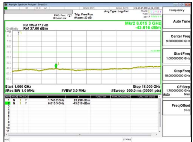
CSE-ENDC_66A_n5-16QAM_5M_CH132322_1745(1,24)
