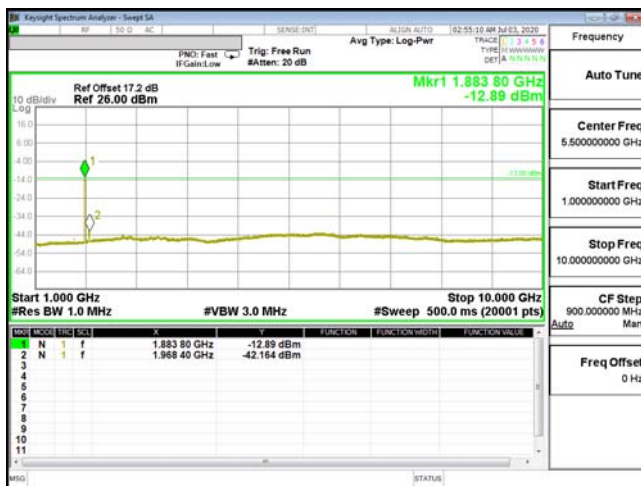
CSE-ENDC_5A_n2-64QAM_1.4M_CH20643_848.3((1,5))
