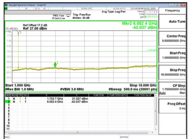
CSE-ENDC_66A_n5-QPSK_20M_CH132322_1745(1,99)
