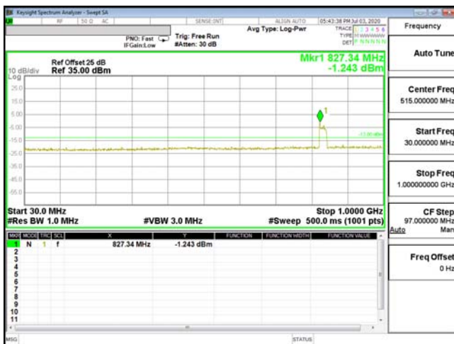
CSE-ENDC_66A_n5-QPSK_3M_CH132322_1745(1,14)
