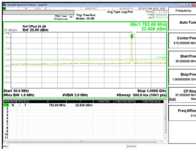
CSE-ENDC_13A_n66-QPSK_5M_CH23230_782(25,0)
