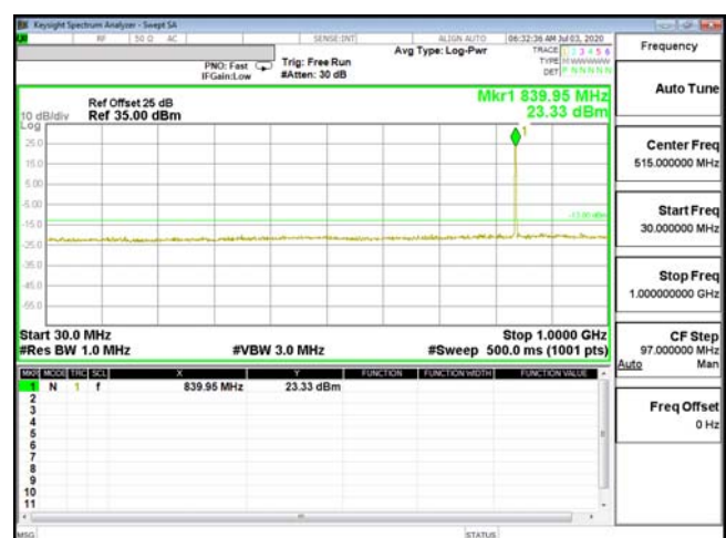
CSE-ENDC_5A_n2-QPSK_10M_CH20600_844(1,0)-30M-1G
