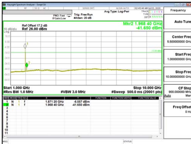
CSE-ENDC_5A_n2-64QAM_1.4M_CH20525_836.5(1,3)
