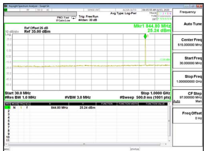
CSE-ENDC_5A_n2-16QAM_3M_CH20625_846.5(1,0)30M-1G
