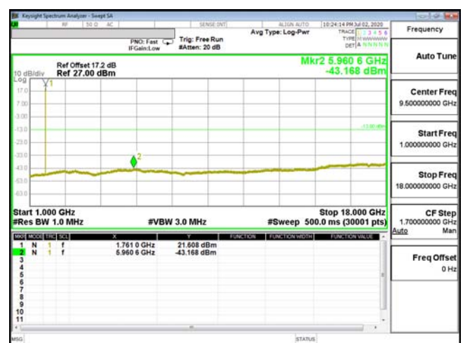
CSE-ENDC_66A_n5-QPSK_20M_CH132572_1770(1,0)
