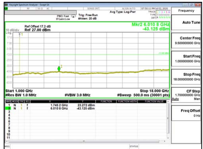
CSE-ENDC_66A_n5-16QAM_3M_CH132322_1745(1,7)-
