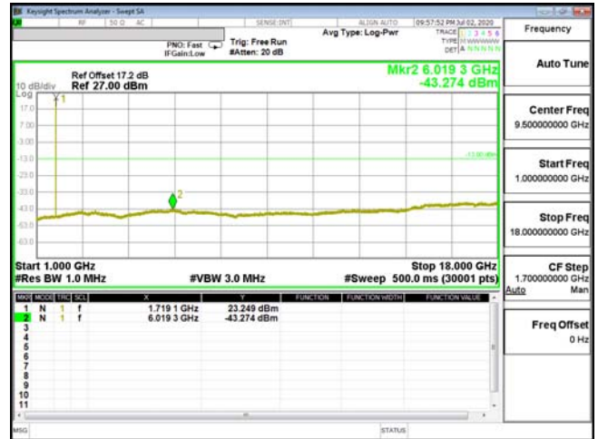
CSE-ENDC_66A_n5-16QAM_10M_CH132022_1715(1,49)
