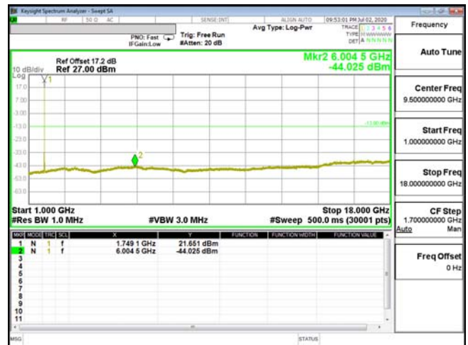
CSE-ENDC_66A_n5-QPSK_10M_CH132322_1745(1,49)
