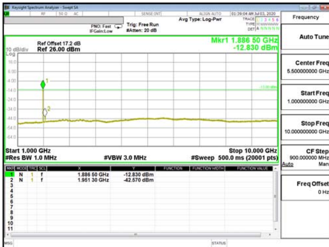
CSE-ENDC_5A_n2-QPSK_10M_CH20450_829(1,0)
