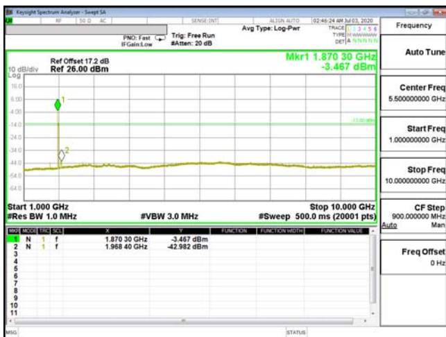
CSE-ENDC_5A_n2-16QAM_1.4M_CH20525_836.5(1,3)
