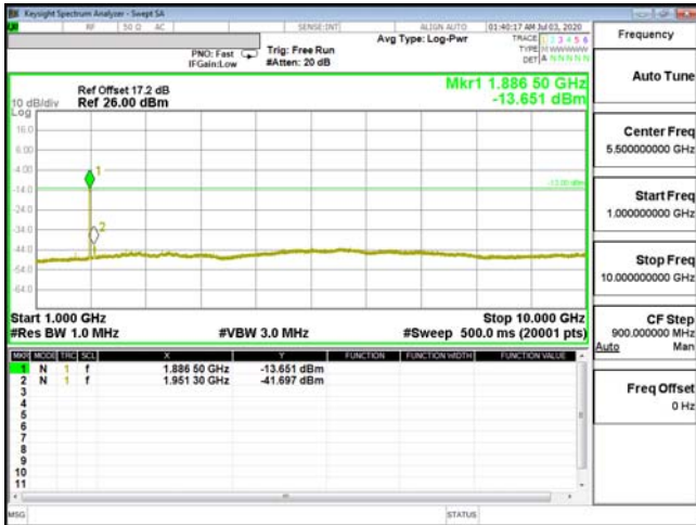
CSE-ENDC_5A_n2-16QAM_10M_CH20450_829(1,0)
