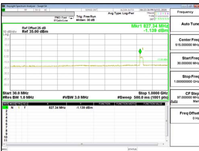
CSE-ENDC_66A_n5-QPSK_10M_CH132622_1775(1,25)
