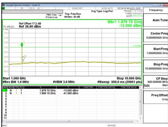
CSE-ENDC_5A_n2-16QAM_3M_CH20625_846.5(1,0)
