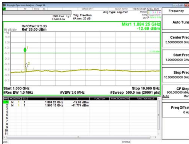
CSE-ENDC_5A_n2-64QAM_3M_CH20525_836.5(1,14)
