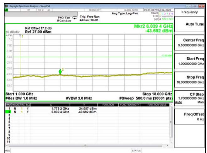
CSE-ENDC_66A_n5-16QAM_5M_CH132647_1777.5(1,0)
