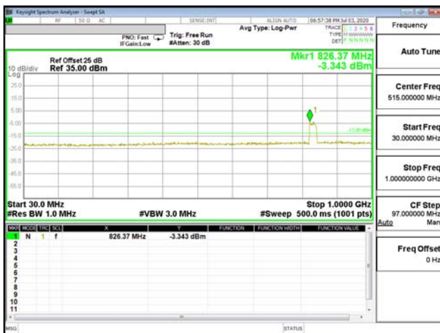
CSE-ENDC_66A_n5-QPSK_20M_CH132322_1745(1,99)
