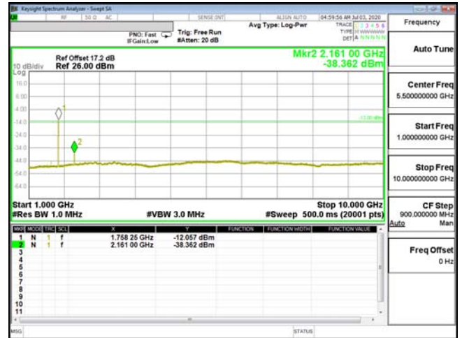
CSE-ENDC_13A_n66-QPSK_10M_CH23230_782(1,49)
