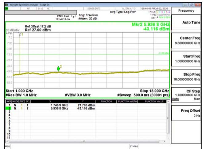
CSE-ENDC_66A_n5-QPSK_5M_CH132322_1745(1,24)
