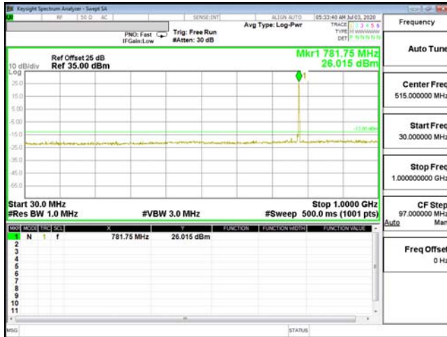
CSE-ENDC_13A_n66-16QAM_5M_CH23205_779.5(1,24)
