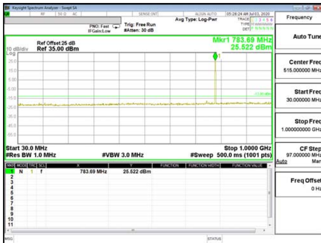
CSE-ENDC_13A_n66-64QAM_5M_CH23230_782(1,24)
