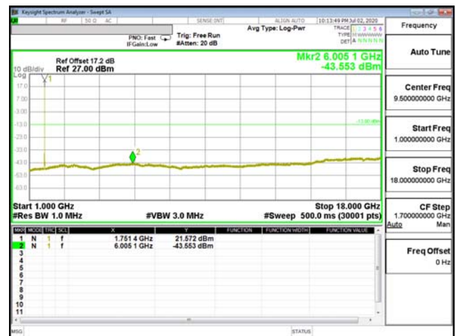
CSE-ENDC_66A_n5-QPSK_15M_CH132322_1745(1,74)
