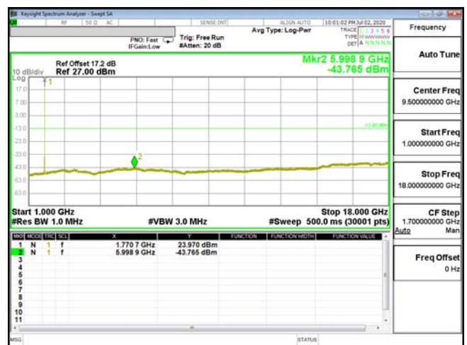
CSE-ENDC_66A_n5-16QAM_10M_CH132622_1775(1,0)
