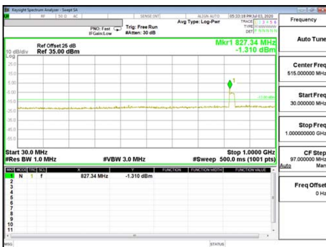
CSE-ENDC_66A_n5-QPSK_1.4M_CH132665_1779.3.7(1,0)
