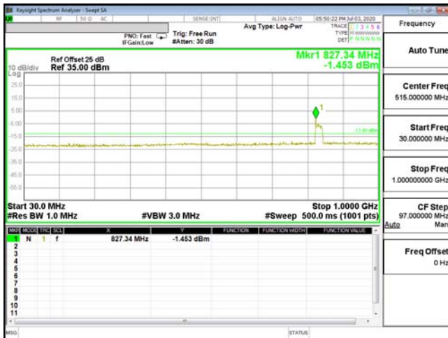
CSE-ENDC_66A_n5-QPSK_3M_CH131987_1711.5(1,14)
