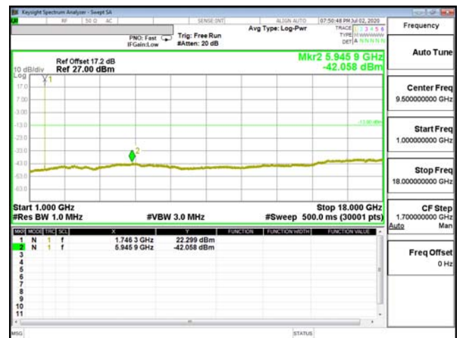
CSE-ENDC_66A_n5-QPSK_3M_CH132322_1745(1,14)
