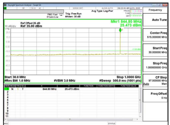
CSE-ENDC_5A_n2-64QAM_5M_CH20625_846.5(1,0)30M-1G
