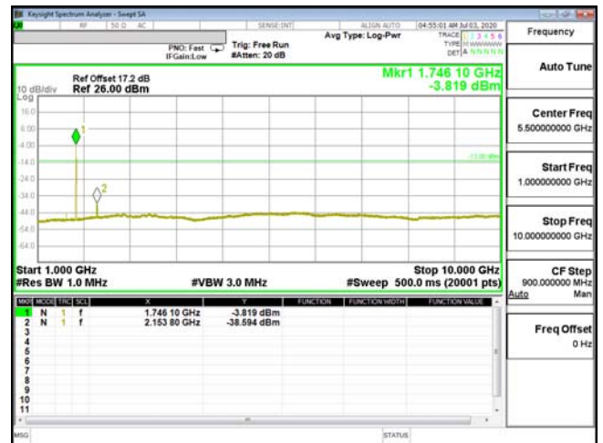
CSE-ENDC_13A_n66-16QAM_5M_CH23230_782(1,12)
