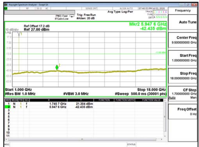
CSE-ENDC_66A_n5-QPSK_1.4M_CH132322_1745(1,5)-
