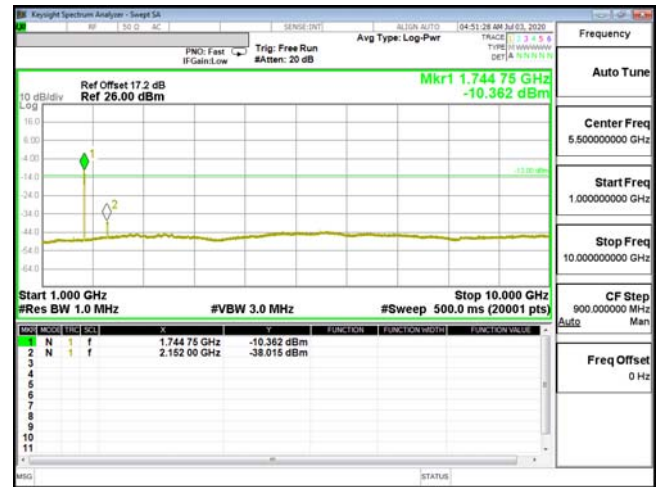
CSE-ENDC_13A_n66-QPSK_5M_CH23205_779.5(1,24)
