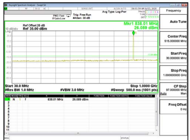
CSE-ENDC_5A_n2-64QAM_3M_CH20525_836.5(1,14)30M-1G
