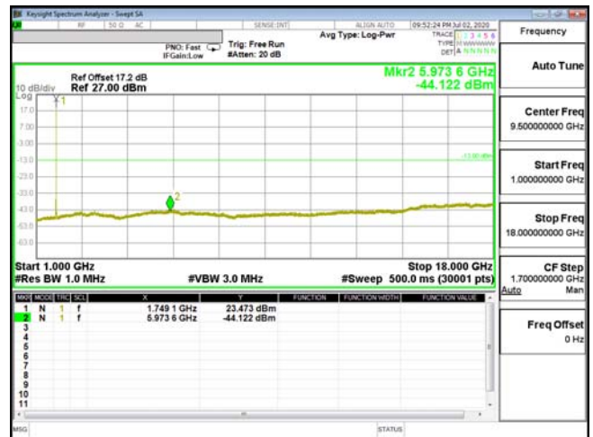
CSE-ENDC_66A_n5-16QAM_10M_CH132322_1745(1,49)
