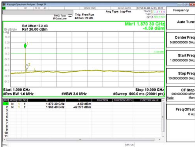
CSE-ENDC_5A_n2-16QAM_1.4M_CH20407_824.7(1,0)
