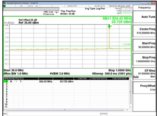
CSE-ENDC_5A_n2-16QAM_10M_CH20450_829(1,0)30M-1G
