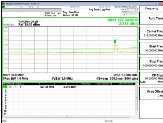
CSE-ENDC_66A_n5-QPSK_15M_CH132047_1717.5(1,74)
