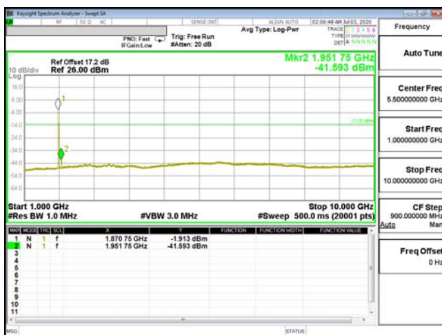
CSE-ENDC_5A_n2-64QAM_5M_CH20625_846.5(1,0)
