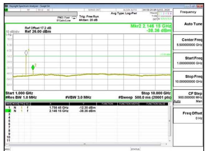
CSE-ENDC_13A_n66-64QAM_10M_CH23230_782(1,25)
