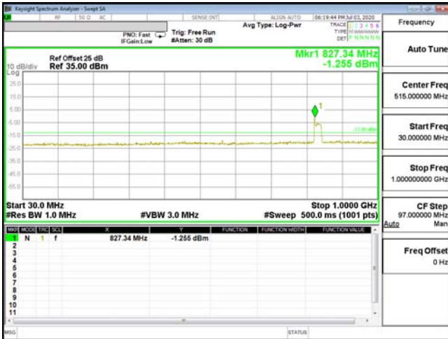
CSE-ENDC_66A_n5-16QAM_10M_CH132022_1715(1,49)
