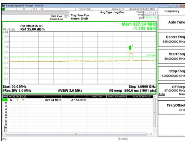
CSE-ENDC_66A_n5-16QAM_5M_CH132647_1777.5(1,0)
