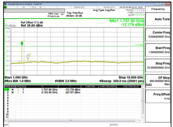
CSE-ENDC_13A_n66-64QAM_5M_CH23230_782(1,24)
