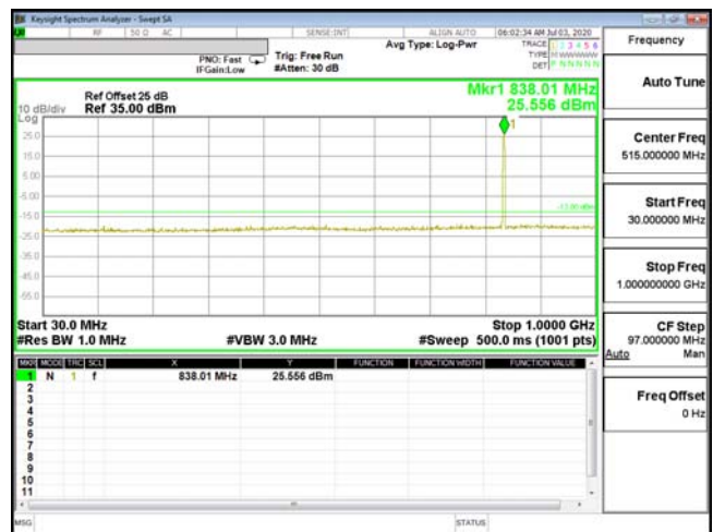
CSE-ENDC_5A_n2-16QAM_3M_CH20525_836.5(1,14)30M-1G
