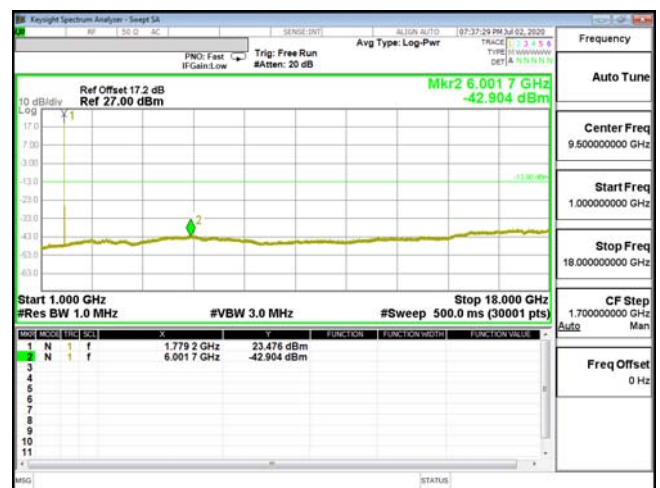
CSE-ENDC_66A_n5-16QAM_1.4M_CH132665_1779.3.7(1,3)
