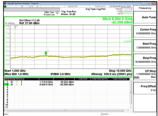
CSE-ENDC_66A_n5-QPSK_3M_CH131987_1711.5(1,14)
