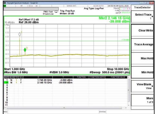
CSE-ENDC_13A_n66-16QAM_5M_CH23205_779.5(1,24)
