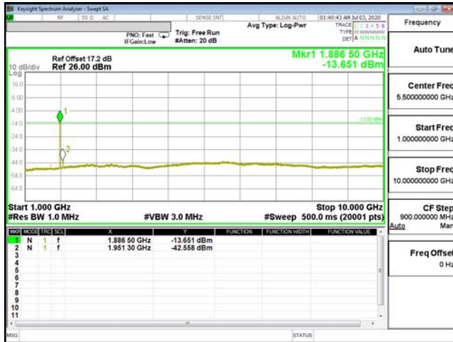
CSE-ENDC_5A_n2-64QAM_10M_CH20450_829(1,0)
