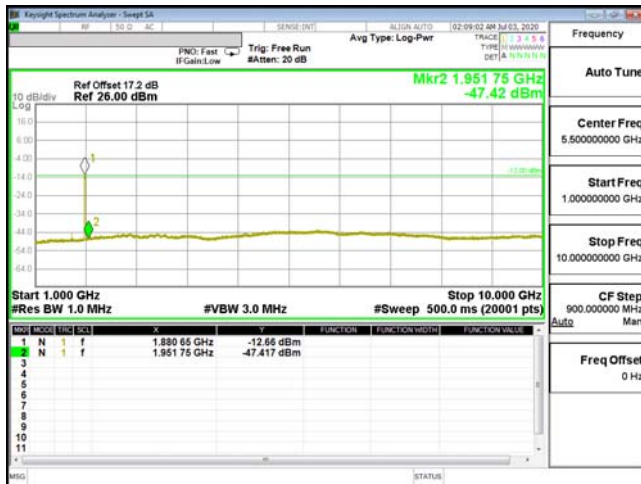
CSE-ENDC_5A_n2-64QAM_5M_CH20425_826.5(1,12)
