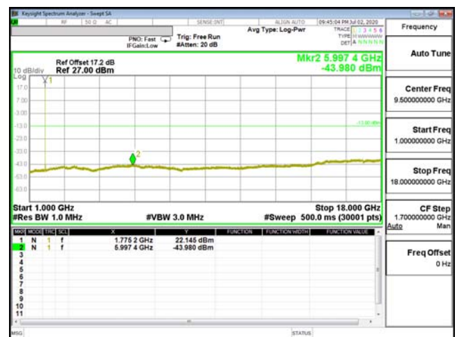
CSE-ENDC_66A_n5-QPSK_5M_CH132647_1777.5(1,0)
