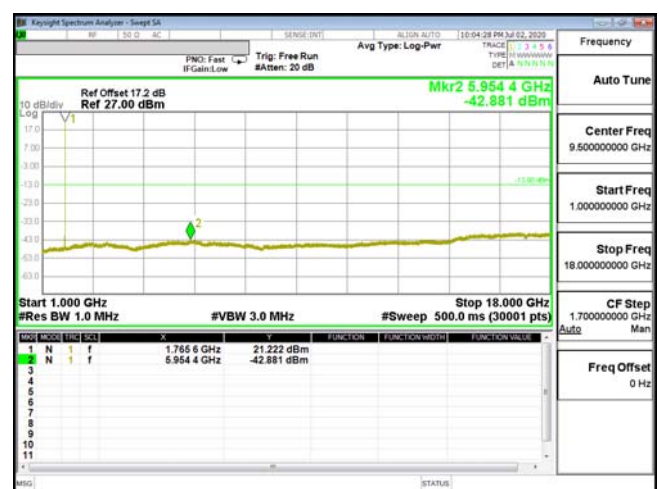
CSE-ENDC_66A_n5-QPSK_15M_CH132597_1772.5(1,0)
