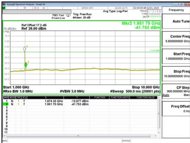
CSE-ENDC_5A_n2-16QAM_5M_CH20425_826.5(1,12)
