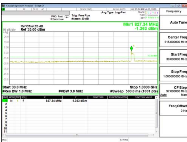
CSE-ENDC_66A_n5-16QAM_10M_CH132622_1775(1,0)
