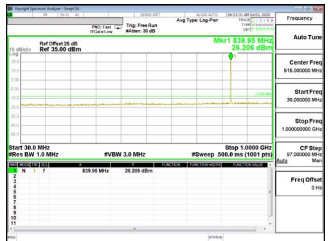
CSE-ENDC_5A_n2-64QAM_10M_CH20600_844(1,0)30M-1G
