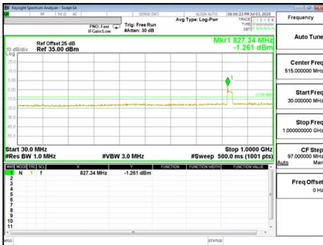
CSE-ENDC_66A_n5-QPSK_5M_CH132322_1745(1,24)
