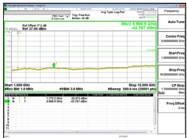
CSE-ENDC_66A_n5-QPSK_10M_CH132622_1775(1,25)
