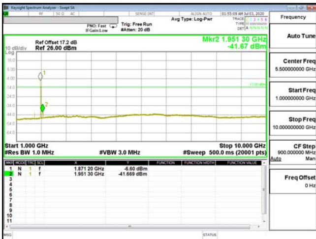
CSE-ENDC_5A_n2-16QAM_10M_CH20525_836.5(1,0)
