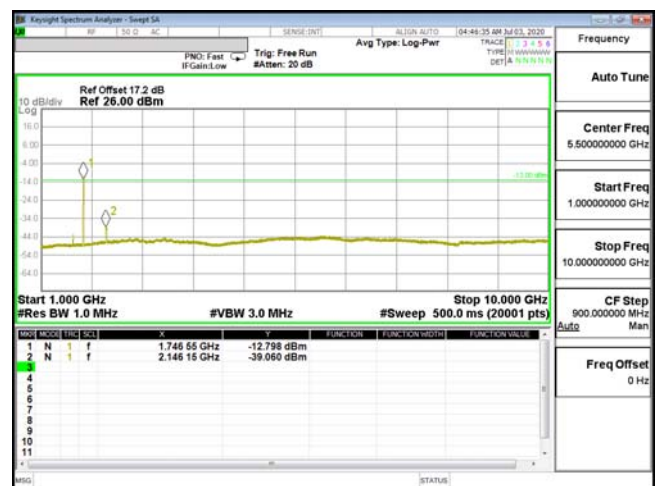
CSE-ENDC_13A_n66-64QAM_5M_CH23255_784.5(1,12)
