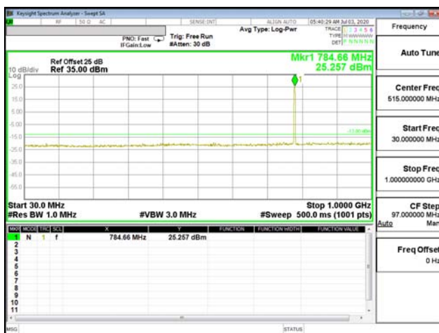
CSE-ENDC_13A_n66-16QAM_5M_CH23255_784.5(1,12)
