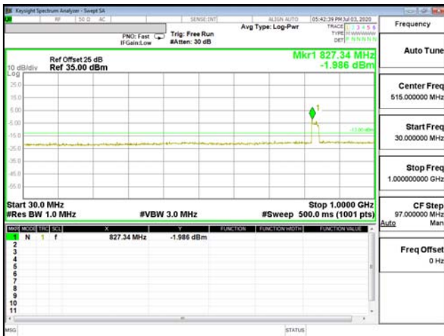
CSE-ENDC_66A_n5-16QAM_3M_CH132322_1745(1,7)
