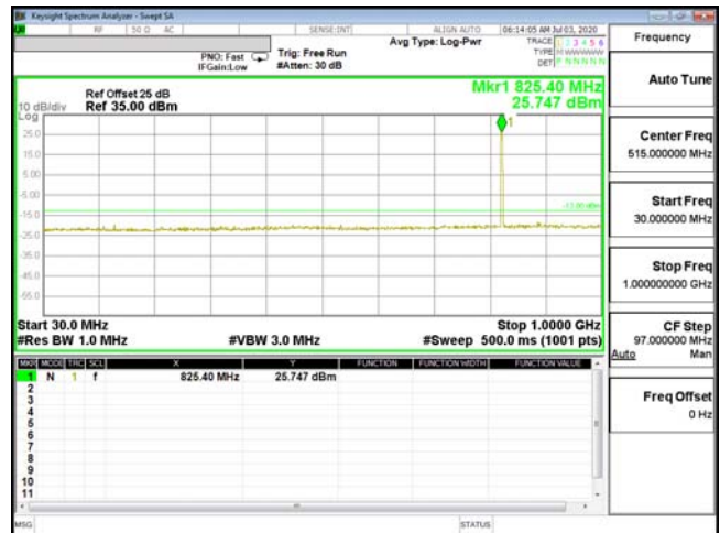
CSE-ENDC_5A_n2-16QAM_3M_CH20415_825.5(1,7)-30M-1G
