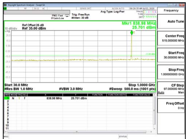
CSE-ENDC_5A_n2-16QAM_5M_CH20525_836.5(1,24)30M-1G
