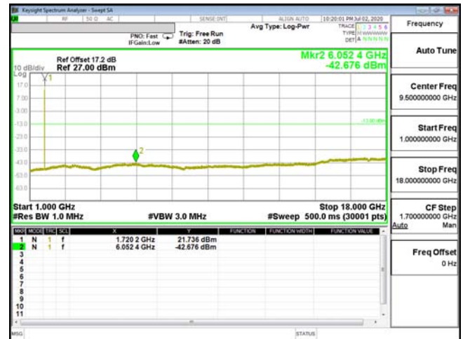
CSE-ENDC_66A_n5-QPSK_20M_CH132072_1720(1,50)
