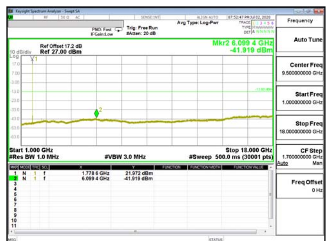
CSE-ENDC_66A_n5-QPSK_3M_CH132657_1778.5(1,7)-
