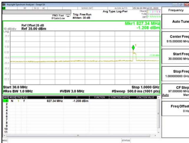
CSE-ENDC_66A_n5-QPSK_1.4M_CH132322_1745(1,5)
