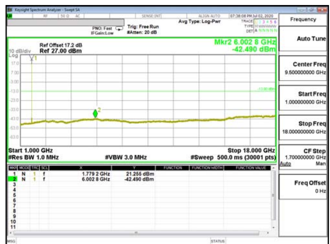
CSE-ENDC_66A_n5-QPSK_1.4M_CH132665_1779.3.7(1,0)-
