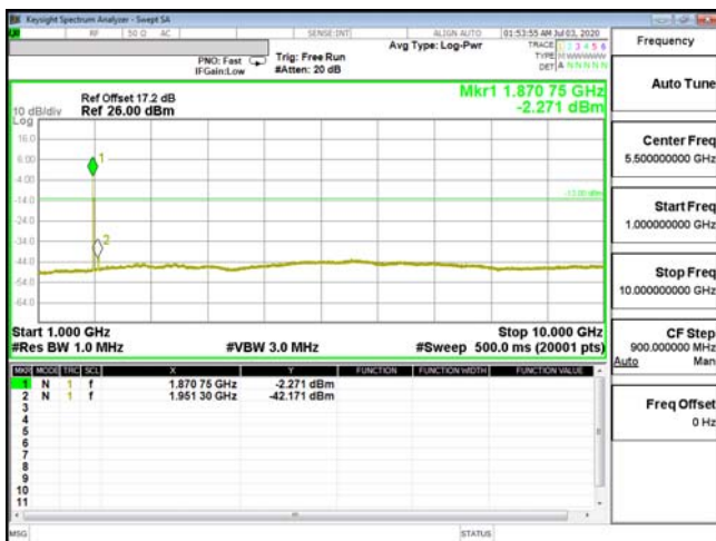
CSE-ENDC_5A_n2-QPSK_10M_CH20525_836.5(1,49)
