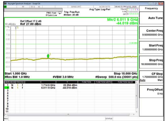
CSE-ENDC_66A_n5-QPSK_5M_CH131997_1712.5(1,24)
