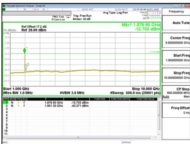
CSE-ENDC_5A_n2-16QAM_5M_CH20625_846.5(1,0)
