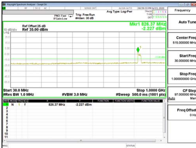
CSE-ENDC_66A_n5-QPSK_20M_CH132072_1720(1,50)
