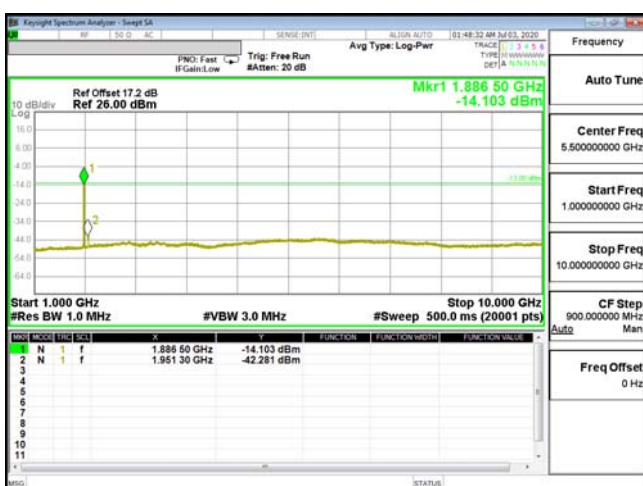
CSE-ENDC_5A_n2-QPSK_10M_CH20600_844(1,0)
