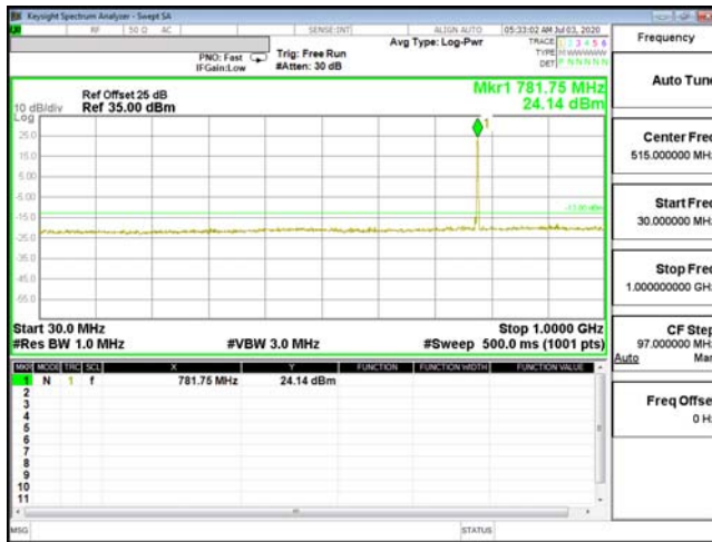
CSE-ENDC_13A_n66-QPSK_5M_CH23205_779.5(1,24)
