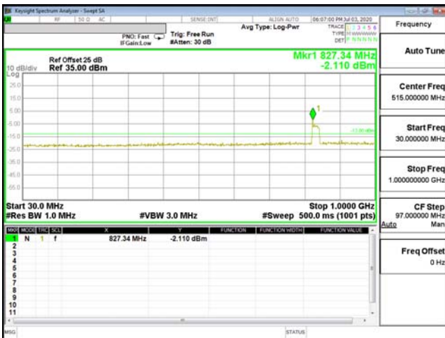
CSE-ENDC_66A_n5-16QAM_5M_CH132322_1745(1,24)
