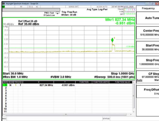
CSE-ENDC_2A_n5-16QAM_15M_CH18675_1857.5(1,0)
