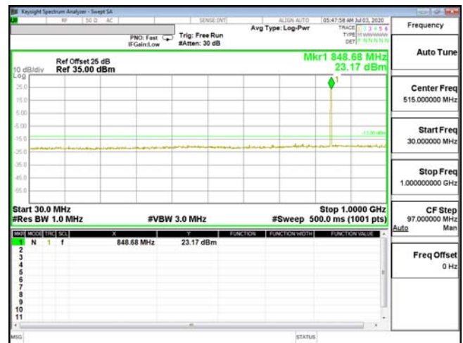
CSE-ENDC_5A_n2-QPSK_1.4M_CH20643_848.3((1,3)30M-1G
