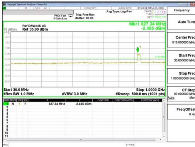
CSE-ENDC_2A_n5-64QAM_15M_CH18675_1857.5(1,37)
