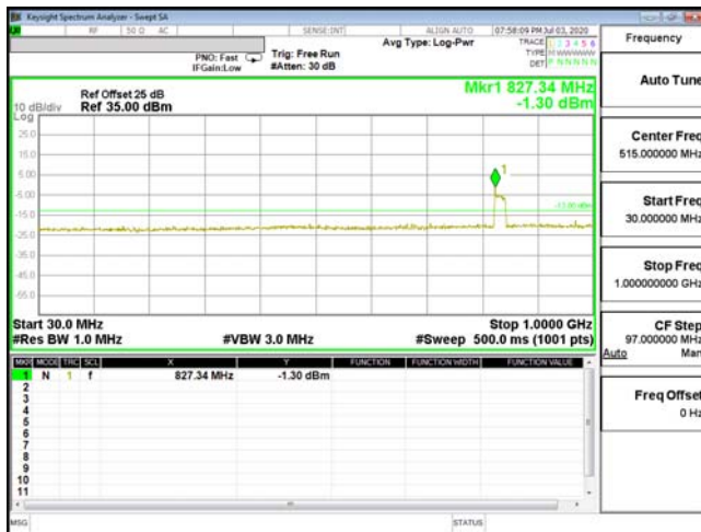
CSE-ENDC_2A_n5-16QAM_20M_CH18900_1880(1,0)
