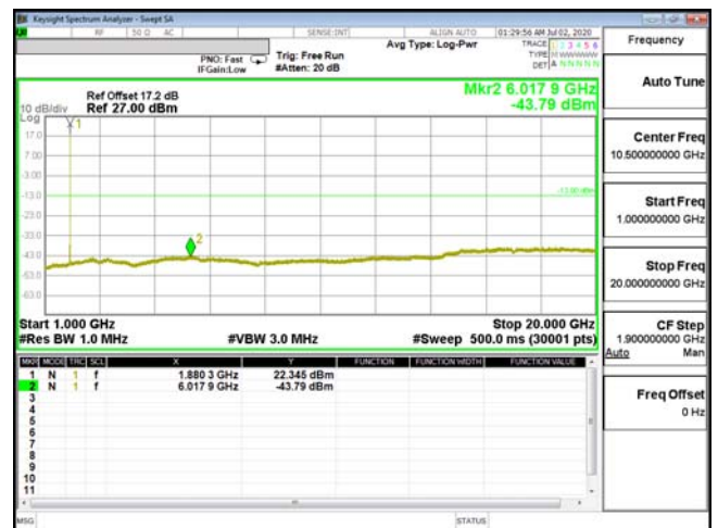
CSE-ENDC_2A_n5-64QAM_15M_CH18900_1880(1,37)
