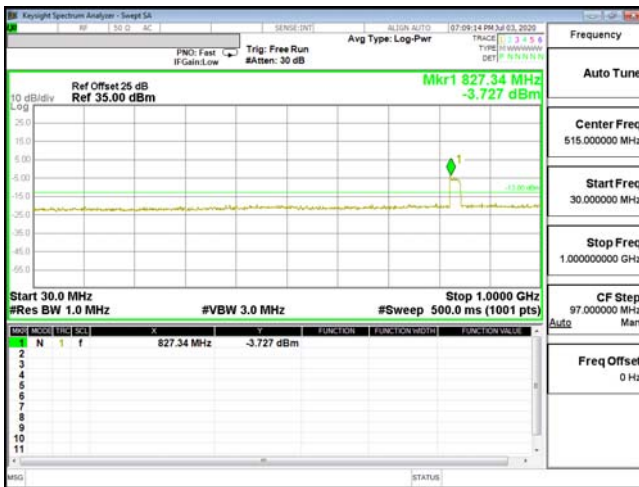
CSE-ENDC_2A_n5-QPSK_1.4M_CH18607_1850.7(6,0)
