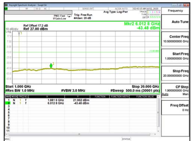
CSE-ENDC_2A_n5-64QAM_3M_CH18900_1880(1,14)
