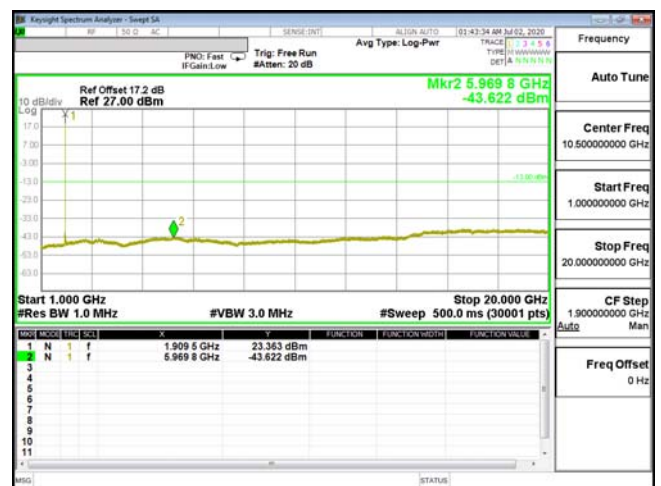
CSE-ENDC_2A_n5-16QAM_15M_CH19125_1902.5(1,74)
