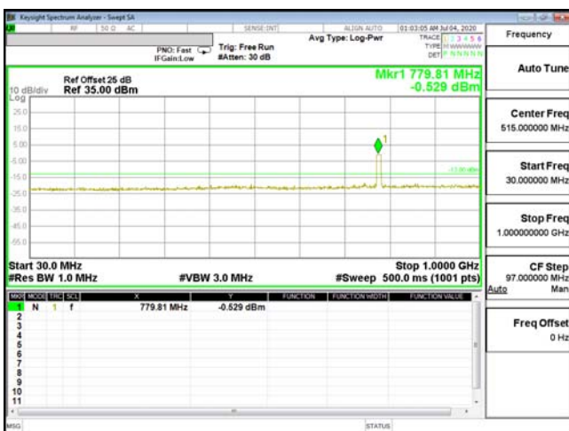
CSE-ENDC_13A_n66-256QAM_20M_CH354900_1745(100,6)
