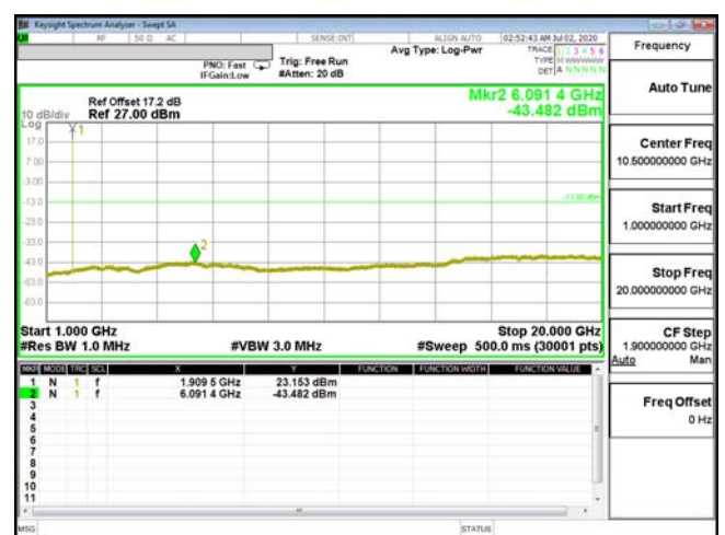
CSE-ENDC_2A_n5-16QAM_1.4M_CH19193_1909.3(1,3)-
