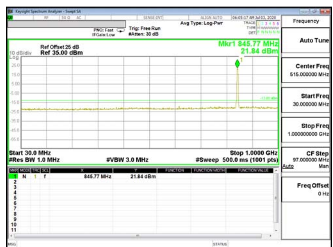
CSE-ENDC_5A_n2-QPSK_3M_CH20625_846.5(15,0)-30M-1G
