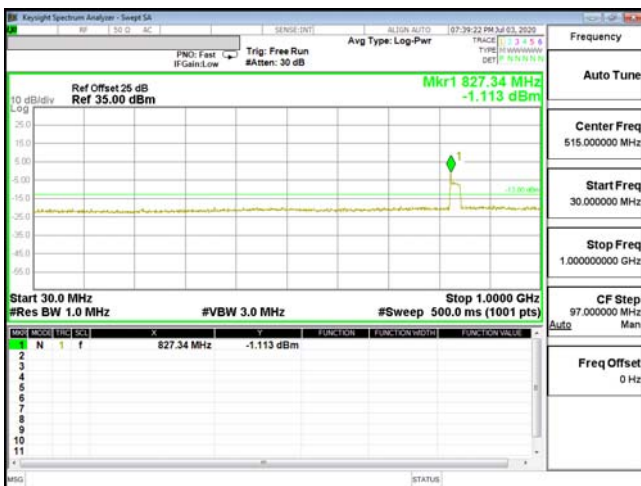
CSE-ENDC_2A_n5-QPSK_10M_CH18900_1880(50,0)
