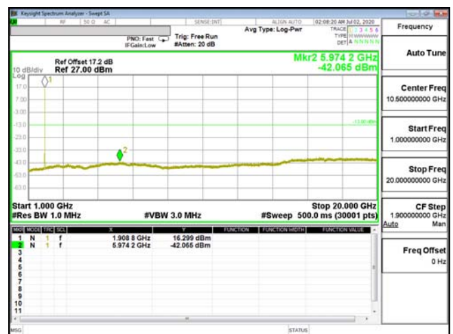
CSE-ENDC_2A_n5-QPSK_5M_CH19175_1907.5(25,0)
