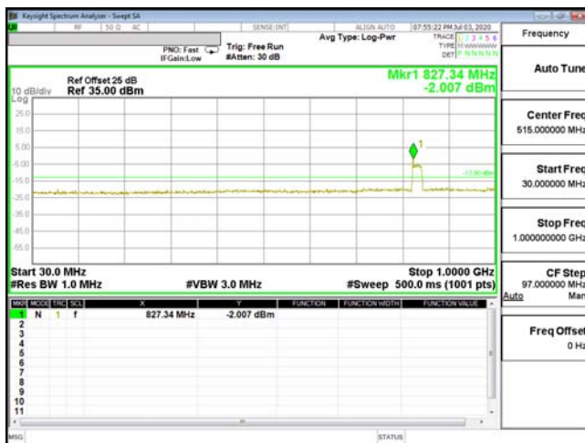
CSE-ENDC_2A_n5-64QAM_15M_CH18900_1880(1,37)
