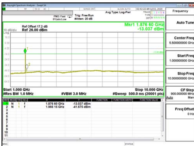
CSE-ENDC_5A_n2-QPSK_3M_CH20525_836.5(1,14)
