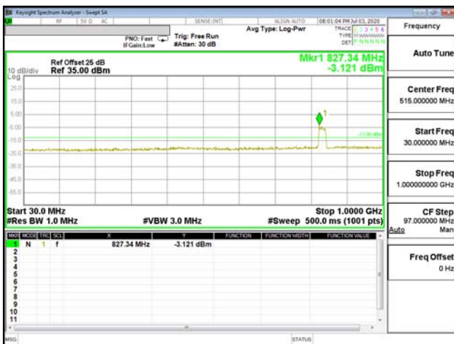
CSE-ENDC_2A_n5-QPSK_20M_CH18900_1880(100,0)
