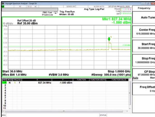
CSE-ENDC_2A_n5-QPSK_3M_CH18615_1851.5(15,0)
