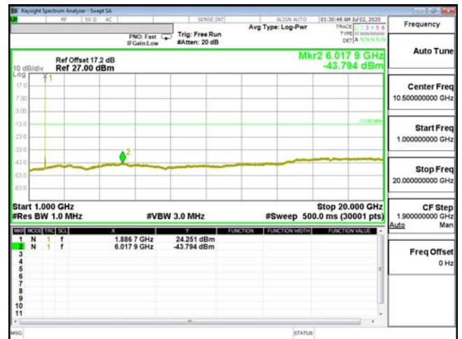
CSE-ENDC_2A_n5-16QAM_15M_CH18900_1880(1,74)
