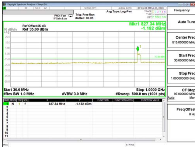
CSE-ENDC_2A_n5-16QAM_3M_CH18615_1851.5(1,0)
