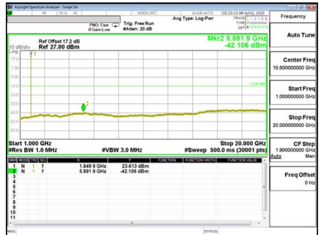
CSE-ENDC_2A_n5-16QAM_3M_CH18615_1851.5(1,0)
