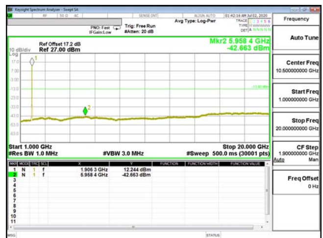
CSE-ENDC_2A_n5-QPSK_15M_CH19125_1902.5(75,0)
