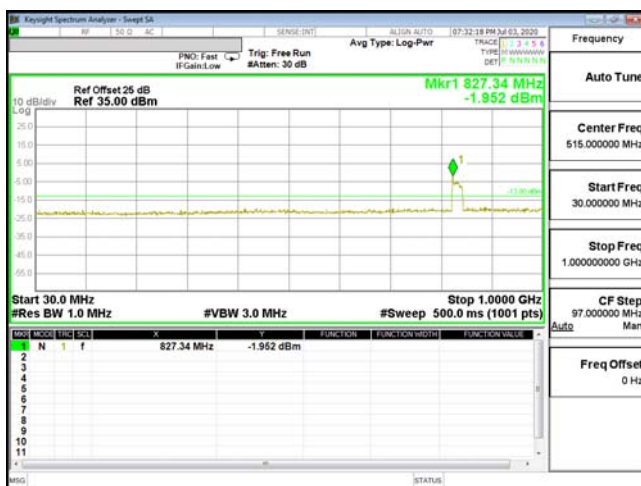
CSE-ENDC_2A_n5-64QAM_5M_CH19175_1907(1,12)
