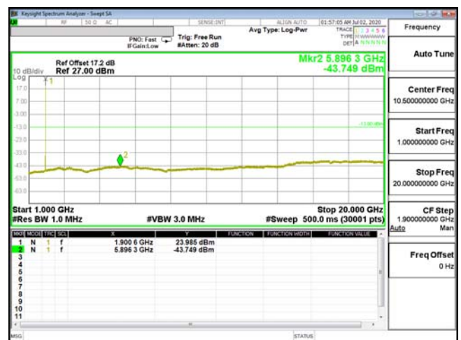
CSE-ENDC_2A_n5-16QAM_10M_CH19150_1905(1,0)
