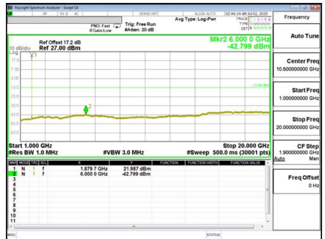
CSE-ENDC_2A_n5-64QAM_1.4M_CH18900_1880(1,3)
