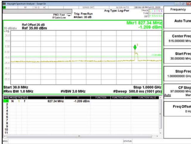
CSE-ENDC_2A_n5-64QAM_20M_CH18700_1860(1,0)
