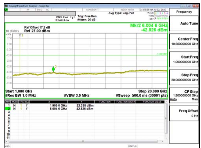
CSE-ENDC_2A_n5-64QAM_10M_CH19150_1905(1,25)
