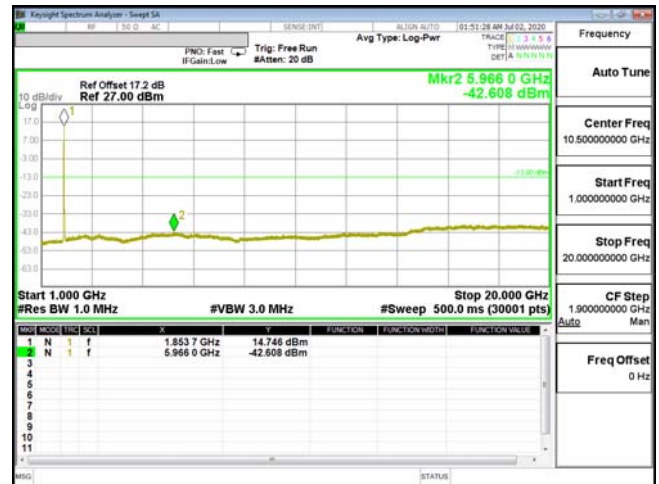
CSE-ENDC_2A_n5-QPSK_10M_CH18650_1855(50,0)
