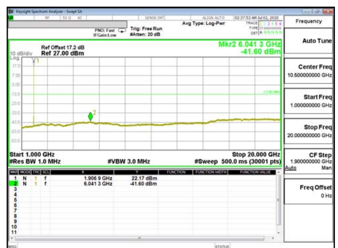
CSE-ENDC_2A_n5-64QAM_3M_CH19185_1908.5(1,0)
