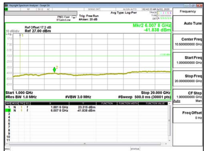
CSE-ENDC_2A_n5-16QAM_3M_CH18900_1880(1,14)
