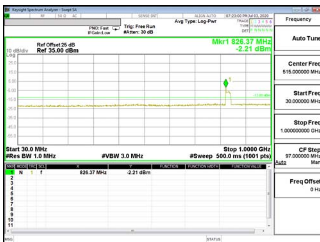
CSE-ENDC_2A_n5-16QAM_3M_CH19185_1908.5(1,0)
