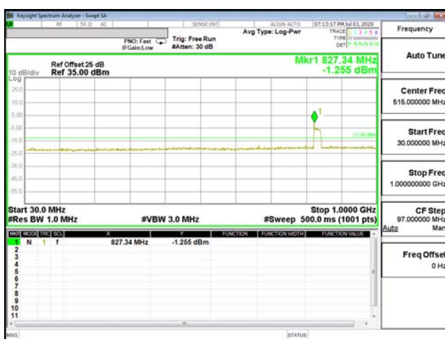
CSE-ENDC_2A_n5-16QAM_1.4M_CH19193_1909.3(1,3)
