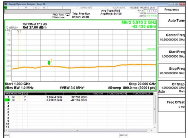
CSE-ENDC_2A_n5-64QAM_5M_CH18625_1852.5(1,24)
