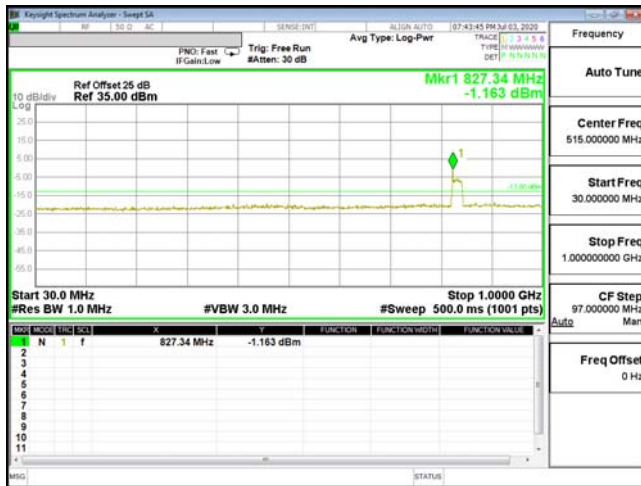
CSE-ENDC_2A_n5-64QAM_10M_CH18650_1855(1,49)
