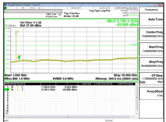
CSE-ENDC_13A_n66-256QAM_15M_CH354900_1745(75,0)
