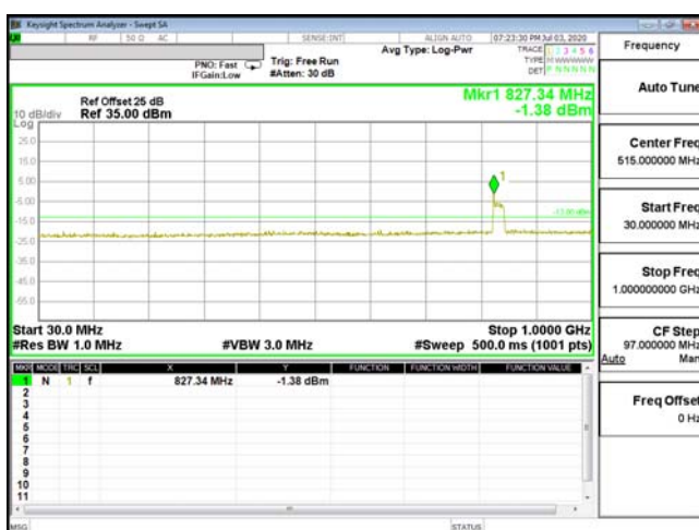
CSE-ENDC_2A_n5-64QAM_3M_CH19185_1908.5(1,0)
