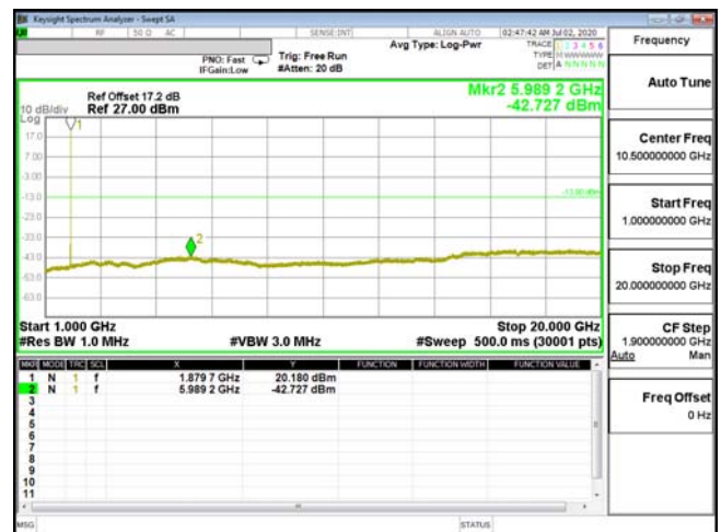
CSE-ENDC_2A_n5-QPSK_1.4M_CH18900_1880(6,0)-
