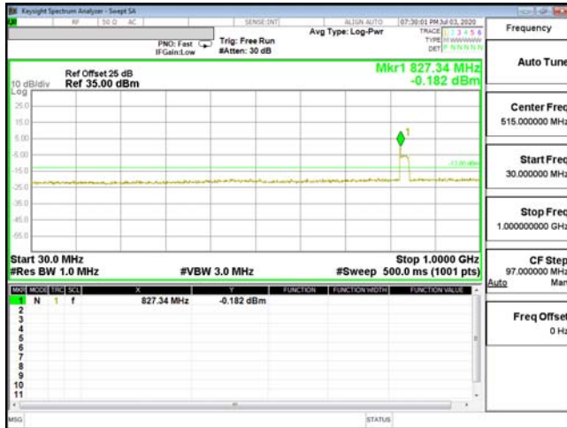
CSE-ENDC_2A_n5-16QAM_5M_CH18625_1852.5(1,0)
