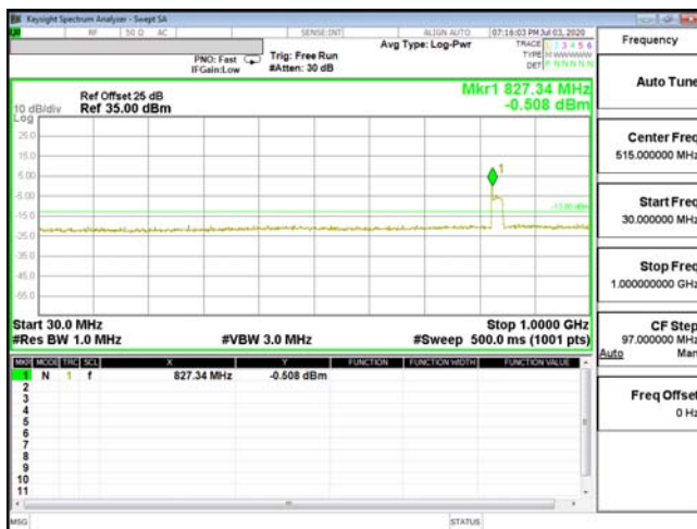
CSE-ENDC_2A_n5-16QAM_1.4M_CH18900_1880(1,3)
