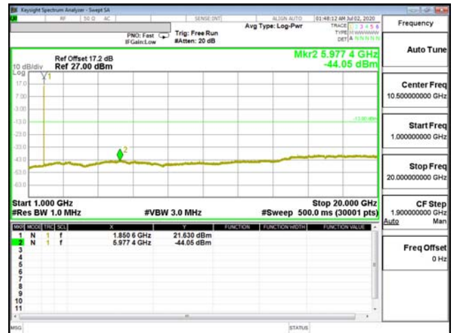
CSE-ENDC_2A_n5-QPSK_15M_CH18675_1857.5(1,0)
