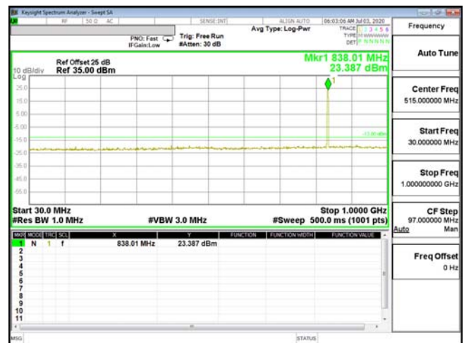
CSE-ENDC_5A_n2-QPSK_3M_CH20525_836.5(1,14)30M-1G
