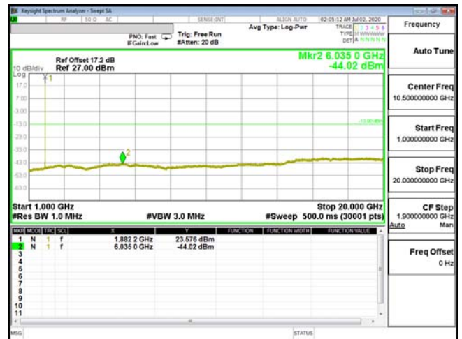
CSE-ENDC_2A_n5-16QAM_5M_CH18900_1880(1,24)
