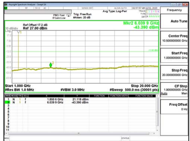
CSE-ENDC_2A_n5-QPSK_1.4M_CH18607_1850.7(6,0)-
