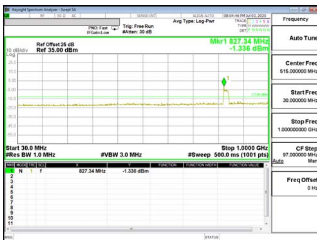
CSE-ENDC_2A_n5-64QAM_20M_CH19100_1900(1,0)
