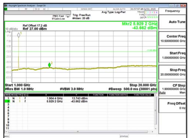
CSE-ENDC_2A_n5-QPSK_10M_CH19150_1905(50,0)
