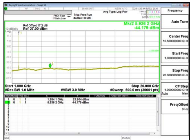
CSE-ENDC_2A_n5-16QAM_10M_CH18900_1880(1,49)-
