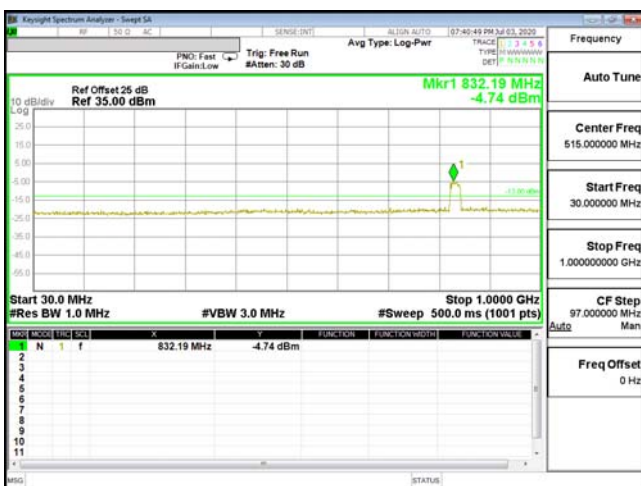
CSE-ENDC_2A_n5-QPSK_10M_CH19150_1905(50,0)
