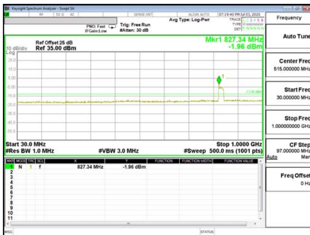
CSE-ENDC_2A_n5-16QAM_3M_CH18900_1880(1,14)
