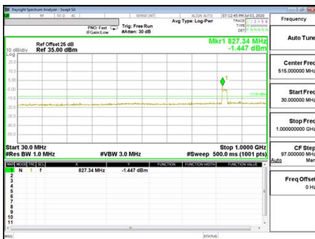
CSE-ENDC_2A_n5-64QAM_1.4M_CH19193_1909.3(1,3)
