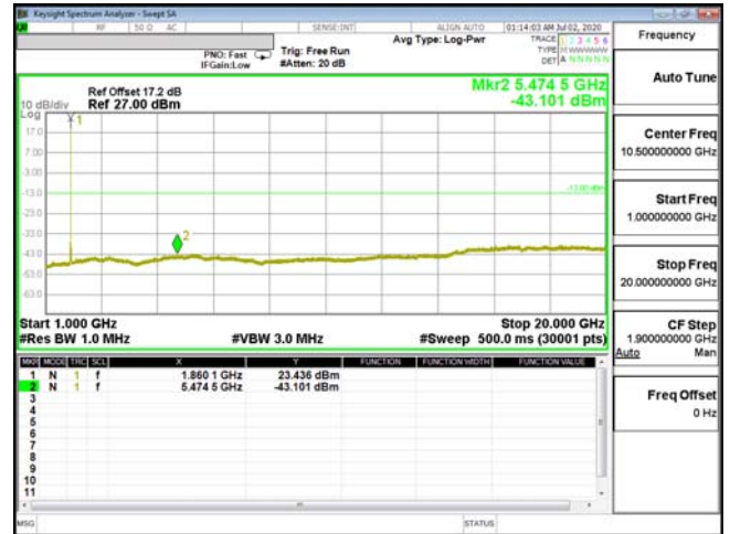
CSE-ENDC_2A_n5-16QAM_20M_CH18700_1860(1,50)
