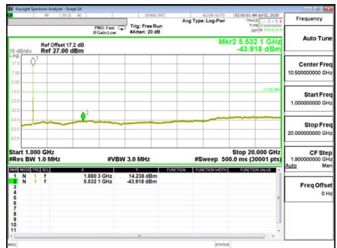
CSE-ENDC_2A_n5-QPSK_10M_CH18900_1880(50,0)
