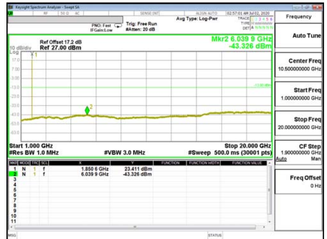
CSE-ENDC_2A_n5-16QAM_1.4M_CH18607_1850.7(1,3)-
