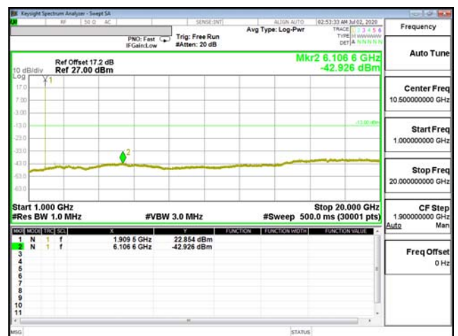
CSE-ENDC_2A_n5-64QAM_1.4M_CH19193_1909.3(1,3)
