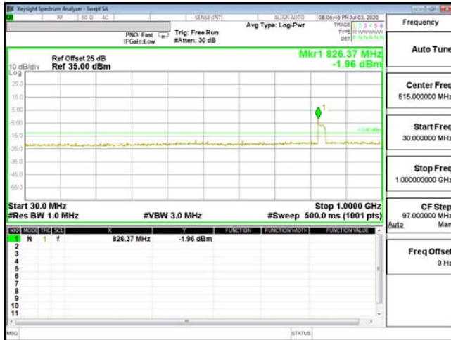
CSE-ENDC_2A_n5-16QAM_20M_CH18700_1860(1,50)
