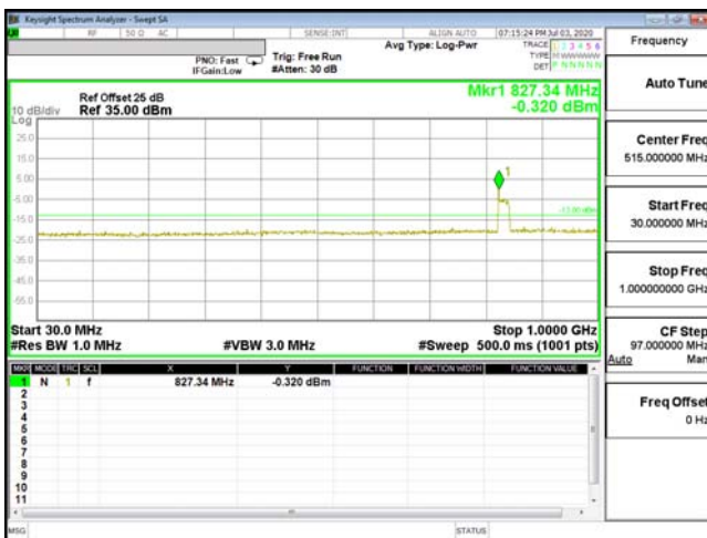
CSE-ENDC_2A_n5-QPSK_1.4M_CH18900_1880(6,0)
