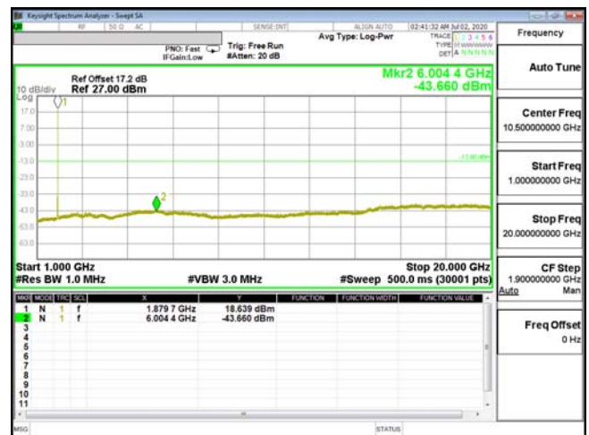
CSE-ENDC_2A_n5-QPSK_3M_CH18900_1880(15,0)-
