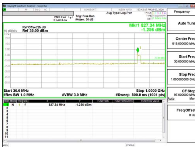
CSE-ENDC_2A_n5-64QAM_10M_CH19150_1905(1,25)
