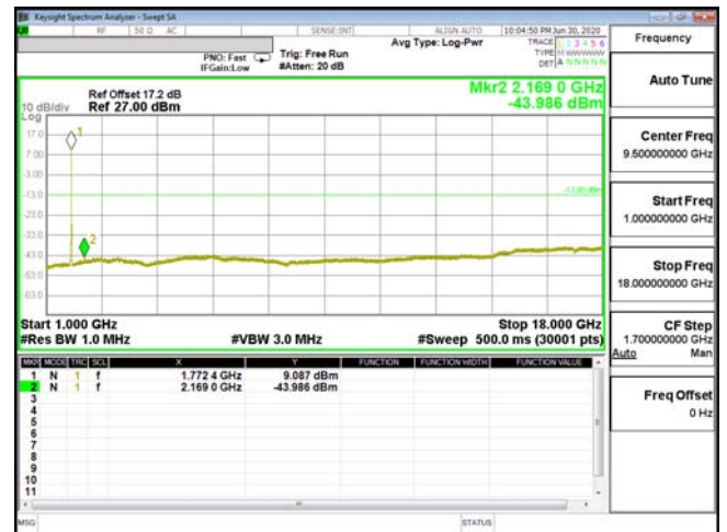
CSE-ENDC_13A_n66-256QAM_15M_CH354500_1772.5(75,4)
