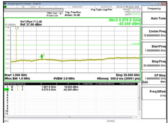
CSE-ENDC_2A_n5-QPSK_3M_CH18615_1851.5(15,0)-
