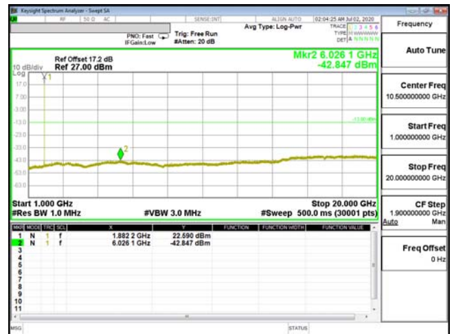
CSE-ENDC_2A_n5-64QAM_5M_CH18900_1880(1,24)
