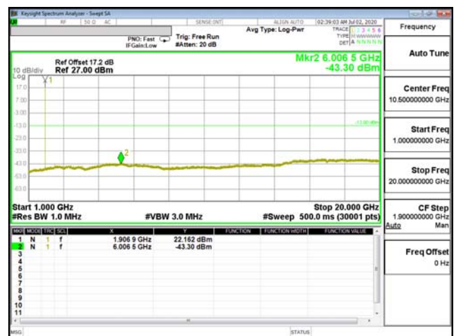
CSE-ENDC_2A_n5-16QAM_3M_CH19185_1908.5(1,0)
