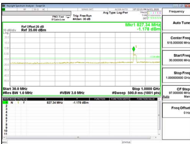
CSE-ENDC_2A_n5-QPSK_3M_CH19185_1908.5(15,0)
