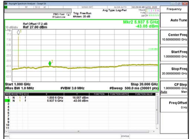
CSE-ENDC_2A_n5-QPSK_5M_CH18625_1852.5(25,0)
