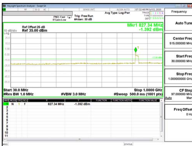
CSE-ENDC_2A_n5-16QAM_5M_CH19175_1907.5(1,0)
