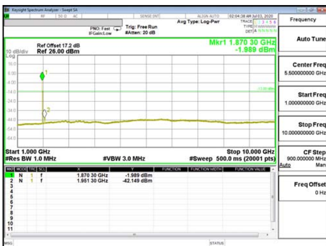
CSE-ENDC_5A_n2-QPSK_5M_CH20625_846.5(1,0)
