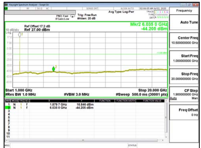
CSE-ENDC_2A_n5-QPSK_5M_CH18900_1880(25,0)
