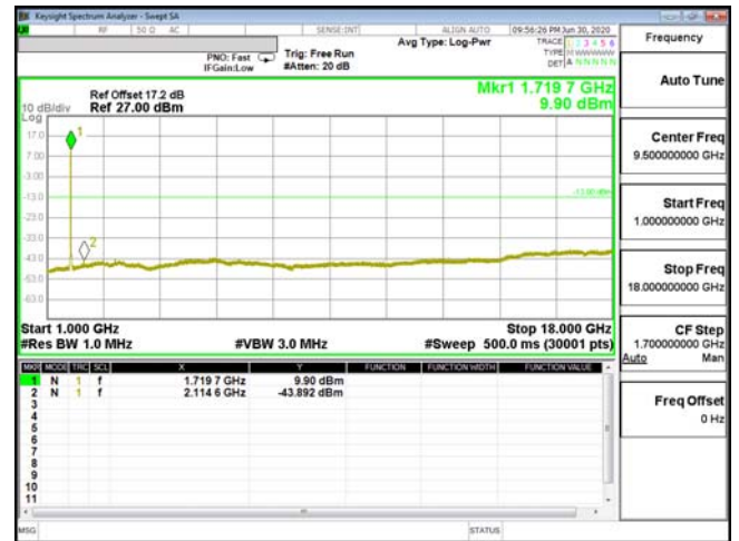
CSE-ENDC_13A_n66-256QAM_15M_CH343500_1717.5(75,0)
