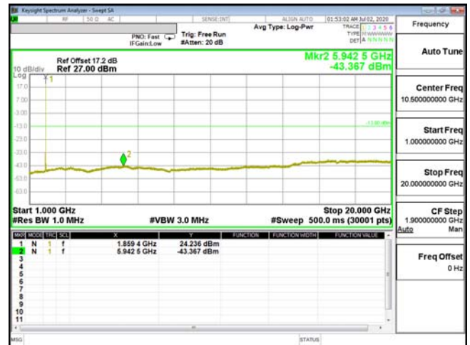
CSE-ENDC_2A_n5-16QAM_10M_CH18650_1855(1,49)-
