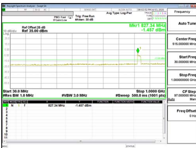
CSE-ENDC_2A_n5-QPSK_20M_CH19100_1900(100,0)
