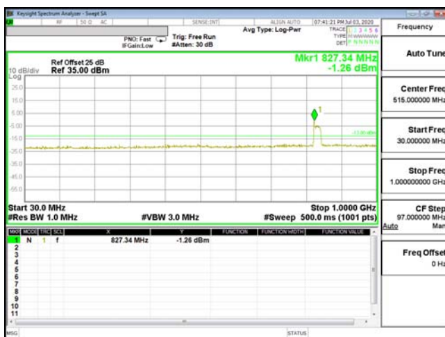
CSE-ENDC_2A_n5-16QAM_10M_CH19150_1905(1,0)
