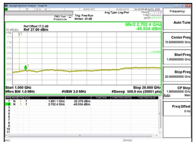
CSE-ENDC_2A_n5-64QAM_20M_CH19100_1900(1,0)
