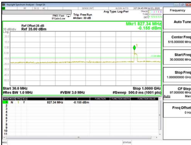
CSE-ENDC_2A_n5-QPSK_5M_CH18900_1880(25,0)
