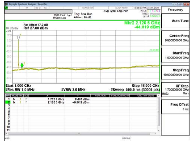
CSE-ENDC_13A_n66-256QAM_20M_CH344000_1720(100,6)
