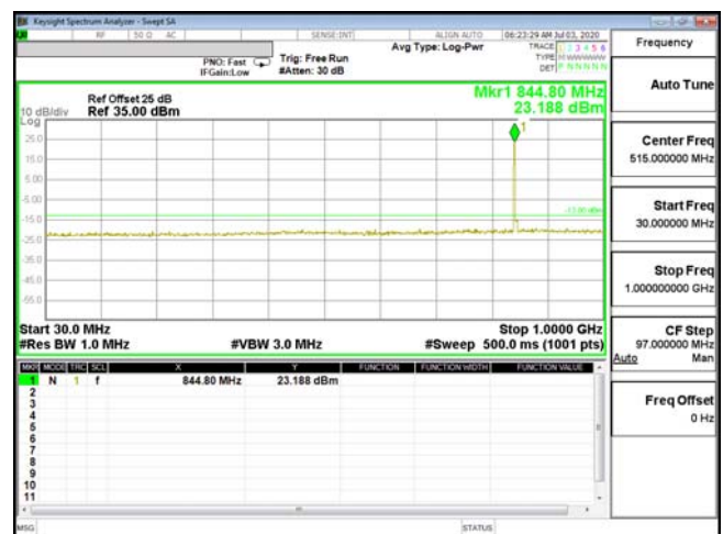
CSE-ENDC_5A_n2-QPSK_5M_CH20625_846.5(1,0)30M-1G
