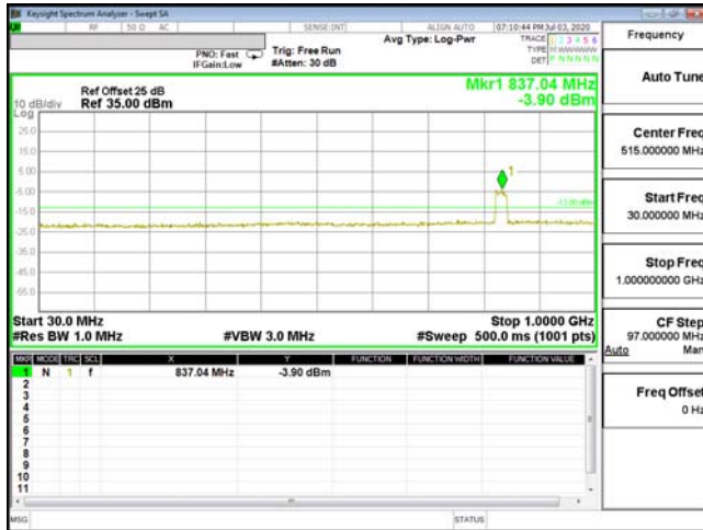
CSE-ENDC_2A_n5-64QAM_1.4M_CH18607_1850.7(1,3)
