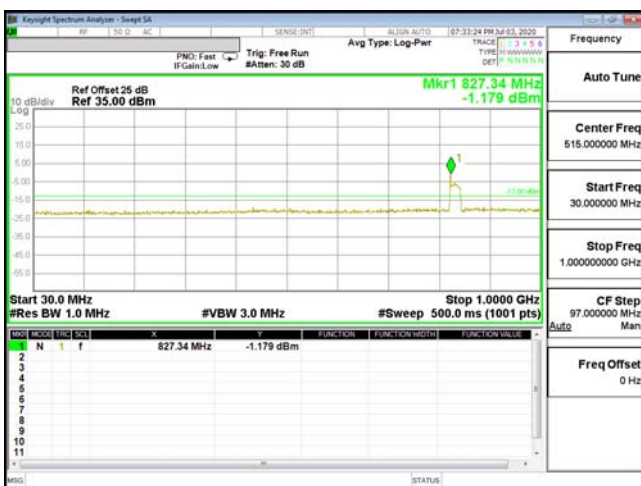
CSE-ENDC_2A_n5-QPSK_5M_CH19175_1907.5(25,0)
