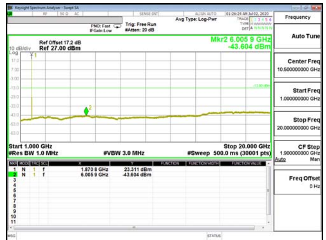
CSE-ENDC_2A_n5-16QAM_20M_CH18900_1880(1,0)
