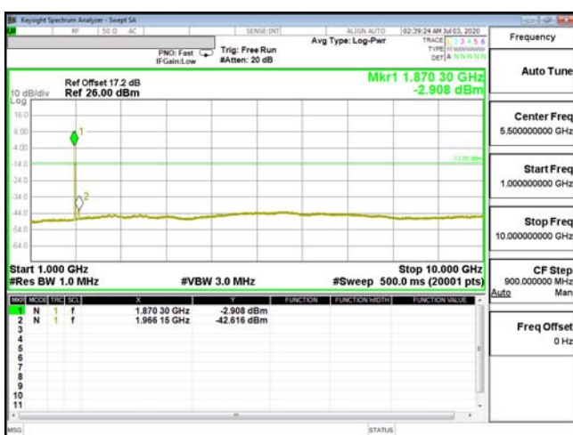
CSE-ENDC_5A_n2-QPSK_3M_CH20625_846.5(15,0)
