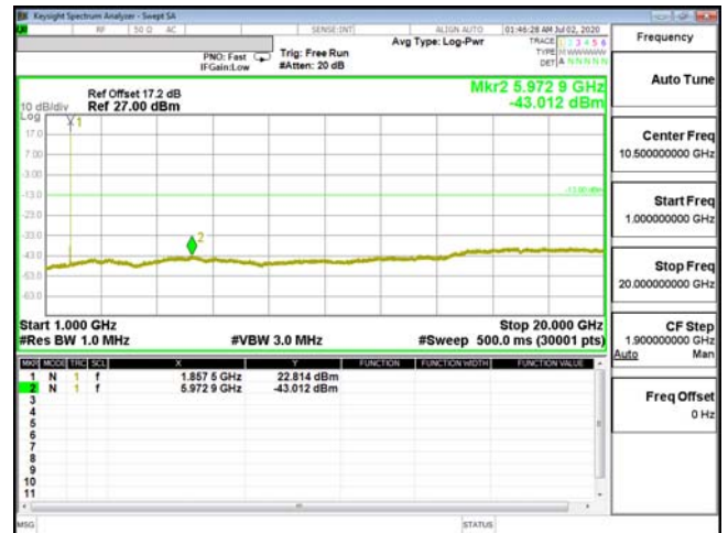
CSE-ENDC_2A_n5-64QAM_15M_CH18675_1857.5(1,37)
