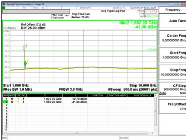
CSE-ENDC_5A_n2-QPSK_3M_CH20415_825.5(1,7)
