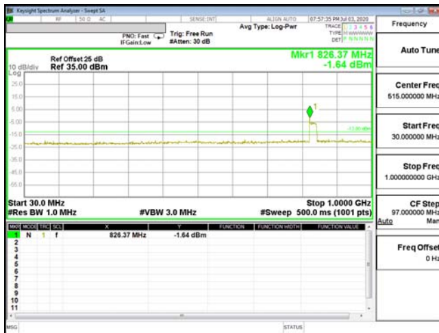
CSE-ENDC_2A_n5-64QAM_20M_CH18900_1880(1,50)
