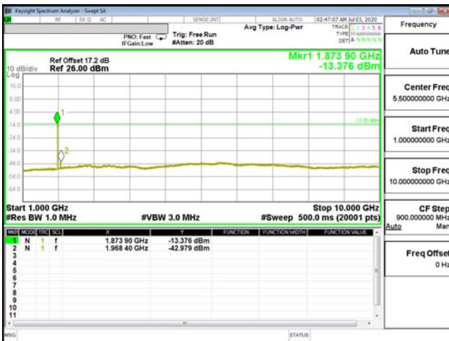
CSE-ENDC_5A_n2-QPSK_1.4M_CH20525_836.5(6,0)
