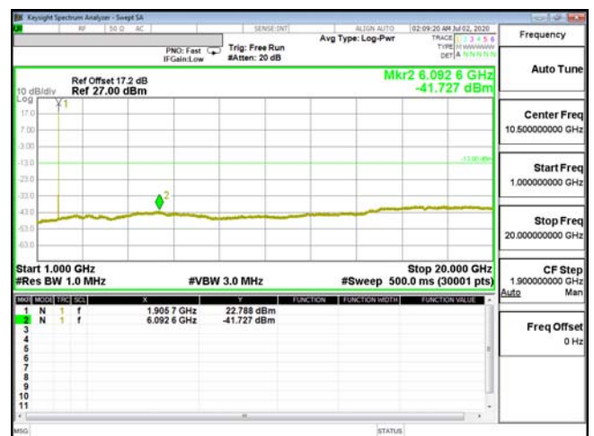
CSE-ENDC_2A_n5-16QAM_5M_CH19175_1907.5(1,0)
