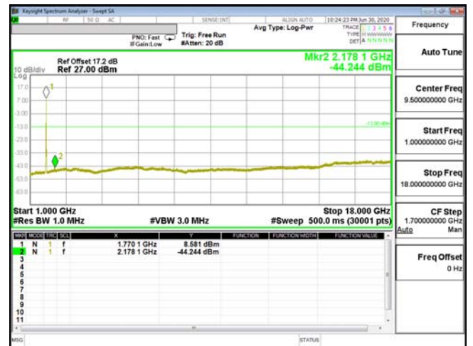
CSE-ENDC_13A_n66-256QAM_20M_CH354000_1770(100,6)
