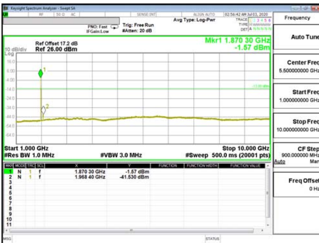
CSE-ENDC_5A_n2-QPSK_1.4M_CH20643_848.3((1,3)
