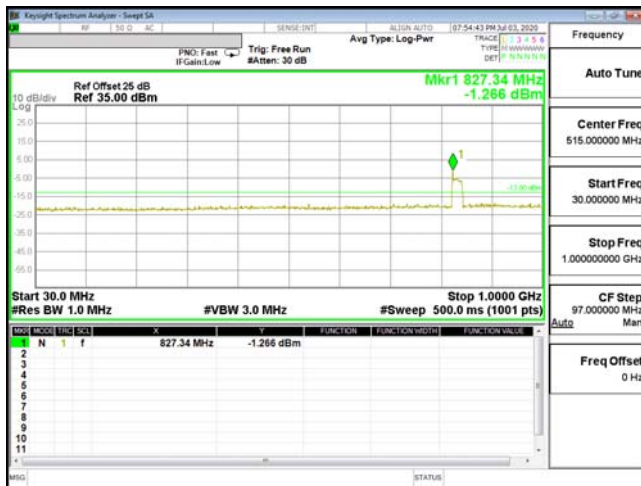
CSE-ENDC_2A_n5-16QAM_15M_CH18900_1880(1,74)
