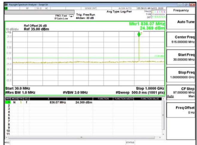
CSE-ENDC_5A_n2-QPSK_1.4M_CH20525_836.5(6,0)-30M-1G
