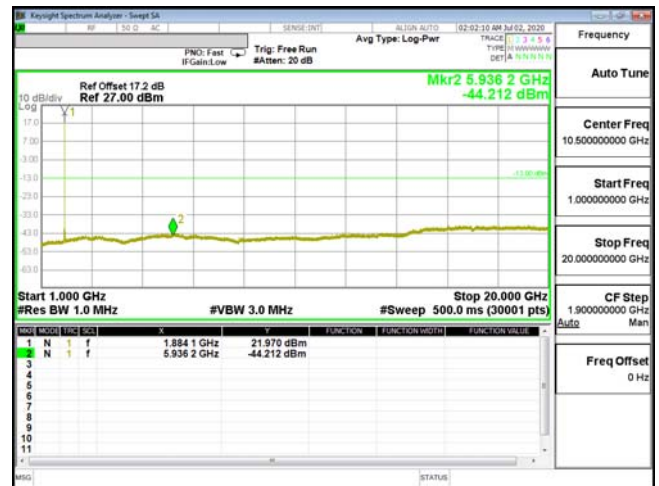
CSE-ENDC_2A_n5-64QAM_10M_CH18900_1880(1,49)
