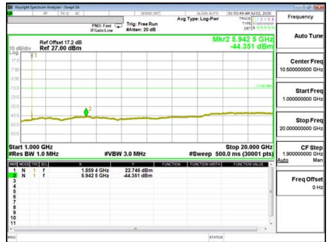
CSE-ENDC_2A_n5-64QAM_10M_CH18650_1855(1,49)
