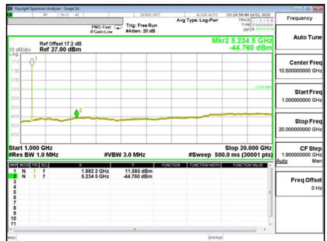
CSE-ENDC_2A_n5-QPSK_20M_CH18900_1880(100,0)
