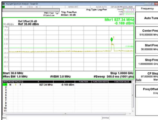
CSE-ENDC_2A_n5-64QAM_1.4M_CH18900_1880(1,3)
