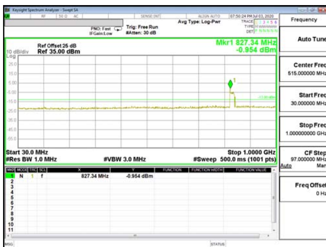
CSE-ENDC_2A_n5-16QAM_15M_CH19125_1902.5(1,74)
