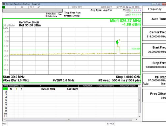
CSE-ENDC_2A_n5-16QAM_5M_CH18900_1880(1,24)
