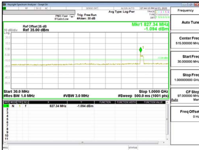
CSE-ENDC_2A_n5-16QAM_10M_CH18650_1855(1,49)
