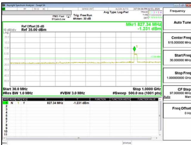
CSE-ENDC_2A_n5-QPSK_15M_CH18900_1880(1,74)
