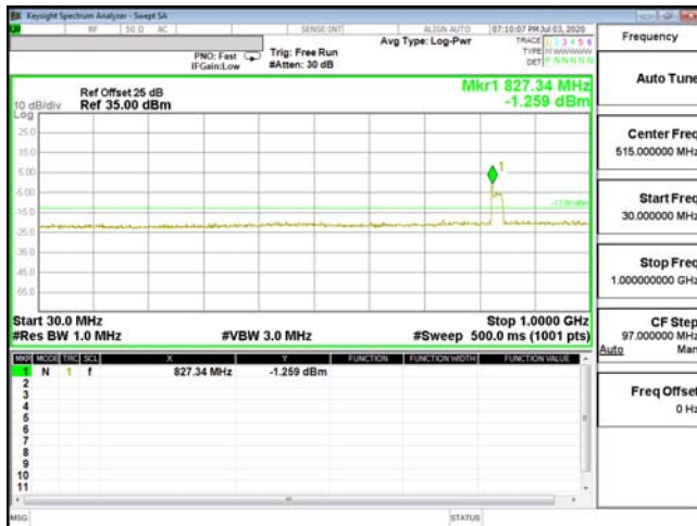
CSE-ENDC_2A_n5-16QAM_1.4M_CH18607_1850.7(1,3)
