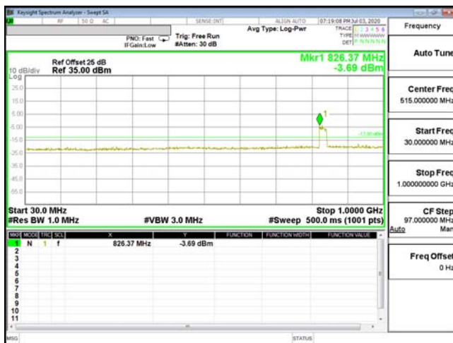
CSE-ENDC_2A_n5-64QAM_3M_CH18900_1880(1,14)
