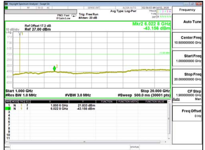
CSE-ENDC_2A_n5-64QAM_1.4M_CH18607_1850.7(1,3)
