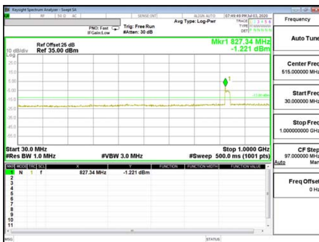
CSE-ENDC_2A_n5-64QAM_15M_CH19125_1902.5(1,74)
