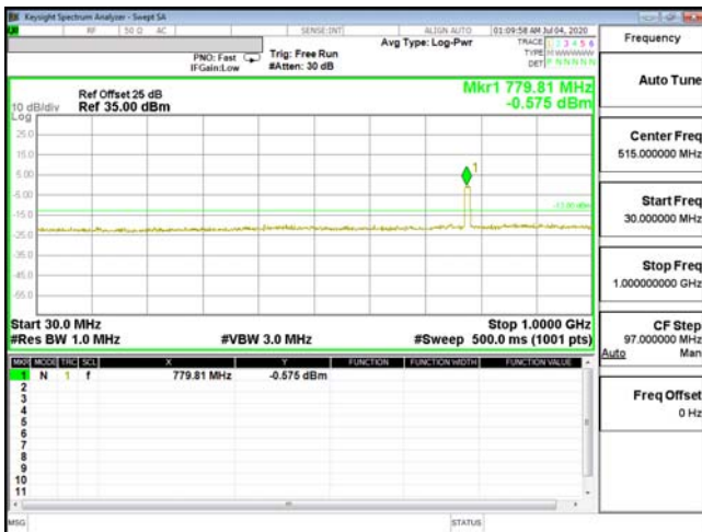
CSE-ENDC_13A_n66-256QAM_20M_CH354000_1770(100,6)
