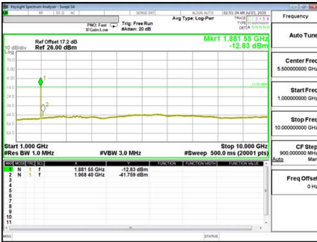
CSE-ENDC_5A_n2-QPSK_1.4M_CH20407_824.7(6,0)
