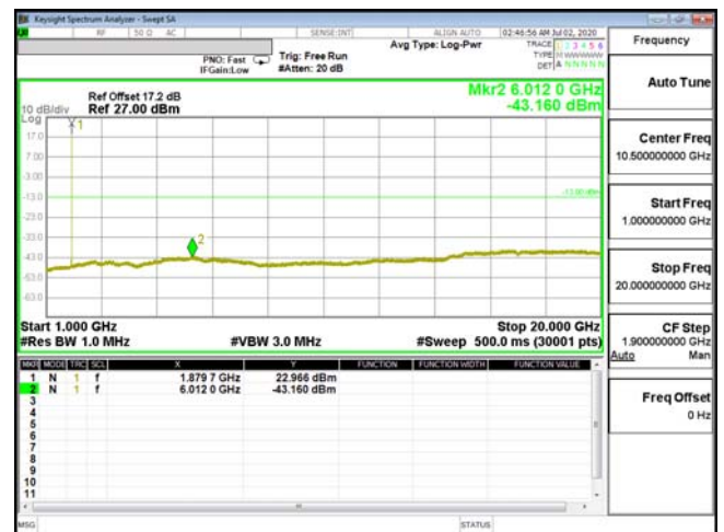
CSE-ENDC_2A_n5-16QAM_1.4M_CH18900_1880(1,3)-
