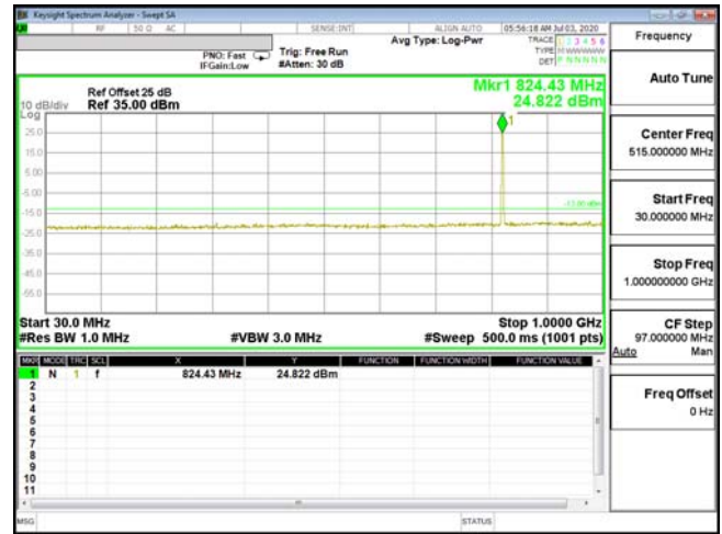
CSE-ENDC_5A_n2-QPSK_1.4M_CH20407_824.7(6,0)-30M-1G
