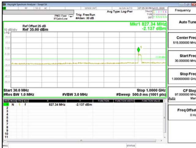
CSE-ENDC_2A_n5-64QAM_3M_CH18615_1851.5(1,14)
