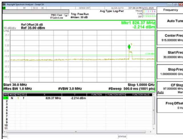
CSE-ENDC_2A_n5-64QAM_10M_CH18900_1880(1,49)
