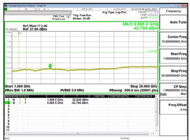
CSE-ENDC_2A_n5-64QAM_15M_CH19125_1902.5(1,74)
