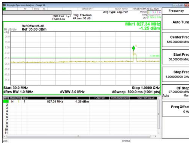
CSE-ENDC_2A_n5-16QAM_10M_CH18900_1880(1,49)
