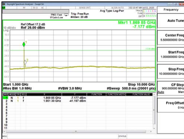
CSE-ENDC_5A_n2-QPSK_5M_CH20425_826.5(1,12)
