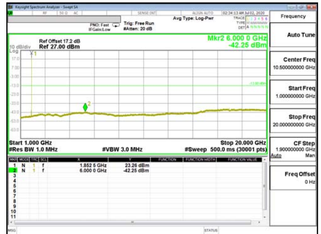
CSE-ENDC_2A_n5-64QAM_3M_CH18615_1851.5(1,14)
