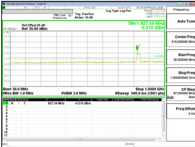
CSE-ENDC_2A_n5-QPSK_5M_CH18625_1852.5(25,0)
