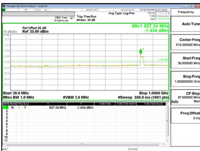
CSE-ENDC_2A_n5-QPSK_15M_CH19125_1902.5(75,0)
