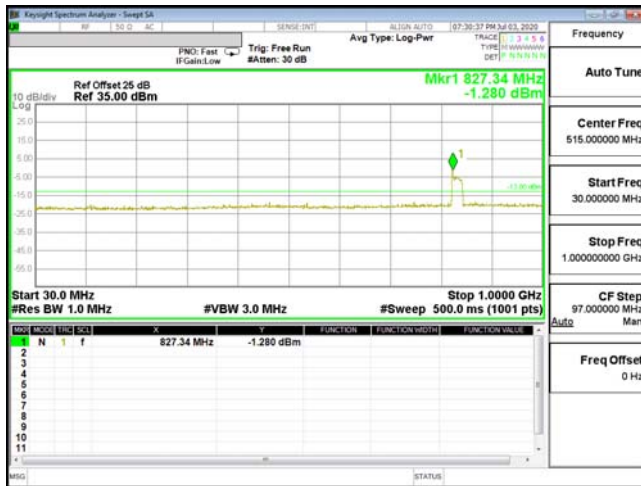
CSE-ENDC_2A_n5-64QAM_5M_CH18625_1852.5(1,24)
