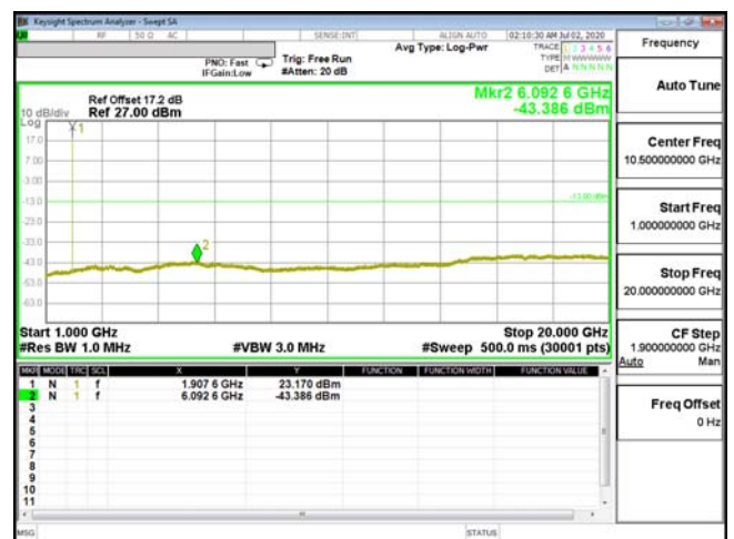
CSE-ENDC_2A_n5-64QAM_5M_CH19175_1907(1,12)
