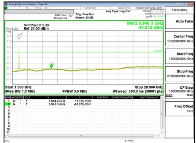
CSE-ENDC_2A_n5-QPSK_20M_CH18700_1860(100,0)
