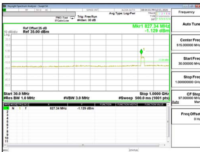
CSE-ENDC_2A_n5-16QAM_20M_CH19100_1900(1,0)
