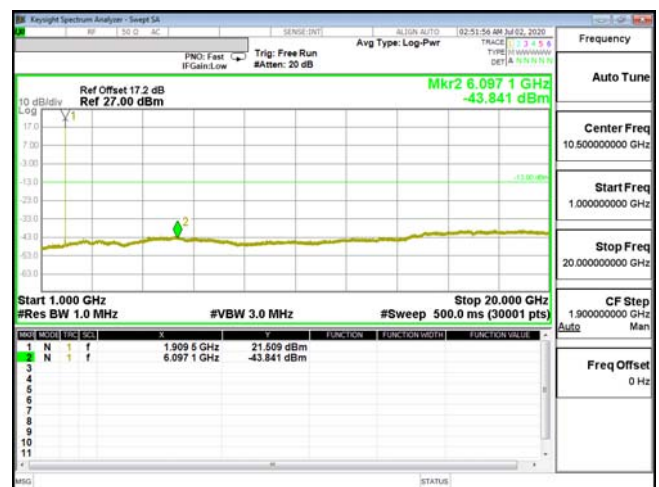
CSE-ENDC_2A_n5-QPSK_1.4M_CH19193_1909.3(1,3)-
