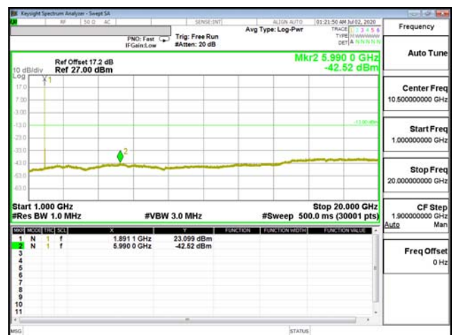
CSE-ENDC_2A_n5-16QAM_20M_CH19100_1900(1,0)
