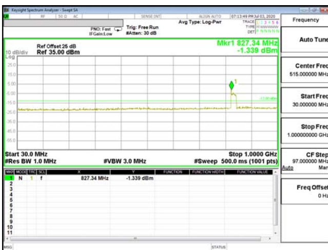
CSE-ENDC_2A_n5-QPSK_1.4M_CH19193_1909.3(1,3)
