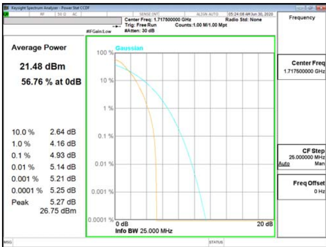
PTAR-ENDC_13A_n66-P12-BPSK_15M_CH343500_1717.5(75,0)
