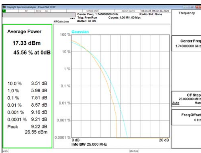
PTAR-ENDC_13A_n66-256QAM_20M_CH349000_1745(100,0)
