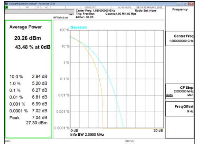
PTAR-ENDC_2A_n5-16QAM_1.4M_CH18900_1880(6,0)
