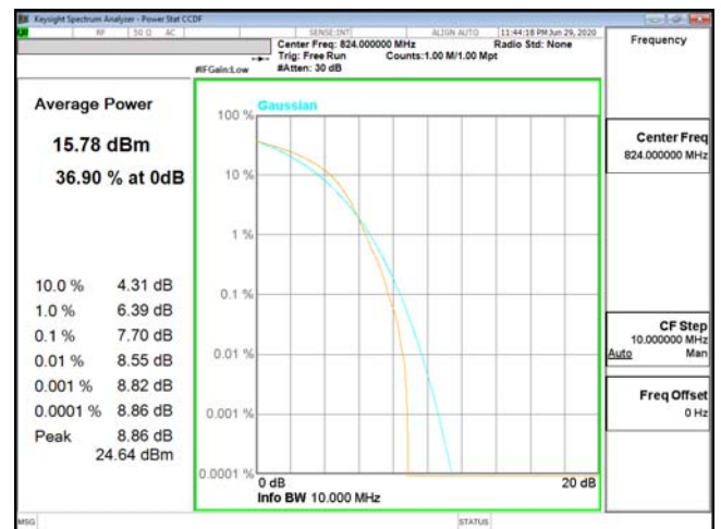
PTAR-ENDC_2A_n5-256QAM_10M_CH165800_824(50,0)
