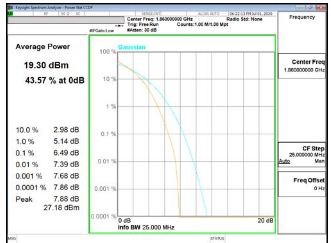
PTAR-ENDC_2A_n5-64QAM_20M_CH18700_1860(100,0)
