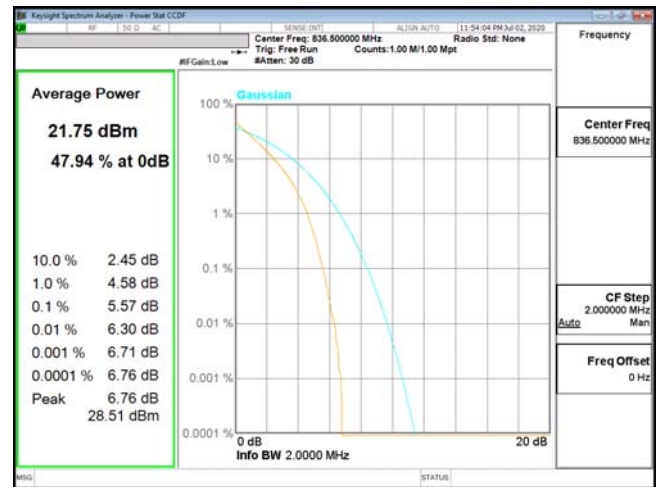
PTAR-ENDC_5A_n2-QPSK_1.4M_CH20525_836.5(6,0)
