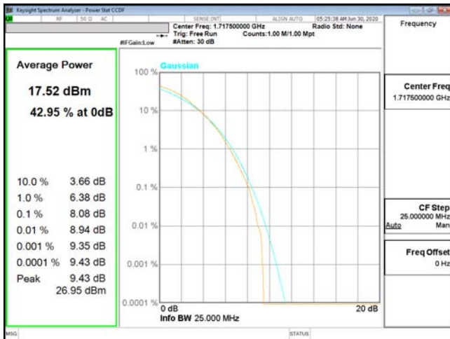
PTAR-ENDC_13A_n66-256QAM_15M_CH343500_1717.5(75,0)
