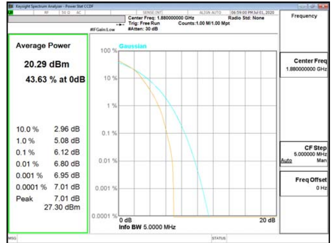
PTAR-ENDC_2A_n5-16QAM_5M_CH18900_1880(25,0)
