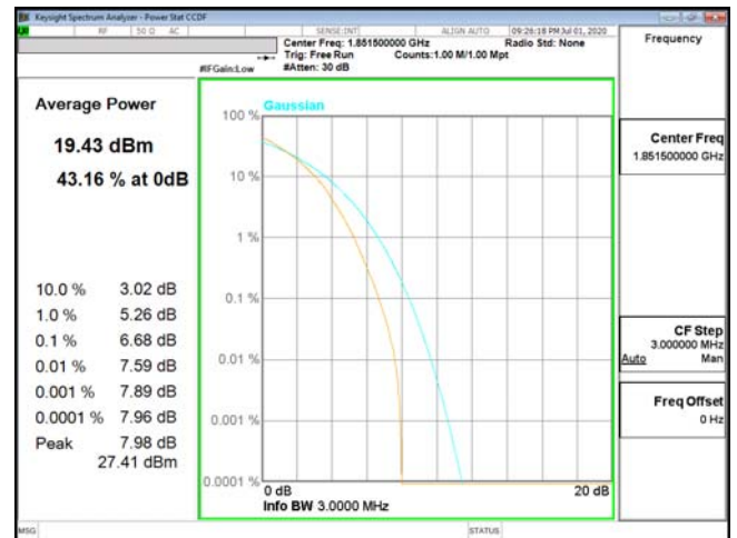
PTAR-ENDC_2A_n5-64QAM_3M_CH18615_1851.5(15,0)
