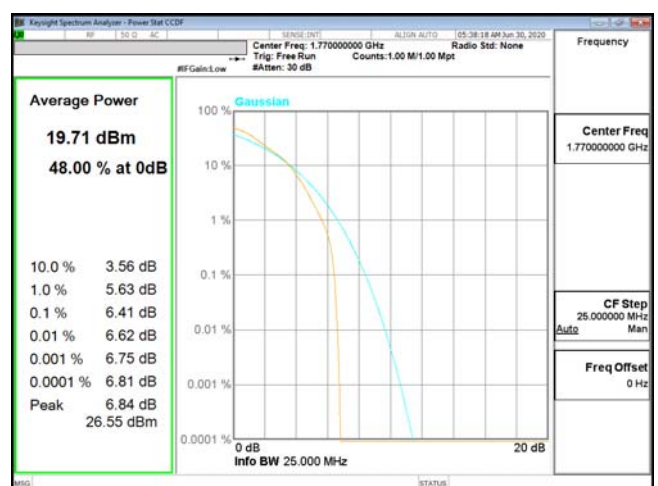
PTAR-ENDC_13A_n66-16QAM_20M_CH349000_1745(100,0) PTAR-ENDC_13A_n66-16QAM_20M_CH354000_1770(100,0)
