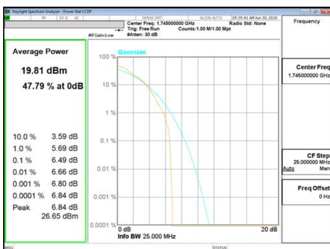
PTAR-ENDC_13A_n66-16QAM_20M_CH349000_1745(100,0) PTAR-ENDC_13A_n66-16QAM_20M_CH354000_1770(100,0)
