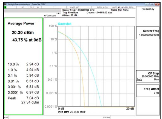
PTAR-ENDC_2A_n5-16QAM_20M_CH18700_1860(100,0)
