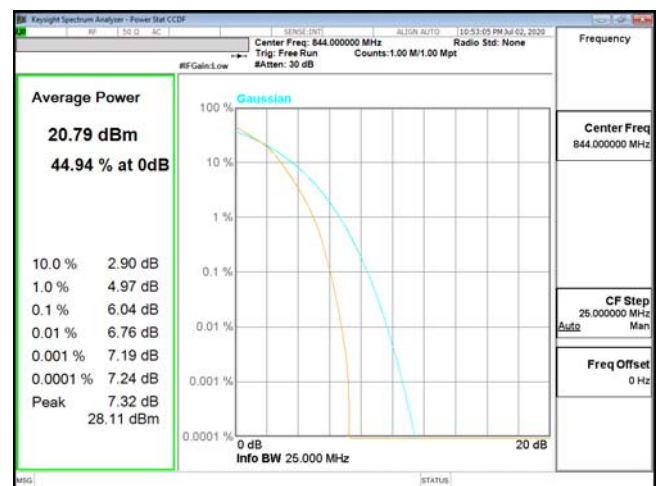
PTAR-ENDC_5A_n2-16QAM_10M_CH20600_844(50,0)
