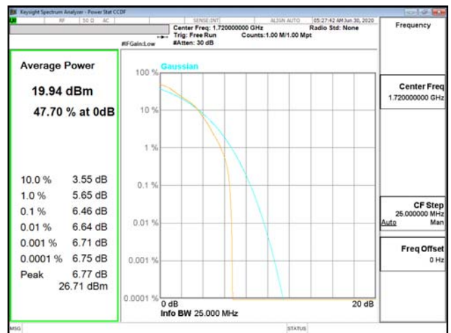
PTAR-ENDC_13A_n66-16QAM_15M_CH354500_1772.5(75,0) PTAR-ENDC_13A_n66-16QAM_20M_CH344000_1720(100,0)
