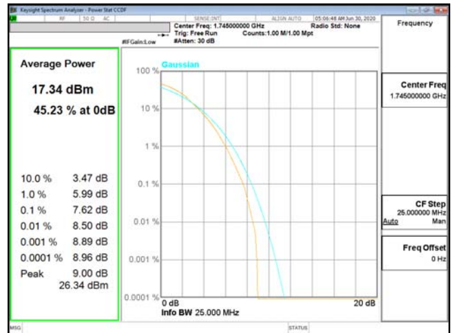
PTAR-ENDC_13A_n66-256QAM_15M_CH349000_1745(75,0)
