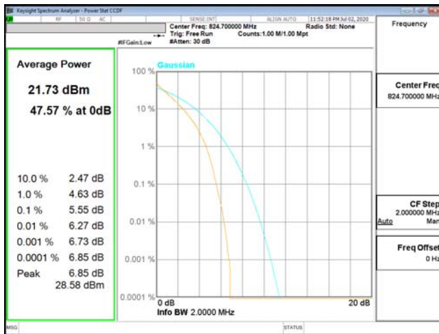
PTAR-ENDC_5A_n2-QPSK_1.4M_CH20407_824.7(6,0)
