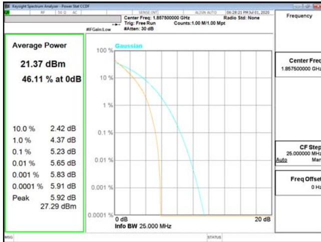
PTAR-ENDC_2A_n5-QPSK_15M_CH18675_1857.5(75,0)
