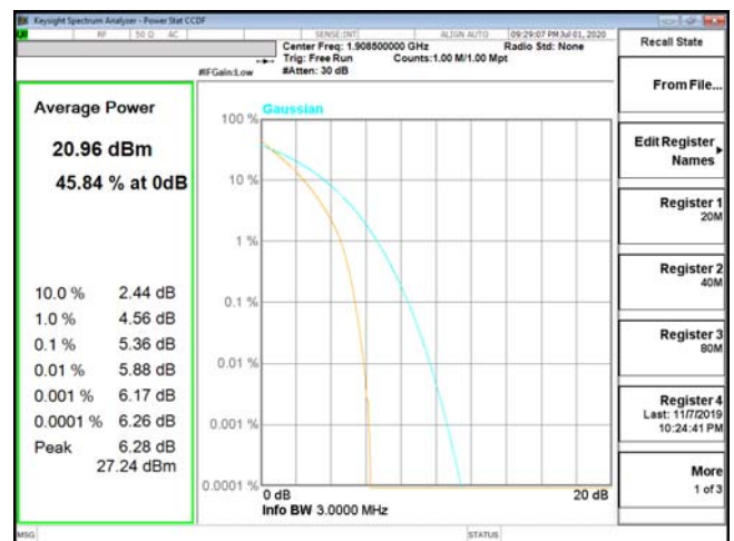
PTAR-ENDC_2A_n5-QPSK_3M_CH19185_1908.5(15,0)
