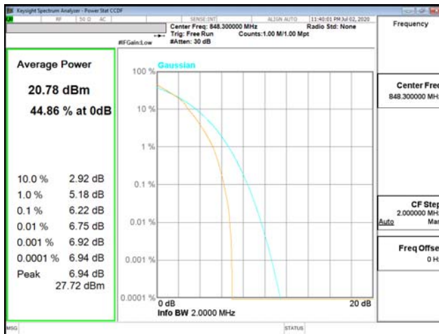
PTAR-ENDC_5A_n2-16QAM_1.4M_CH20643_848.3(6,0)
