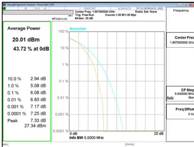
PTAR-ENDC_2A_n5-16QAM_5M_CH19175_1907.5(25,0)
