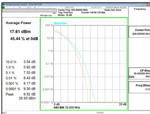
PTAR-ENDC_2A_n5-256QAM_20M_CH167300_836.5(100,0)
