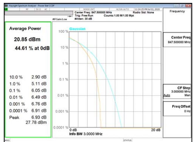
PTAR-ENDC_5A_n2-16QAM_3M_CH20635_847.5(15,0)
