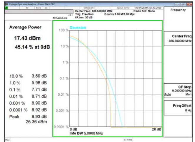
PTAR-ENDC_2A_n5-256QAM_5M_CH167300_836.5(25,0)
