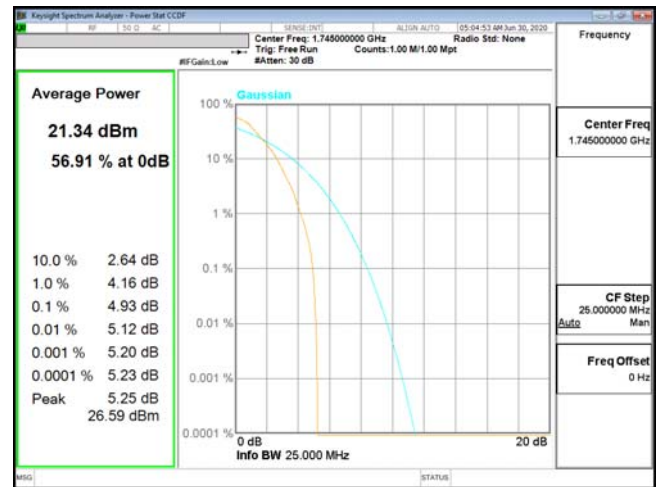
PTAR-ENDC_13A_n66-P12-BPSK_15M_CH349000_1745(75,0)
