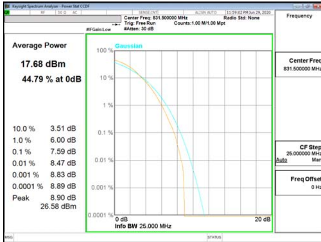
PTAR-ENDC_2A_n5-256QAM_15M_CH166300_831.5(75,0)
