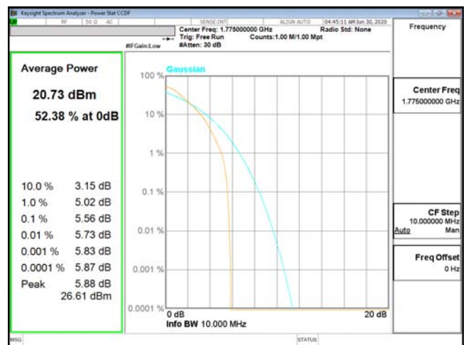
PTAR-ENDC_13A_n66-QPSK_10M_CH355000_1775(50,0)
