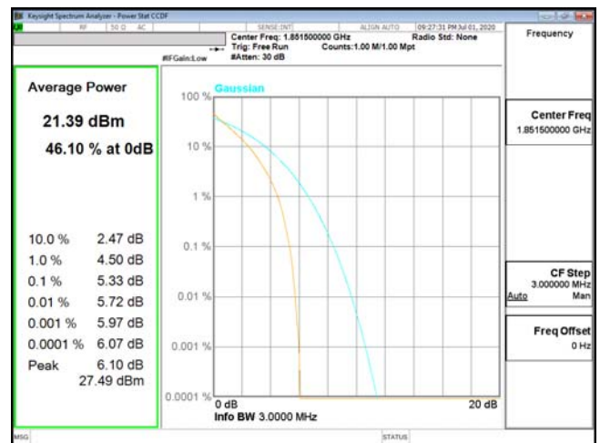
PTAR-ENDC_2A_n5-QPSK_3M_CH18615_1851.5(15,0)
