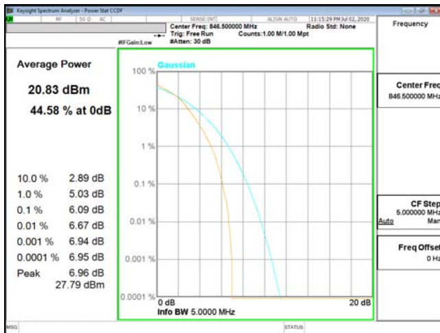
PTAR-ENDC_5A_n2-16QAM_5M_CH20625_846.5(25,0)
