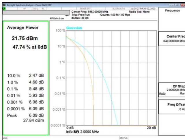
PTAR-ENDC_5A_n2-QPSK_1.4M_CH20643_848.3(6,0)
