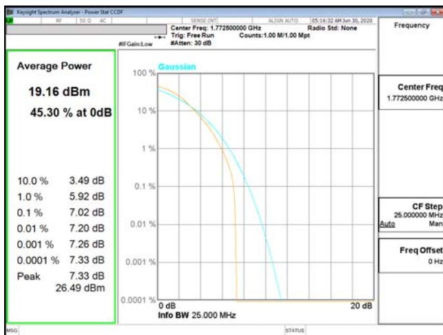
PTAR-ENDC_13A_n66-64QAM_15M_CH354500_1772.5(75,0)
