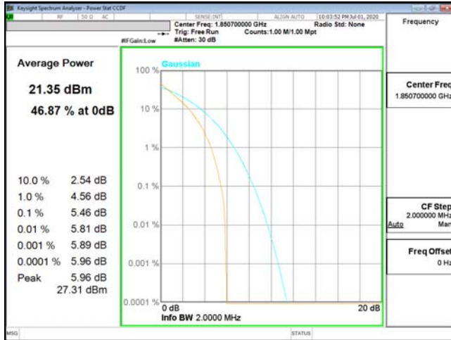
PTAR-ENDC_2A_n5-QPSK_1.4M_CH18607_18507(6,0)
