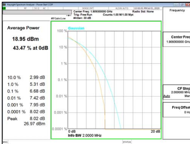
PTAR-ENDC_2A_n5-64QAM_1.4M_CH19193_1909.3(6,0)
