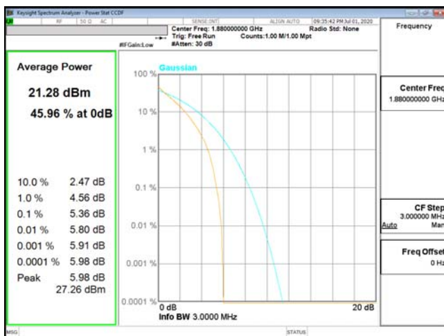
PTAR-ENDC_2A_n5-QPSK_3M_CH18900_1880(15,0)
