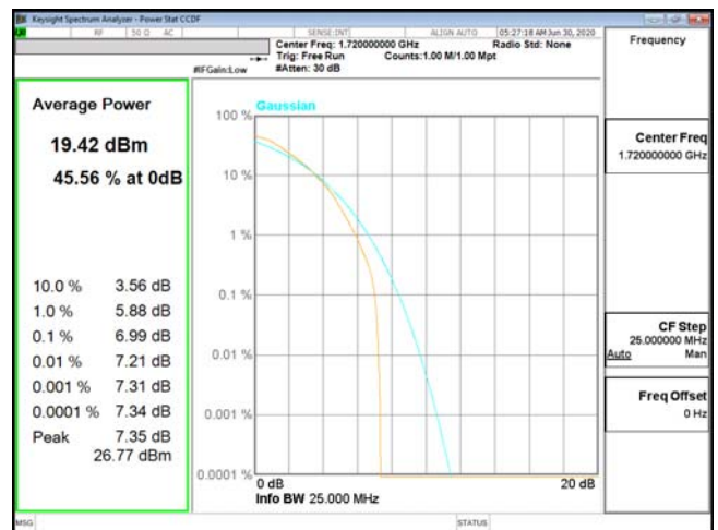
PTAR-ENDC_13A_n66-64QAM_20M_CH344000_1720(100,0)
