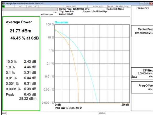
PTAR-ENDC_5A_n2-QPSK_5M_CH20425_826.5(25,0)
