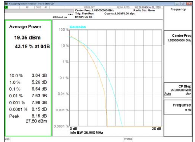
PTAR-ENDC_2A_n5-64QAM_15M_CH18900_1880(75,0)
