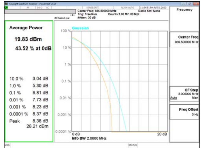
PTAR-ENDC_5A_n2-64QAM_1.4M_CH20525_836.5(6,0)
