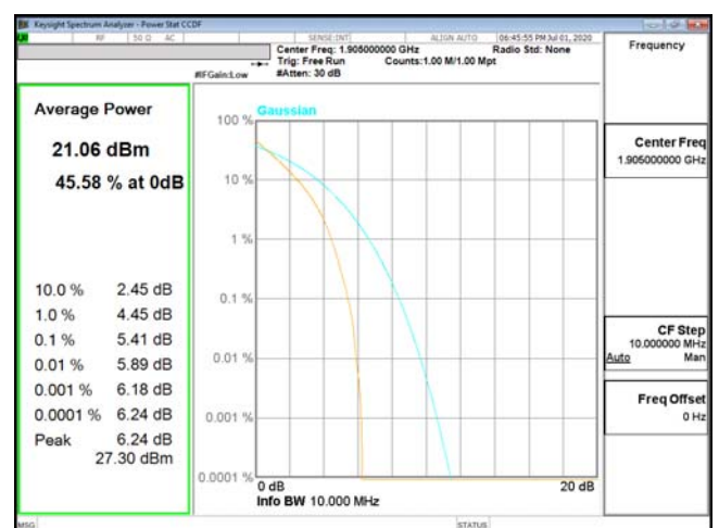
PTAR-ENDC_2A_n5-QPSK_10M_CH19150_1905(50,0)
