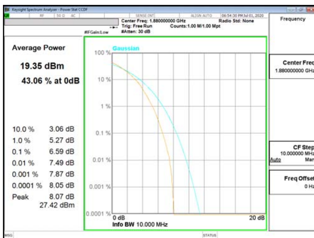
PTAR-ENDC_2A_n5-64QAM_10M_CH18900_1880(50,0)
