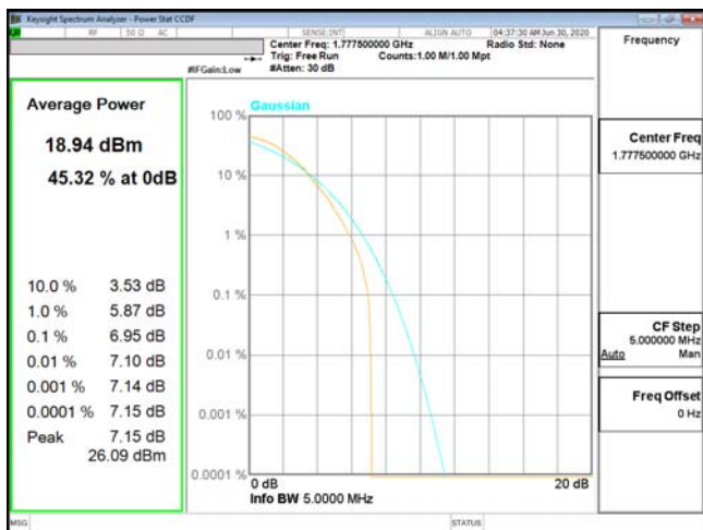
PTAR-ENDC_13A_n66-64QAM_5M_CH355500_1777.5(25,0)
