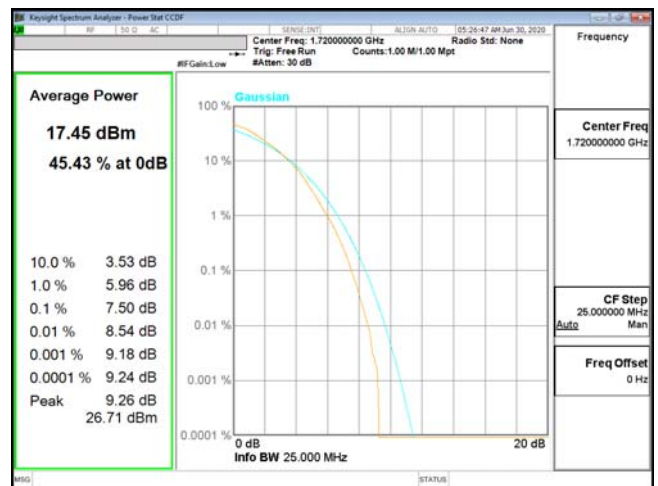
PTAR-ENDC_13A_n66-256QAM_20M_CH344000_1720(100,0)
