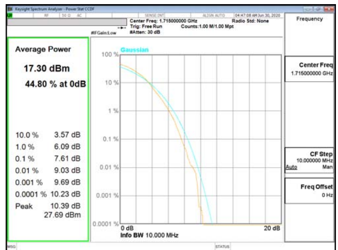
PTAR-ENDC_13A_n66-256QAM_10M_CH343000_1715(50,0)
