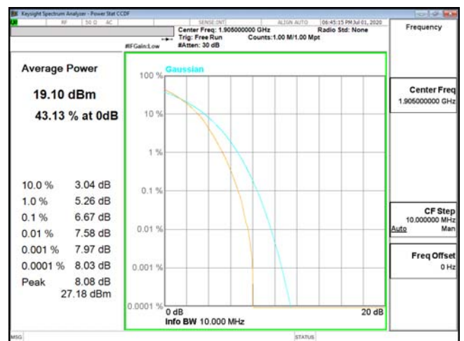
PTAR-ENDC_2A_n5-64QAM_10M_CH19150_1905(50,0)
