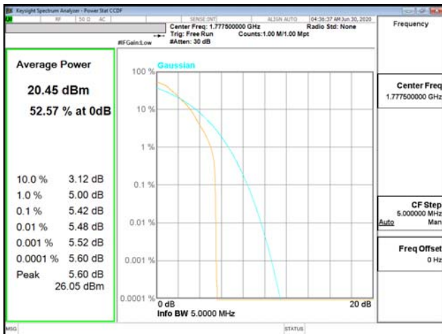
PTAR-ENDC_13A_n66-QPSK_5M_CH355500_1777.5(25,0)
