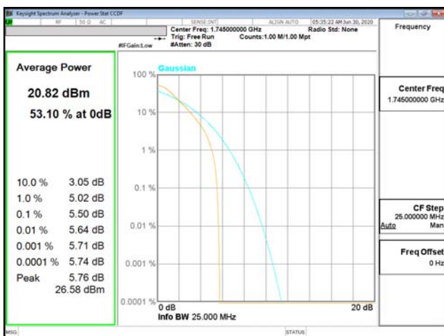
PTAR-ENDC_13A_n66-QPSK_20M_CH349000_1745(100,0)
