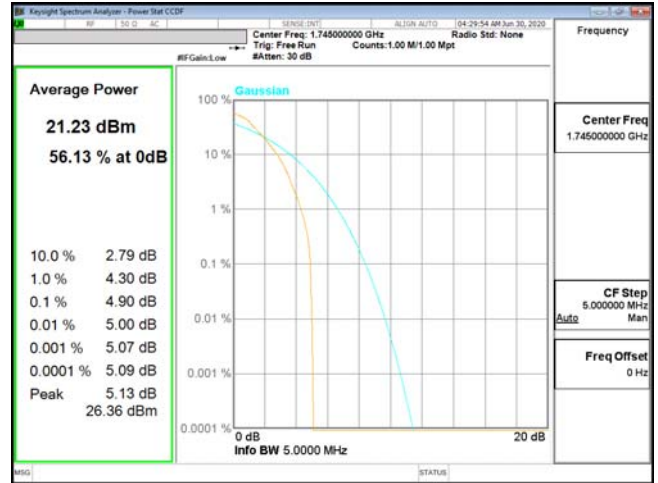
PTAR-ENDC_13A_n66-PI2-BPSK_5M_CH349000_1745(25,0)
