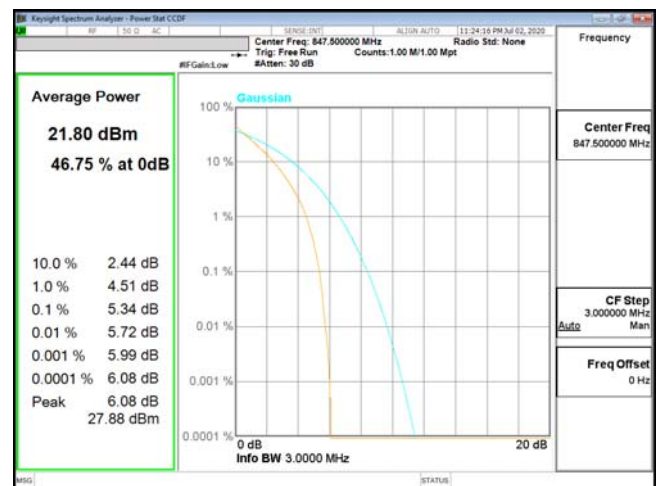
PTAR-ENDC_5A_n2-QPSK_3M_CH20635_847.5(15,0)
