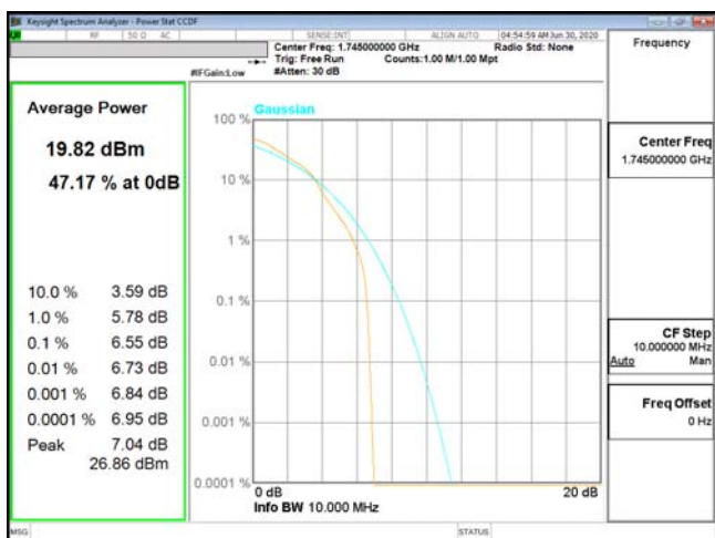
PTAR-ENDC_13A_n66-16QAM_10M_CH349000_1745(50,0)
