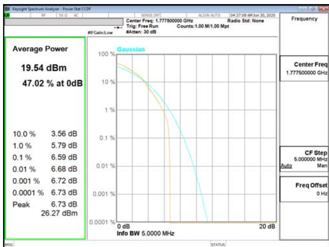
PTAR-ENDC_13A_n66-16QAM_5M_CH355500_1777.5(25,0)
