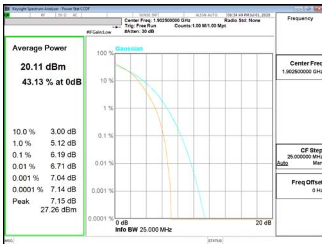
PTAR-ENDC_2A_n5-16QAM_15M_CH19125_1902.5(75,0)
