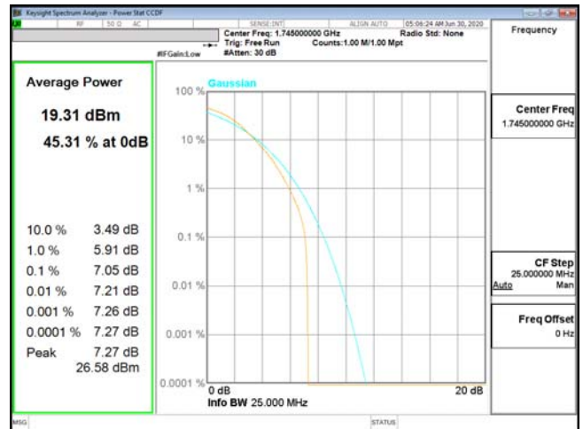
PTAR-ENDC_13A_n66-64QAM_15M_CH349000_1745(75,0)
