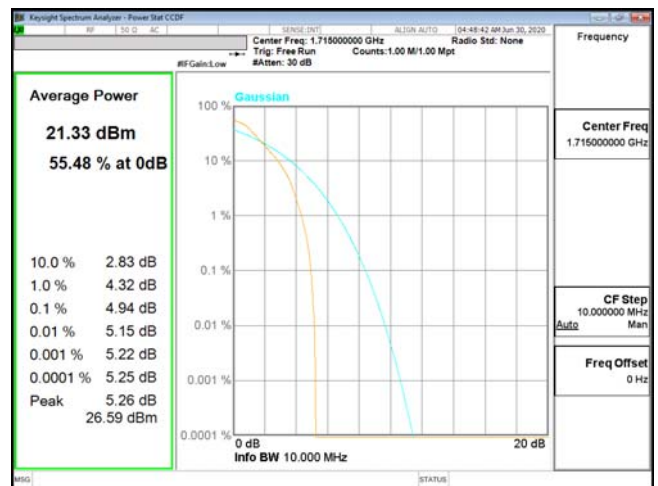
PTAR-ENDC_13A_n66-PI2-BPSK_10M_CH343000_1715(50,0)
