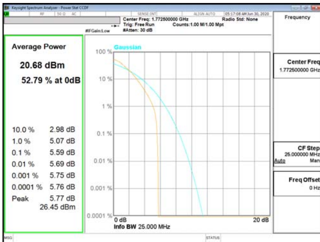
PTAR-ENDC_13A_n66-QPSK_15M_CH354500_1772.5(75,0)
