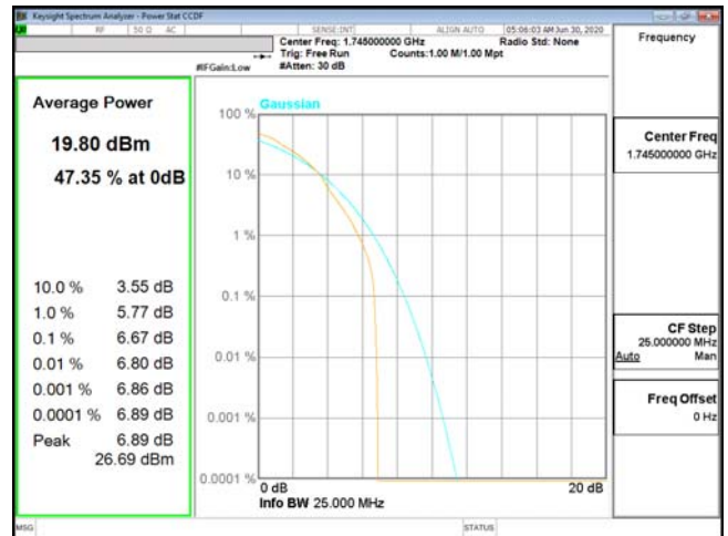
PTAR-ENDC_13A_n66-16QAM_15M_CH343500_1717.5(75,0) PTAR-ENDC_13A_n66-16QAM_15M_CH349000_1745(75,0)
