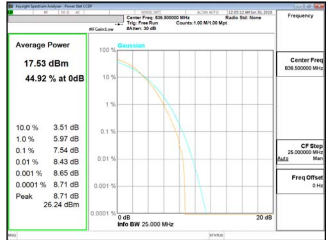
PTAR-ENDC_2A_n5-256QAM_15M_CH167300_836.5(75,0)
