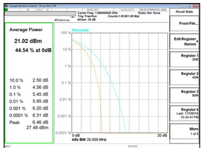
PTAR-ENDC_2A_n5-QPSK_20M_CH19100_1900(100,0)
