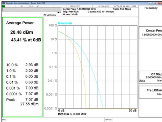
PTAR-ENDC_2A_n5-16QAM_5M_CH18625_1852.5(25,0)
