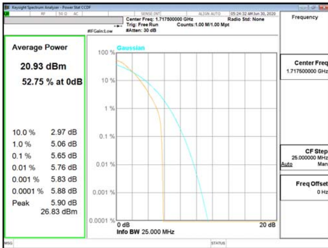
PTAR-ENDC_13A_n66-QPSK_15M_CH343500_1717.5(75,0)
