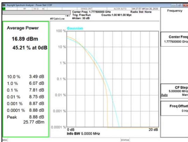
PTAR-ENDC_13A_n66-256QAM_5M_CH355500_1777.5(25,0)
