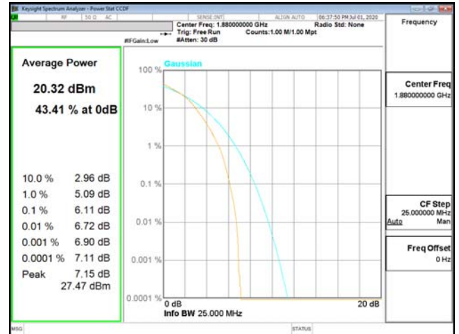
PTAR-ENDC_2A_n5-16QAM_15M_CH18900_1880(75,0)
