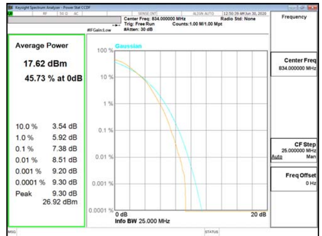
PTAR-ENDC_2A_n5-256QAM_20M_CH166800_834(100,0)
