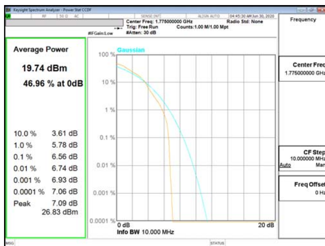
PTAR-ENDC_13A_n66-16QAM_10M_CH355000_1775(50,0)
