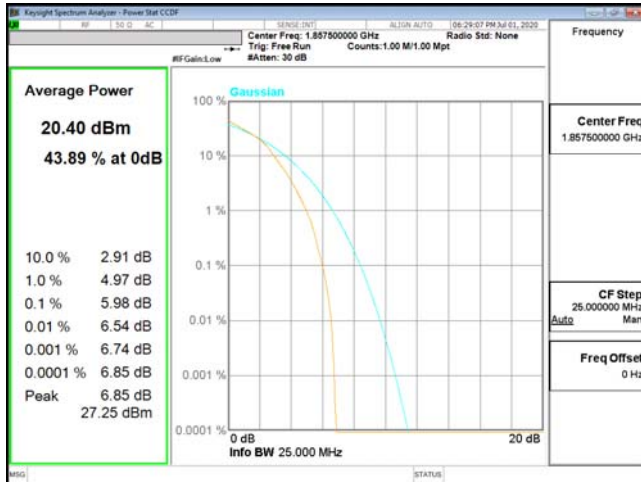
PTAR-ENDC_2A_n5-16QAM_15M_CH18675_1857.5(75,0)
