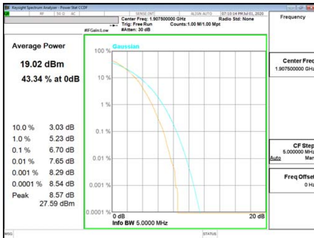
PTAR-ENDC_2A_n5-64QAM_5M_CH19175_1907.5(25,0)
