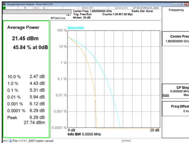
PTAR-ENDC_2A_n5-QPSK_5M_CH18625_1852.5(25,0)
