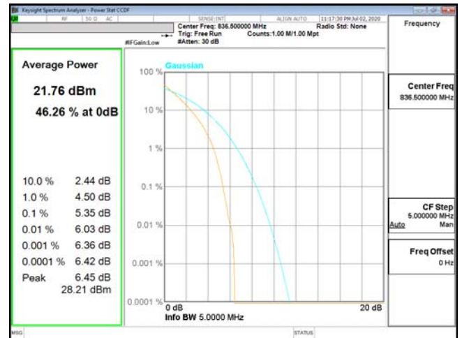
PTAR-ENDC_5A_n2-QPSK_5M_CH20525_836.5(25,0)
