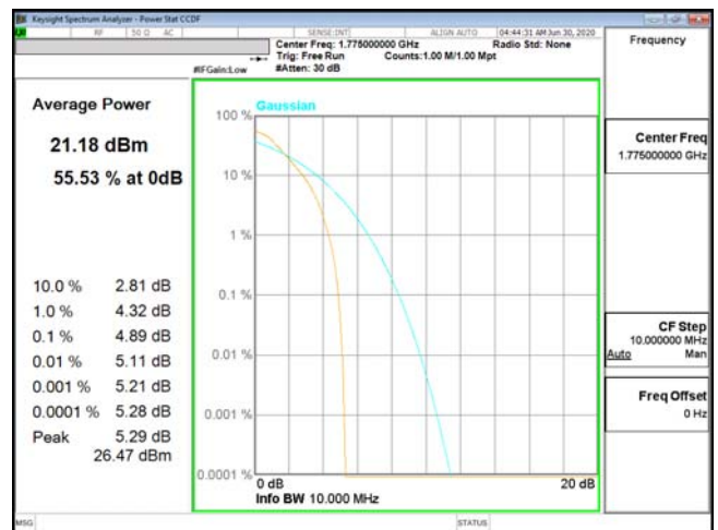
PTAR-ENDC_13A_n66-PI2-BPSK_10M_CH355000_1775(50,0)
