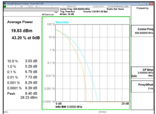
PTAR-ENDC_5A_n2-64QAM_3M_CH20415_825.5(15,0)
