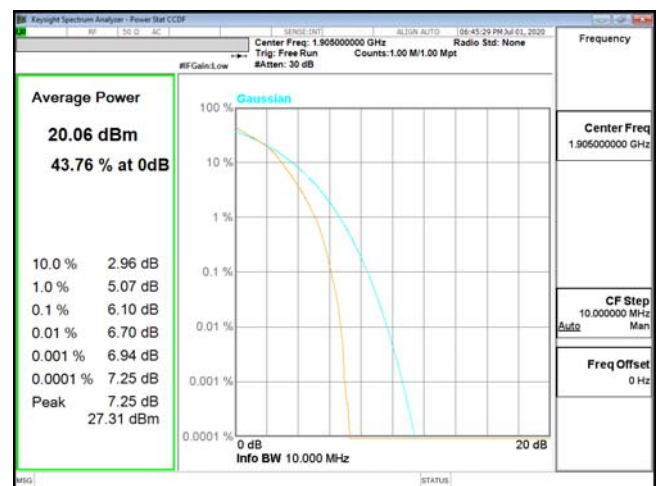
PTAR-ENDC_2A_n5-16QAM_10M_CH19150_1905(50,0)
