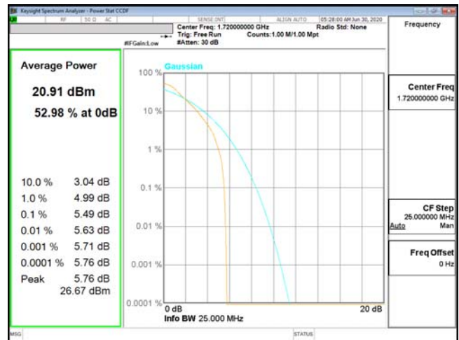
PTAR-ENDC_13A_n66-QPSK_20M_CH344000_1720(100,0)
