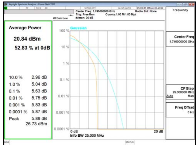
PTAR-ENDC_13A_n66-QPSK_15M_CH349000_1745(75,0)
