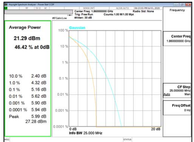
PTAR-ENDC_2A_n5-QPSK_20M_CH18700_1860(100,0)
