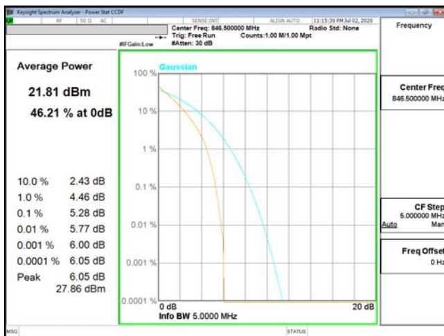
PTAR-ENDC_5A_n2-QPSK_5M_CH20625_846.5(25,0)
