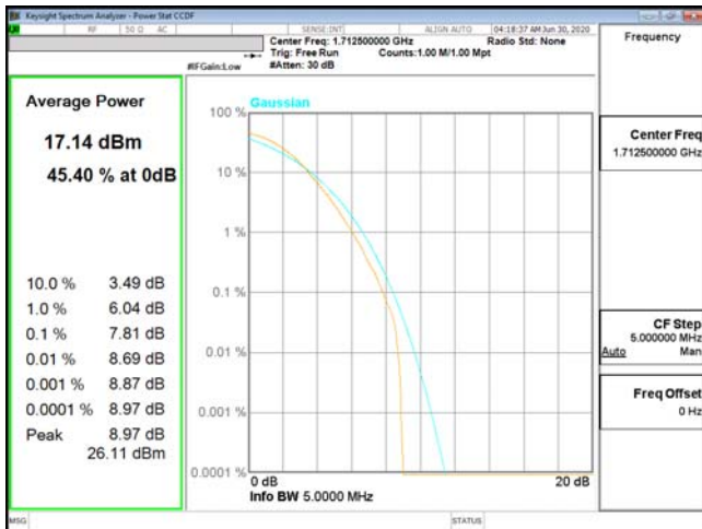
PTAR-ENDC_13A_n66-256QAM_5M_CH342500_1712.5(25,0)
