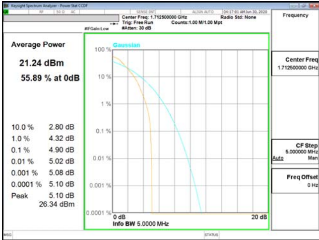
PTAR-ENDC_13A_n66-PI2-BPSK_5M_CH342500_1712.5(25,0)
