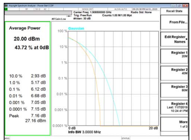
PTAR-ENDC_2A_n5-16QAM_3M_CH19185_1908.5(15,0)
