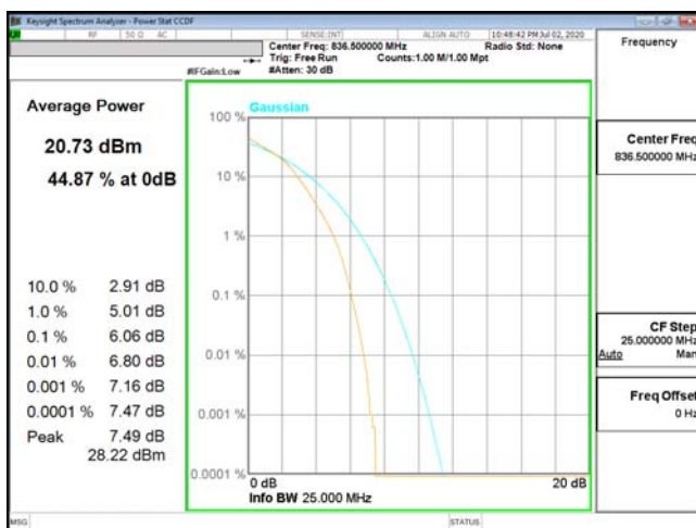
PTAR-ENDC_5A_n2-16QAM_10M_CH20525_836.5(50,0)
