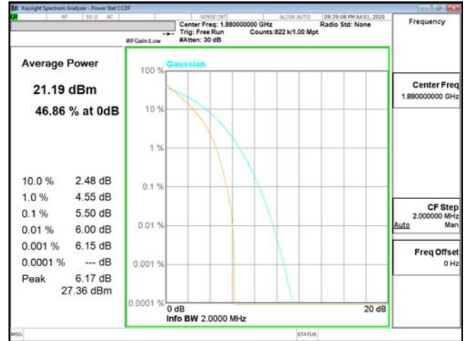
PTAR-ENDC_2A_n5-QPSK_1.4M_CH18900_1880(6,0)
