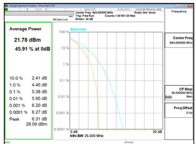
PTAR-ENDC_5A_n2-QPSK_10M_CH20600_844(50,0)
