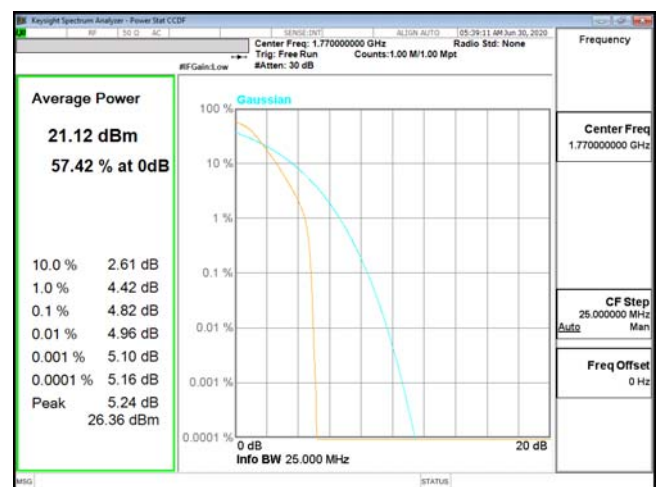
PTAR-ENDC_13A_n66-P12-BPSK_20M_CH354000_1770(100,0)
