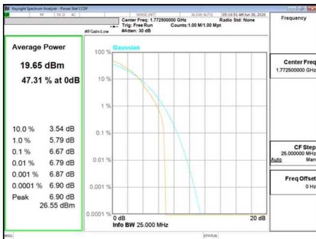
PTAR-ENDC_13A_n66-16QAM_15M_CH354500_1772.5(75,0) PTAR-ENDC_13A_n66-16QAM_20M_CH344000_1720(100,0)
