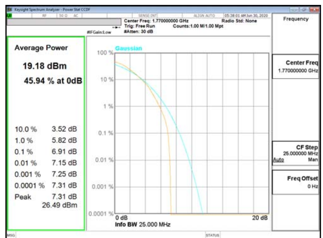
PTAR-ENDC_13A_n66-64QAM_20M_CH354000_1770(100,0)
