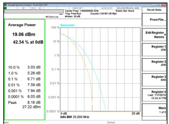
PTAR-ENDC_2A_n5-64QAM_20M_CH19100_1900(100,0)
