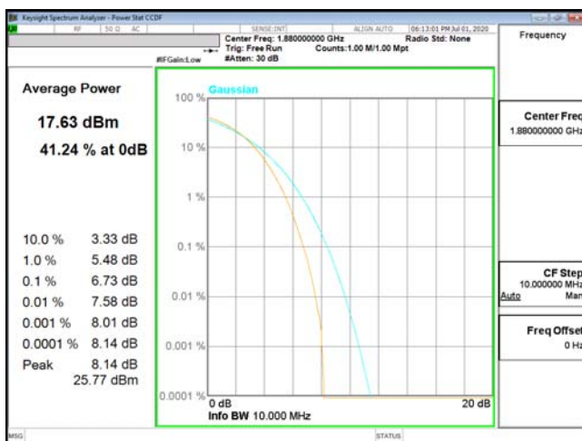
PTAR-ENDC_2A_n5-64QAM_20M_CH18900_1880(100,0)
