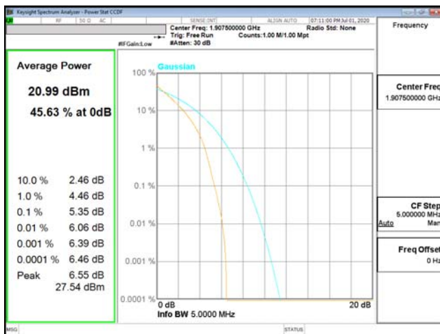
PTAR-ENDC_2A_n5-QPSK_5M_CH19175_1907.5(25,0)
