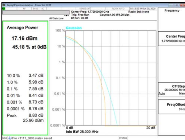
PTAR-ENDC_13A_n66-256QAM_15M_CH354500_1772.5(75,0)
