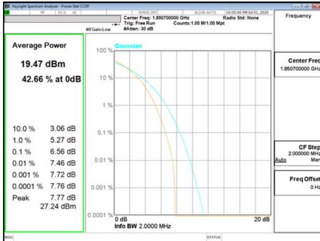
PTAR-ENDC_2A_n5-64QAM_1.4M_CH18607_18507(6,0)
