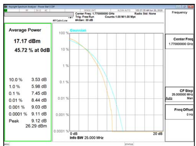
PTAR-ENDC_13A_n66-256QAM_20M_CH354000_1770(100,0)
