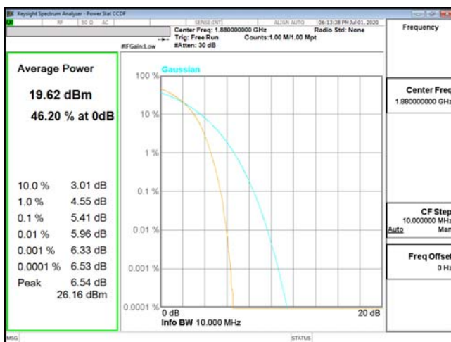
PTAR-ENDC_2A_n5-QPSK_20M_CH18900_1880(100,0)
