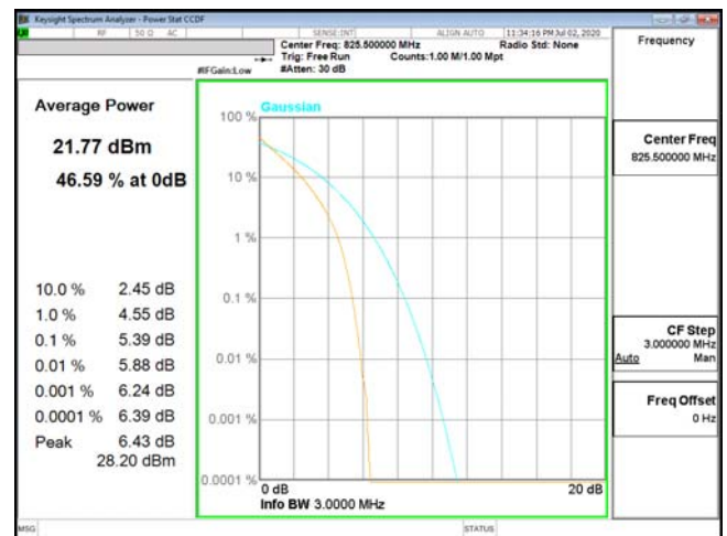
PTAR-ENDC_5A_n2-QPSK_3M_CH20415_825.5(15,0)
