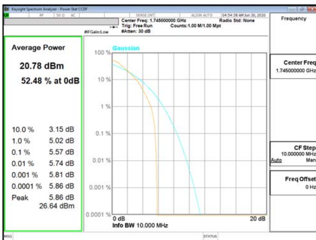
PTAR-ENDC_13A_n66-QPSK_10M_CH349000_1745(50,0)
