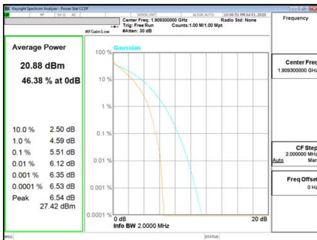
PTAR-ENDC_2A_n5-QPSK_1.4M_CH19193_1909.3(6,0)
