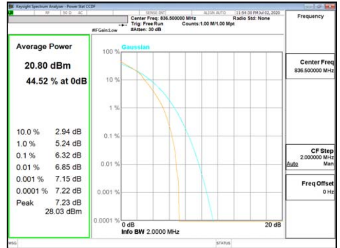
PTAR-ENDC_5A_n2-16QAM_1.4M_CH20525_836.5(6,0)
