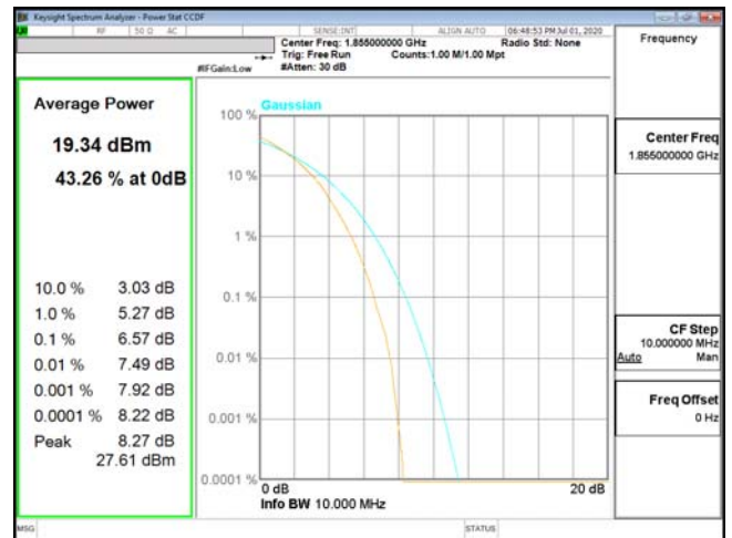
PTAR-ENDC_2A_n5-64QAM_10M_CH18650_1855(50,0)
