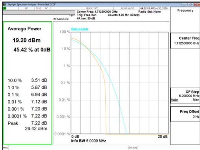
PTAR-ENDC_13A_n66-64QAM_5M_CH342500_1712.5(25,0)
