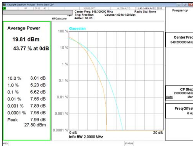
PTAR-ENDC_5A_n2-64QAM_1.4M_CH20643_848.3(6,0)
