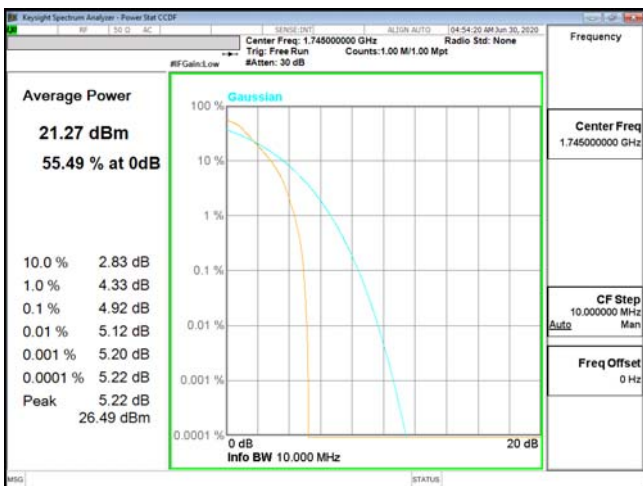
PTAR-ENDC_13A_n66-PI2-BPSK_10M_CH349000_1745(50,0)
