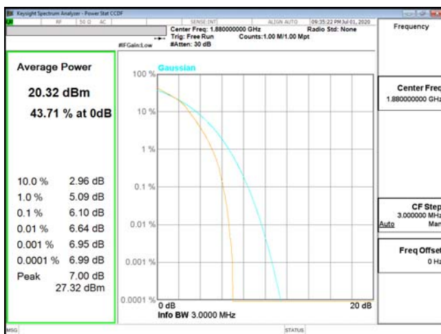
PTAR-ENDC_2A_n5-16QAM_3M_CH18900_1880(15,0)
