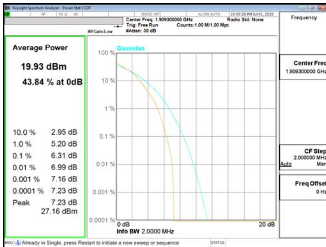
PTAR-ENDC_2A_n5-16QAM_1.4M_CH19193_1909.3(6,0)
