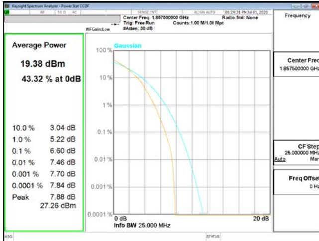
PTAR-ENDC_2A_n5-64QAM_15M_CH18675_1857.5(75,0)
