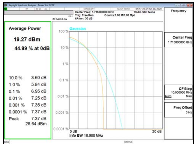
PTAR-ENDC_13A_n66-64QAM_10M_CH343000_1715(50,0)
