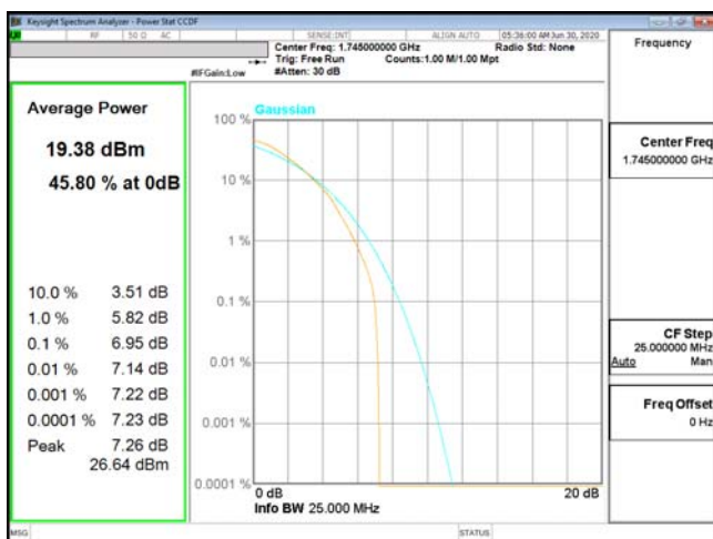
PTAR-ENDC_13A_n66-64QAM_20M_CH349000_1745(100,0)
