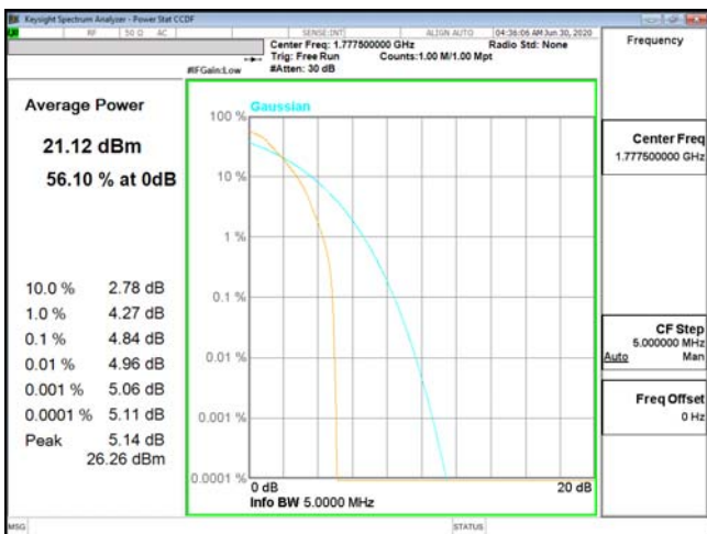
PTAR-ENDC_13A_n66-PI2-BPSK_5M_CH355500_1777.5(25,0)
