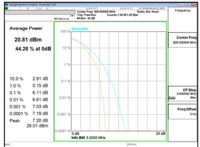
PTAR-ENDC_5A_n2-16QAM_3M_CH20415_825.5(15,0)
