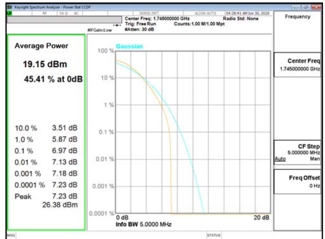
PTAR-ENDC_13A_n66-64QAM_5M_CH349000_1745(25,0)
