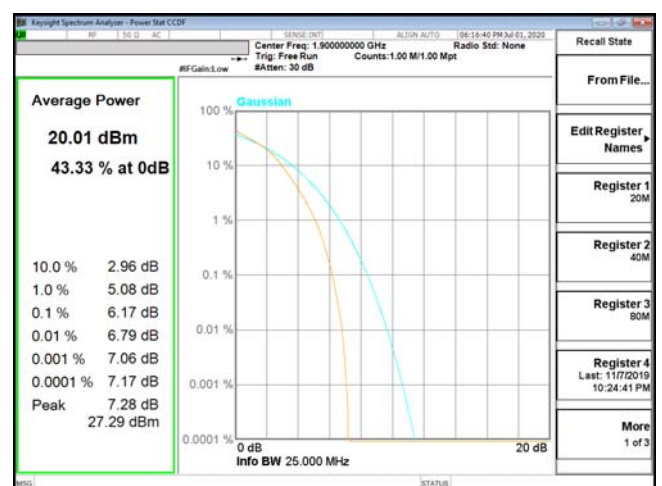
PTAR-ENDC_2A_n5-16QAM_20M_CH19100_1900(100,0)
