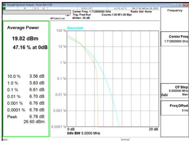
PTAR-ENDC_13A_n66-16QAM_5M_CH342500_1712.5(25,0)
