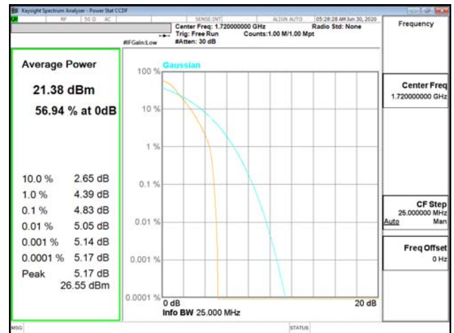
PTAR-ENDC_13A_n66-P12-BPSK_20M_CH344000_1720(100,0)
