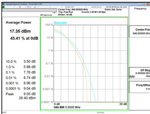
PTAR-ENDC_2A_n5-256QAM_5M_CH169300_846.5(25,0)
