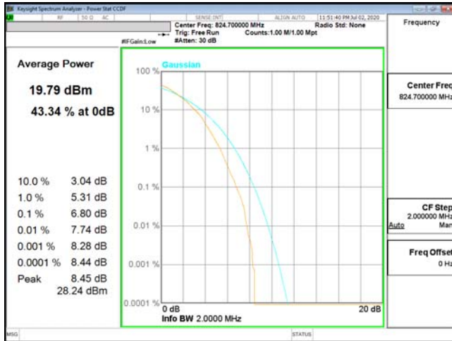
PTAR-ENDC_5A_n2-64QAM_1.4M_CH20407_824.7(6,0)
