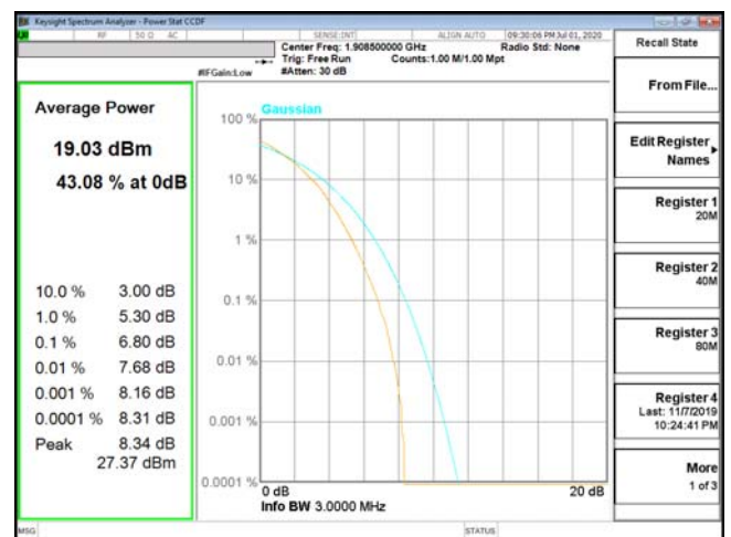
PTAR-ENDC_2A_n5-64QAM_3M_CH19185_1908.5(15,0)
