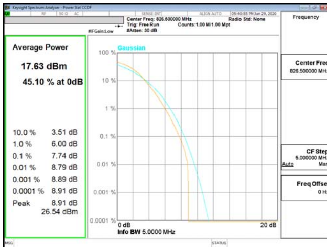
PTAR-ENDC_2A_n5-256QAM_5M_CH165300_826.5(25,0)
