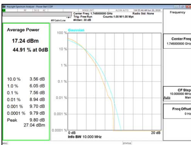
PTAR-ENDC_13A_n66-256QAM_10M_CH349000_1745(50,0)
