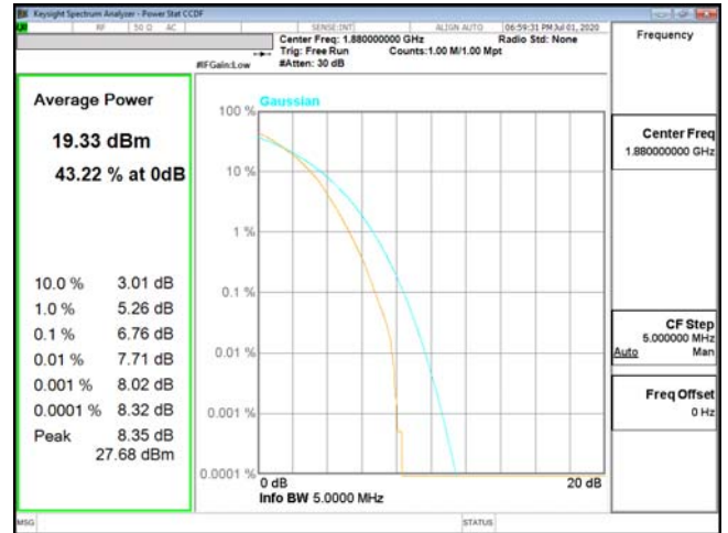
PTAR-ENDC_2A_n5-64QAM_5M_CH18900_1880(25,0)
