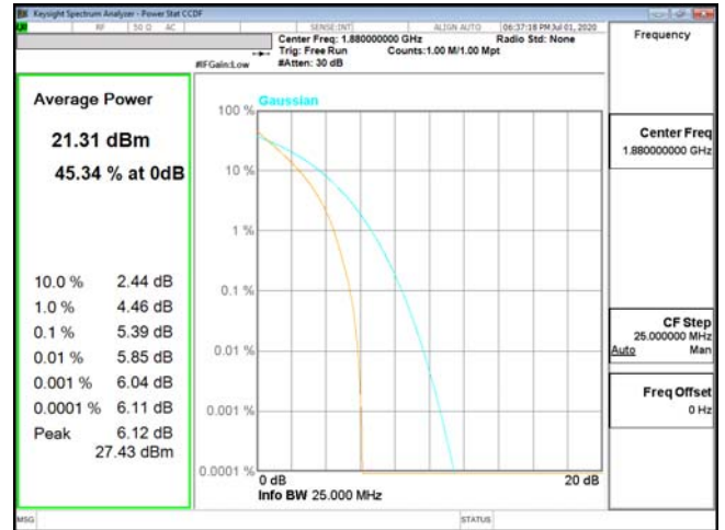
PTAR-ENDC_2A_n5-QPSK_15M_CH18900_1880(75,0)
