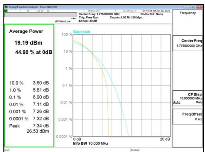
PTAR-ENDC_13A_n66-64QAM_10M_CH355000_1775(50,0)
