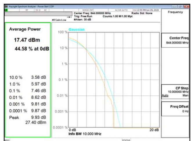
PTAR-ENDC_2A_n5-256QAM_10M_CH168800_844(50,0)
