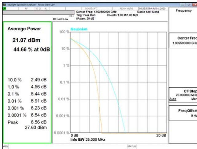
PTAR-ENDC_2A_n5-QPSK_15M_CH19125_1902.5(75,0)
