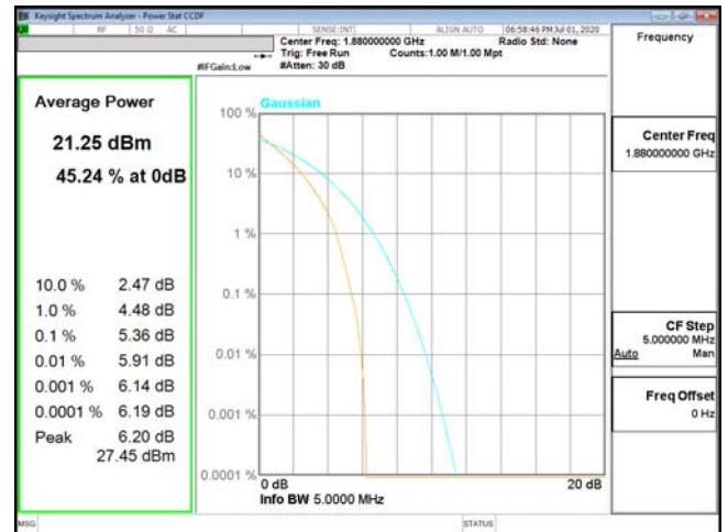
PTAR-ENDC_2A_n5-QPSK_5M_CH18900_1880(25,0)
