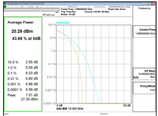
PTAR-ENDC_2A_n5-16QAM_10M_CH18650_1855(50,0)
