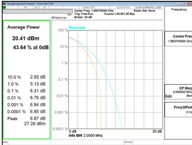
PTAR-ENDC_2A_n5-16QAM_1.4M_CH18607_18507(6,0)
