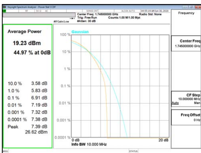
PTAR-ENDC_13A_n66-64QAM_10M_CH349000_1745(50,0)
