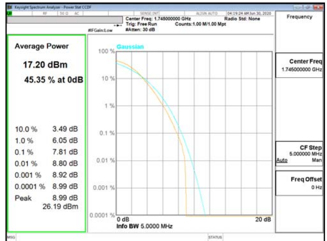
PTAR-ENDC_13A_n66-256QAM_5M_CH349000_1745(25,0)
