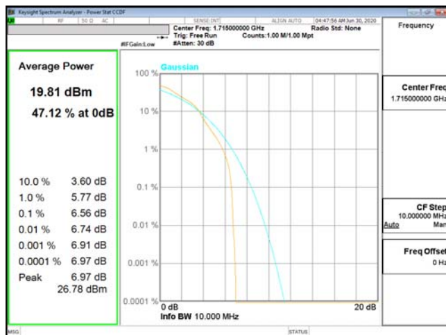
PTAR-ENDC_13A_n66-16QAM_10M_CH343000_1715(50,0)
