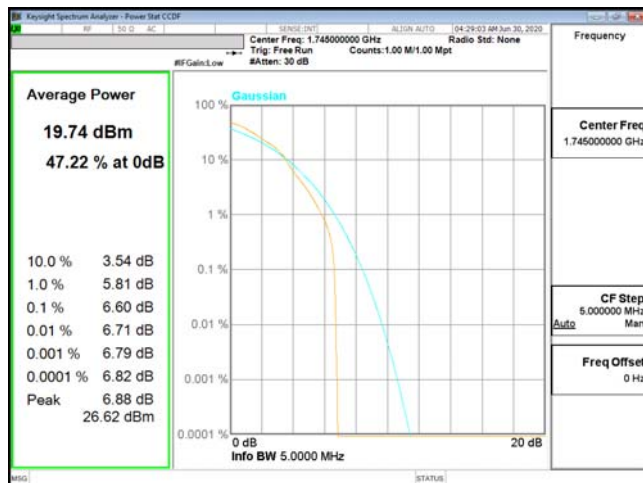
PTAR-ENDC_13A_n66-16QAM_5M_CH349000_1745(25,0)
