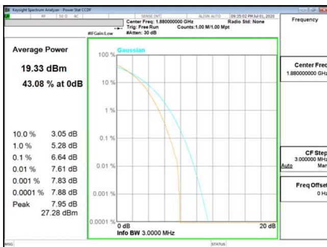
PTAR-ENDC_2A_n5-64QAM_3M_CH18900_1880(15,0)
