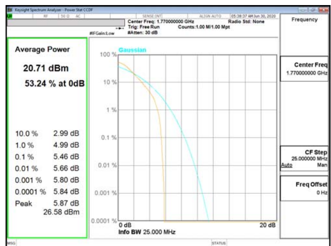
PTAR-ENDC_13A_n66-QPSK_20M_CH354000_1770(100,0)
