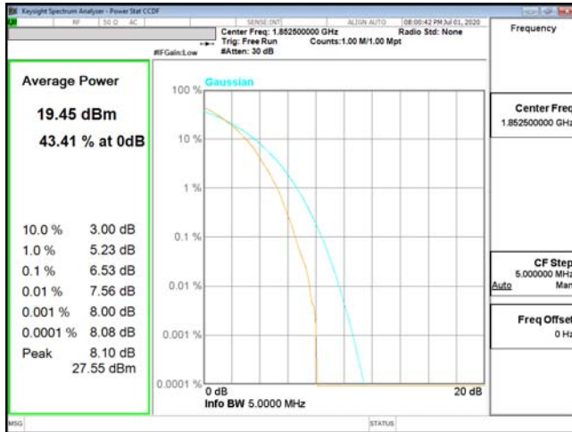
PTAR-ENDC_2A_n5-64QAM_5M_CH18625_1852.5(25,0)
