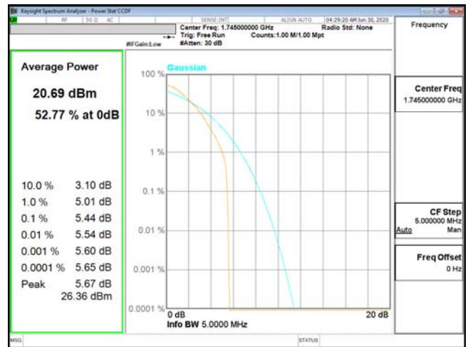
PTAR-ENDC_13A_n66-QPSK_5M_CH349000_1745(25,0)
