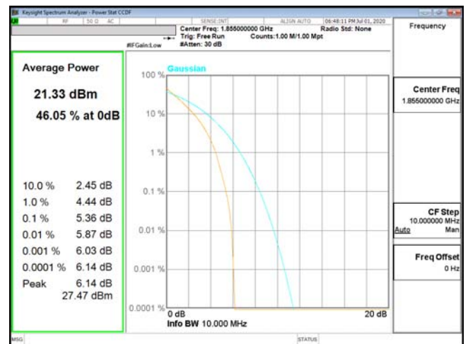
PTAR-ENDC_2A_n5-QPSK_10M_CH18650_1855(50,0)
