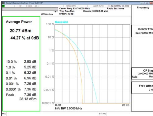
PTAR-ENDC_5A_n2-16QAM_1.4M_CH20407_824.7(6,0)
