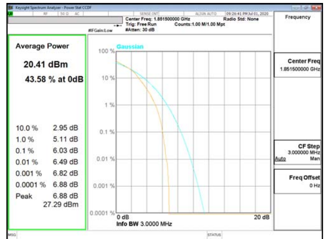
PTAR-ENDC_2A_n5-16QAM_3M_CH18615_1851.5(15,0)
