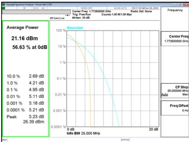
PTAR-ENDC_13A_n66-P12-BPSK_15M_CH354500_1772.5(75,0)
