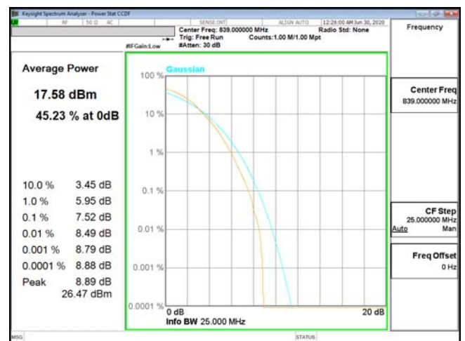
PTAR-ENDC_2A_n5-256QAM_20M_CH167800_839(100,0)
