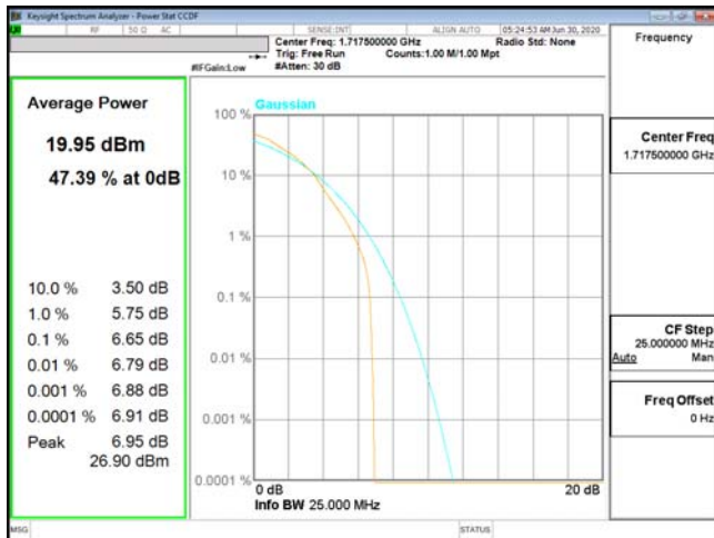
PTAR-ENDC_13A_n66-16QAM_15M_CH343500_1717.5(75,0) PTAR-ENDC_13A_n66-16QAM_15M_CH349000_1745(75,0)
