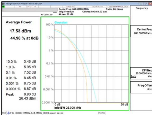
PTAR-ENDC_2A_n5-256QAM_15M_CH168300_841.5(75,0)
