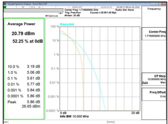
PTAR-ENDC_13A_n66-QPSK_10M_CH343000_1715(50,0)
