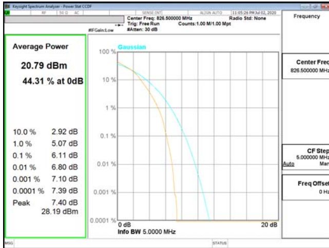
PTAR-ENDC_5A_n2-16QAM_5M_CH20425_826.5(25,0)
