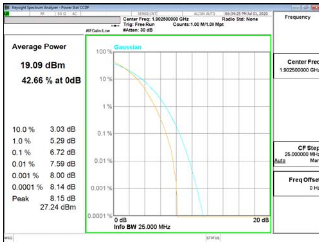
PTAR-ENDC_2A_n5-64QAM_15M_CH19125_1902.5(75,0)
