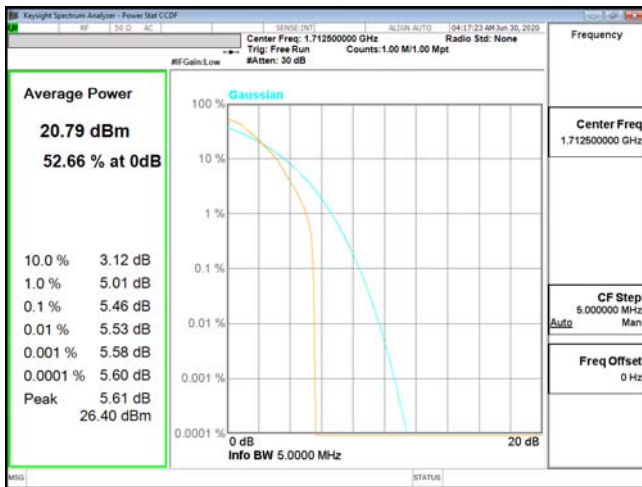
PTAR-ENDC_13A_n66-QPSK_5M_CH342500_1712.5(25,0)
