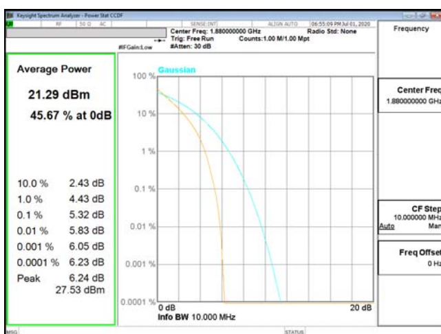
PTAR-ENDC_2A_n5-QPSK_10M_CH18900_1880(50,0)
