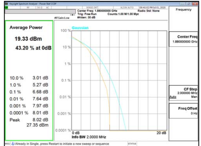
PTAR-ENDC_2A_n5-64QAM_1.4M_CH18900_1880(6,0)
