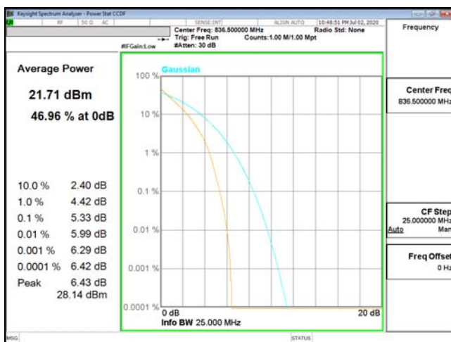
PTAR-ENDC_5A_n2-QPSK_10M_CH20525_836.5(50,0)
