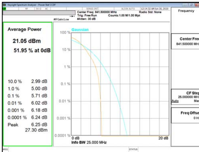
PTAR-ENDC_2A_n5-QPSK_15M_CH168300_841.5(75,0)
