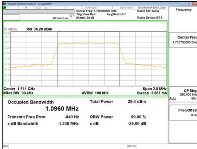
OCC-ENDC_66A_n5-16QAM_1.4M_CH131979_1710.7(6,0)
