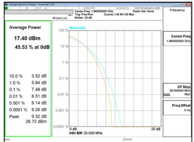
PTAR-ENDC_5A_n2-256QAM_20M_CH372000_1860(100,0)
