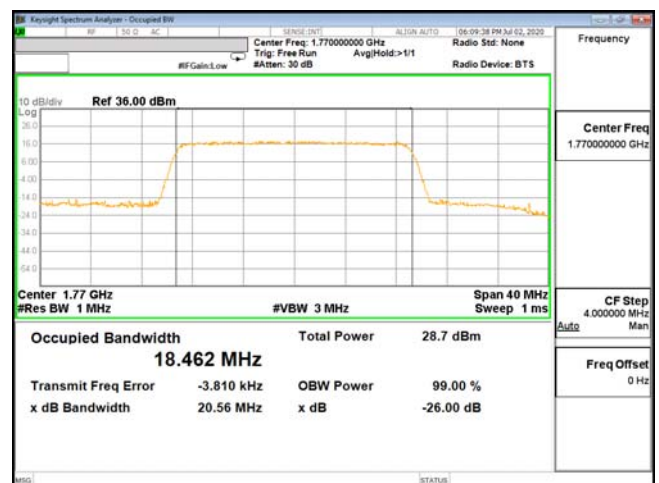
OCC-ENDC_66A_n5-QPSK_20M_CH132572_1770(100,0)
