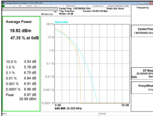
PTAR-ENDC_5A_n2-16QAM_15M_CH371500_1857.5(75,0)
