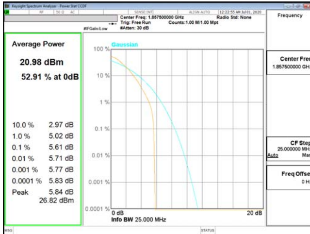
PTAR-ENDC_5A_n2-QPSK_15M_CH371500_1857.5(75,0)
