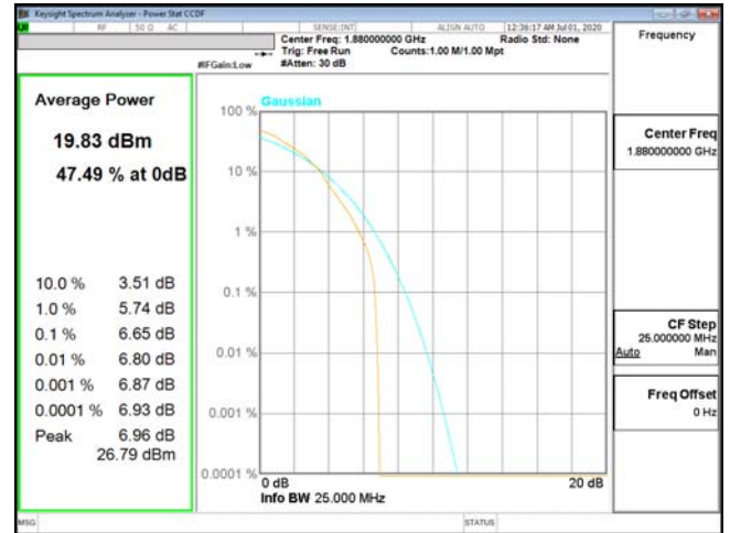
PTAR-ENDC_5A_n2-16QAM_15M_CH376000_1880(75,0)
