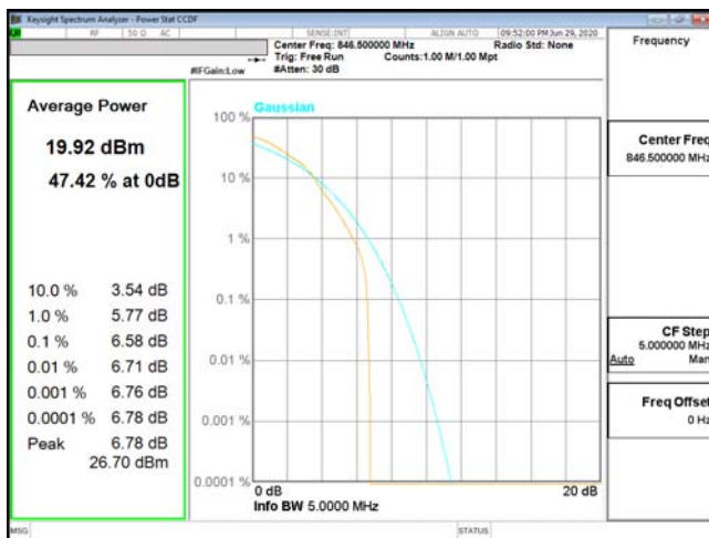
PTAR-ENDC_2A_n5-16QAM_5M_CH169300_846.5(25,0)
