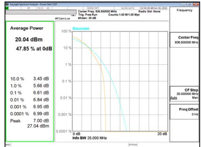
PTAR-ENDC_2A_n5-16QAM_15M_CH167300_836.5(75,0)
