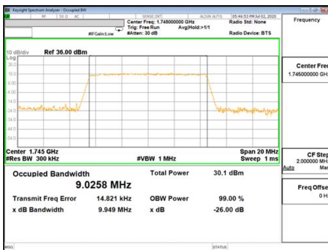
OCC-ENDC_66A_n5-QPSK_10M_CH132322_1745(50,0)
