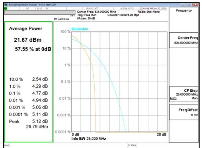
PTAR-ENDC_2A_n5-PI2-BPSK_20M_CH166800_834(100,0)
