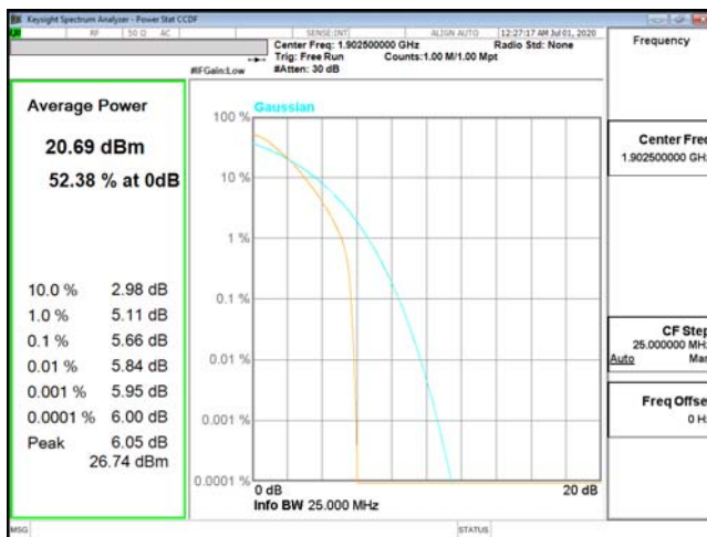
PTAR-ENDC_5A_n2-QPSK_15M_CH380500_1902.5(75,0)
