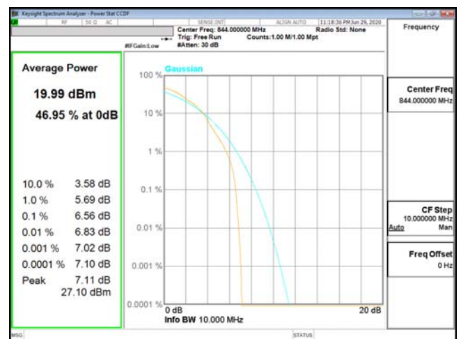
PTAR-ENDC_2A_n5-16QAM_10M_CH168800_844(50,0)
