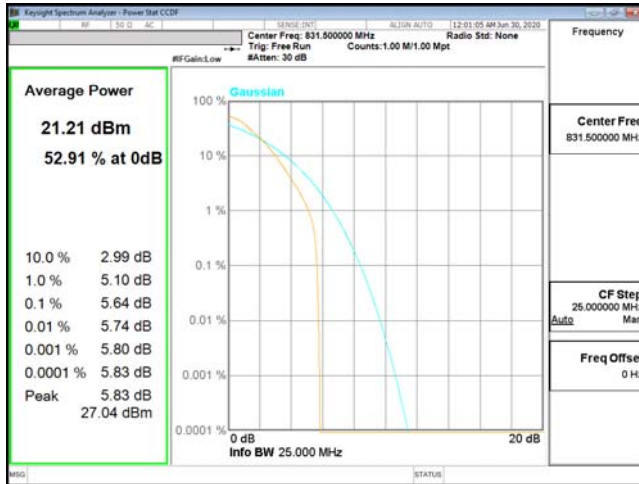
PTAR-ENDC_2A_n5-QPSK_15M_CH166300_831.5(75,0)
