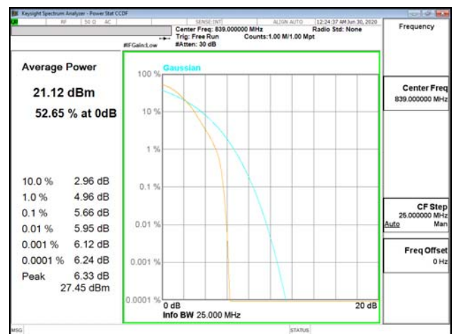
PTAR-ENDC_2A_n5-QPSK_20M_CH167800_839(100,0)
