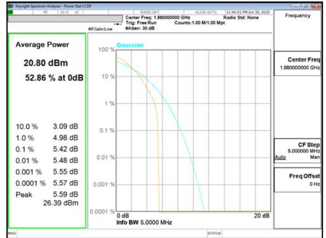
PTAR-ENDC_5A_n2-QPSK_5M_CH376000_1880(25,0)
