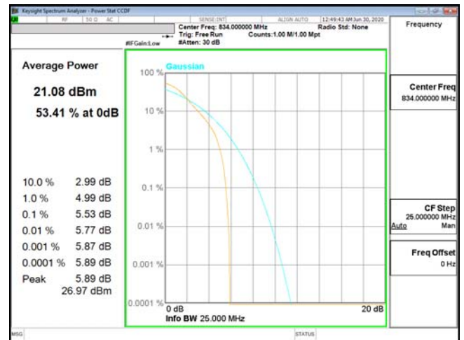
PTAR-ENDC_2A_n5-QPSK_20M_CH166800_834(100,0)
