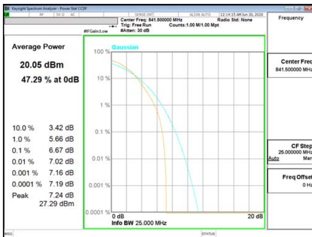
PTAR-ENDC_2A_n5-16QAM_15M_CH168300_841.5(75,0)
