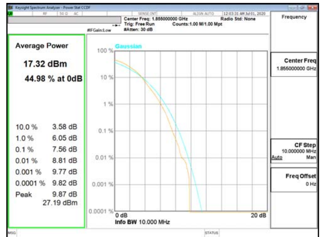
PTAR-ENDC_5A_n2-256QAM_10M_CH371000_1855(50,0)
