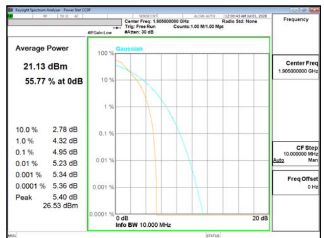
PTAR-ENDC_5A_n2-PI2-BPSK_10M_CH381000_1905(50,0)
