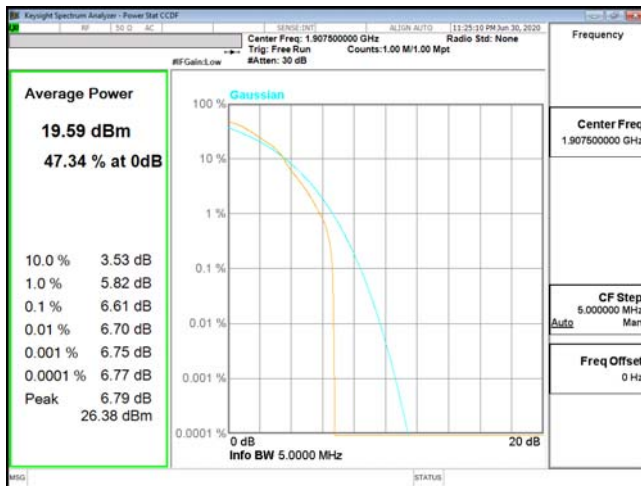
PTAR-ENDC_5A_n2-16QAM_5M_CH381500_1907.5(25,0)
