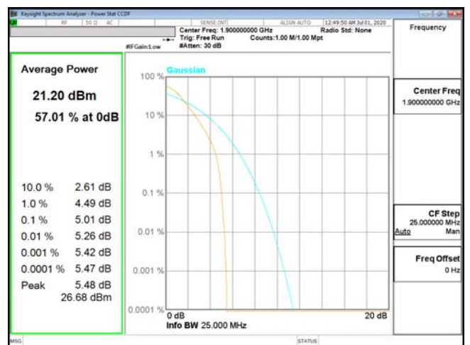
PTAR-ENDC_5A_n2-PI2-BPSK_20M_CH380000_1900(100,0)
