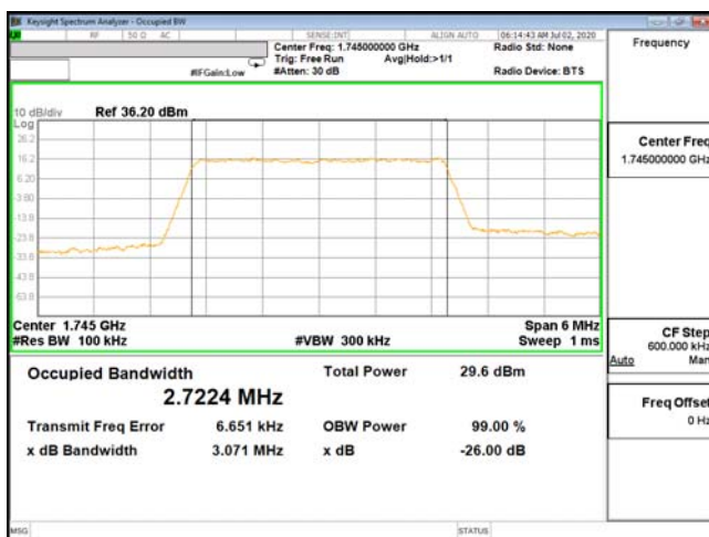
OCC-ENDC_66A_n5-16QAM_3M_CH132322_1745(15,0)
