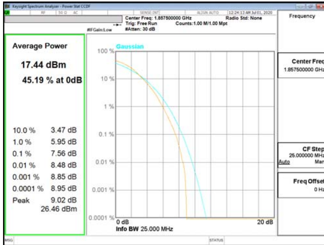
PTAR-ENDC_5A_n2-256QAM_15M_CH371500_1857.5(75,0)
