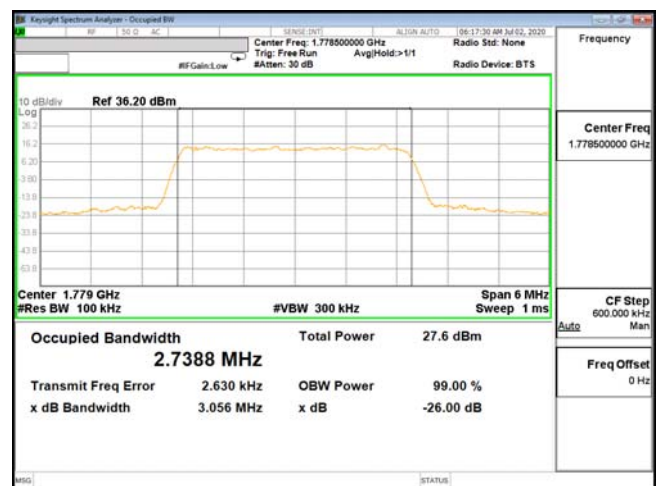
OCC-ENDC_66A_n5-64QAM_3M_CH132657_1778.5(15,0)
