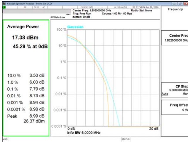
PTAR-ENDC_5A_n2-256QAM_5M_CH370500_1852.5(25,0)
