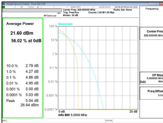
PTAR-ENDC_2A_n5-PI2-BPSK_5M_CH165300_826.5(25,0)
