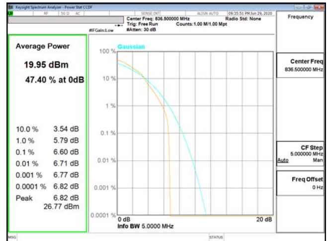
PTAR-ENDC_2A_n5-16QAM_5M_CH167300_836.5(25,0)
