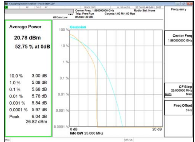
PTAR-ENDC_5A_n2-QPSK_15M_CH376000_1880(75,0)
