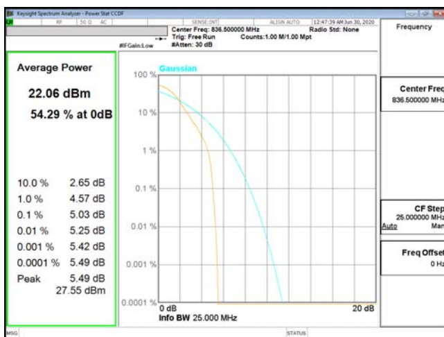
PTAR-ENDC_2A_n5-PI2-BPSK_20M_CH167300_836.5(100,0)
