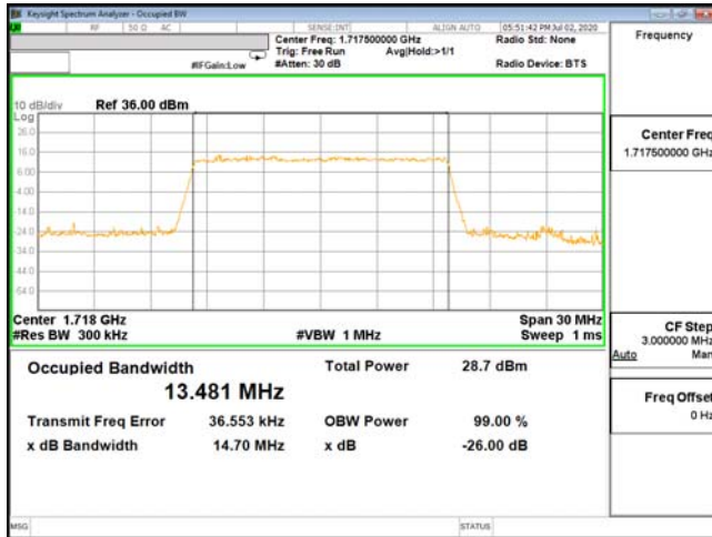
OCC-ENDC_66A_n5-64QAM_15M_CH132047_1717.5(75,0)
