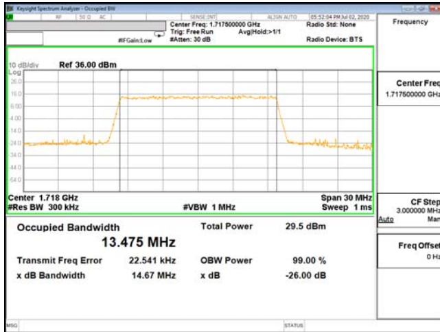
OCC-ENDC_66A_n5-16QAM_15M_CH132047_1717.5(75,0)
