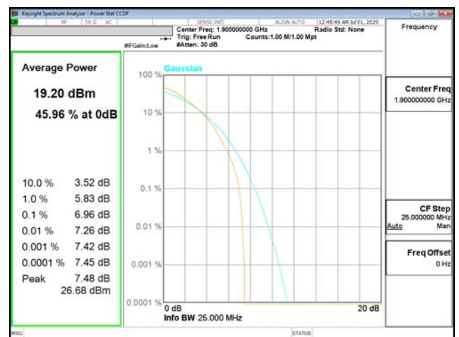
PTAR-ENDC_5A_n2-64QAM_20M_CH380000_1900(100,0)
