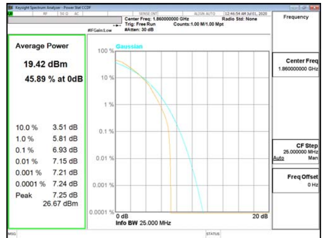
PTAR-ENDC_5A_n2-64QAM_20M_CH372000_1860(100,0)
