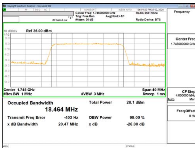
OCC-ENDC_66A_n5-16QAM_20M_CH132322_1745(100,0)
