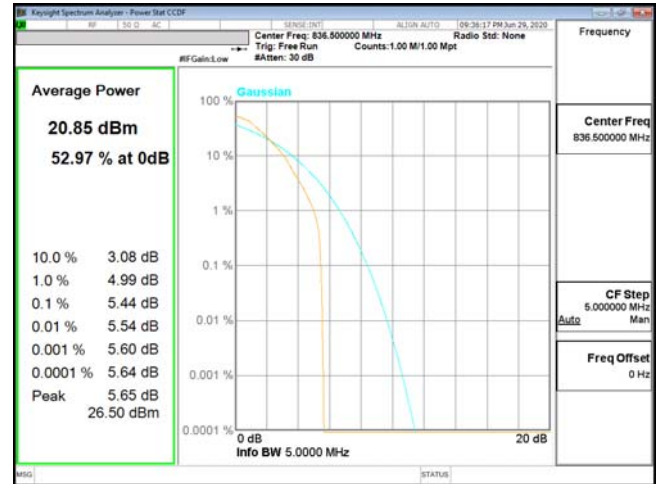
PTAR-ENDC_2A_n5-QPSK_5M_CH167300_836.5(25,0)
