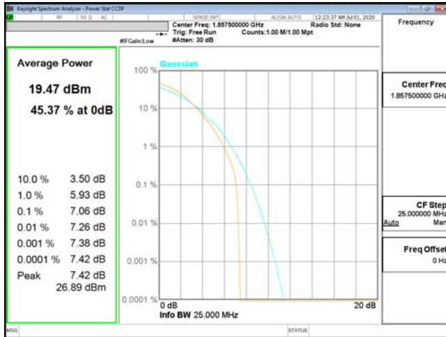
PTAR-ENDC_5A_n2-64QAM_15M_CH371500_1857.5(75,0)
