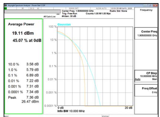
PTAR-ENDC_5A_n2-64QAM_10M_CH381000_1905(50,0)
