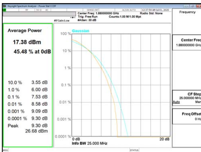
PTAR-ENDC_5A_n2-256QAM_20M_CH376000_1880(100,0)
