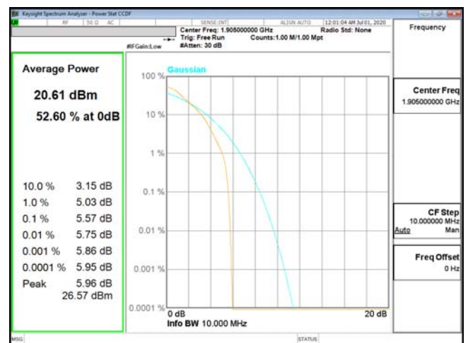
PTAR-ENDC_5A_n2-QPSK_10M_CH381000_1905(50,0)
