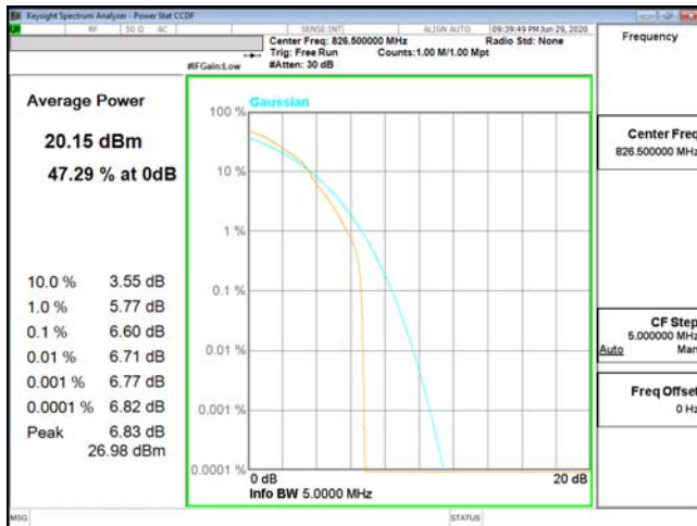
PTAR-ENDC_2A_n5-16QAM_5M_CH165300_826.5(25,0)
