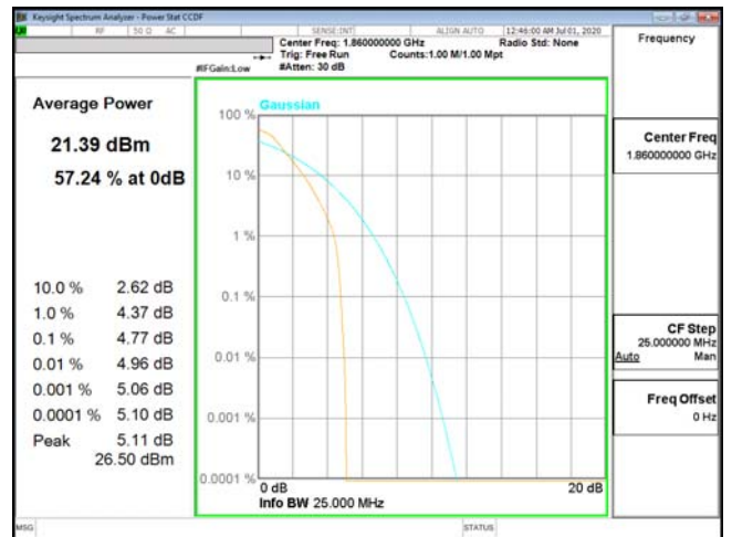
PTAR-ENDC_5A_n2-PI2-BPSK_20M_CH372000_1860(100,0)
