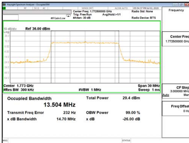
OCC-ENDC_66A_n5-16QAM_15M_CH132597_1772.5(75,0)
