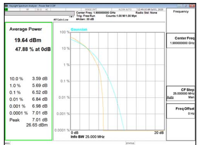
PTAR-ENDC_5A_n2-16QAM_20M_CH380000_1900(100,0)
