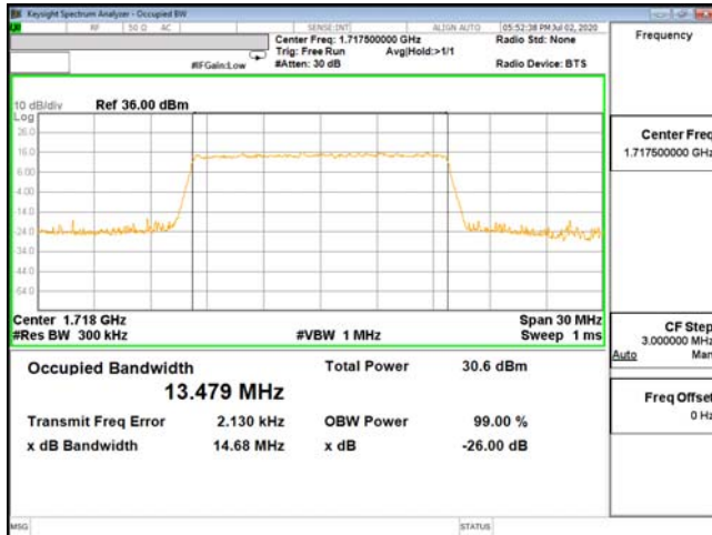
OCC-ENDC_66A_n5-QPSK_15M_CH132047_1717.5(75,0)
