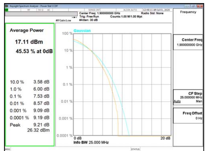
PTAR-ENDC_5A_n2-256QAM_20M_CH380000_1900(100,0)
