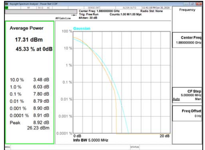
PTAR-ENDC_5A_n2-256QAM_5M_CH376000_1880(25,0)
