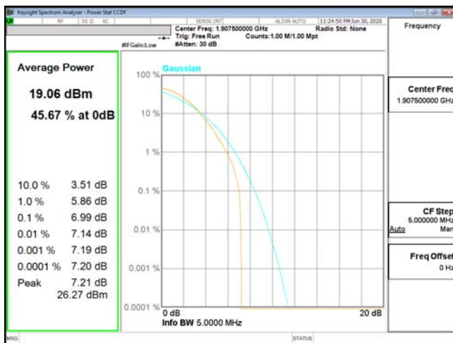
PTAR-ENDC_5A_n2-64QAM_5M_CH381500_1907.5(25,0)
