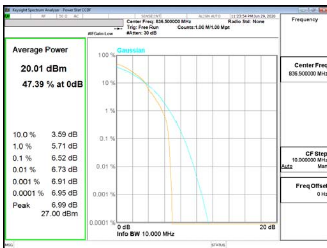
PTAR-ENDC_2A_n5-16QAM_10M_CH167300_836.5(50,0)
