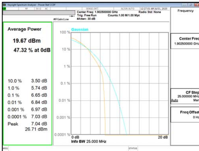
PTAR-ENDC_5A_n2-16QAM_15M_CH380500_1902.5(75,0)
