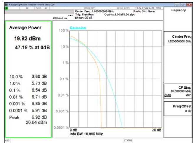
PTAR-ENDC_5A_n2-16QAM_10M_CH371000_1855(50,0)
