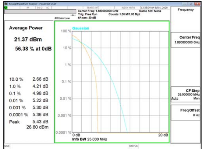
PTAR-ENDC_5A_n2-PI2-BPSK_15M_CH376000_1880(75,0)
