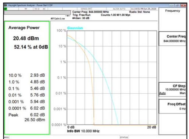
PTAR-ENDC_2A_n5-PI2-BPSK_10M_CH168800_844(50,0)
