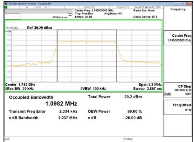
OCC-ENDC_66A_n5-16QAM_1.4M_CH132322_1745(6,0)
