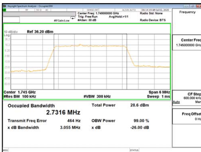
OCC-ENDC_66A_n5-64QAM_3M_CH132322_1745(15,0)
