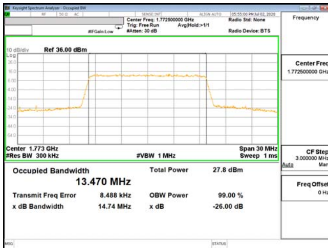
OCC-ENDC_66A_n5-64QAM_15M_CH132597_1772.5(75,0)
