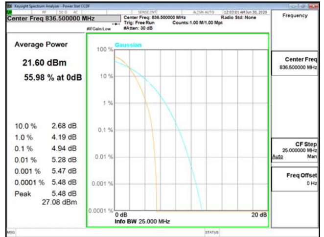
PTAR-ENDC_2A_n5-PI2-BPSK_15M_CH167300_836.5(75,0)
