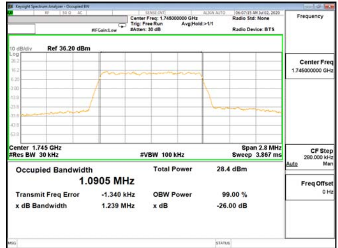
OCC-ENDC_66A_n5-64QAM_1.4M_CH132322_1745(6,0)
