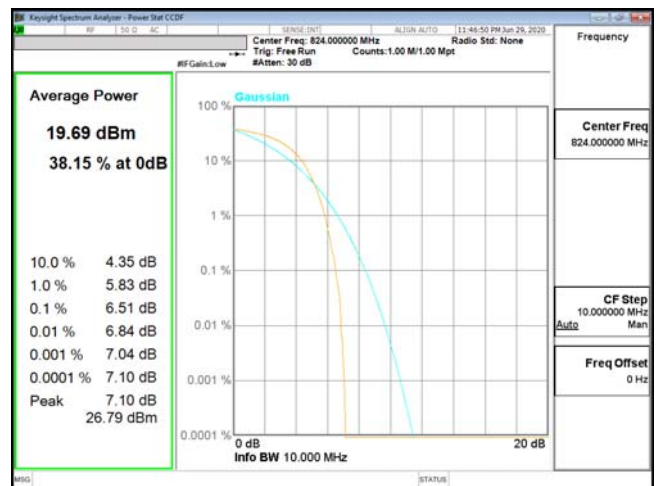
PTAR-ENDC_2A_n5-PI2-BPSK_10M_CH165800_824(50,0)
