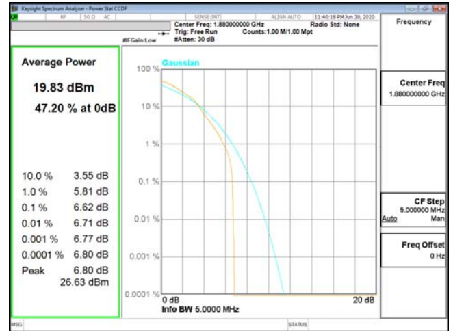
PTAR-ENDC_5A_n2-16QAM_5M_CH376000_1880(25,0)
