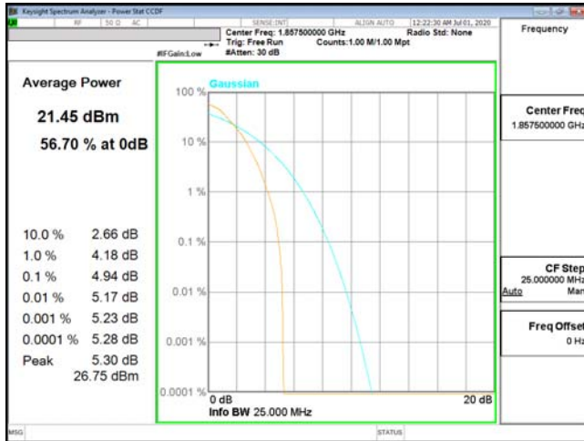
PTAR-ENDC_5A_n2-PI2-BPSK_15M_CH371500_1857.5(75,0)
