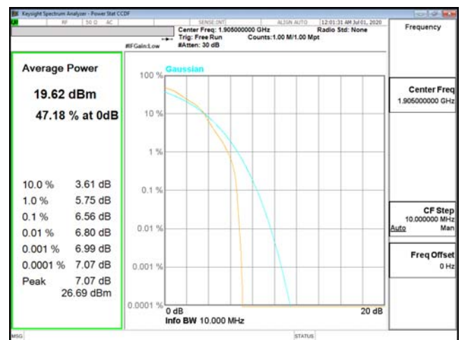
PTAR-ENDC_5A_n2-16QAM_10M_CH381000_1905(50,0)
