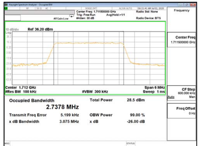
OCC-ENDC_66A_n5-64QAM_3M_CH131987_1711.5(15,0)
