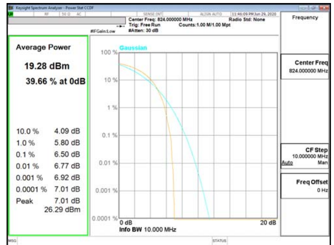
PTAR-ENDC_2A_n5-QPSK_10M_CH165800_824(50,0)
