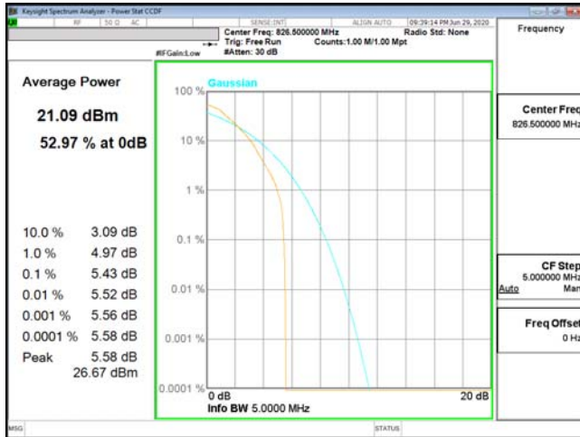
PTAR-ENDC_2A_n5-QPSK_5M_CH165300_826.5(25,0)
