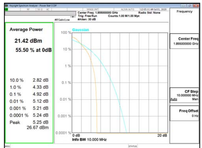
PTAR-ENDC_5A_n2-PI2-BPSK_10M_CH371000_1855(50,0)
