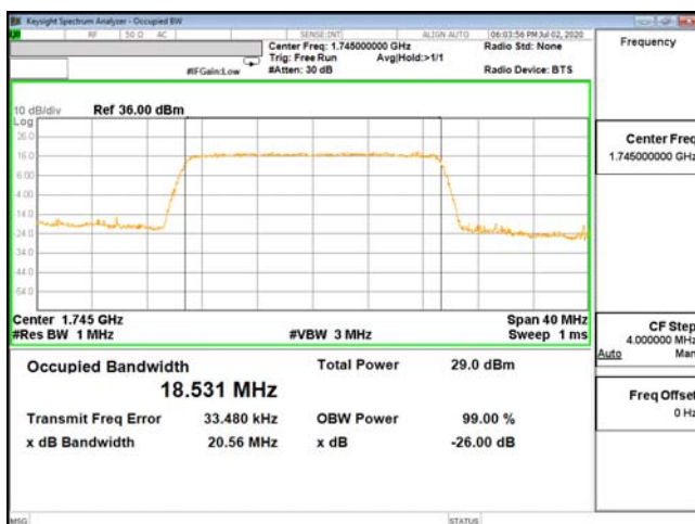
OCC-ENDC_66A_n5-QPSK_20M_CH132322_1745(100,0)
