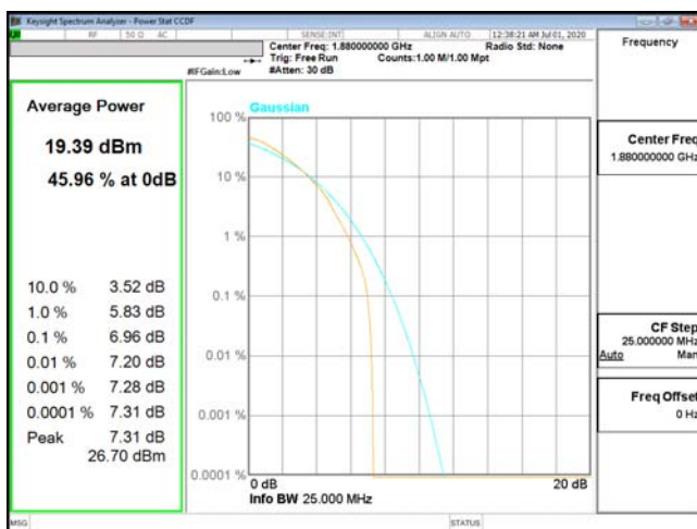
PTAR-ENDC_5A_n2-64QAM_20M_CH376000_1880(100,0)
