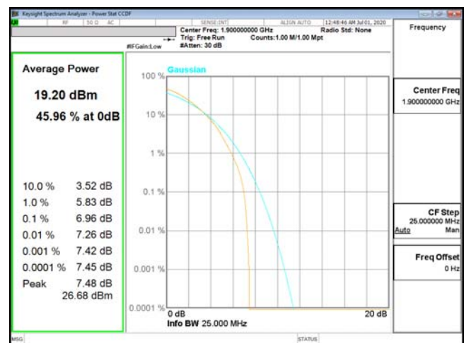
PTAR-ENDC_5A_n2-64QAM_20M_CH380000_1900(100,0)
