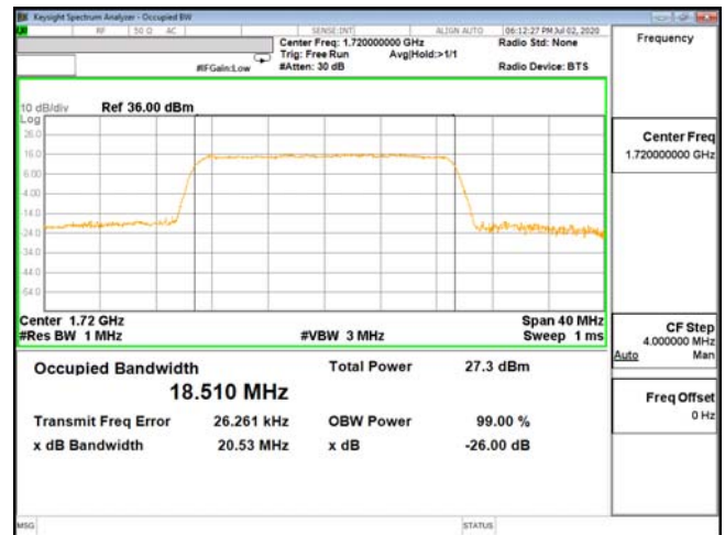
OCC-ENDC_66A_n5-64QAM_20M_CH132072_1720(100,0)
