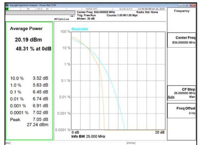
PTAR-ENDC_2A_n5-16QAM_20M_CH166800_834(100,0)
