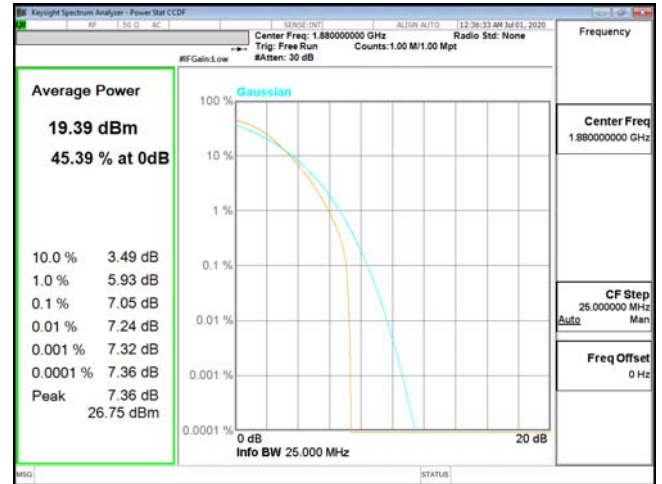
PTAR-ENDC_5A_n2-64QAM_15M_CH376000_1880(75,0)
