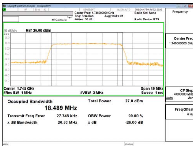
OCC-ENDC_66A_n5-64QAM_20M_CH132322_1745(100,0)
