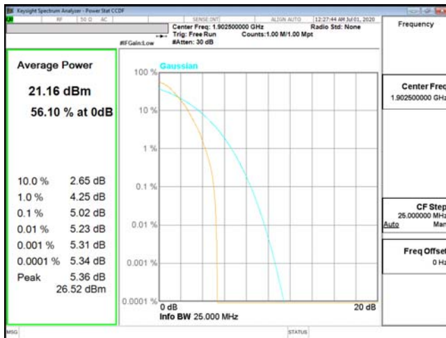
PTAR-ENDC_5A_n2-PI2-BPSK_15M_CH380500_1902.5(75,0)
