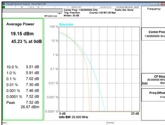
PTAR-ENDC_5A_n2-64QAM_15M_CH380500_1902.5(75,0)
