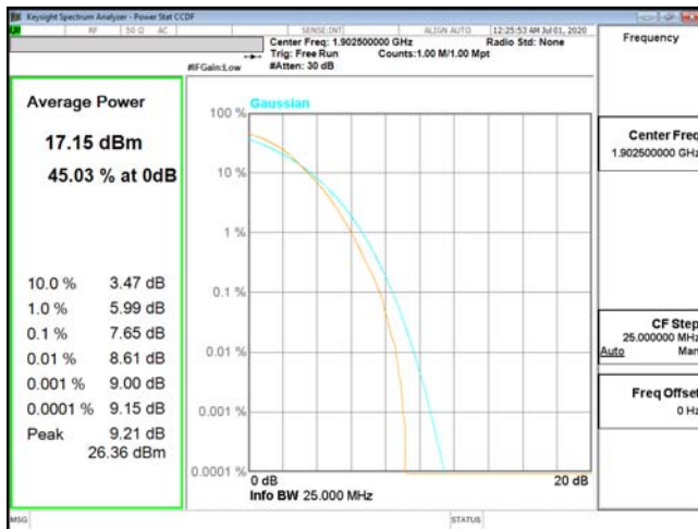
PTAR-ENDC_5A_n2-256QAM_15M_CH380500_1902.5(75,0)
