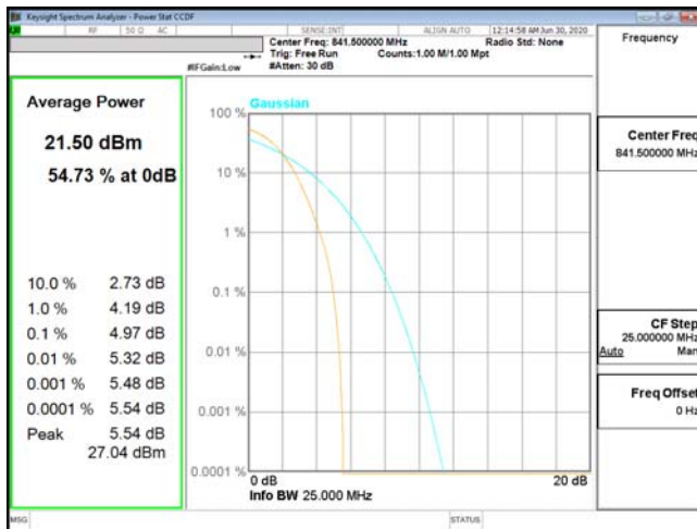
PTAR-ENDC_2A_n5-PI2-BPSK_15M_CH168300_841.5(75,0)
