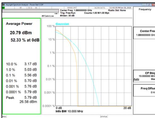
PTAR-ENDC_5A_n2-QPSK_10M_CH376000_1880(50,0)
