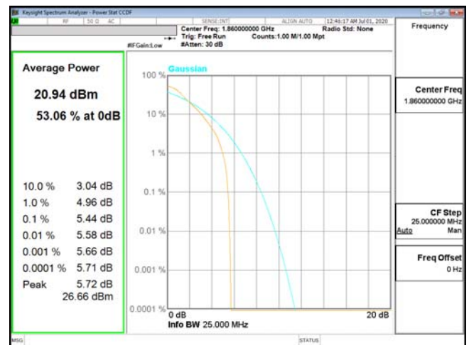
PTAR-ENDC_5A_n2-QPSK_20M_CH372000_1860(100,0)
