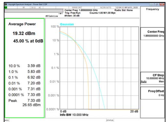
PTAR-ENDC_5A_n2-64QAM_10M_CH371000_1855(50,0)
