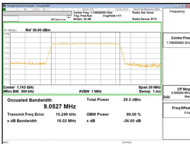
OCC-ENDC_66A_n5-64QAM_10M_CH132322_1745(50,0)
