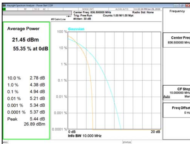
PTAR-ENDC_2A_n5-PI2-BPSK_10M_CH167300_836.5(50,0)
