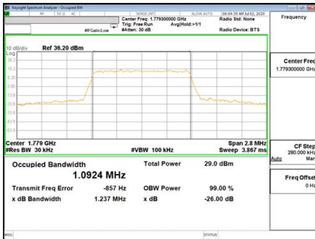
OCC-ENDC_66A_n5-16QAM_1.4M_CH132665_1779.3(6,0)
