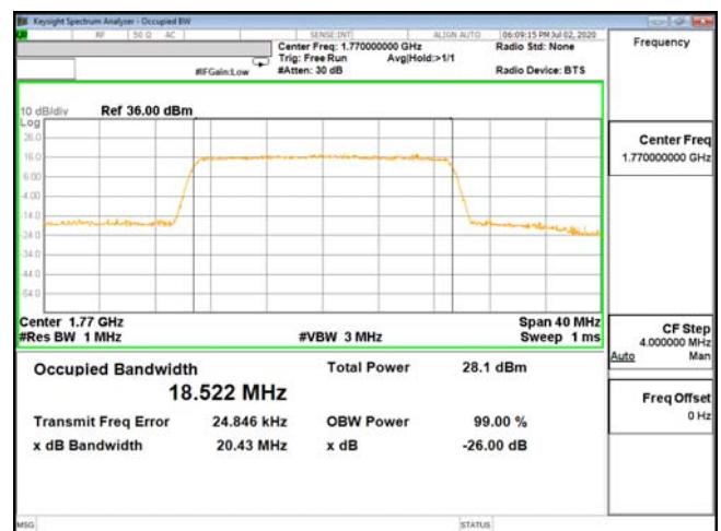
OCC-ENDC_66A_n5-16QAM_20M_CH132572_1770(100,0)
