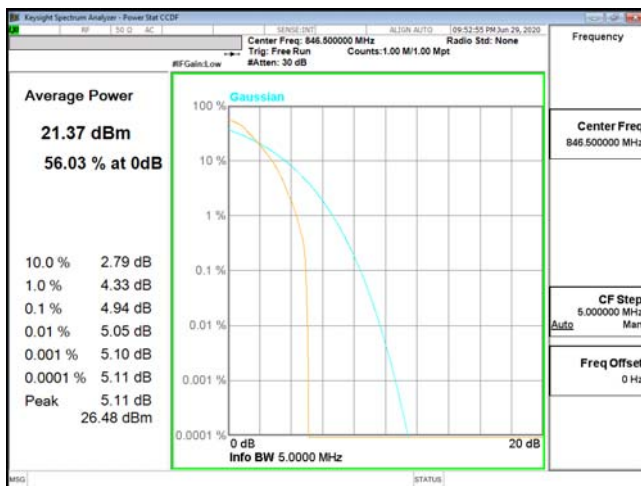
PTAR-ENDC_2A_n5-PI2-BPSK_5M_CH169300_846.5(25,0)
