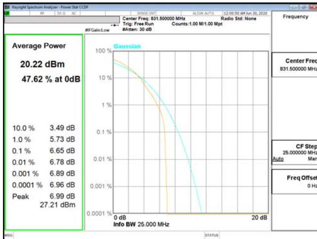
PTAR-ENDC_2A_n5-16QAM_15M_CH166300_831.5(75,0)
