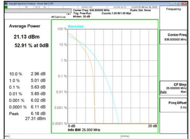
PTAR-ENDC_2A_n5-QPSK_15M_CH167300_836.5(75,0)
