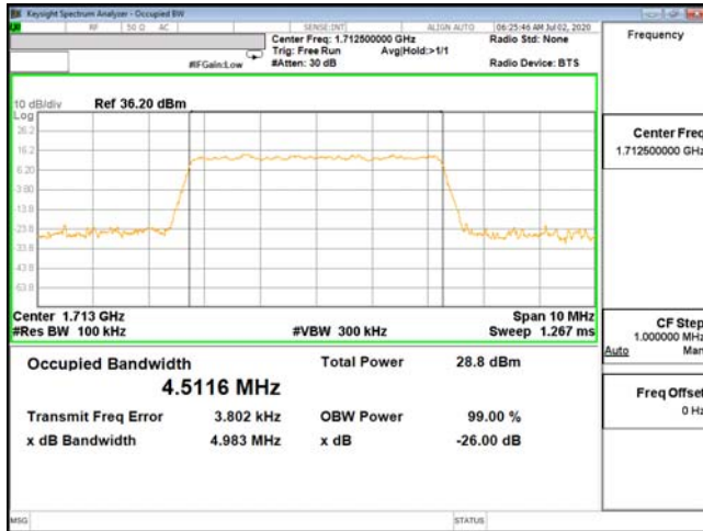
OCC-ENDC_66A_n5-64QAM_5M_CH131997_1712.5(25,0)
