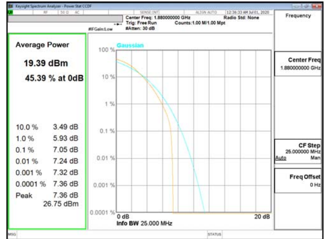
PTAR-ENDC_5A_n2-64QAM_15M_CH376000_1880(75,0)
