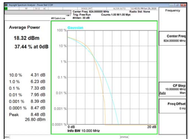
PTAR-ENDC_2A_n5-16QAM_10M_CH165800_824(50,0)
