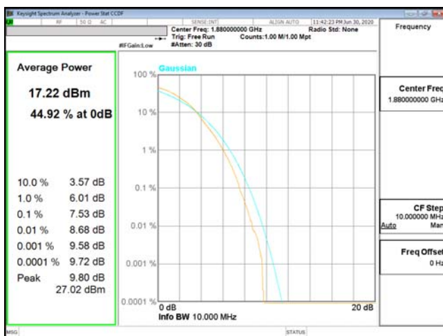
PTAR-ENDC_5A_n2-256QAM_10M_CH376000_1880(50,0)
