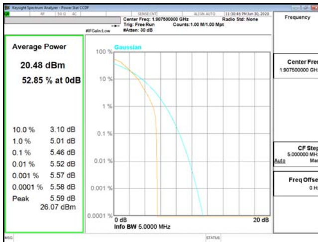
PTAR-ENDC_5A_n2-QPSK_5M_CH381500_1907.5(25,0)
