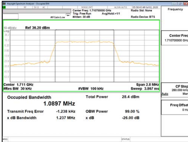
OCC-ENDC_66A_n5-64QAM_1.4M_CH131979_1710.7(6,0)
