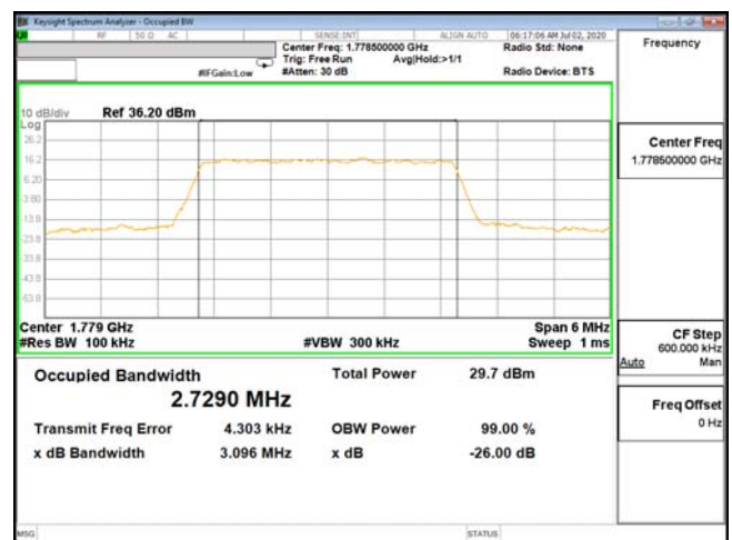
OCC-ENDC_66A_n5-16QAM_3M_CH132657_1778.5(15,0)
