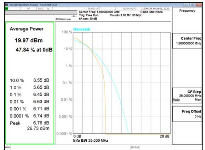
PTAR-ENDC_5A_n2-16QAM_20M_CH372000_1860(100,0)
