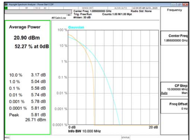
PTAR-ENDC_5A_n2-QPSK_10M_CH371000_1855(50,0)
