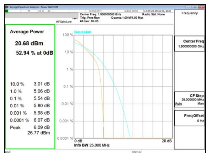
PTAR-ENDC_5A_n2-QPSK_20M_CH380000_1900(100,0)
