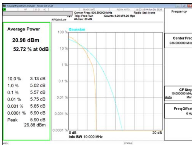
PTAR-ENDC_2A_n5-QPSK_10M_CH167300_836.5(50,0)
