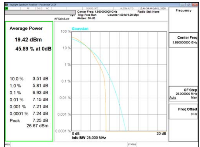
PTAR-ENDC_5A_n2-64QAM_20M_CH372000_1860(100,0)
