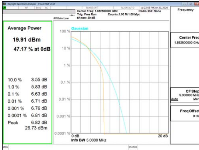
PTAR-ENDC_5A_n2-16QAM_5M_CH370500_1852.5(25,0)
