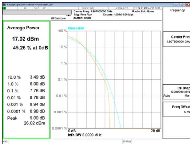
PTAR-ENDC_5A_n2-256QAM_5M_CH381500_1907.5(25,0)
