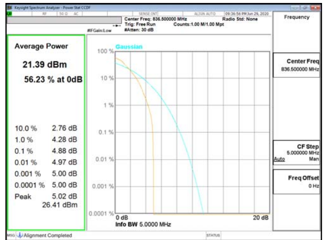
PTAR-ENDC_2A_n5-PI2-BPSK_5M_CH167300_836.5(25,0)
