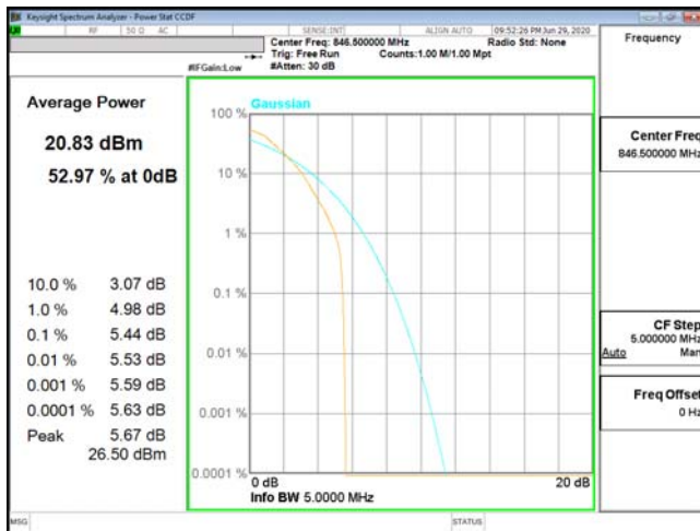
PTAR-ENDC_2A_n5-QPSK_5M_CH169300_846.5(25,0)
