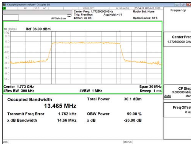
OCC-ENDC_66A_n5-QPSK_15M_CH132597_1772.5(75,0)
