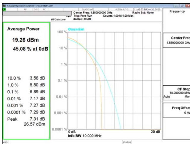
PTAR-ENDC_5A_n2-64QAM_10M_CH376000_1880(50,0)
