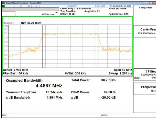
OCC-ENDC_13A_n66-QPSK_5M_CH23205_779.5(25,0)
