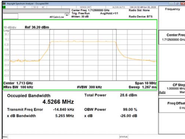
OCC-ENDC_13A_n66-64QAM_5M_CH342500_1712.5(25,0)
