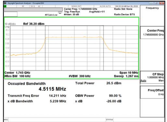
OCC-ENDC_13A_n66-256QAM_5M_CH349000_1745(25,0)
