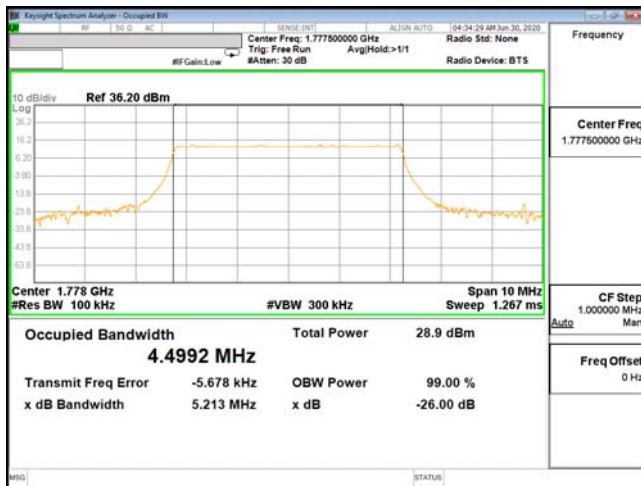
OCC-ENDC_13A_n66-16QAM_5M_CH355500_1777.5(25,0)
