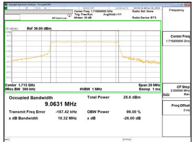
OCC-ENDC_13A_n66-16QAM_10M_CH343000_1715(50,0)
