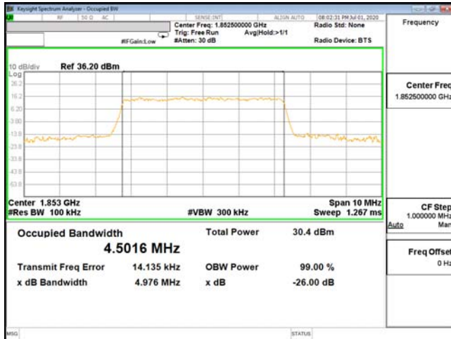
OCC-ENDC_2A_n5-QPSK_5M_CH18625_1852.5(25,0)
