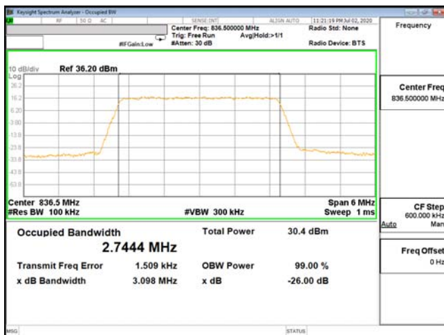
OCC-ENDC_5A_n2-QPSK_3M_CH20525_836.5(15,0)
