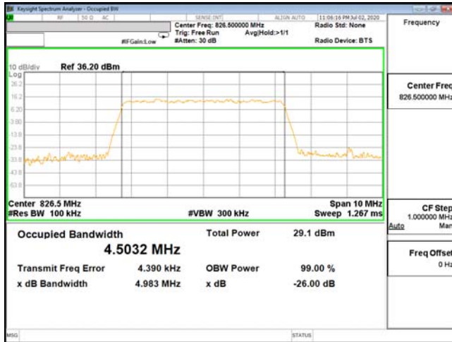
OCC-ENDC_5A_n2-64QAM_5M_CH20425_826.5(25,0)
