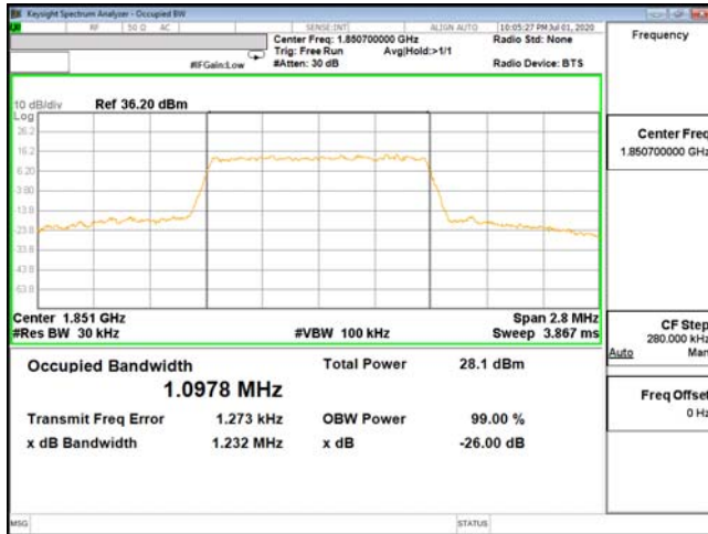
OCC-ENDC_2A_n5-64QAM_1.4M_CH18607_18507(6,0)
