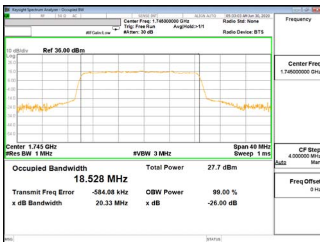
OCC-ENDC_13A_n66-16QAM_20M_CH349000_1745(100,0)
