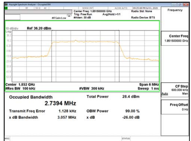
OCC-ENDC_2A_n5-64QAM_3M_CH18615_1851.5(15,0)
