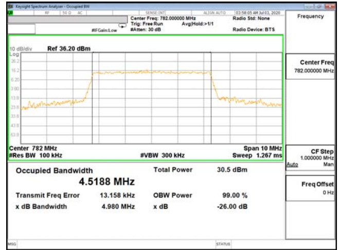
OCC-ENDC_13A_n66-QPSK_5M_CH23230_782(25,0)
