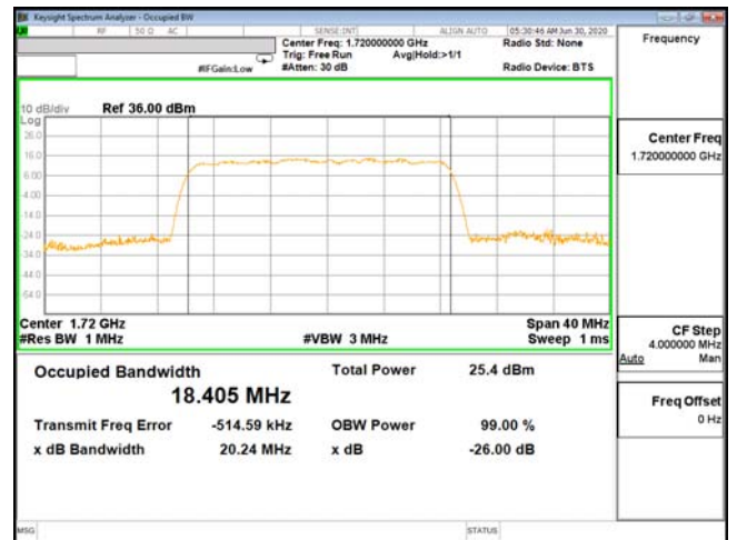
OCC-ENDC_13A_n66-256QAM_20M_CH344000_1720(100,0)
