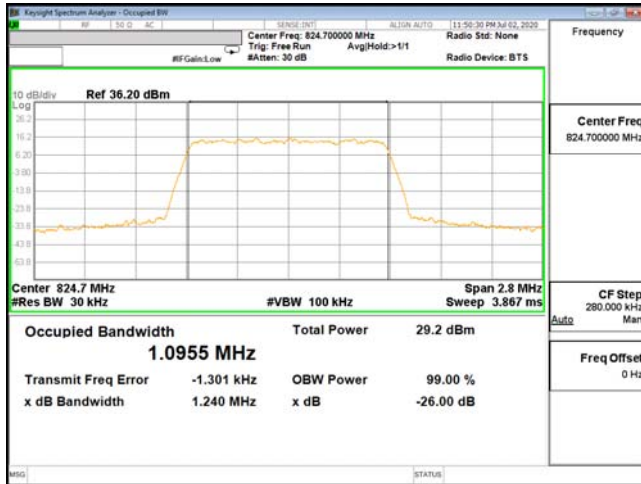
OCC-ENDC_5A_n2-16QAM_1.4M_CH20407_824.7(6,0)
