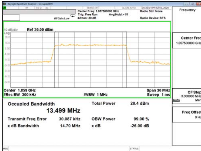
OCC-ENDC_2A_n5-64QAM_15M_CH18675_1857.5(75,0)
