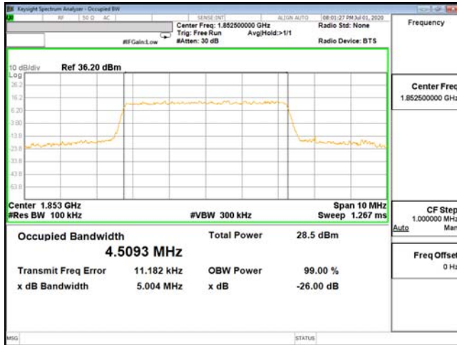
OCC-ENDC_2A_n5-64QAM_5M_CH18625_1852.5(25,0)
