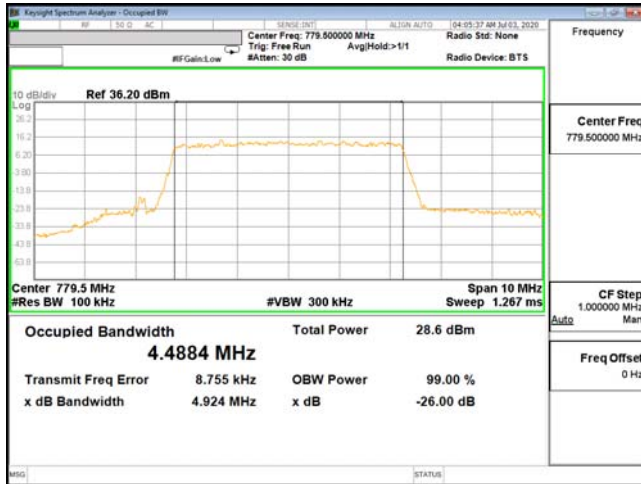
OCC-ENDC_13A_n66-64QAM_5M_CH23205_779.5(25,0)
