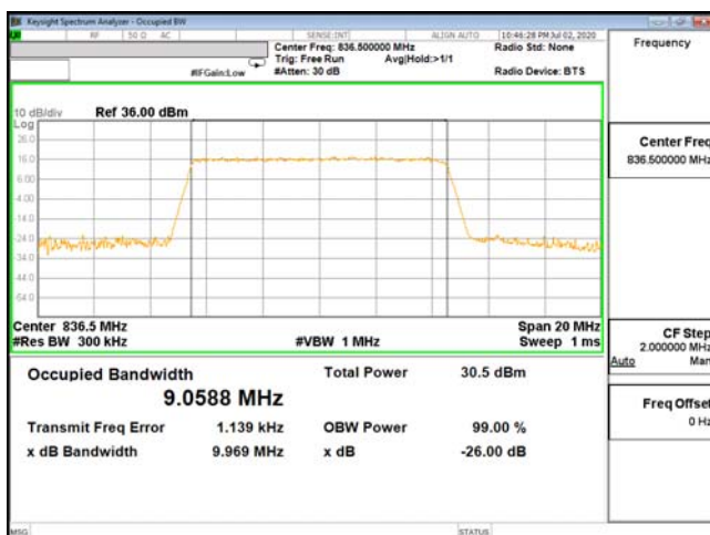
OCC-ENDC_5A_n2-QPSK_10M_CH20525_836.5(50,0)
