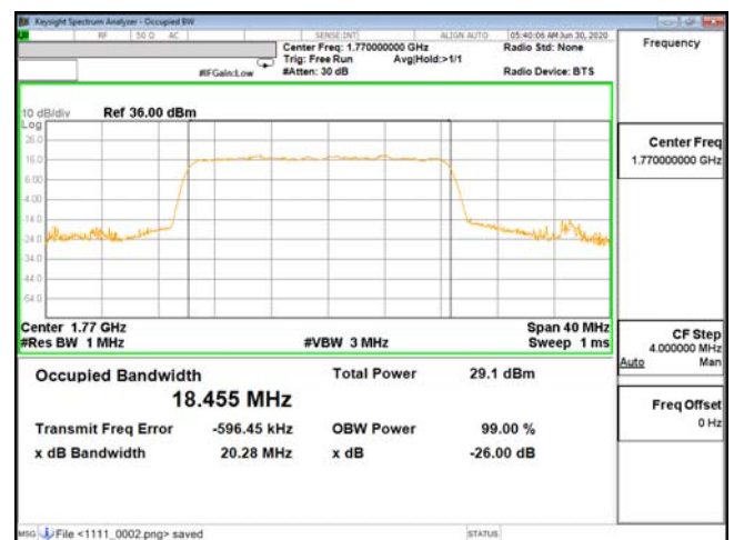
OCC-ENDC_13A_n66-QPSK_20M_CH354000_1770(100,0)
