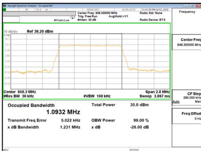
OCC-ENDC_5A_n2-QPSK_1.4M_CH20643_848.3(6,0)
