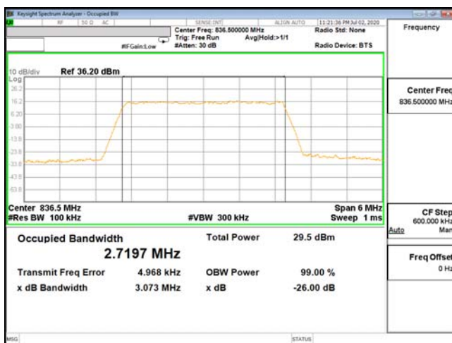
OCC-ENDC_5A_n2-16QAM_3M_CH20525_836.5(15,0)
