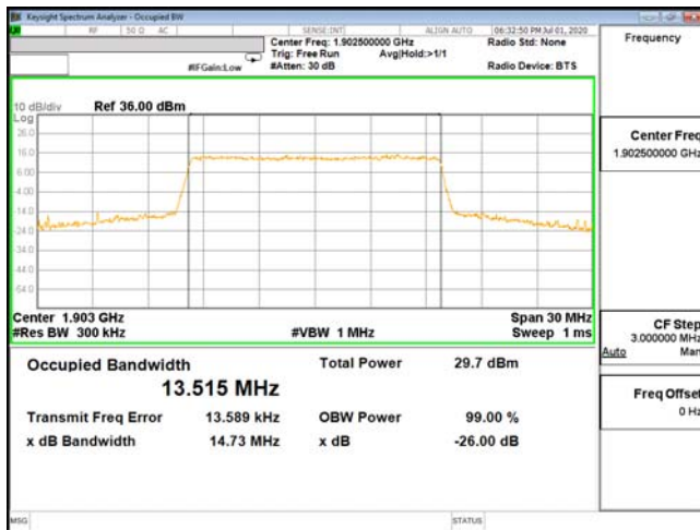
OCC-ENDC_2A_n5-QPSK_15M_CH19125_1902.5(75,0)
