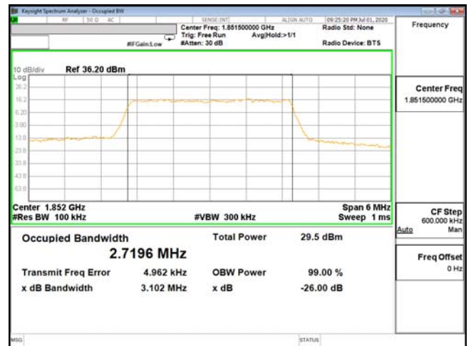
OCC-ENDC_2A_n5-16QAM_3M_CH18615_1851.5(15,0)
