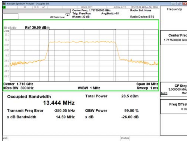
OCC-ENDC_13A_n66-64QAM_15M_CH343500_1717.5(75,0)
