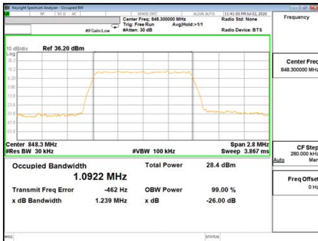
OCC-ENDC_5A_n2-64QAM_1.4M_CH20643_848.3(6,0)
