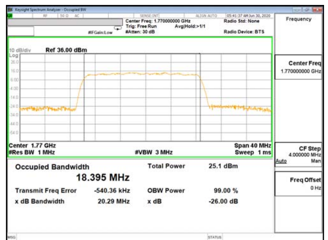
OCC-ENDC_13A_n66-256QAM_20M_CH354000_1770(100,0)
