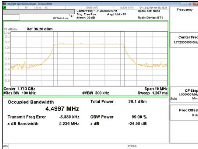
OCC-ENDC_13A_n66-16QAM_5M_CH342500_1712.5(25,0)
