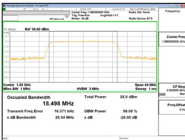
OCC-ENDC_2A_n5-16QAM_20M_CH18900_1880(100,0)
