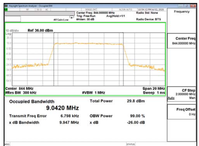
OCC-ENDC_5A_n2-16QAM_10M_CH20600_844(50,0)
