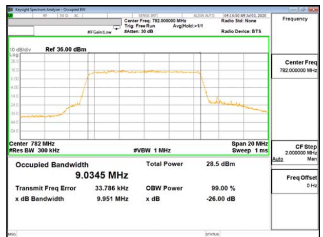
OCC-ENDC_13A_n66-64QAM_10M_CH23230_782(50,0)
