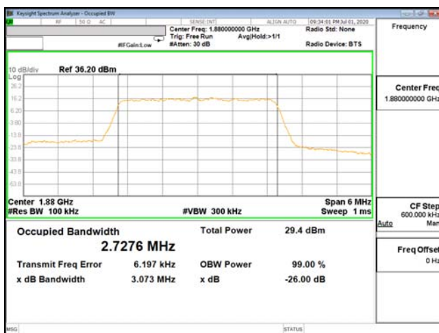
OCC-ENDC_2A_n5-16QAM_3M_CH18900_1880(15,0)
