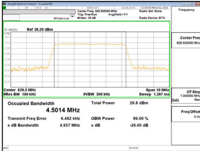
OCC-ENDC_5A_n2-16QAM_5M_CH20425_826.5(25,0)
