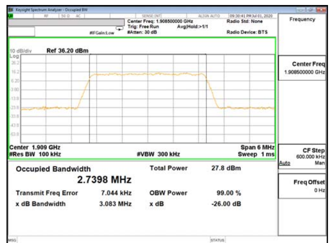
OCC-ENDC_2A_n5-64QAM_3M_CH19185_1908.5(15,0)
