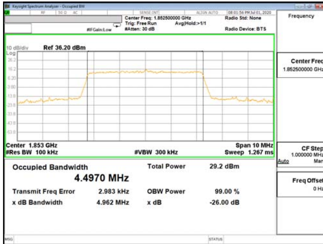
OCC-ENDC_2A_n5-16QAM_5M_CH18625_1852.5(25,0)
