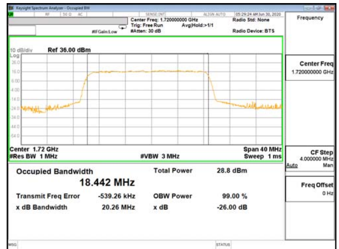
OCC-ENDC_13A_n66-QPSK_20M_CH344000_1720(100,0)
