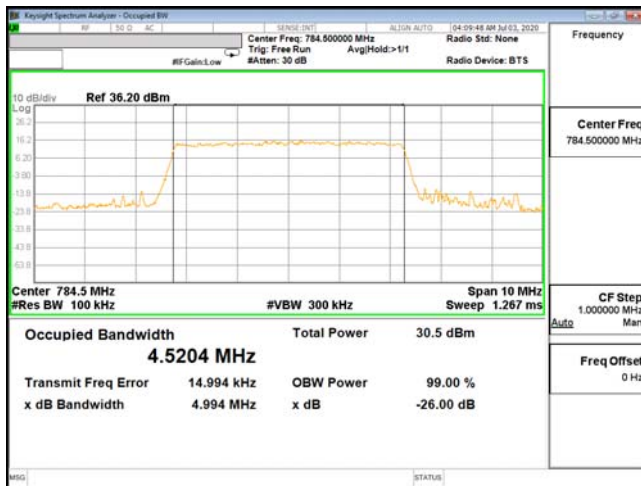
OCC-ENDC_13A_n66-QPSK_5M_CH23255_784.5(25,0)
