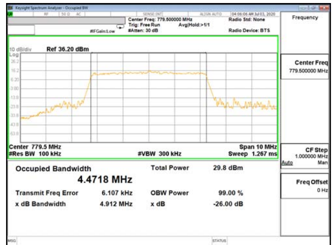
OCC-ENDC_13A_n66-16QAM_5M_CH23205_779.5(25,0)
