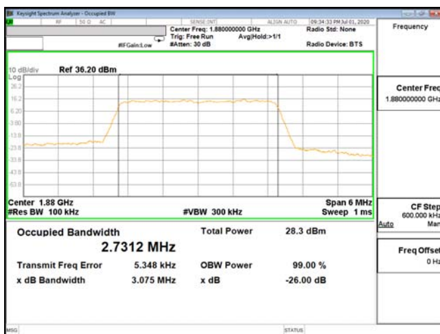
OCC-ENDC_2A_n5-64QAM_3M_CH18900_1880(15,0)
