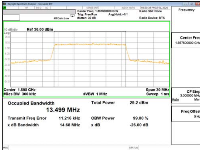
OCC-ENDC_2A_n5-16QAM_15M_CH18675_1857.5(75,0)
