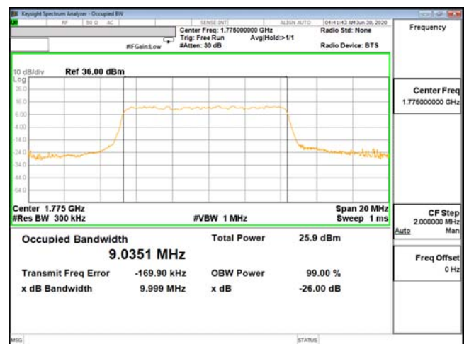
OCC-ENDC_13A_n66-256QAM_10M_CH355000_1775(50,0)
