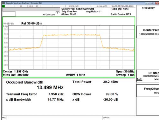
OCC-ENDC_2A_n5-QPSK_15M_CH18675_1857.5(75,0)
