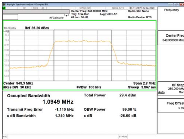
OCC-ENDC_5A_n2-16QAM_1.4M_CH20643_848.3(6,0)
