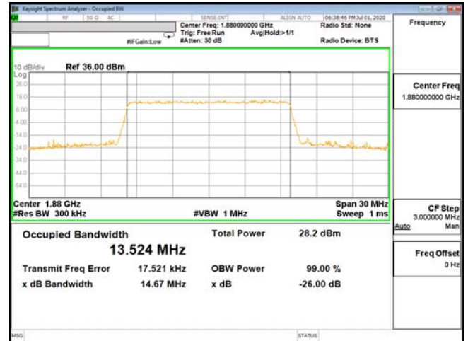
OCC-ENDC_2A_n5-64QAM_15M_CH18900_1880(75,0)
