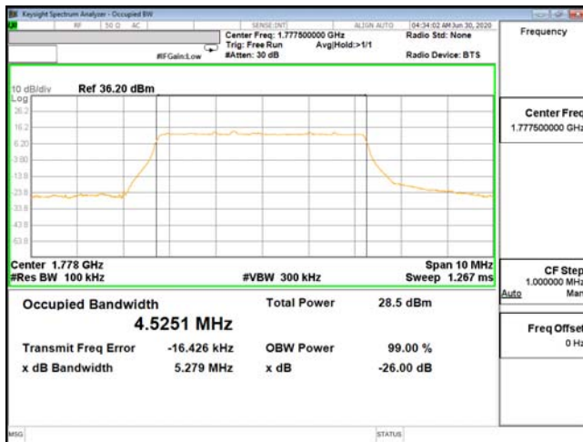
OCC-ENDC_13A_n66-64QAM_5M_CH355500_1777.5(25,0)
