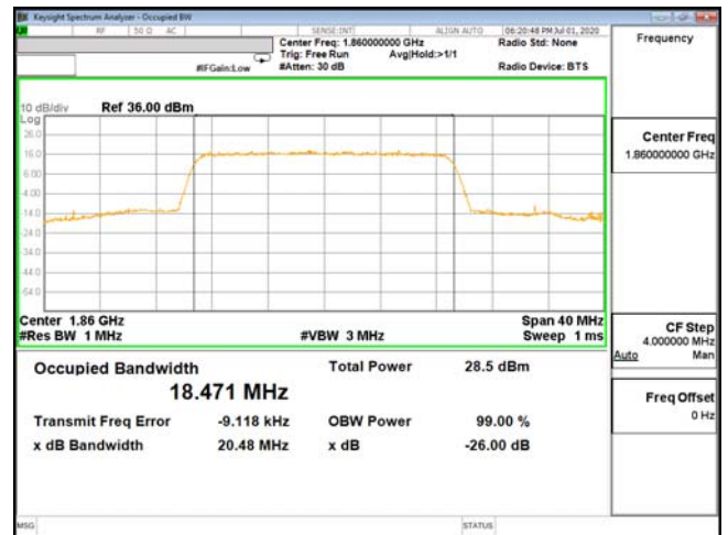
OCC-ENDC_2A_n5-QPSK_20M_CH18700_1860(100,0)
