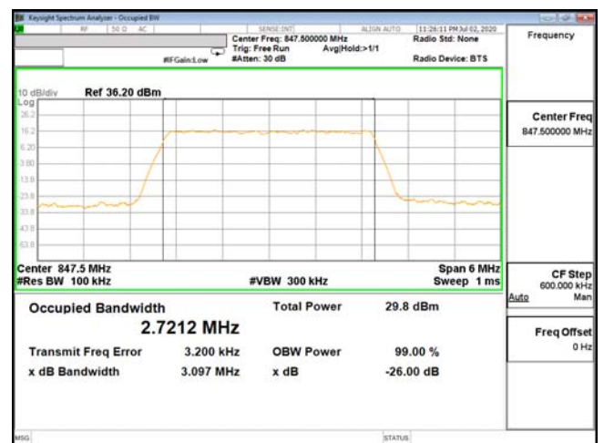
OCC-ENDC_5A_n2-16QAM_3M_CH20635_847.5(15,0)
