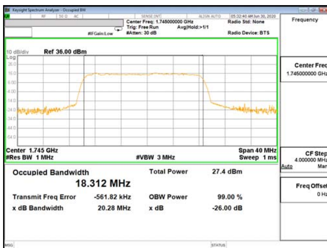
OCC-ENDC_13A_n66-64QAM_20M_CH349000_1745(100,0)
