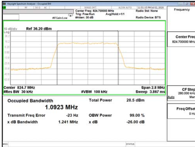
OCC-ENDC_5A_n2-64QAM_1.4M_CH20407_824.7(6,0)
