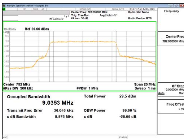
OCC-ENDC_13A_n66-16QAM_10M_CH23230_782(50,0)
