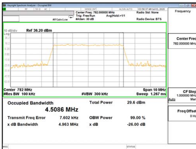
OCC-ENDC_13A_n66-16QAM_5M_CH23230_782(25,0)
