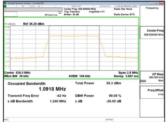
OCC-ENDC_5A_n2-64QAM_1.4M_CH20525_836.5(6,0)
