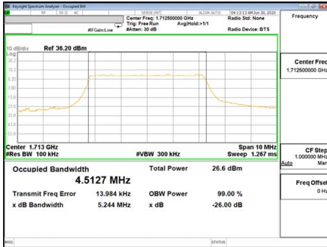
OCC-ENDC_13A_n66-256QAM_5M_CH342500_1712.5(25,0)
