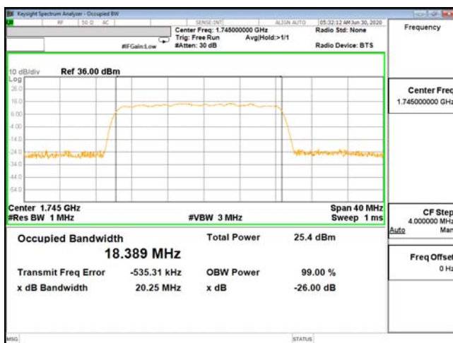
OCC-ENDC_13A_n66-256QAM_20M_CH349000_1745(100,0)
