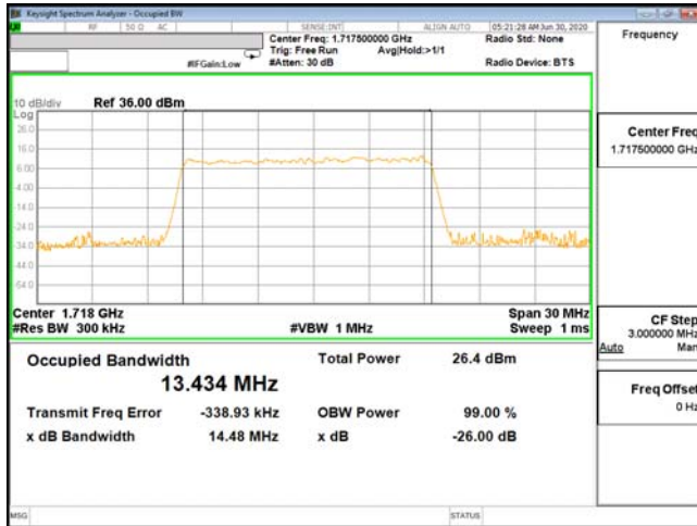
OCC-ENDC_13A_n66-256QAM_15M_CH343500_1717.5(75,0)
