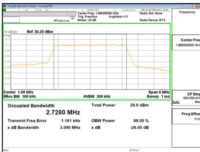
OCC-ENDC_2A_n5-QPSK_3M_CH18900_1880(15,0)
