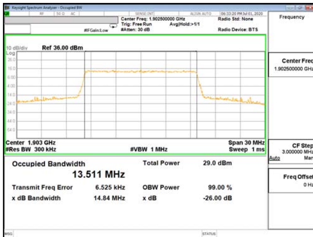
OCC-ENDC_2A_n5-16QAM_15M_CH19125_1902.5(75,0)
