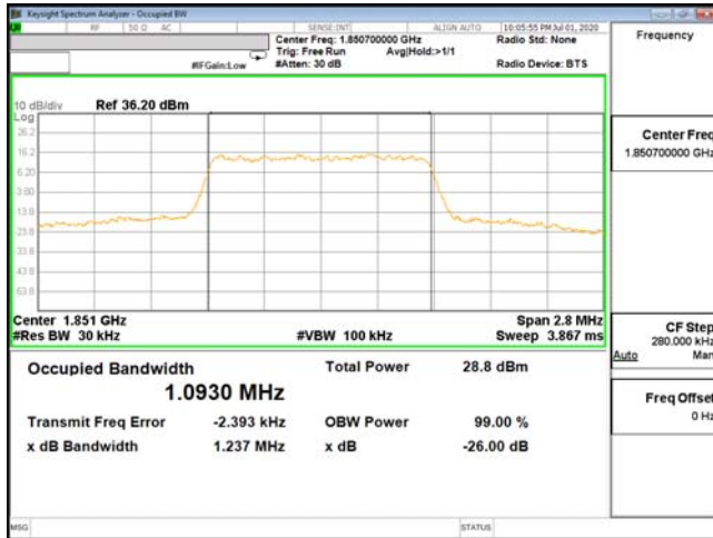
OCC-ENDC_2A_n5-16QAM_1.4M_CH18607_18507(6,0)
