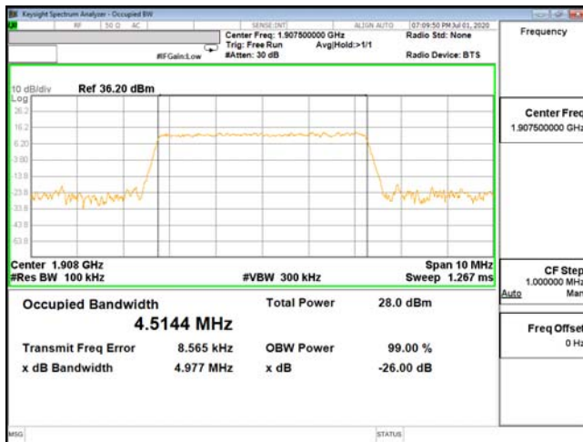
OCC-ENDC_2A_n5-64QAM_5M_CH19175_1907.5(25,0)
