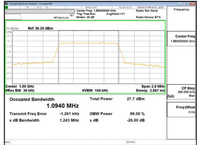
OCC-ENDC_2A_n5-64QAM_1.4M_CH18900_1880(6,0)
