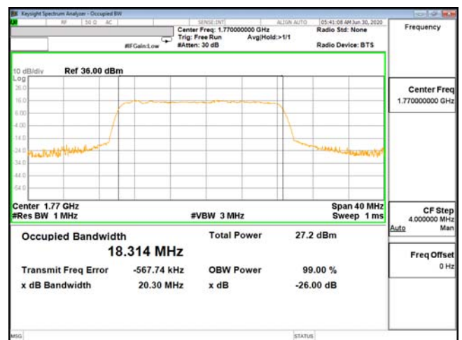
OCC-ENDC_13A_n66-64QAM_20M_CH354000_1770(100,0)
