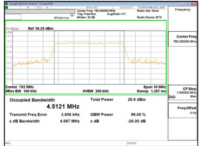
OCC-ENDC_13A_n66-64QAM_5M_CH23230_782(25,0)
