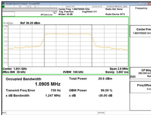
OCC-ENDC_2A_n5-QPSK_1.4M_CH18607_18507(6,0)
