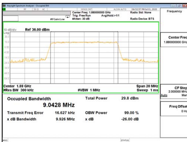
OCC-ENDC_2A_n5-QPSK_10M_CH18900_1880(50,0)
