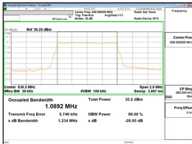
OCC-ENDC_5A_n2-QPSK_1.4M_CH20525_836.5(6,0)
