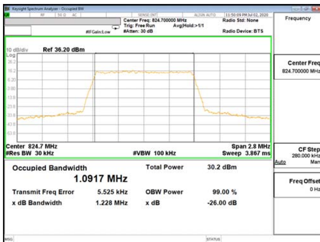
OCC-ENDC_5A_n2-QPSK_1.4M_CH20407_824.7(6,0)
