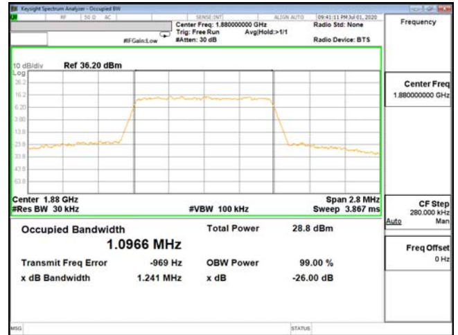
OCC-ENDC_2A_n5-16QAM_1.4M_CH18900_1880(6,0)
