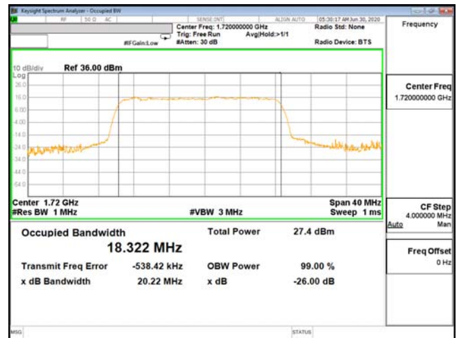
OCC-ENDC_13A_n66-64QAM_20M_CH344000_1720(100,0)
