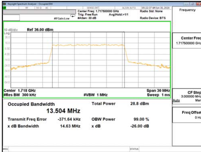
OCC-ENDC_13A_n66-16QAM_15M_CH343500_1717.5(75,0)
