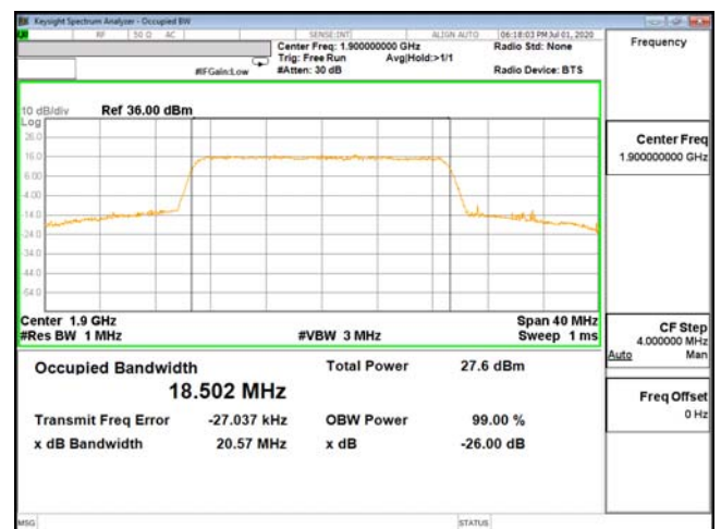
OCC-ENDC_2A_n5-16QAM_20M_CH19100_1900(100,0)
