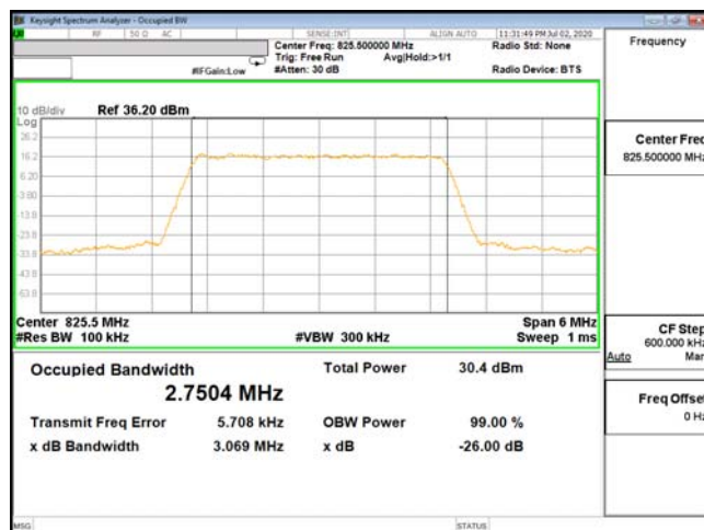
OCC-ENDC_5A_n2-QPSK_3M_CH20415_825.5(15,0)
