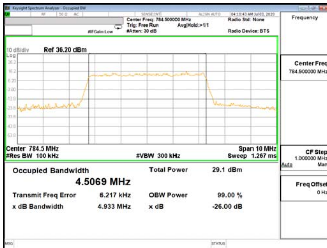
OCC-ENDC_13A_n66-64QAM_5M_CH23255_784.5(25,0)
