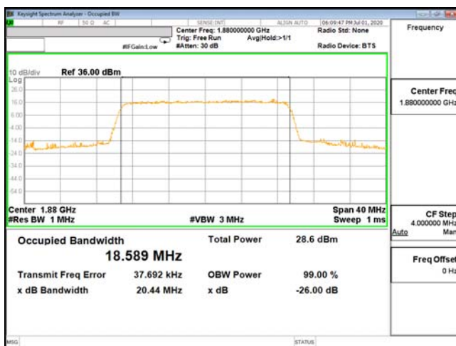
OCC-ENDC_2A_n5-QPSK_20M_CH18900_1880(100,0)
