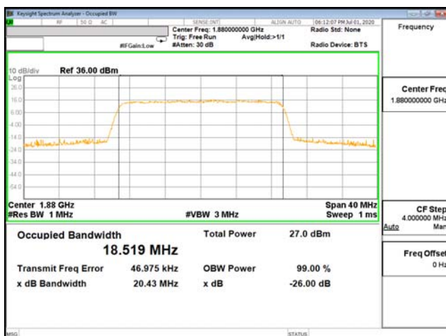
OCC-ENDC_2A_n5-64QAM_20M_CH18900_1880(100,0)
