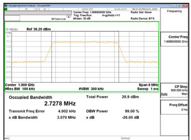
OCC-ENDC_2A_n5-16QAM_3M_CH19185_1908.5(15,0)
