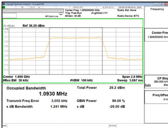
OCC-ENDC_2A_n5-QPSK_1.4M_CH19193_1909.3(6,0)
