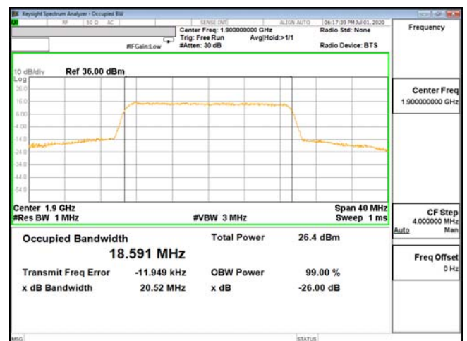
OCC-ENDC_2A_n5-64QAM_20M_CH19100_1900(100,0)
