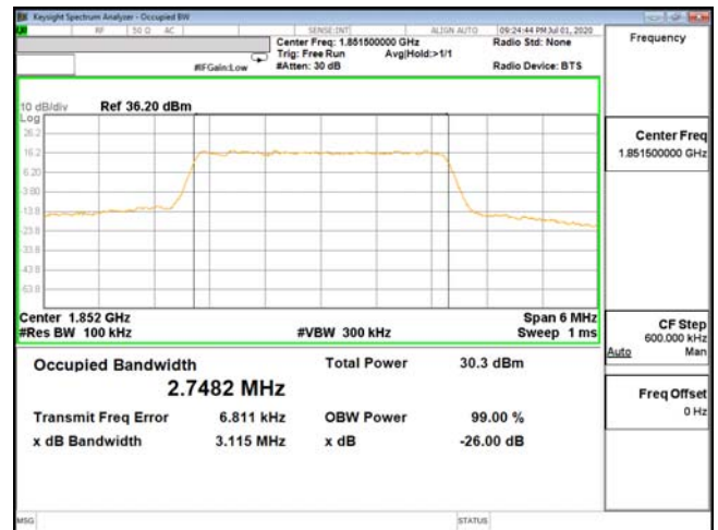
OCC-ENDC_2A_n5-QPSK_3M_CH18615_1851.5(15,0)
