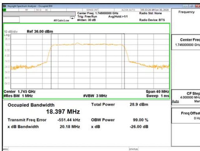
OCC-ENDC_13A_n66-QPSK_20M_CH349000_1745(100,0)
