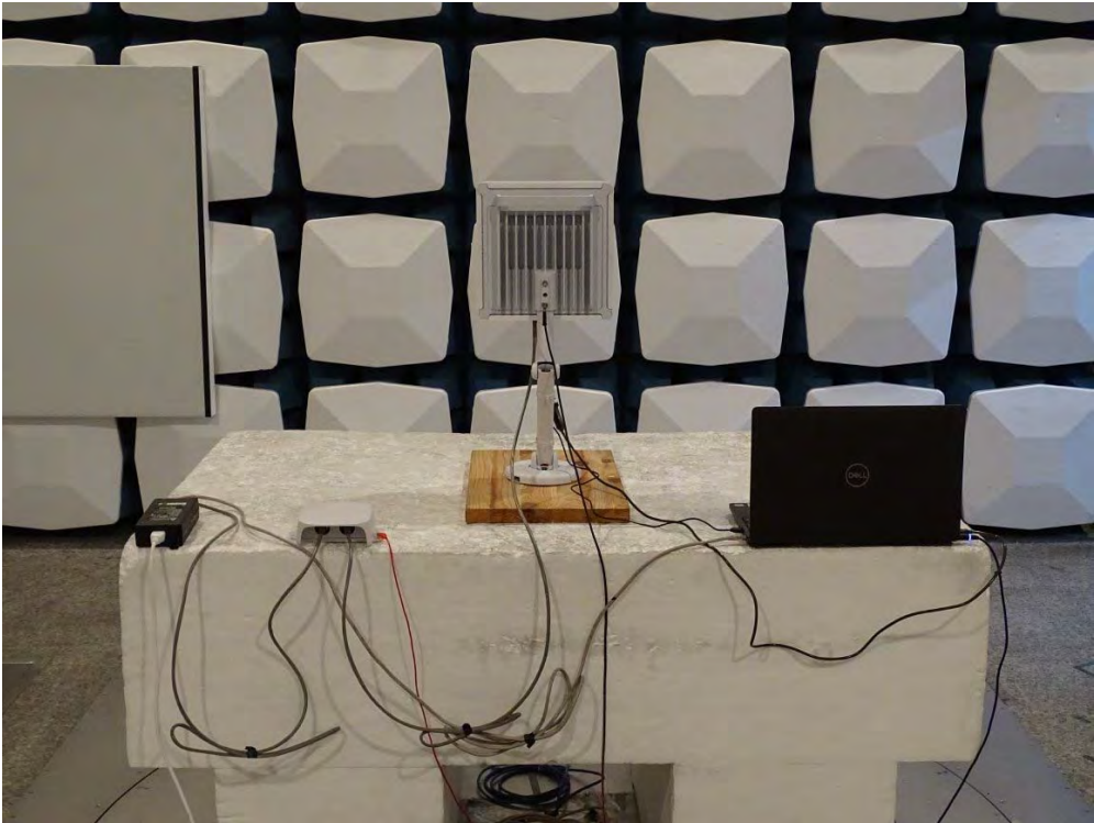
Back View of Radiated Test (PoE Mode)
