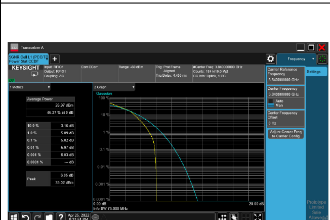
5G NR n77_CH656000_70M_1RB_16-QAM_Ratio
