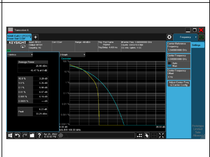
5G NR n77_CH656000_80M_1RB_16-QAM_Ratio
