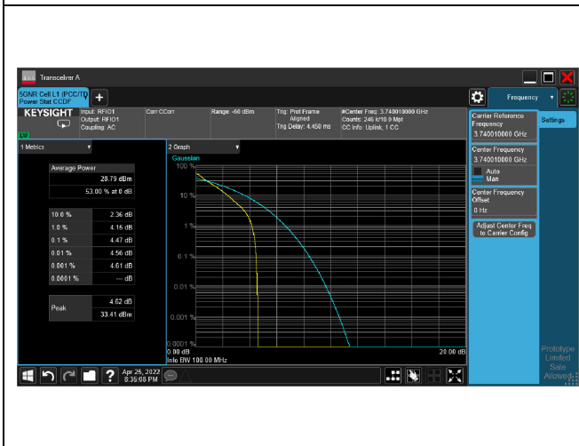
5G NR n77_CH649334_80M_1RB_16-QAM_Ratio
