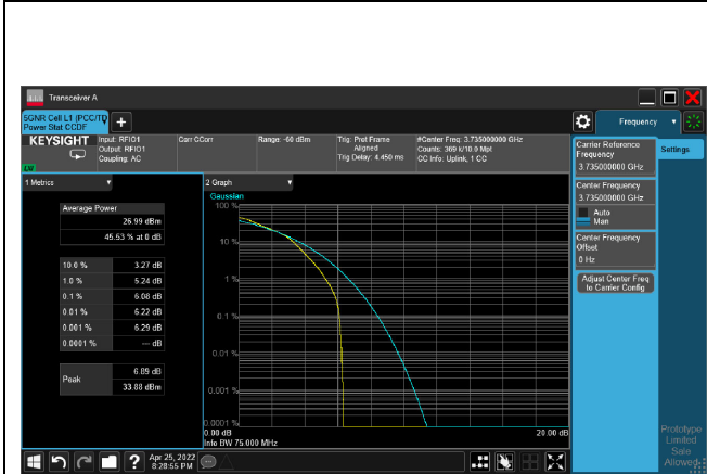
5G NR n77_CH649000_70M_1RB_16-QAM_Ratio
