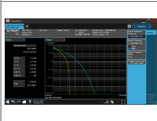
5G NR n77_CH648668_60M_1RB_16-QAM_Ratio
