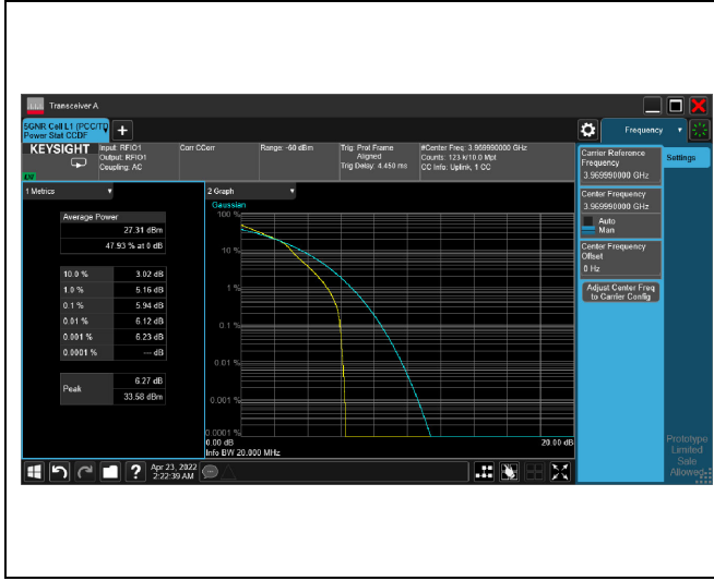
5G NR n77_CH664666_20M_1RB_16-QAM_Ratio
