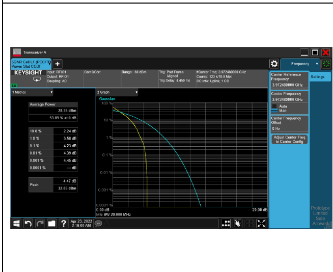
5G NR n77_CH664832_15M_1RB_16-QAM_Ratio
