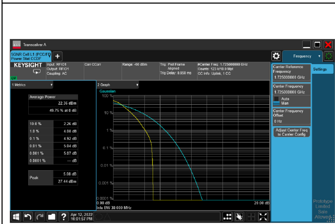
5G NR n66_CH345000_30M_1RB_pi/2 BPSK_Ratio
