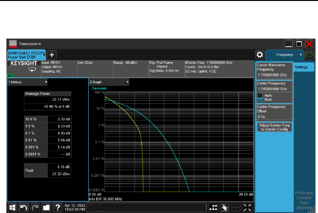
5G NR n66_CH349000_30M_1RB_pi/2 BPSK_Ratio
