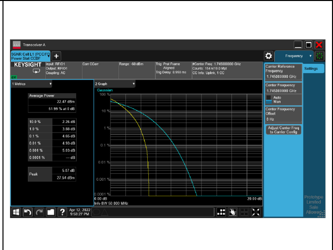
5G NR n66_CH349000_40M_1RB_16-QAM_Ratio
