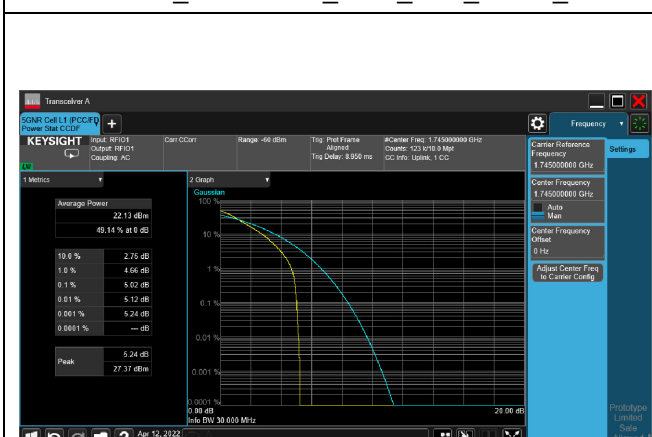
5G NR n66_CH349000_30M_1RB_QPSK_Ratio
