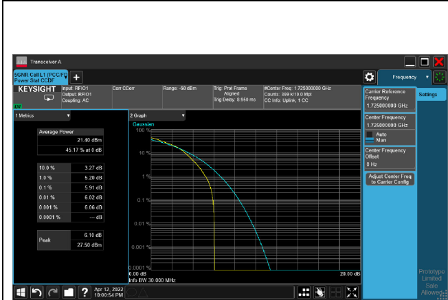
5G NR n66_CH345000_30M_1RB_16-QAM_Ratio
