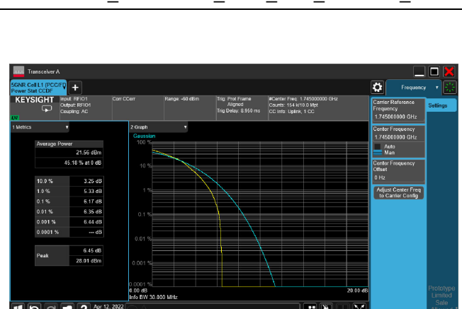
5G NR n66_CH349000_30M_1RB_16-QAM_Ratio
