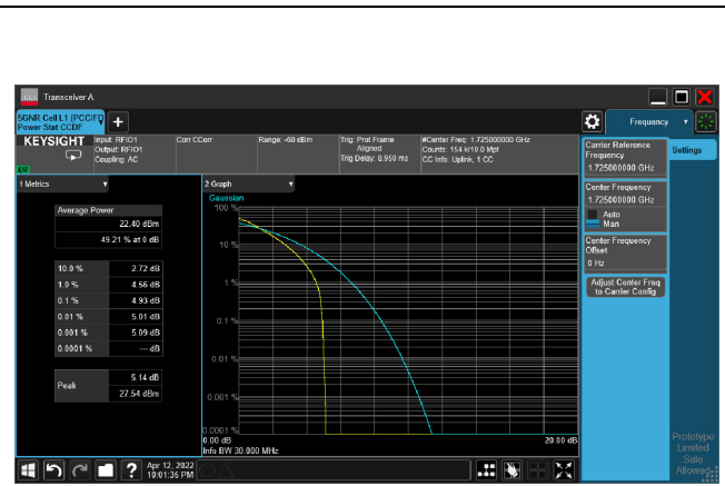
5G NR n66_CH345000_30M_1RB_QPSK_Ratio
