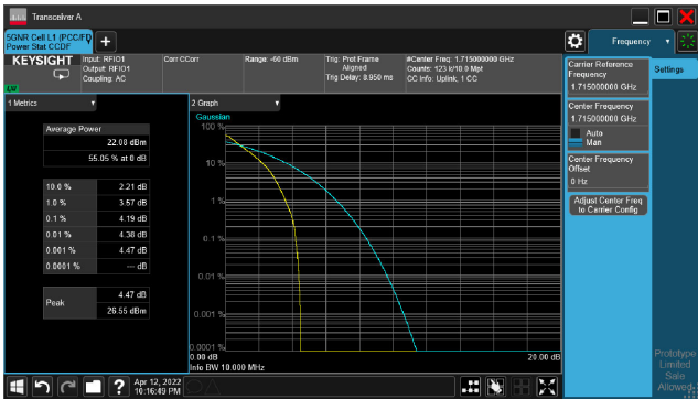
5G NR n66_CH343000_10M_1RB_16-QAM_Ratio
