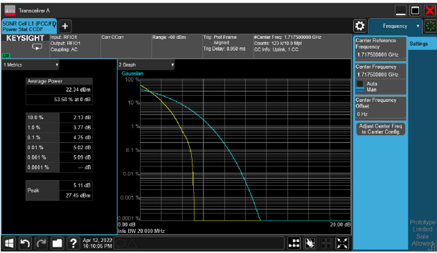
5G NR n66_CH343500_15M_1RB_16-QAM_Ratio
