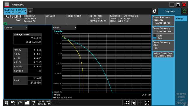
5G NR n66_CH349000_15M_1RB_16-QAM_Ratio
