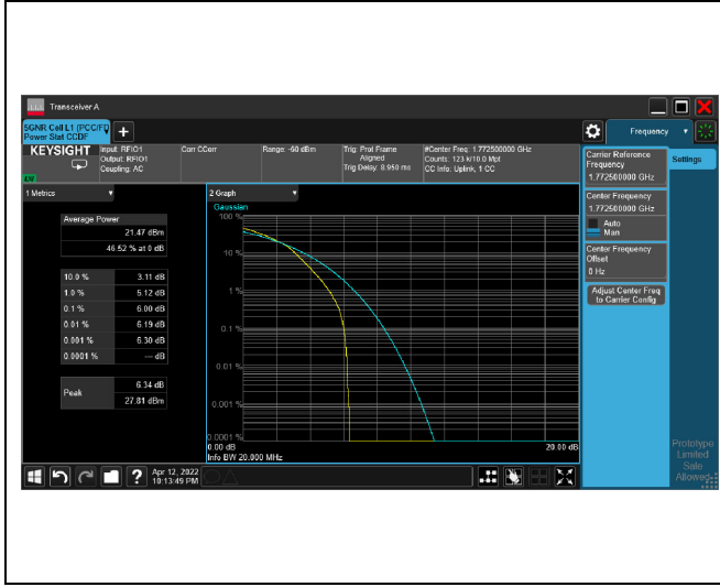
5G NR n66_CH354500_15M_1RB_16-QAM_Ratio
