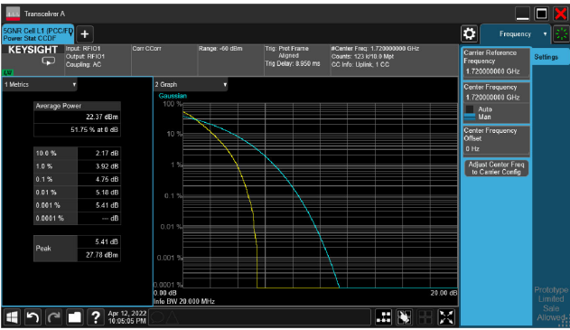
5G NR n66_CH344000_20M_1RB_16-QAM_Ratio
