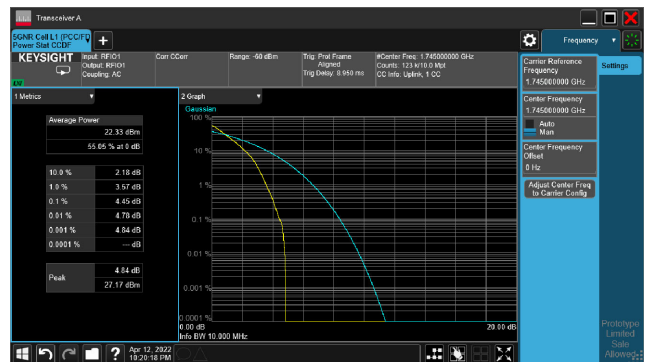
5G NR n66_CH349000_10M_1RB_16-QAM_Ratio
