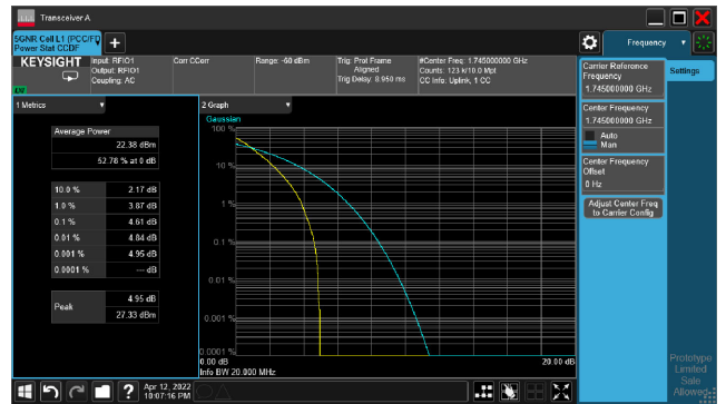
5G NR n66_CH349000_20M_1RB_16-QAM_Ratio
