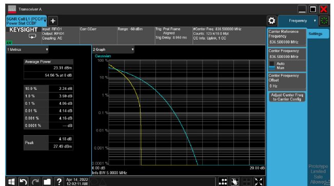
5G NR n5_CH167300_5M_1RB_16-QAM_Ratio
