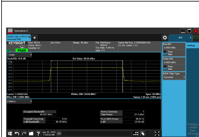
16QAMCH649668_90M
