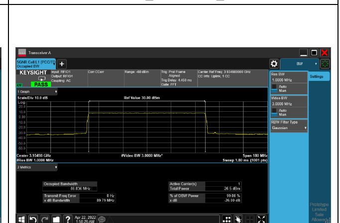
64QAM_CH662332_90M
