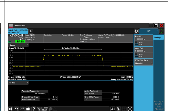
64QAM_CH649668_90M
