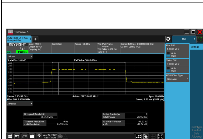
16QAM_CH662332_90M
