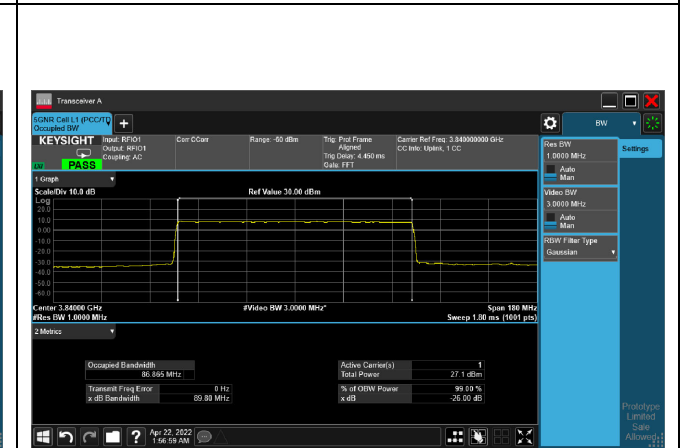
16QAM_CH656000_90M
