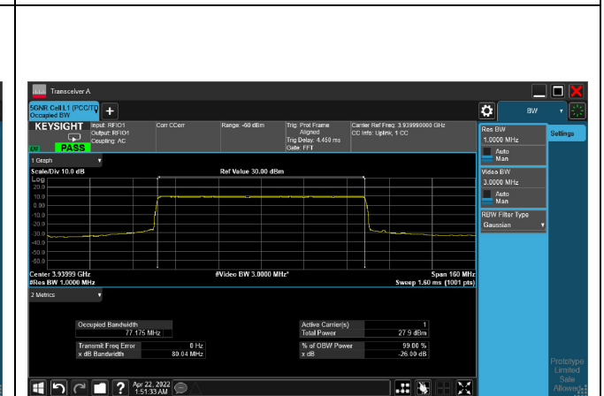
QPSK_CH662666_80M
