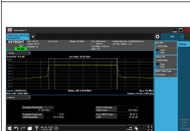
QPSK_CH656000_80M
