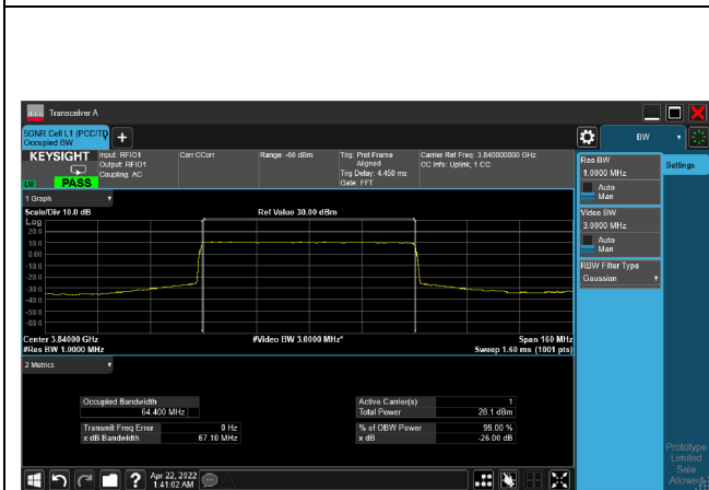
QPSK_CH656000_70M
