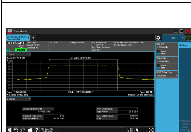
QPSK_CH656000_60M
