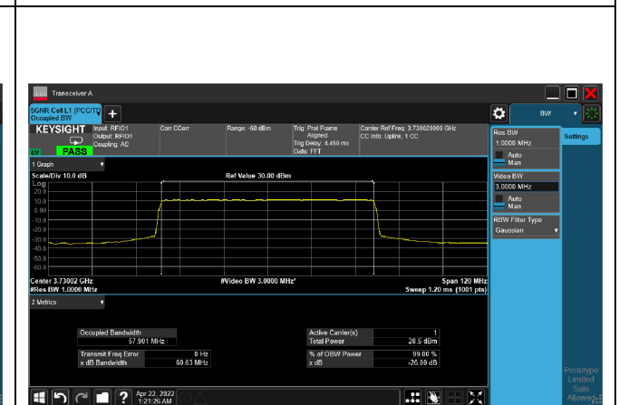
QPSK_CH648668_60M
