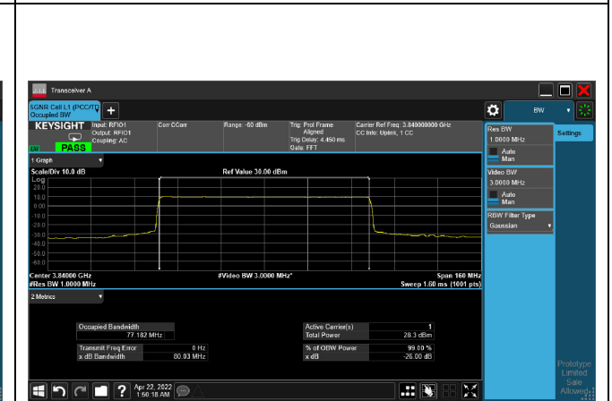
pi/2-BPSK_CH656000_80M
