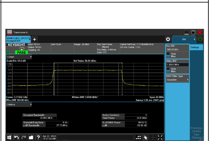
64QAM_CH647668_30M
