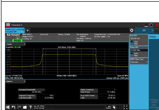
16QAM_CH647668_30M
