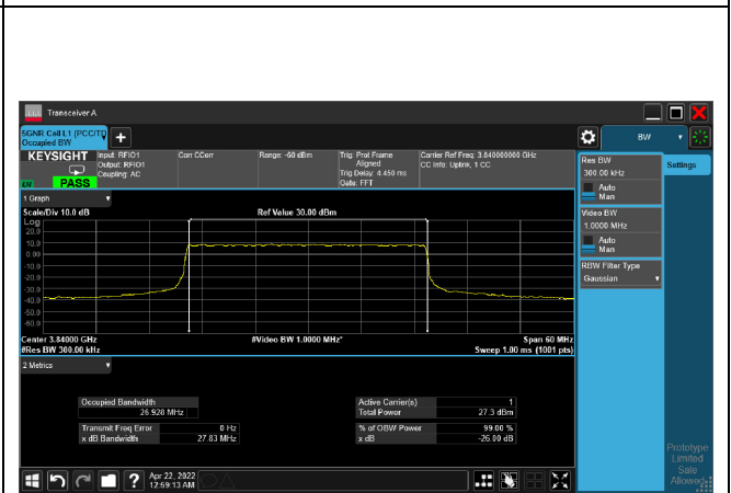
16QAM_CH656000_30M
