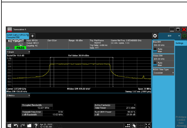
16QAM_CH664832_15M
