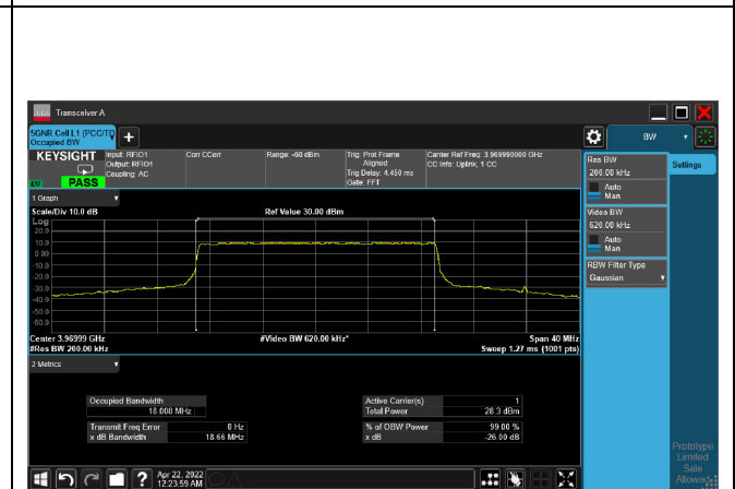
QPSK_CH664666_20M
