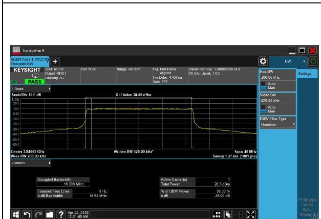
QPSK_CH656000_20M
