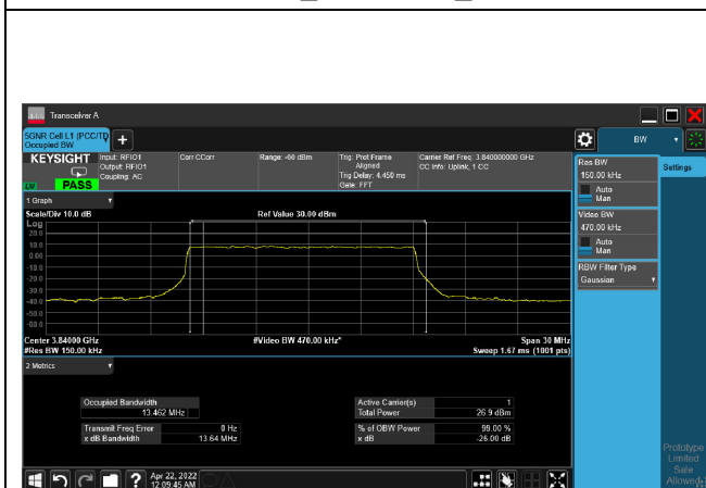
64QAM_CH656000_15M
