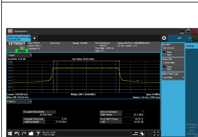
16QAM_CH664332_30M
