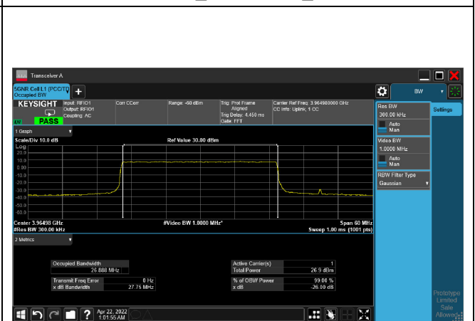
64QAM_CH664332_30M
