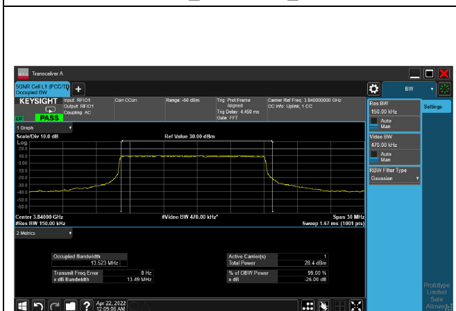
QPSK_CH656000_15M
