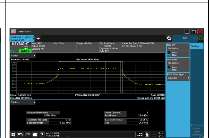
64QAM_CH647000_10M
