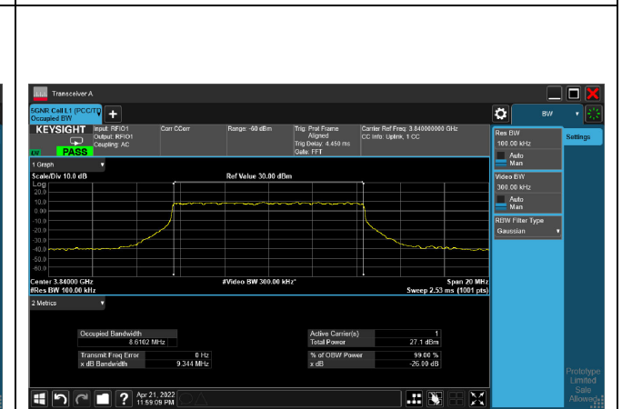
16QAM_CH656000_10M
