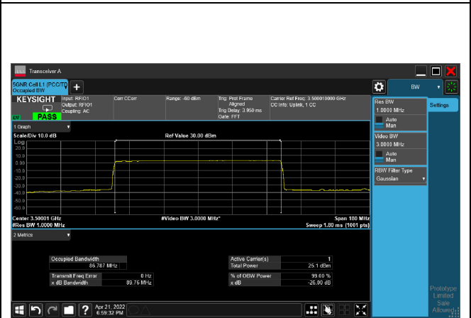
256QAM_CH633334_90M
