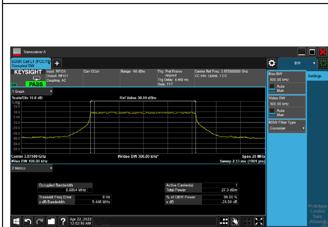
16QAM_CH665000_10M
