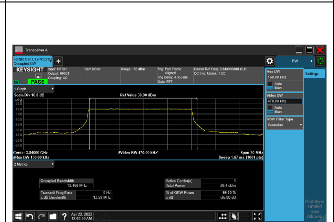
pi/2-BPSK_CH656000_15M
