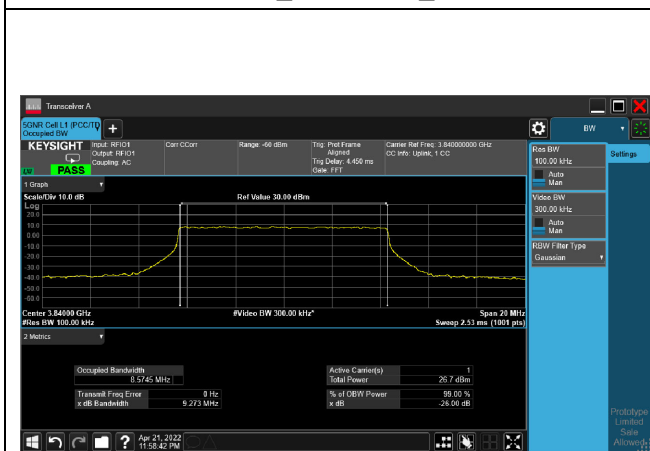
64QAM_CH656000_10M
