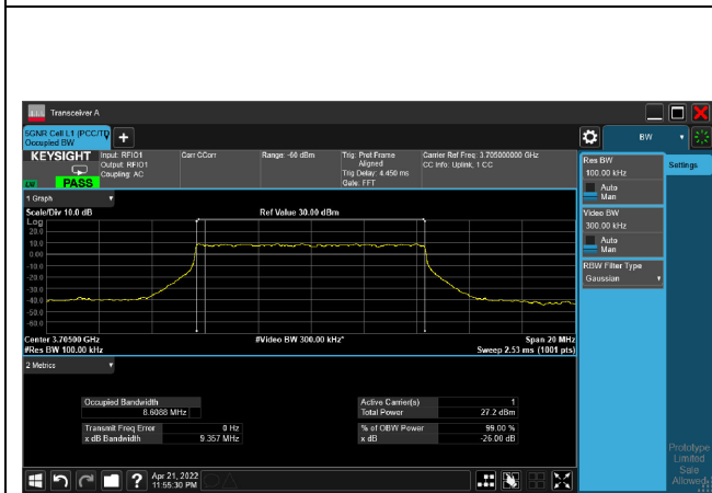
16QAM_CH647000_10M
