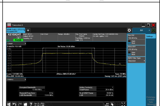
QPSK_CH664832_15M
