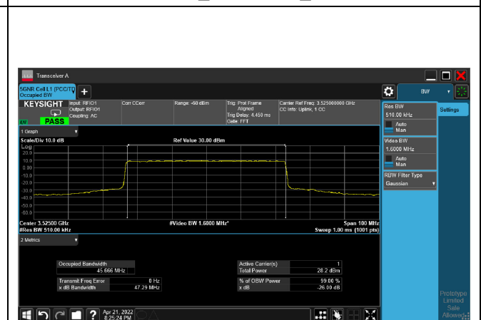
QPSK_CH635000_50M
