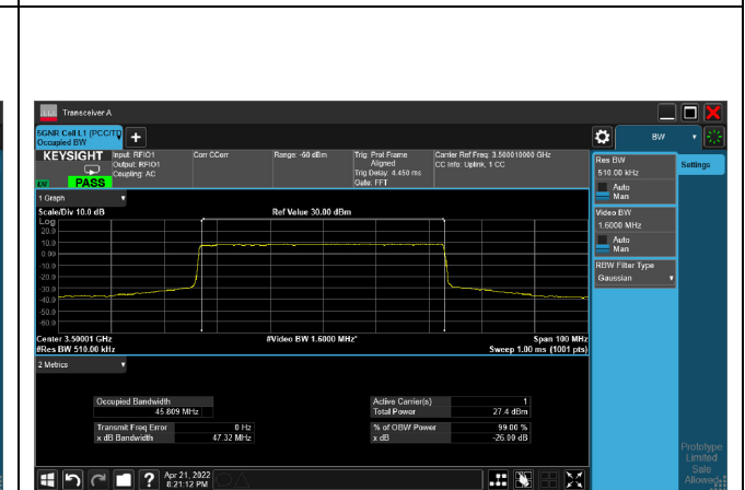
16QAM_CH633334_50M
