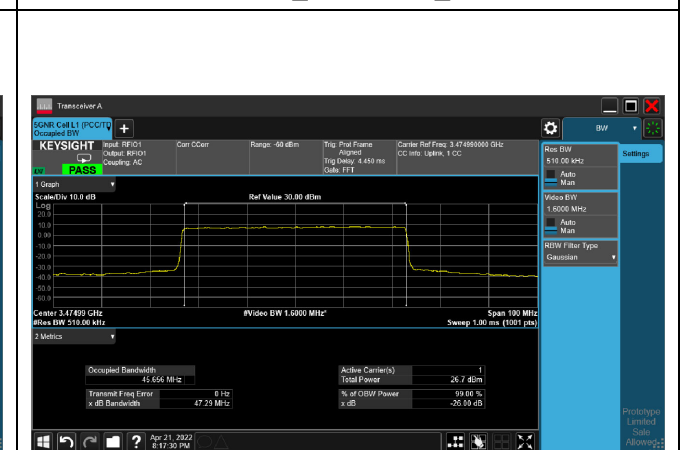
64QAM_CH631666_50M
