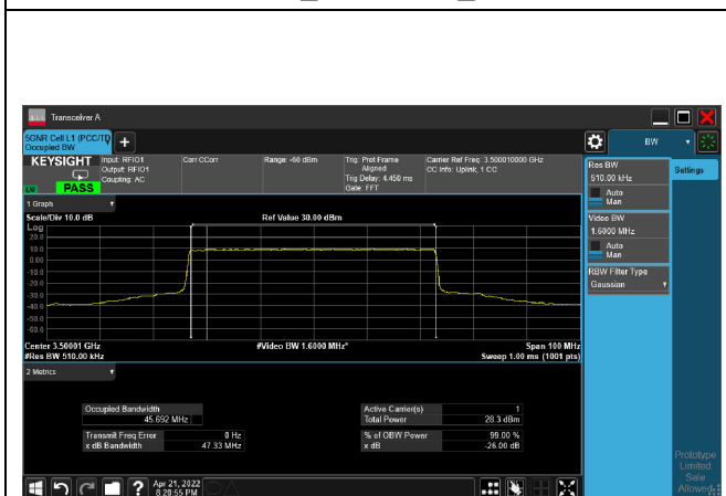
QPSK_CH633334_50M
