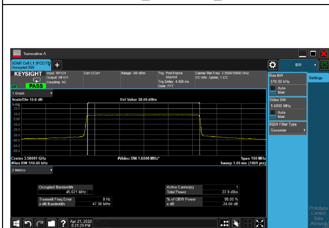
64QAM_CH633334_50M
