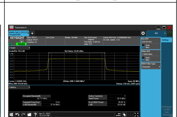
64QAM_CH635332_40M
