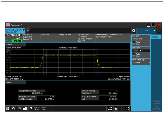
256QAM_CH635666_30M
