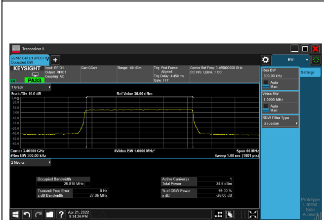
256QAM_CH631000_30M
