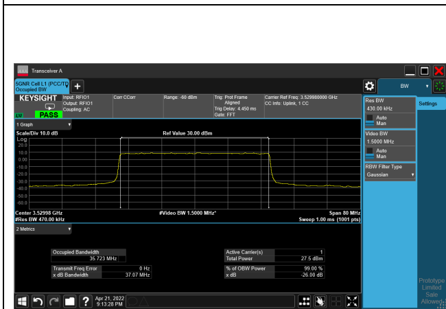
16QAM_CH635332_40M
