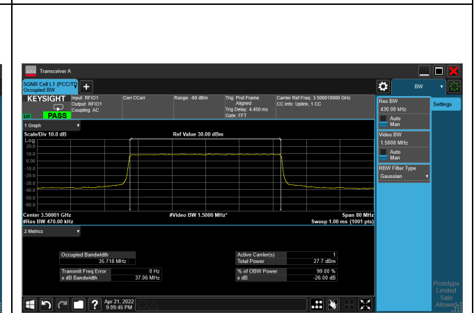
16QAM_CH633334_40M
