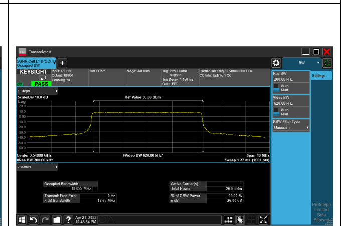
64QAM_CH636000_20M
