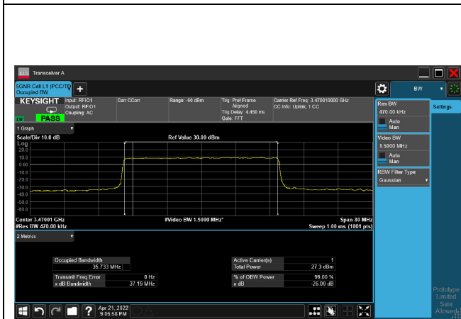
16QAM_CH631334_40M
