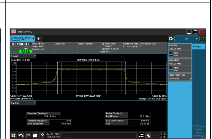
64QAM_CH630668_20M
