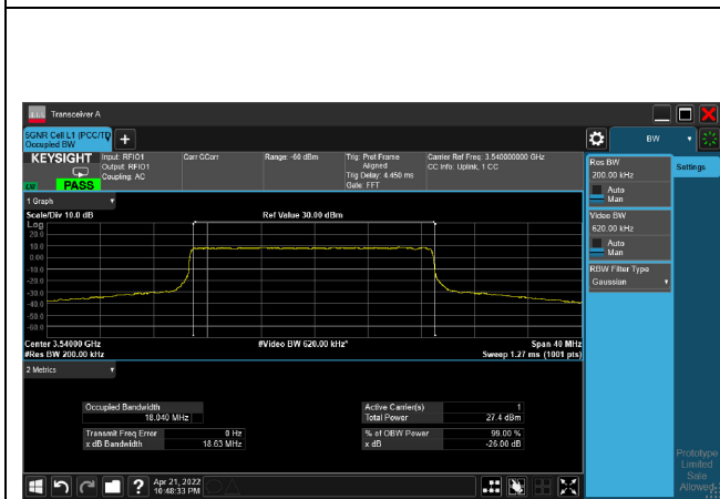
16QAM_CH636000_20M
