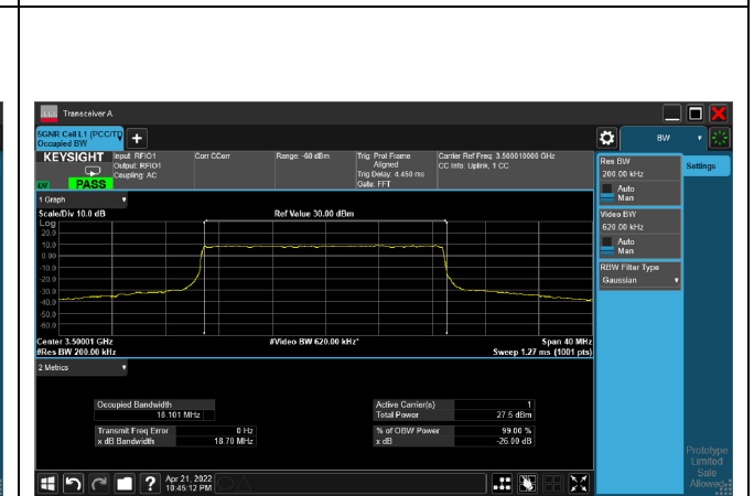
16QAM_CH633334_20M
