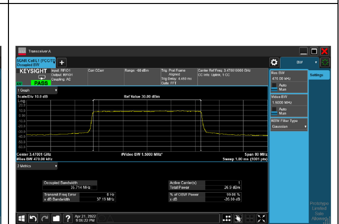
64QAM_CH631334_40M
