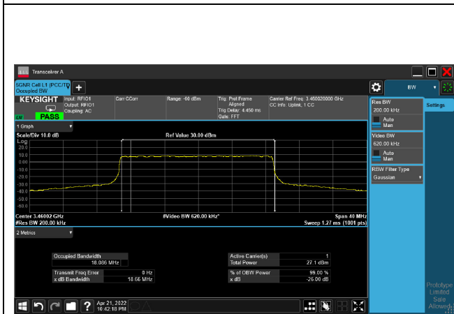
16QAM_CH630668_20M
