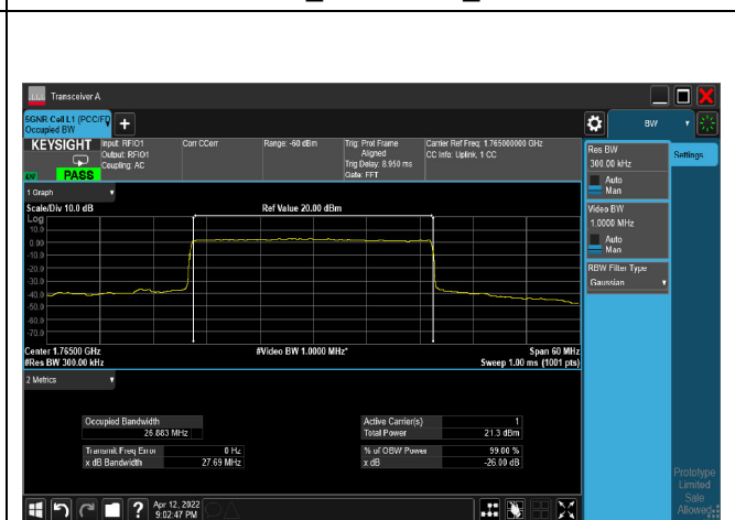
64QAM_CH353000_30M
