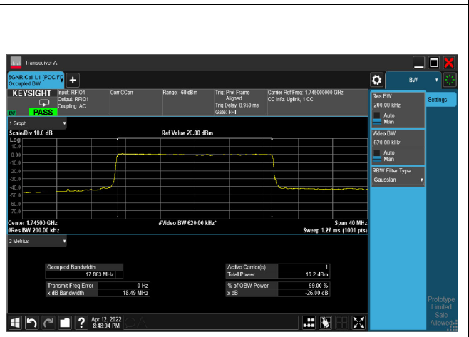
256QAM_CH349000_20M
