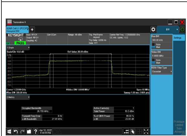
256QAM_CH345000_30M
