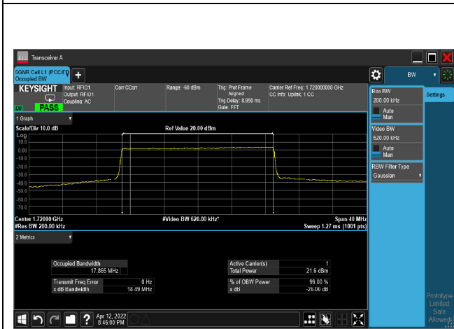
16QAM_CH344000_20M
