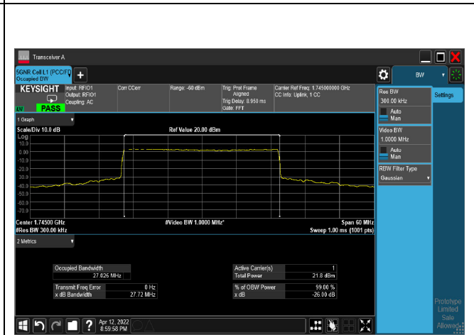
16QAM_CH349000_30M
