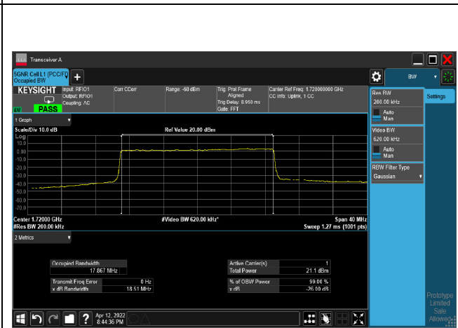
64QAM_CH344000_20M
