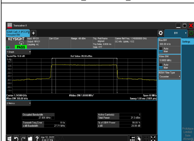
64QAM_CH349000_30M
