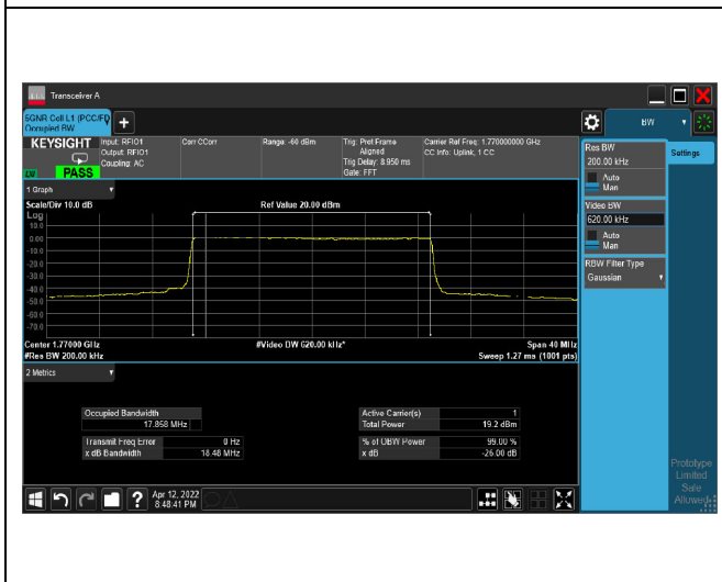
256QAM_CH354000_20M
