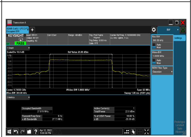
pi/2-BPSK_CH349000_30M
