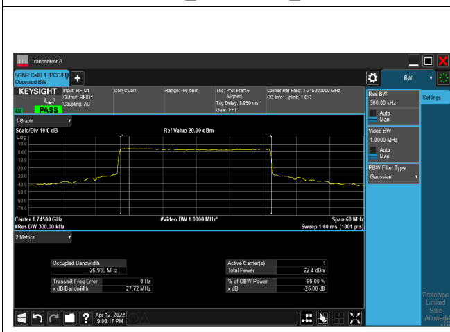
QPSK_CH349000_30M
