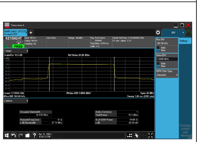
256QAM_CH349000_30M
