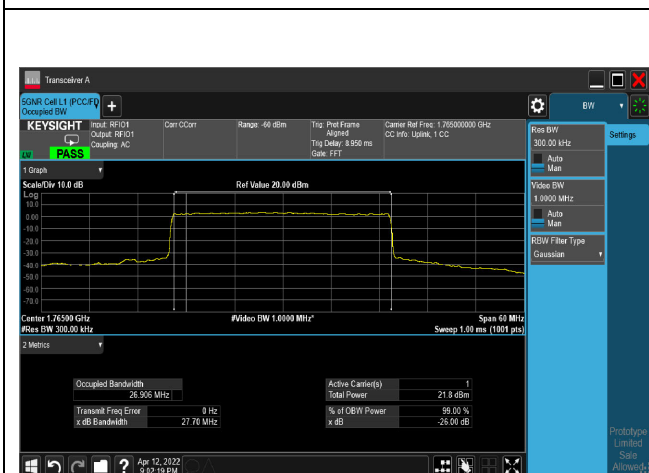
16QAM_CH353000_30M
