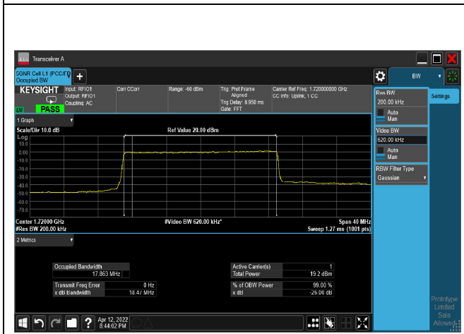
256QAM_CH344000_20M
