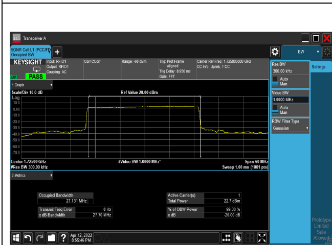
pi/2-BPSK_CH345000_30M
