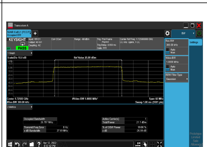
64QAM_CH345000_30M
