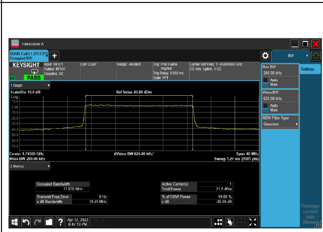
16QAM_CH349000_20M
