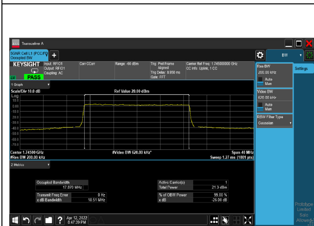
64QAM_CH349000_20M
