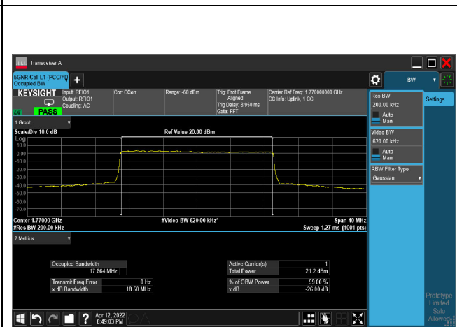
64QAM_CH354000_20M
