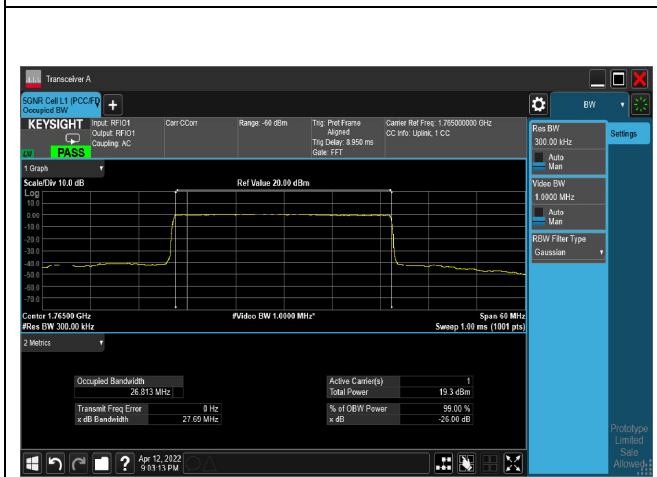
256QAM_CH353000_30M
