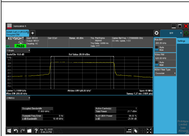
16QAM_CH354000_20M
