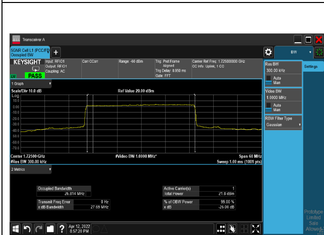
16QAM_CH345000_30M
