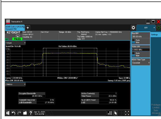
pi/2-BPSK_CH353000_30M
