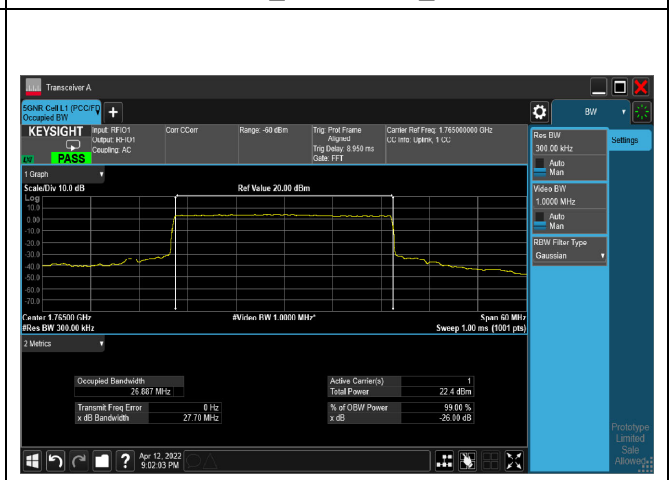
QPSK_CH353000_30M
