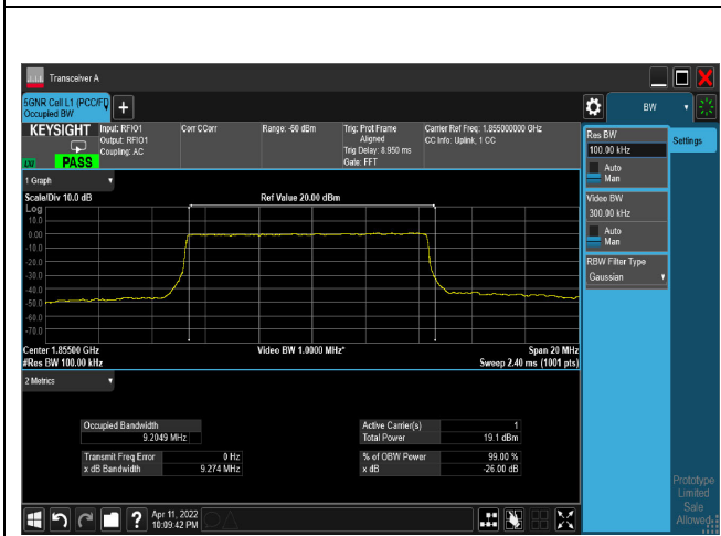
256QAM_CH371000_10M
