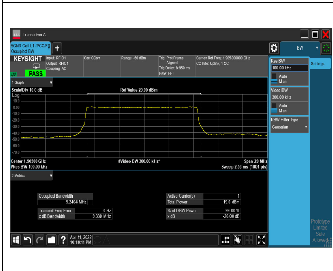
256QAM_CH381000_10M
