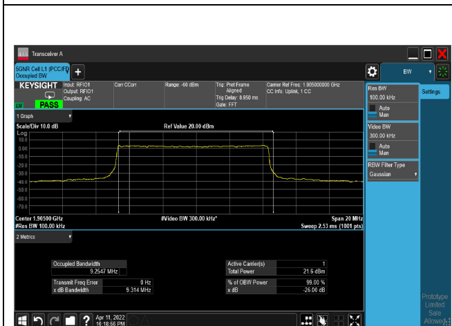
16QAM_CH381000_10M
