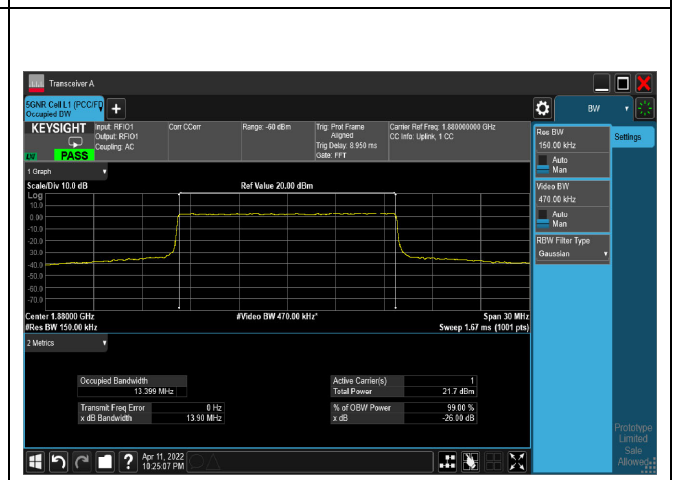
16QAM_CH376000_15M
