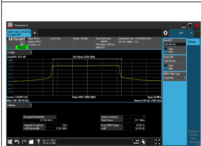
16QAM_CH371000_10M
