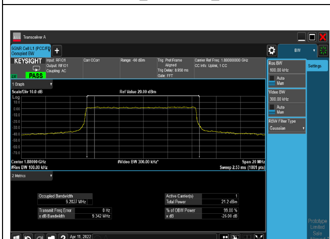
64QAM_CH376000_10M
