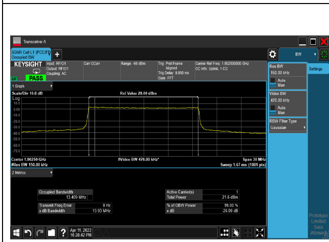
16QAM_CH380500_15M
