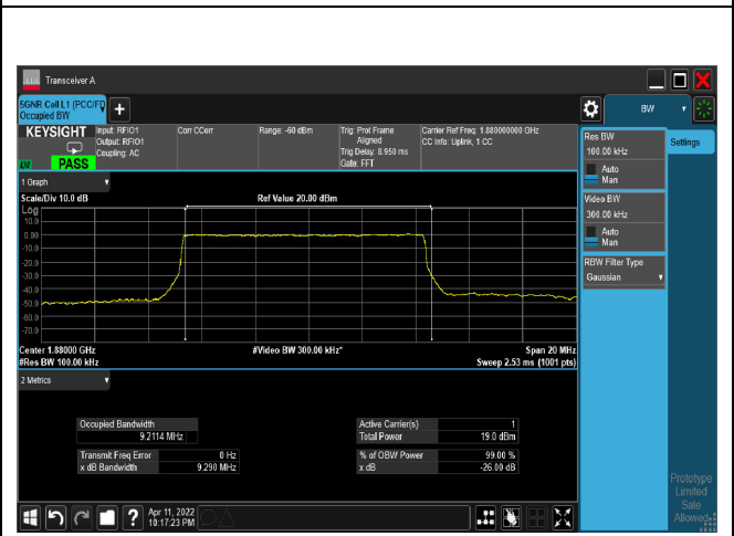
256QAM_CH376000_10M
