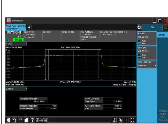
16QAM_CH371500_15M
