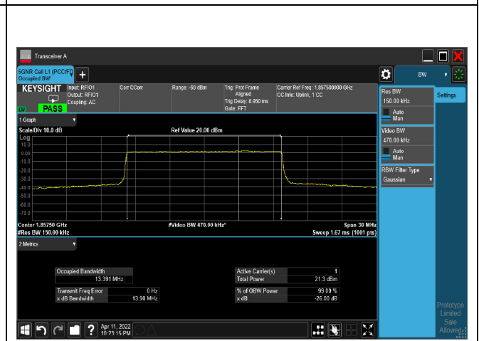
64QAM_CH371500_15M
