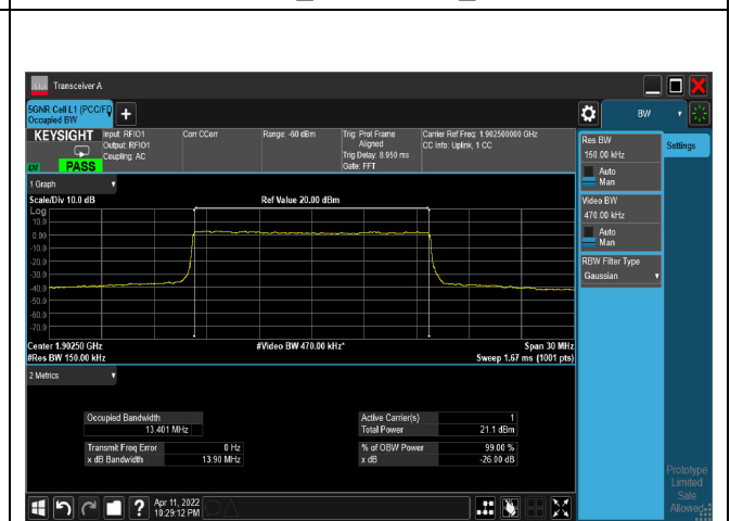
64QAM_CH380500_15M
