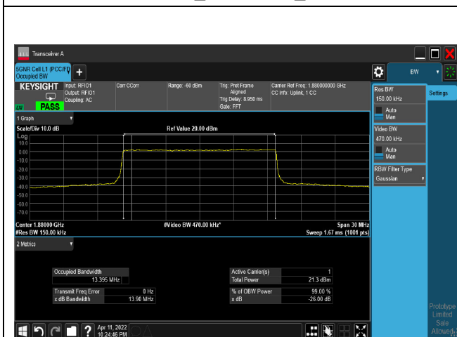
64QAM_CH376000_15M
